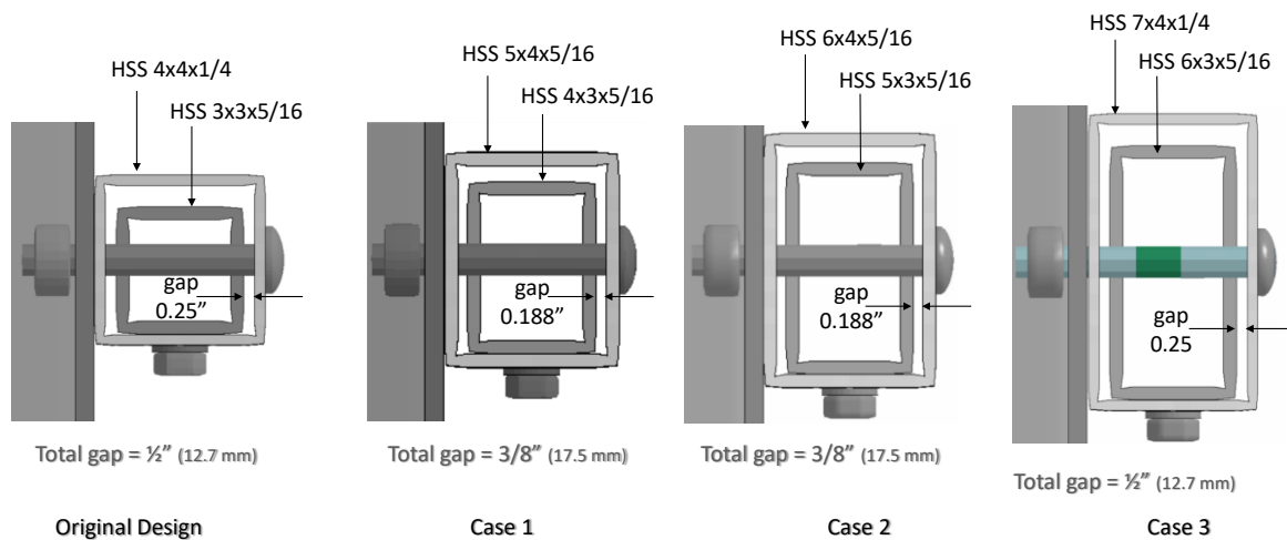
Figure 438. Cross-section view of splice for each case identifying tube size and internal gap size.
