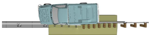
Figure 1. Sequential views from FEA and Test 401181-1 from an overhead viewpoint.
