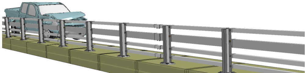
Figure R-3. [Continued] Sequential views from analysis of MASH Test 4-11 for NETC 4-Bar bridge rail from from an oblique viewpoint.
