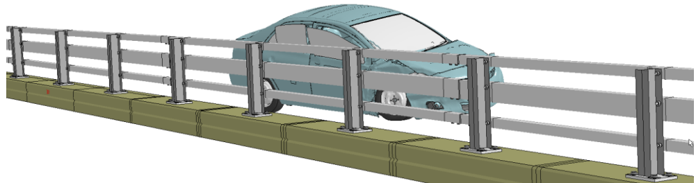
Figure J-3. [Continued] Sequential views from analysis of MASH Test 4-10 for NETC 3-Bar bridge rail from an oblique viewpoint.
