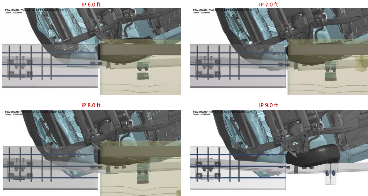
Figure 473. Test 4-21 results at time of impact with expansion splice (underneath view).
