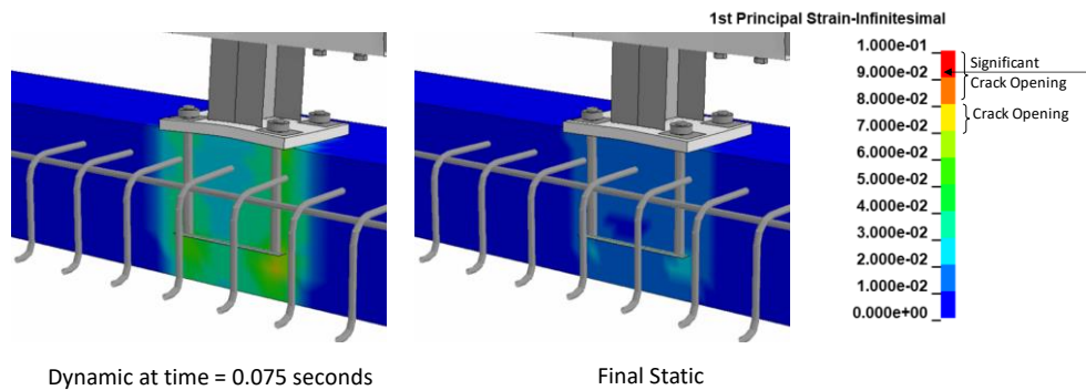
Figure 393. Contours of 1 st principal strains for concrete at the critical post for Test 3-11 on the NETC 2-bar bridge rail.
