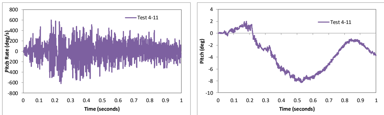
Figure 254. Pitch rate and pitch angle time-history from FEA of Test 4-11 on the NETC 4-bar bridge rail.
