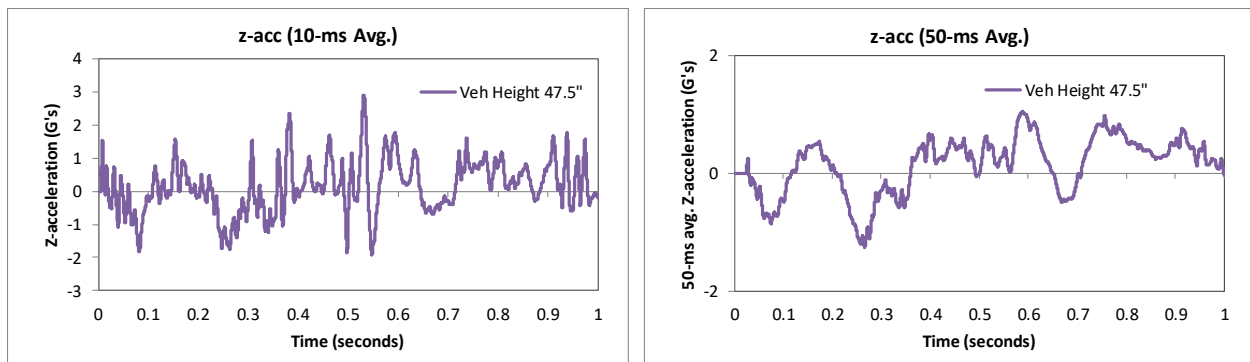
Figure 266. 10- and 50-millisecond average Z-acceleration from FEA of Test 4-12 on the NETC 4-bar bridge rail (c.g. accelerometer).
