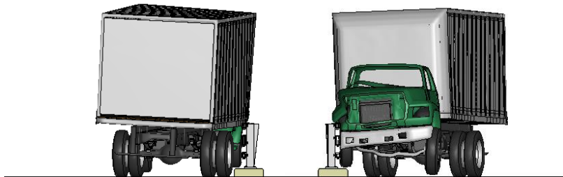
Figure M-2. Sequential views from analysis of MASH Test 4-12 for NETC 3-Bar bridge rail from upstream and downstream viewpoints – Case 2.
