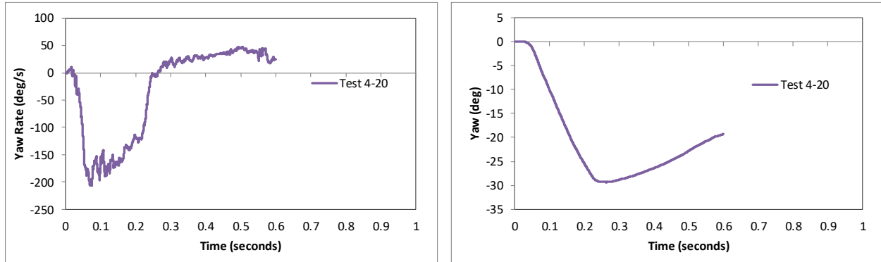
Figure 177. Yaw rate and yaw angle time-history from FEA of Test 4-20 on the 3-bar transition.
