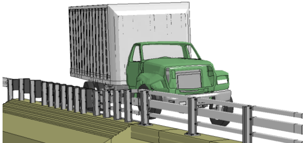
Figure P-3. Sequential views from analysis of MASH Test 4-22 for AGT 3-Bar transition from an oblique viewpoint.
