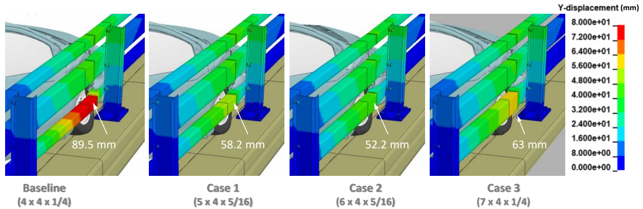
Figure 441. Oblique view showing maximum dynamic deflections of the barrier for each analysis case compared to baseline.
