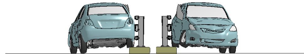
Figure J-2. Sequential views from analysis of MASH Test 4-10 for NETC 3-Bar bridge rail from upstream and downstream viewpoints.
