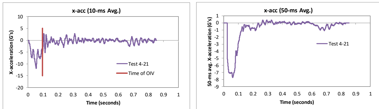
Figure 194. 10- and 50-millisecond average X-acceleration from FEA of Test 4-21 on the 3-bar transition.
