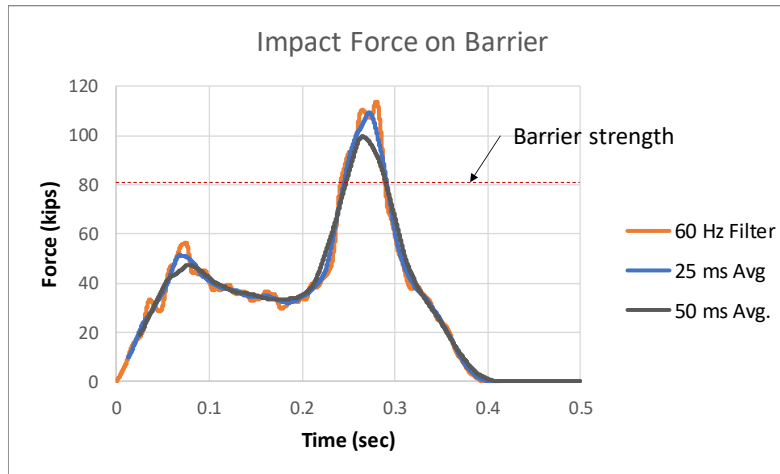
Figure 162. Lateral force-time history between vehicle and barrier for Test 4-12 on NETC 3-bar bridge rail.
