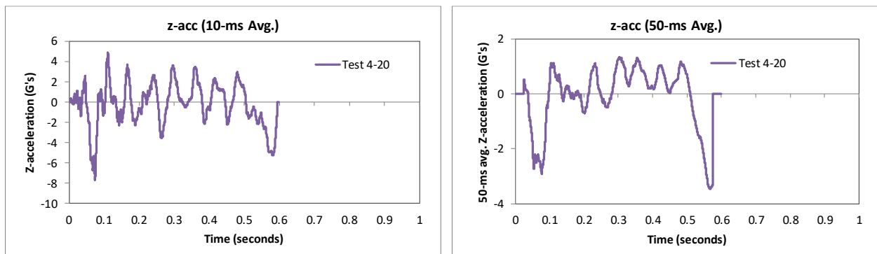
Figure 176. 10- and 50-millisecond average Z-acceleration from FEA of Test 4-20 on the 3-bar transition.
