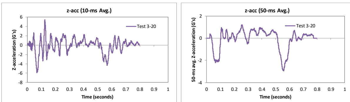
Figure 405. 10- and 50-millisecond average Z-acceleration from FEA of Test 3-20 on the 2-bar transition.
