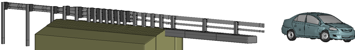
Figure Y-3. [Continued] Sequential views from analysis of MASH Test 3-20 for AGT 2-Bar bridge rail from an oblique viewpoint.
