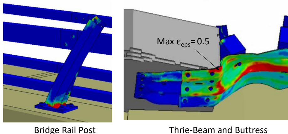
Figure 358. Close-up view of end-post on bridge rail and the high deformation area of the thrie-beam at the buttress.
