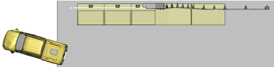
Figure U-1. [Continued] Sequential views from analysis of MASH Test 4-21 for AGT 4-Bar bridge rail from an overhead viewpoint.
