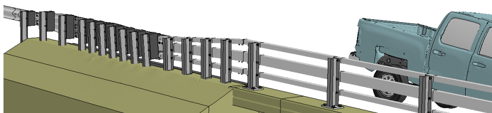
Figure O-3. [Continued] Sequential views from analysis of MASH Test 4-21 for AGT 3-Bar transition from an oblique viewpoint.
