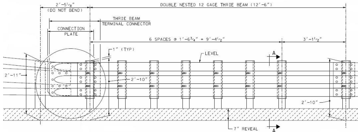
Figure 29. NHDOT T3 AGT double nested thrie-beam section.
