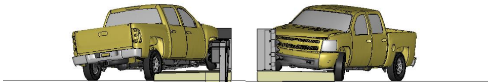
Figure U-2. Sequential views from analysis of MASH Test 4-21 for AGT 4-Bar bridge rail from upstream and downstream viewpoints.
