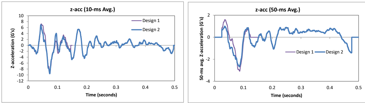
Figure 463. 10- and 50-millisecond average Z-acceleration from FEA of Test 4-20 on the 3-bar transition with 5.5-ft post spacing.
