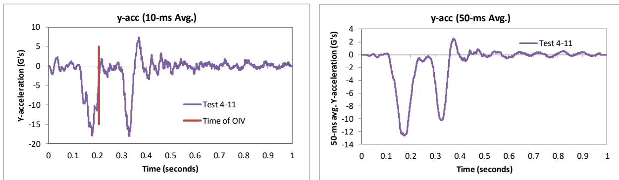
Figure 250. 10- and 50-millisecond average Y-acceleration from FEA of Test 4-11 on the NETC 4-bar bridge rail.
