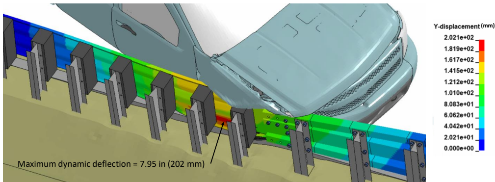
Figure 202. Contour plot of lateral displacement for Test 4-21 on the 3-bar transition at the time of maximum dynamic deflection.
