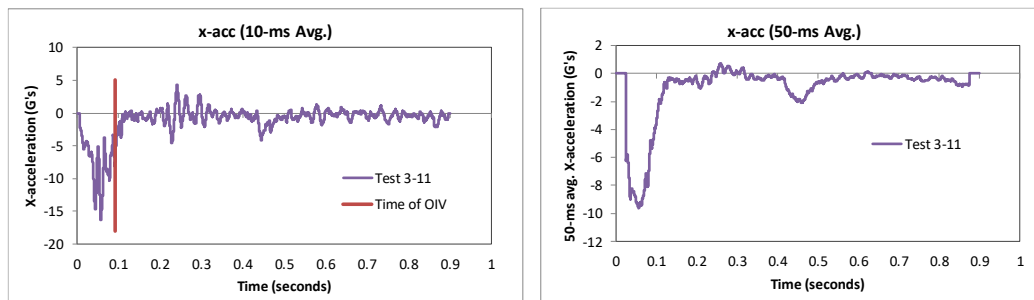
Figure 382. 10- and 50-millisecond average X-acceleration from FEA of Test 3-11 on the NETC 2-bar bridge rail.
