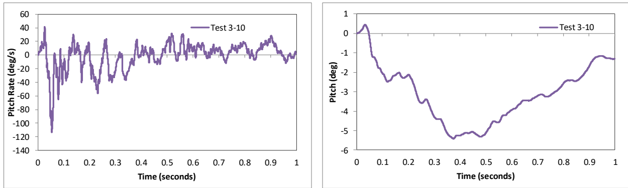
Figure 371. Pitch rate and pitch angle time-history from FEA of Test 3-10 on the NETC 2-bar bridge rail.
