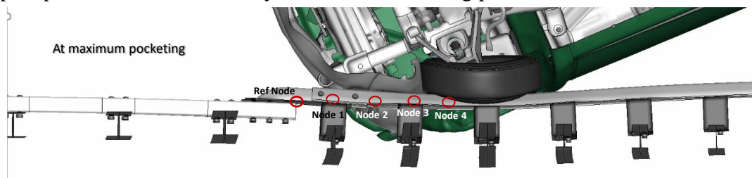
Figure 417. Measurement points for determining CIP for pocketing for Test 3-21.
