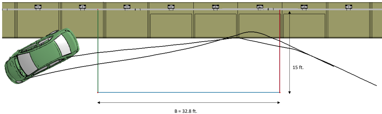
Figure 245. Exit box for Test 4-10 analysis of the NETC 4-bar bridge rail.
