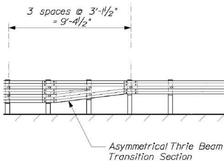
Figure 32. MaineDOT Type IA AGT asymmetrical w-beam to thrie-beam transition section.
