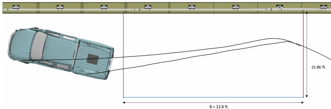
Figure 144. Exit box for Test 4-11 analysis of the NETC 3-bar bridge rail.
