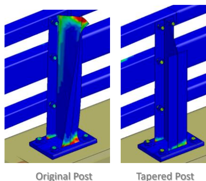
Figure 493. Typical damage to Post 1 of the bridge rail for original (non-tapered) and modified (tapered) post designs.
