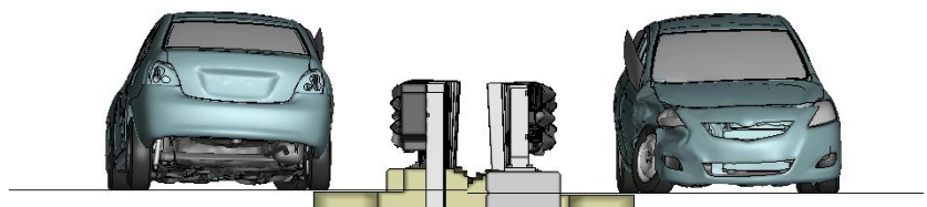
Figure Y-2. [Continued] Sequential views from analysis of MASH Test 3-20 for AGT 2-Bar bridge rail from upstream and downstream viewpoints.
