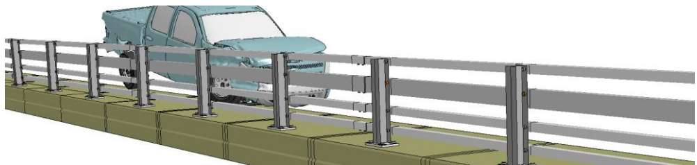
Figure R-3. [Continued] Sequential views from analysis of MASH Test 4-11 for NETC 4-Bar bridge rail from an oblique viewpoint.
