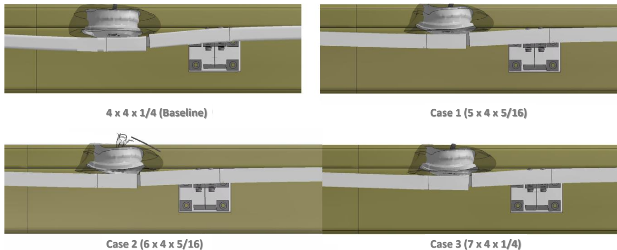
Figure 440. Overhead transparent view showing maximum deflections of the lower rail for each analysis case compared to baseline.
