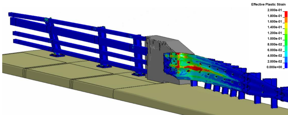
Figure 357. Contours of effective plastic strains on the transition and bridge rail for Test 4-22 on the MaineDOT transition.
