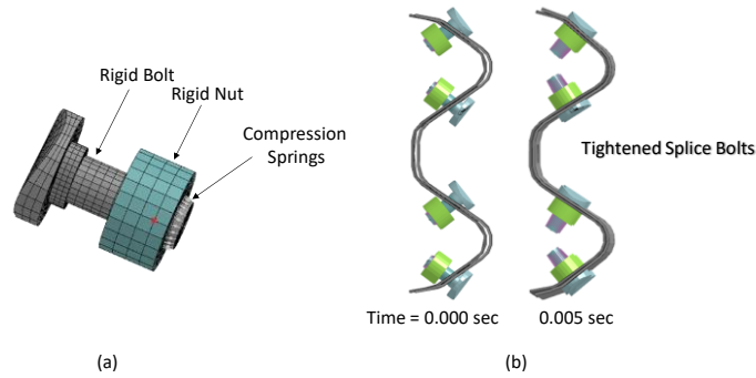
Figure 88. (a) FEA mesh for splice bolt and (b) profile of splice before and after tightening splice bolt tightening.
