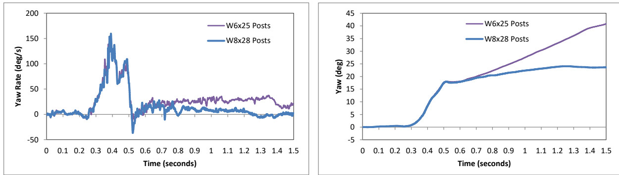
Figure 503. Yaw rate and yaw angle time-history from FEA of Test 4-12 on the baseline and modified NETC 4-bar bridge rail (c.g. accelerometer).
