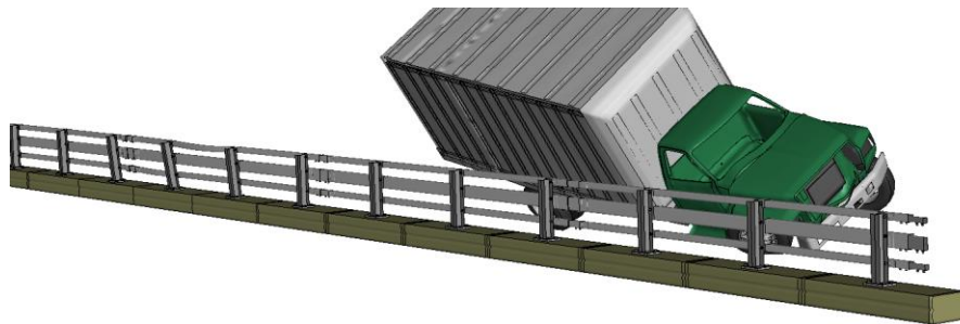
Figure M-3. [Continued] Sequential views from analysis of MASH Test 4-12 for NETC 3-Bar bridge rail from an oblique viewpoint – Case 2.
