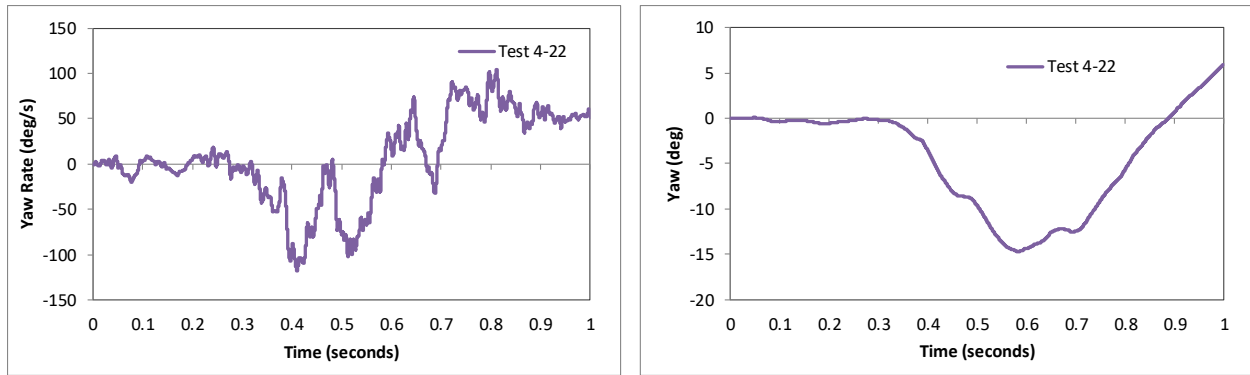
Figure 352. Yaw rate and yaw angle time-history from FEA of Test 4-22 on the MaineDOT transition (cabin accelerometer).
