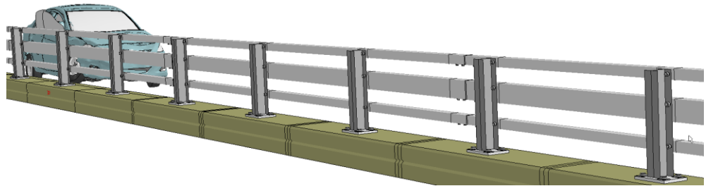
Figure J-3. Sequential views from analysis of MASH Test 4-10 for NETC 3-Bar bridge rail from an oblique viewpoint.
