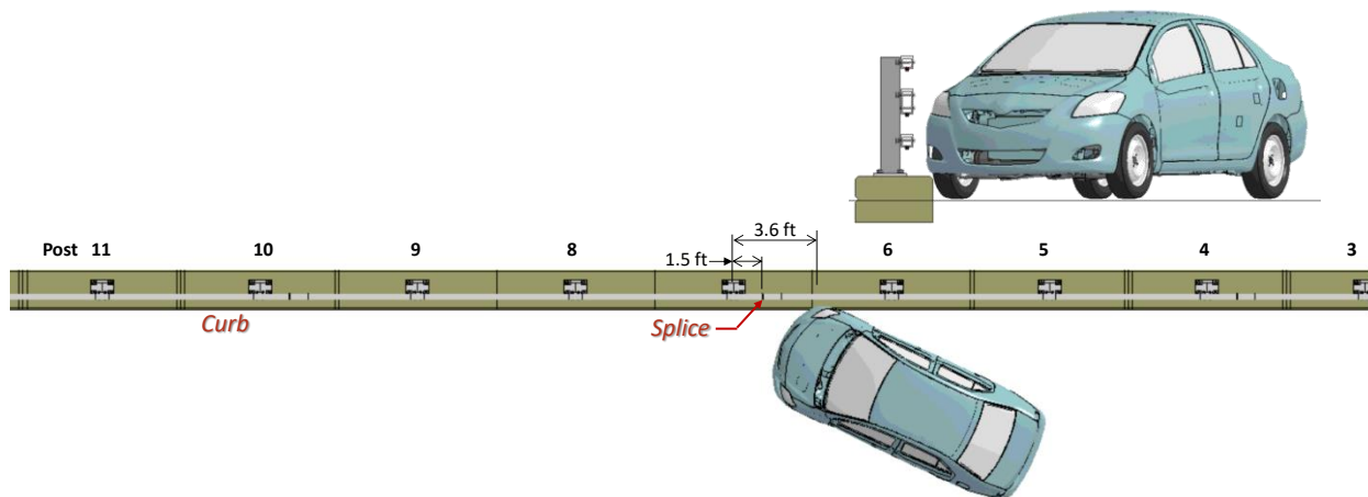
Figure 439. Impact point for Test 4-10 on the Modified NETC 3-bar bridge rail.
