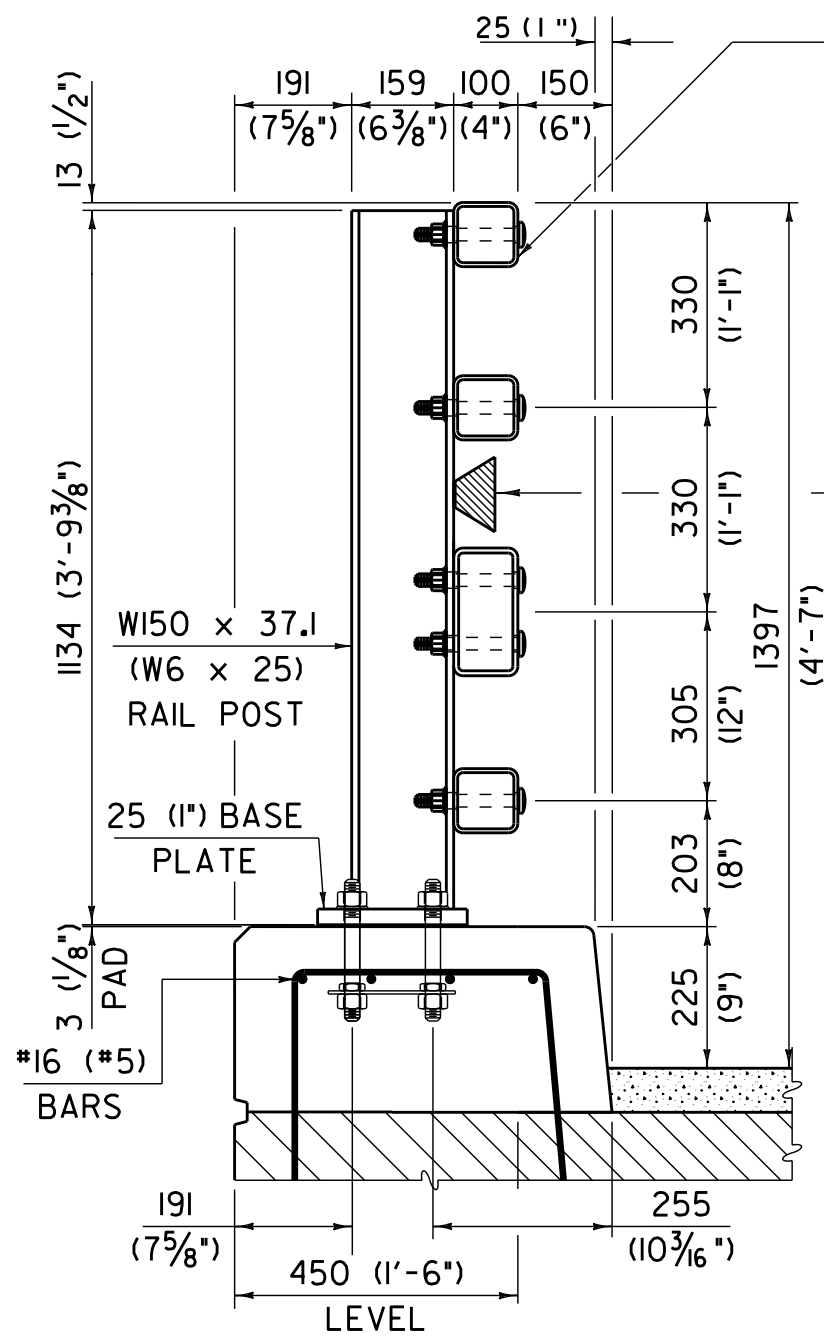
TYPICAL SECTION
