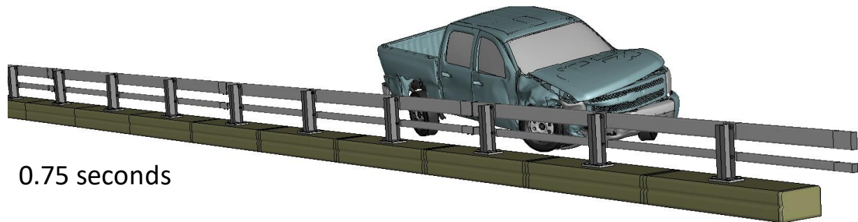
Figure X-3. [Continued] Sequential views from analysis of MASH Test 3-11 for NETC 2-Bar bridge rail from an oblique viewpoint.
