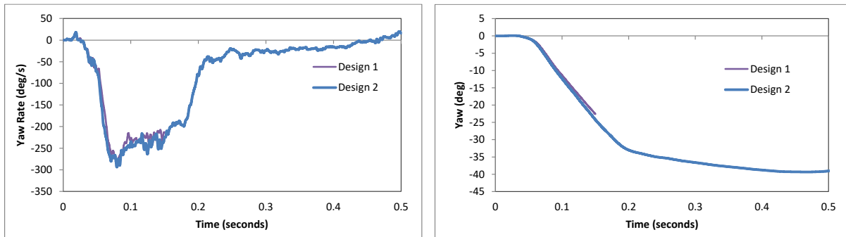
Figure 464. Yaw rate and yaw angle time-history from FEA of Test 4-20 on the 3-bar transition with 5.5-ft post spacing.
