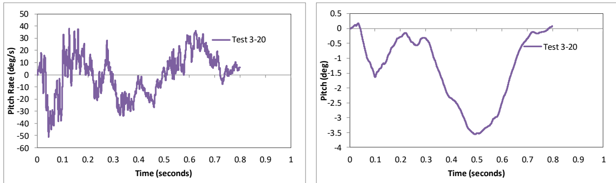
Figure 408. Pitch rate and pitch angle time-history from FEA of Test 3-20 on the 2-bar transition.
