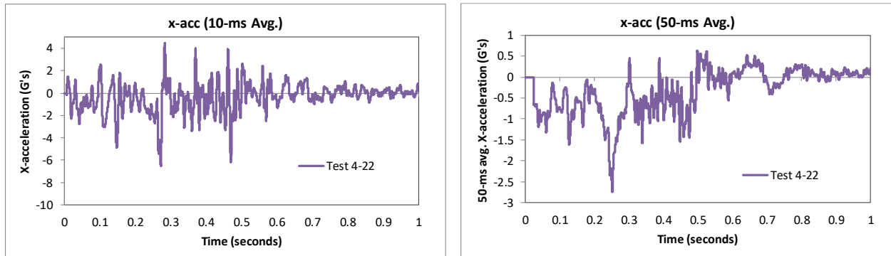
Figure 212. 10- and 50-millisecond average X-acceleration from FEA of Test 4-22 on the 3-bar transition (c.g. accelerometer).
