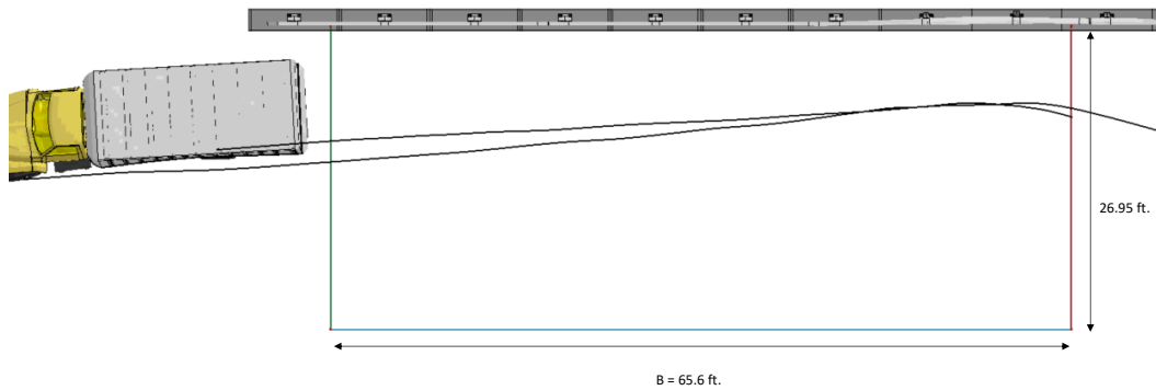
Figure 164. Exit box for Test 4-12 for Case 1 on the NETC 3-bar bridge rail.
