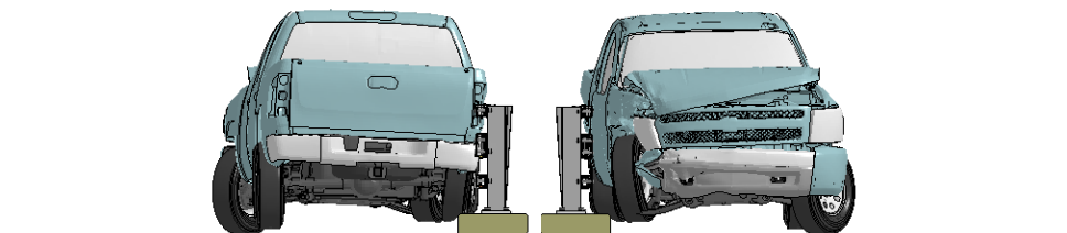
Figure K-2. Sequential views from analysis of MASH Test 4-11 for NETC 3-Bar bridge rail from upstream and downstream viewpoints.
