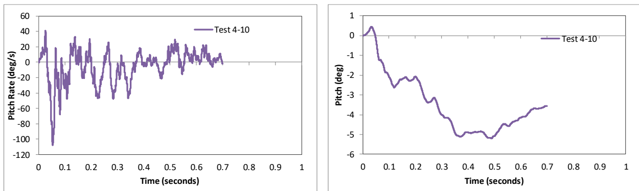
Figure 120. Pitch rate and pitch angle time-history from FEA of Test 4-10 on the NETC 3-bar bridge rail.
