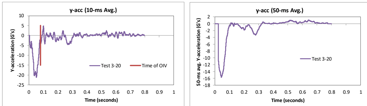
Figure 404. 10- and 50-millisecond average Y-acceleration from FEA of Test 3-20 on the 2-bar transition.
