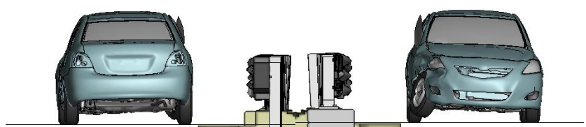
Figure Y-2. [Continued] Sequential views from analysis of MASH Test 3-20 for AGT 2-Bar bridge rail from upstream and downstream viewpoints.
