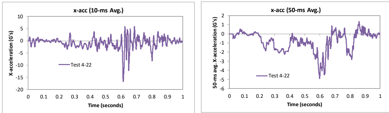
Figure 346. 10- and 50-millisecond average X-acceleration from FEA of Test 4-22 on the MaineDOT transition (c.g. accelerometer).
