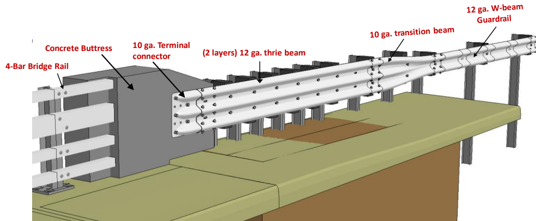
Figure 285. FEA model illustrating the various components of the system.
