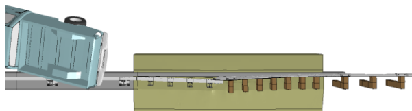
Figure 97. [Continued] Sequential views of FE analysis and Test 401181-1 from an overhead viewpoint.
