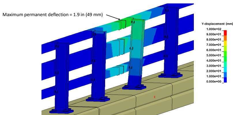
Figure 140. Contour plot of maximum permanent deflection of the bridge rail for test 4-11.
