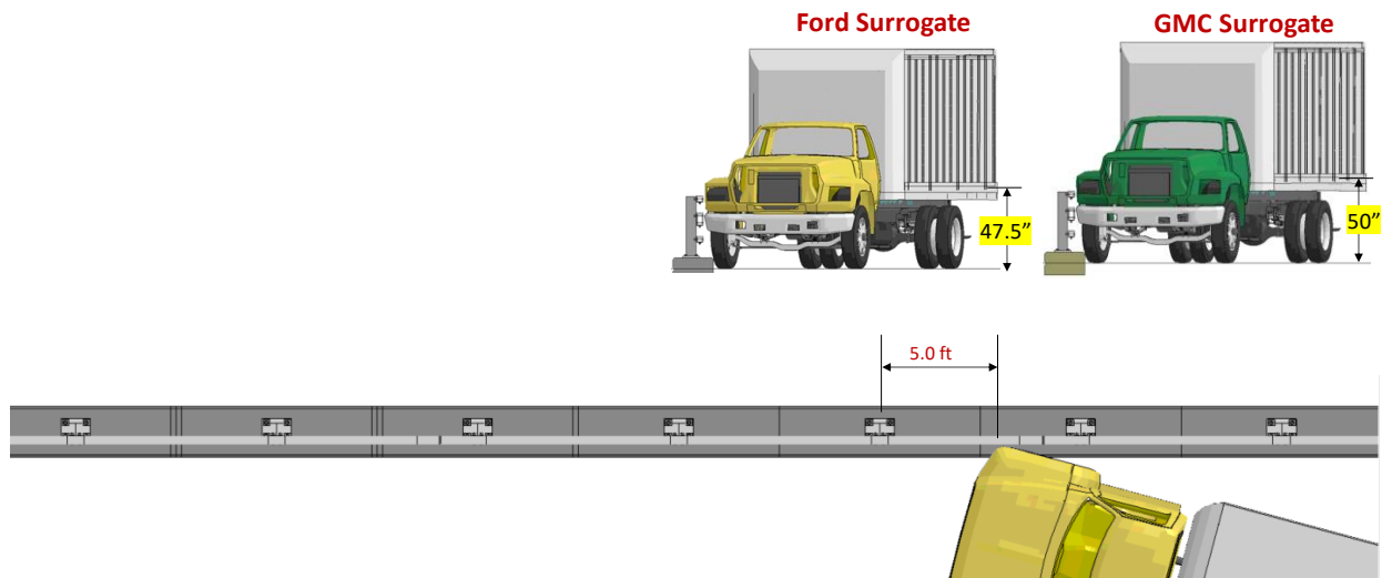
Figure 146. Impact point for Test 4-12 on the NETC 3-bar bridge rail.
