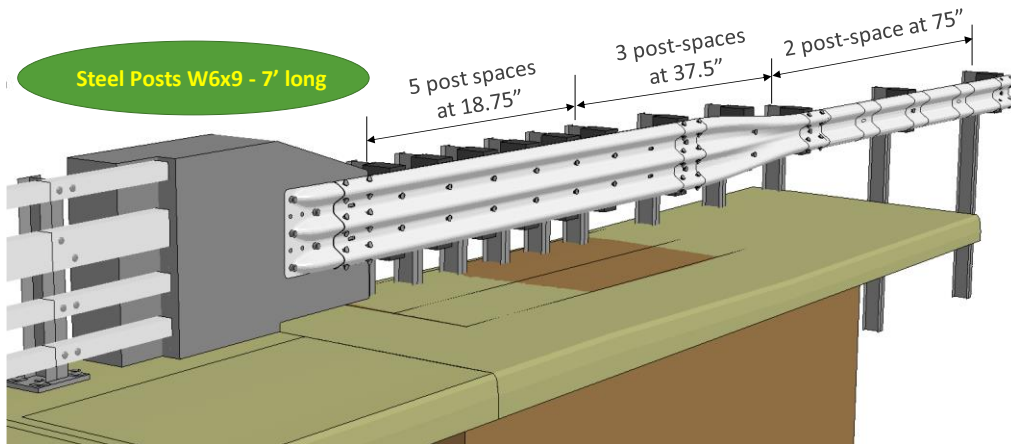
Figure 286. FEA model illustrating the post types and post spacing.
