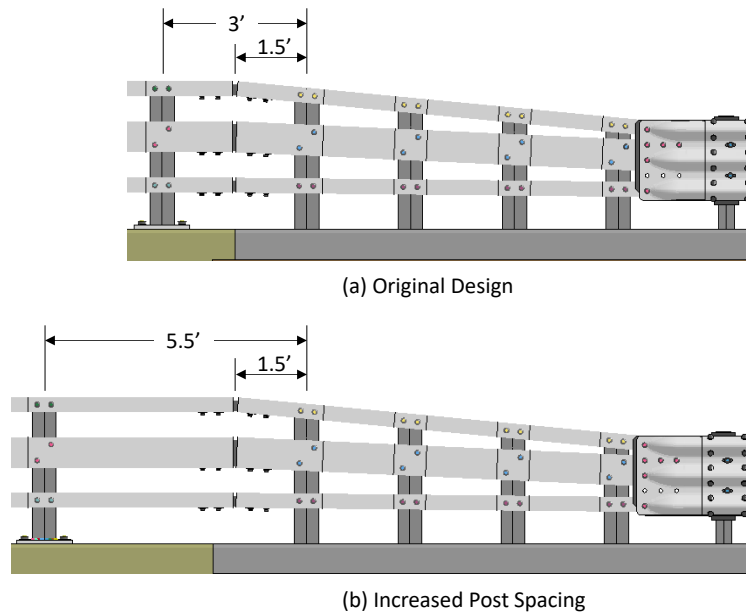
Figure 450. Post and splice spacing for (a) original and (b) modified designs.
