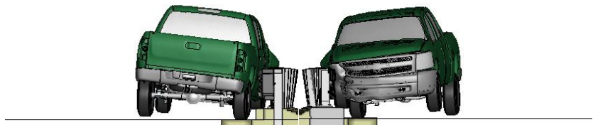
Figure Z-2. Sequential views from analysis of MASH Test 3-21 for AGT 2-Bar bridge rail from upstream and downstream viewpoints.
