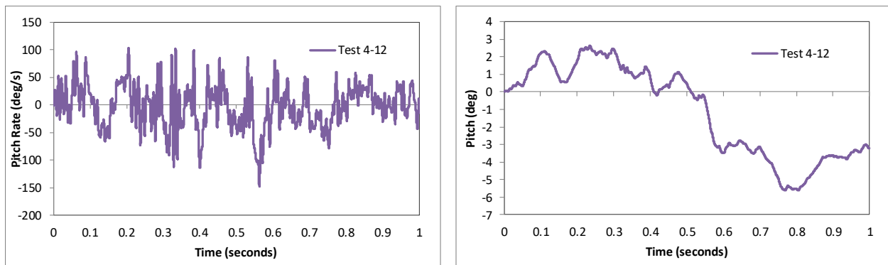
Figure 272. Pitch rate and pitch angle time-history from FEA of Test 4-12 on the NETC 4-bar bridge rail (cabin accelerometer).
