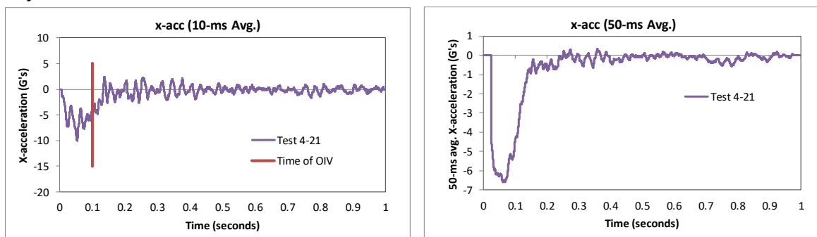
Figure 424. 10- and 50-millisecond average X-acceleration from FEA of Test 3-21 on the 3-bar transition.
