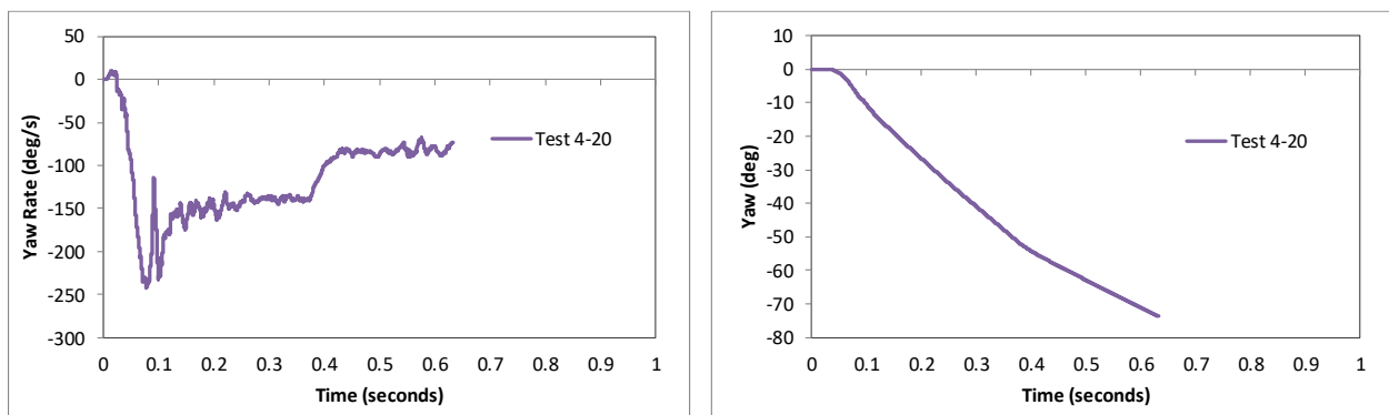
Figure 300. Yaw rate and yaw angle time-history from FEA of Test 4-20 on the MaineDOT transition.
