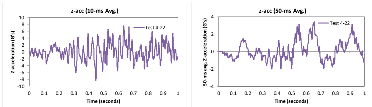
Figure 351. 10- and 50-millisecond average Z-acceleration from FEA of Test 4-22 on the MaineDOT transition (cabin accelerometer).
