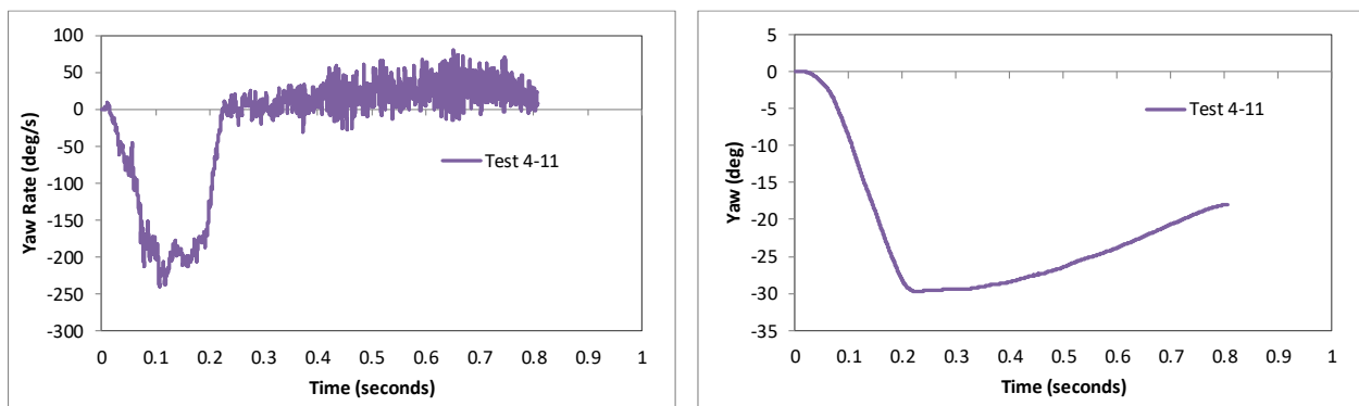
Figure 134. Yaw rate and yaw angle time-history from FEA of Test 4-11 on the NETC 3-bar bridge rail.
