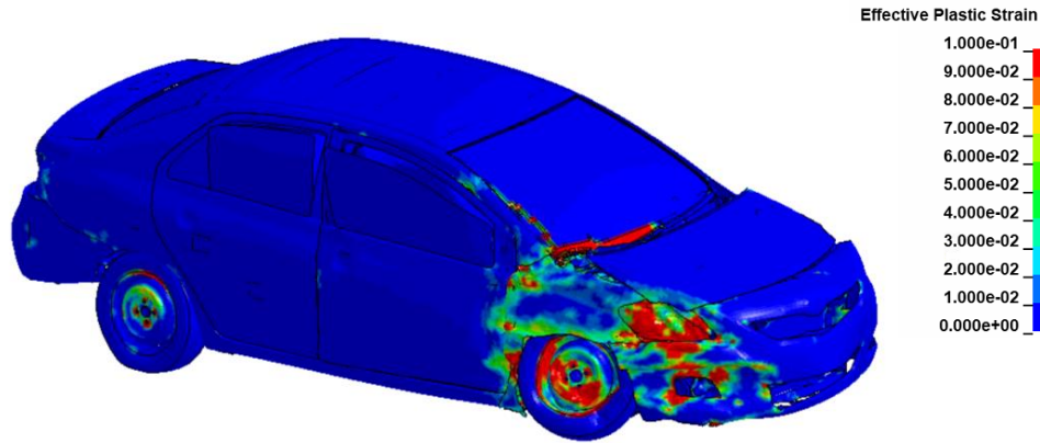
Figure 127. Damages to vehicle in Test 4-10 analysis of the NETC 3-bar bridge rail.
