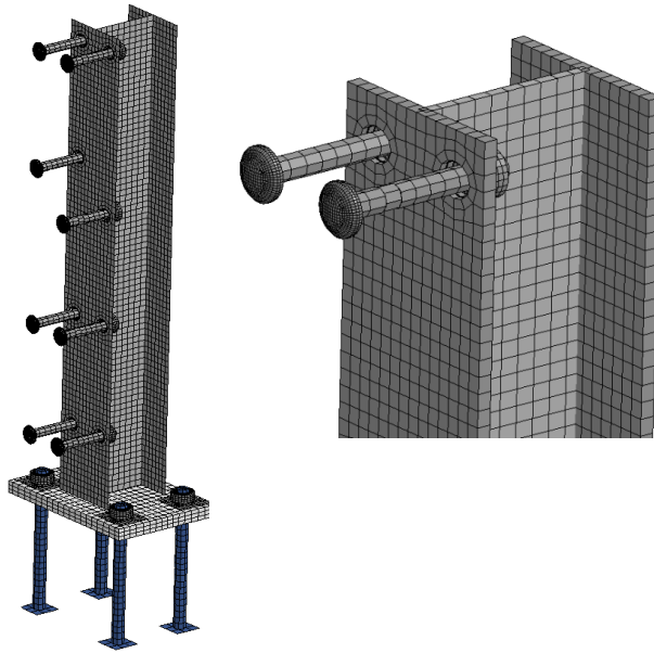
Figure 51. FEA Model of bridge rail post.
