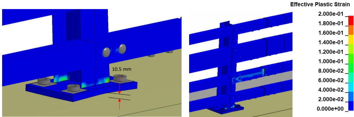
Figure 242. Contours of effective plastic strains for Test 4-10 on the NETC 4-bar bridge rail.
