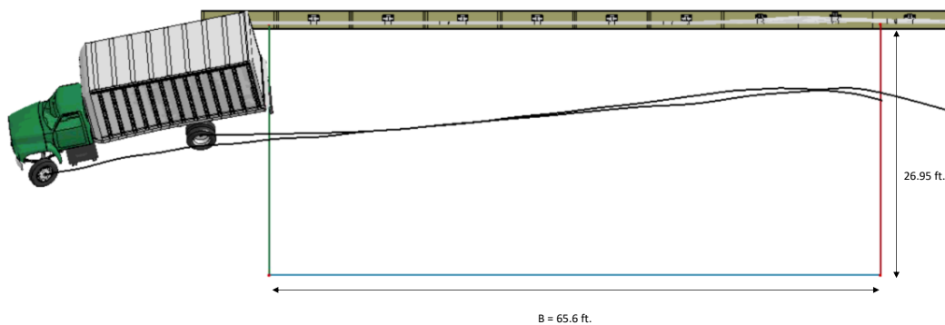
Figure 165. Exit box for Test 4-12 for Case 2 on the NETC 3-bar bridge rail.
