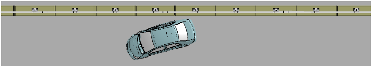
Figure J-1. [Continued] Sequential views from analysis of MASH Test 4-10 for NETC 3-Bar bridge rail from an overhead viewpoint.
