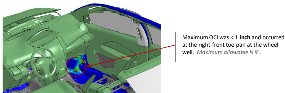
Figure 180. Occupant compartment deformation resulting from Test 4-20 on the 3-bar transition.
