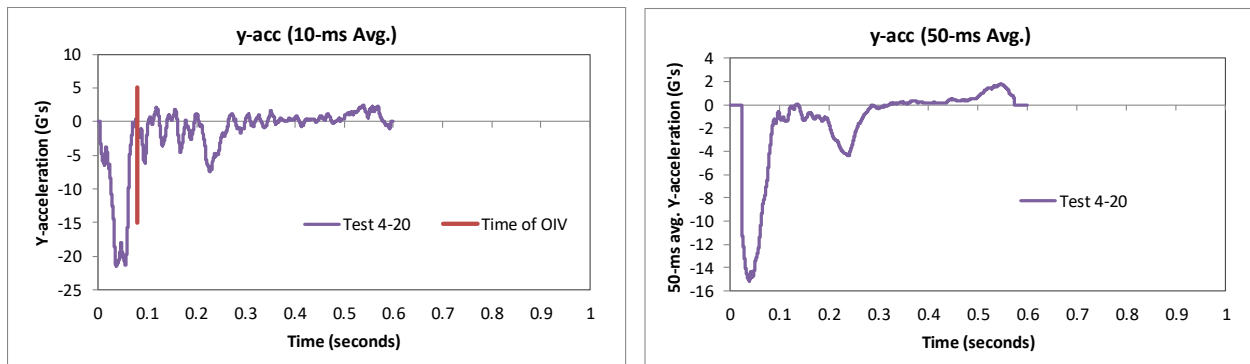
Figure 175. 10- and 50-millisecond average Y-acceleration from FEA of Test 4-20 on the 3-bar transition.
