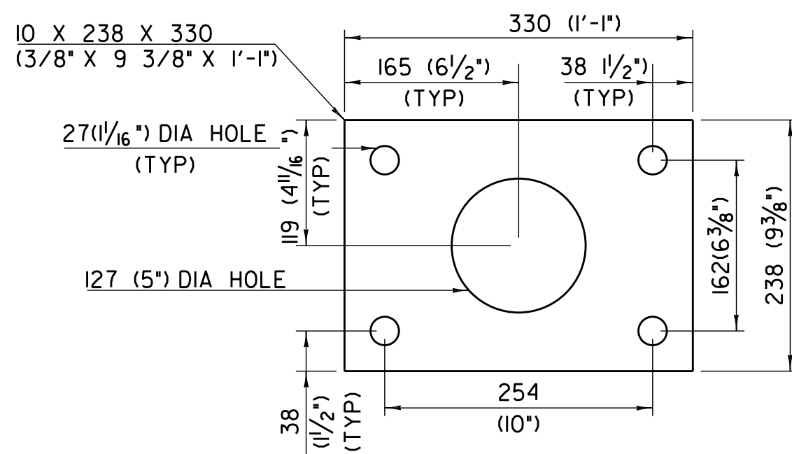
ANCHOR PLATE
