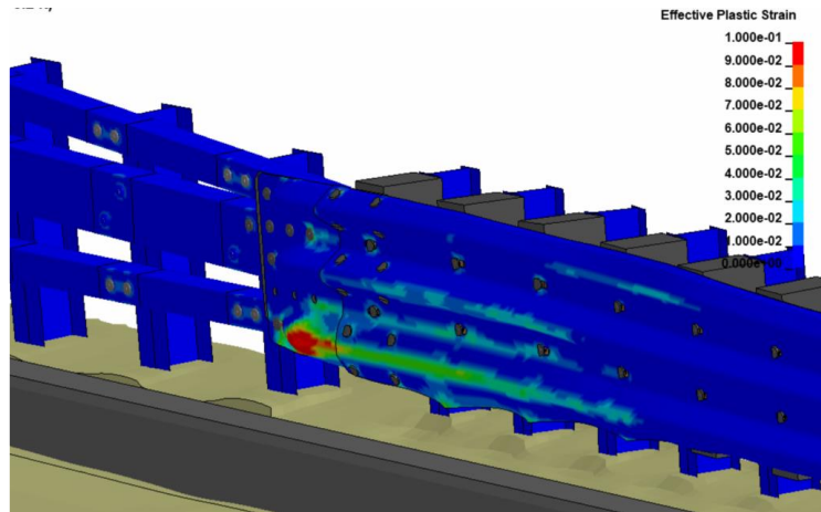
Figure 204. Contours of effective plastic strains on the steel rails and posts for Test 4-21 on 3-bar transition.
