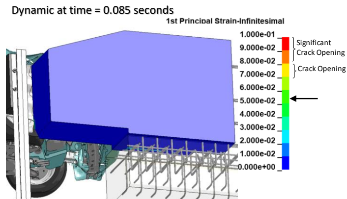
Figure 308. Contour plot of 1 st principle strain on concrete buttress.
