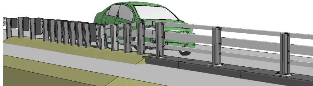
Figure N-3. Sequential views from analysis of MASH Test 4-20 for AGT 3-Bar transition from an oblique viewpoint.
