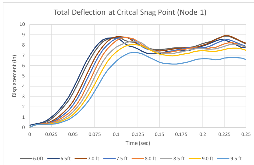
Figure 419. Total deflection of the rail at the critical snag point on the transition for Test 3-21.
