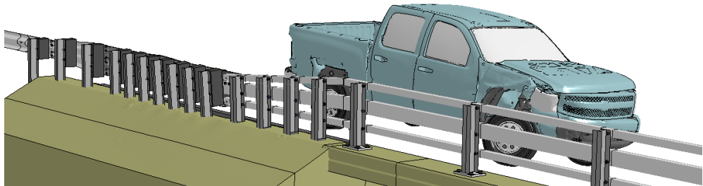
Figure O-3. [Continued] Sequential views from analysis of MASH Test 4-21 for AGT 3-Bar transition from from an oblique viewpoint.
