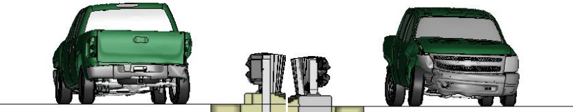
Figure Z-2. [Continued] Sequential views from analysis of MASH Test 3-21 for AGT 2-Bar bridge rail from upstream and downstream viewpoints.
