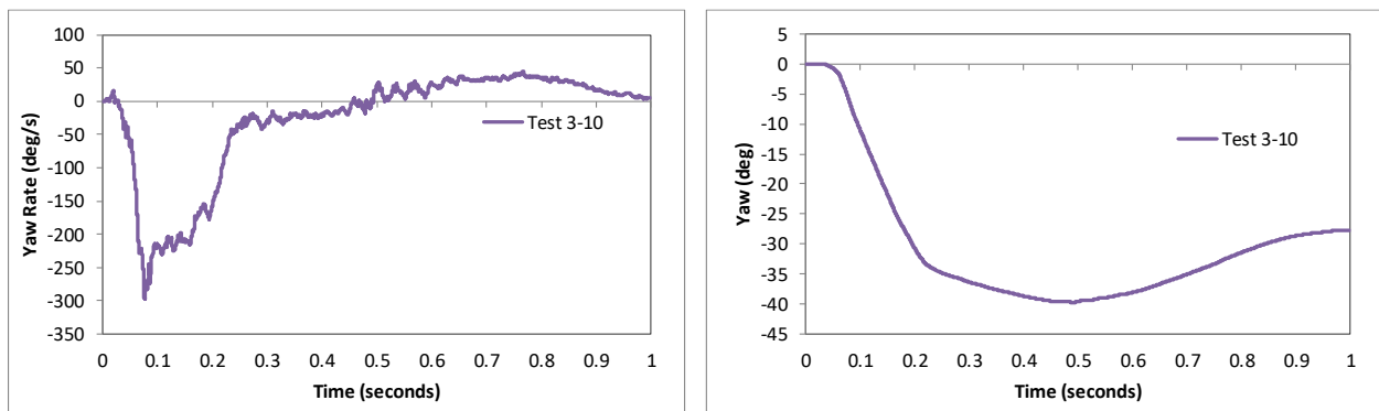
Figure 369. Yaw rate and yaw angle time-history from FEA of Test 3-10 on the NETC 2-bar bridge rail.
