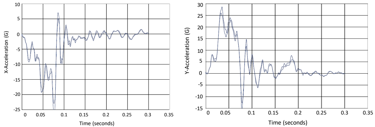
Figure 314. Overlay of the accelerations from Slice 1 and Slice 2 from full-scale test 34AGT-2. [Rosenbaugh19]
