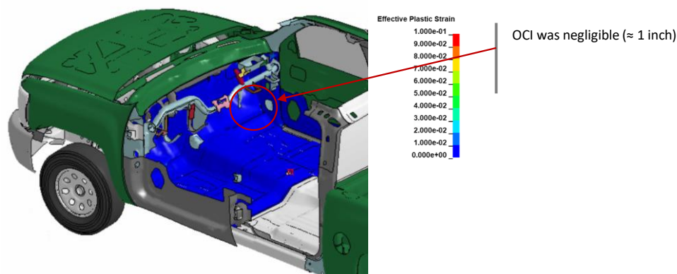
Figure 430. Occupant compartment deformation resulting from Test 3-21 on the 2-bar transition.
