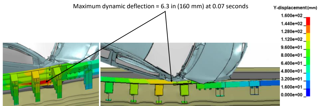
Figure 411. Contour plot of lateral displacement for the transition at the time of maximum dynamic deflection.
