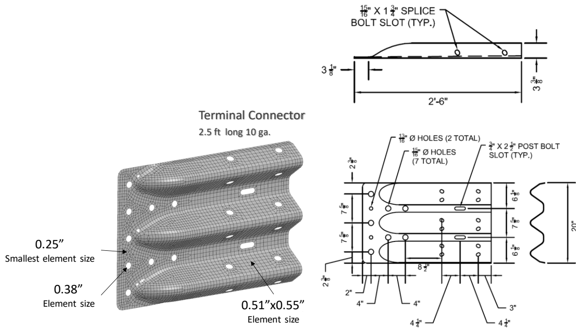
Figure 85. FEA mesh for the thrie-beam end-shoe terminal connector.
