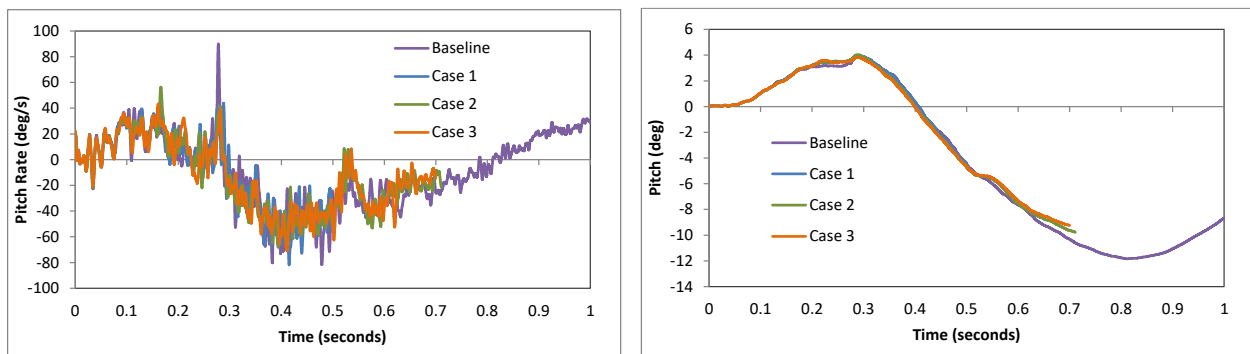
Figure 489. Pitch rate and pitch angle time-history from FEA of Test 4-22 for Case 1-3 on the 3-bar transition with 5.5-ft post spacing compared with baseline (c.g. accelerometer).
