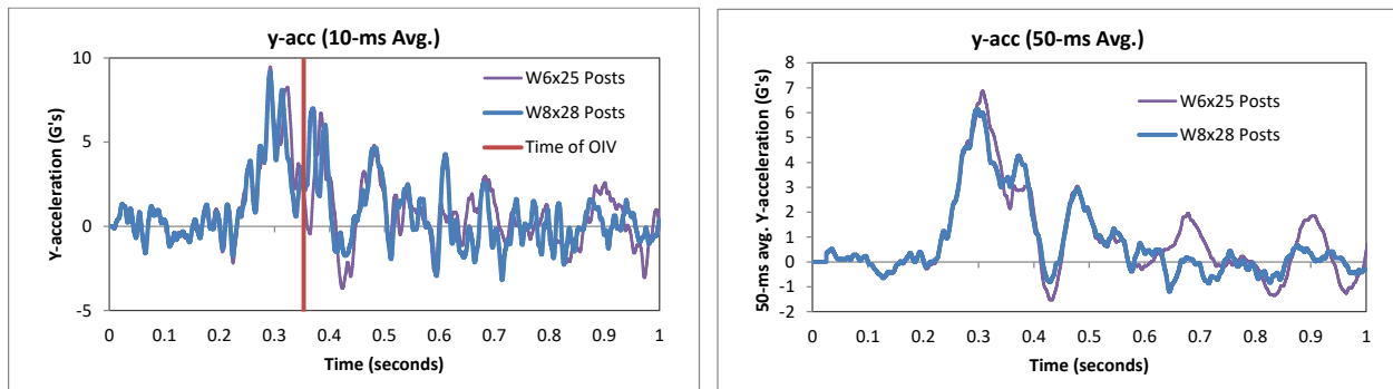
Figure 498. 10- and 50-millisecond average Y-acceleration from FEA of Test 4-12 on the baseline and modified NETC 4-bar bridge rail (cabin accelerometer).
