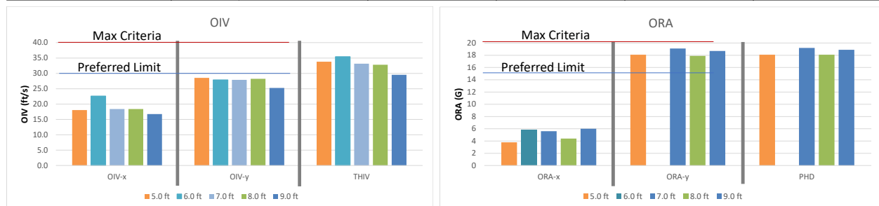
Figure 477. Graphical representation of OIV, THIV, ORA and PHD metrics for Test 4-21.
