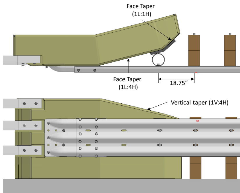
Figure 36. Plan and profile view of the shaped buttress.
