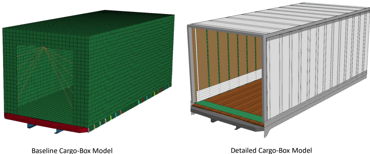
Figure 42. Images of the FEA model for the baseline and detailed cargo-box models (rear door not shown to facilitate viewing inside of cargo box).
