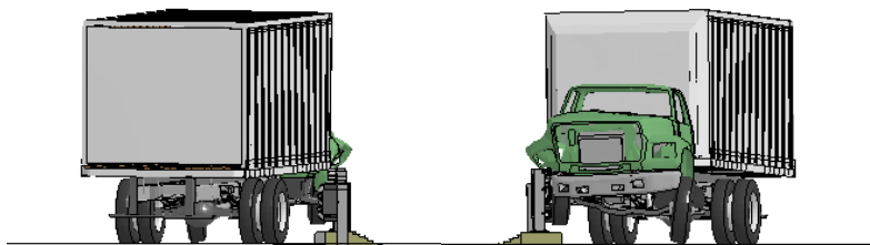
Figure P-2. Sequential views from analysis of MASH Test 4-22 for AGT 3-Bar transition from upstream and downstream viewpoints.
