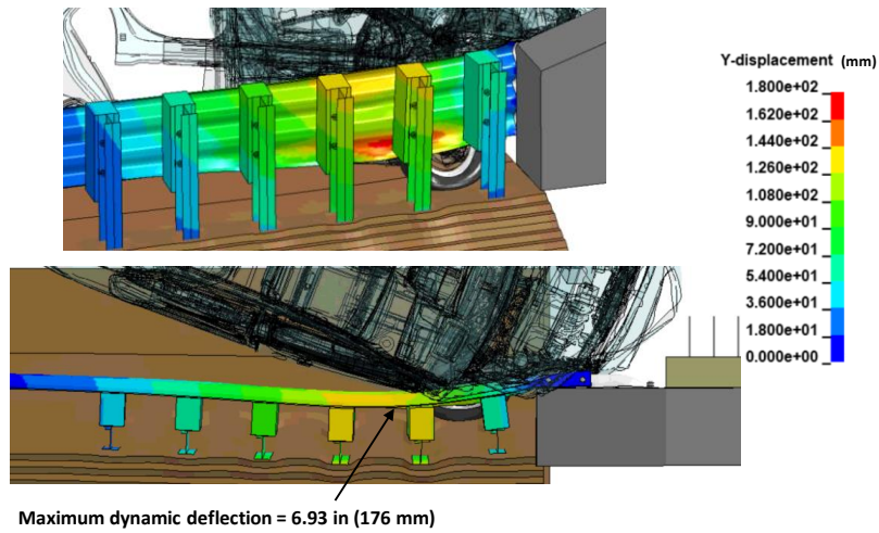
Figure 306. Contour plot of lateral displacement for the MaineDOT transition at the time of maximum dynamic deflection.
