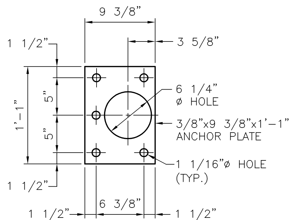
ANCHOR PLATE
