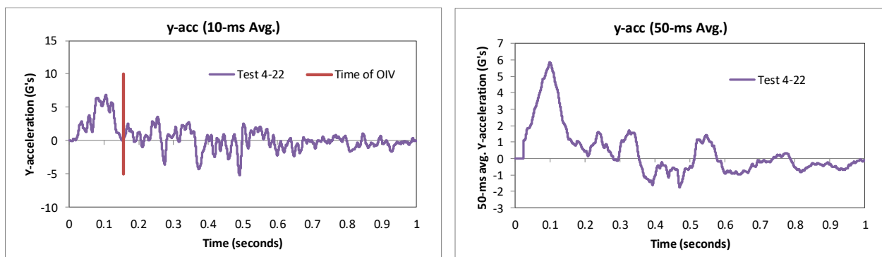
Figure 216. 10- and 50-millisecond average Y-acceleration from FEA of Test 4-22 on the 3-bar transition (cabin accelerometer).
