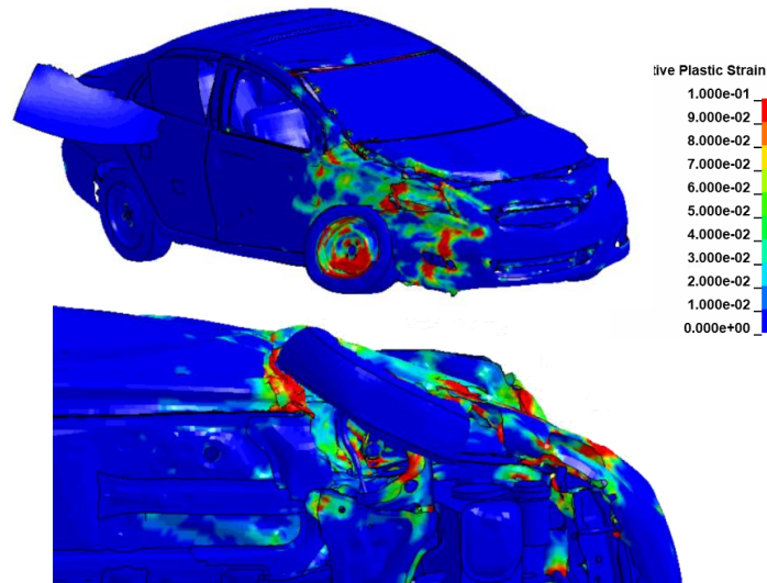
Figure 309. Damages to vehicle in Test 4-20 analysis of the MaineDOT transition.
