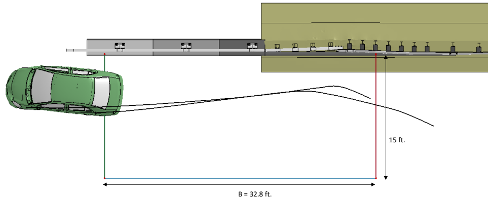
Figure 186. Exit box for Test 4-20 analysis of the 3-bar transition.
