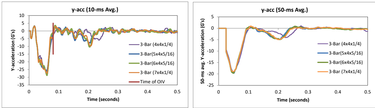
Figure 443. 10- and 50-millisecond average y-acceleration from FEA of Test 4-10 on the Modified NETC 3-bar bridge rail design cases.
