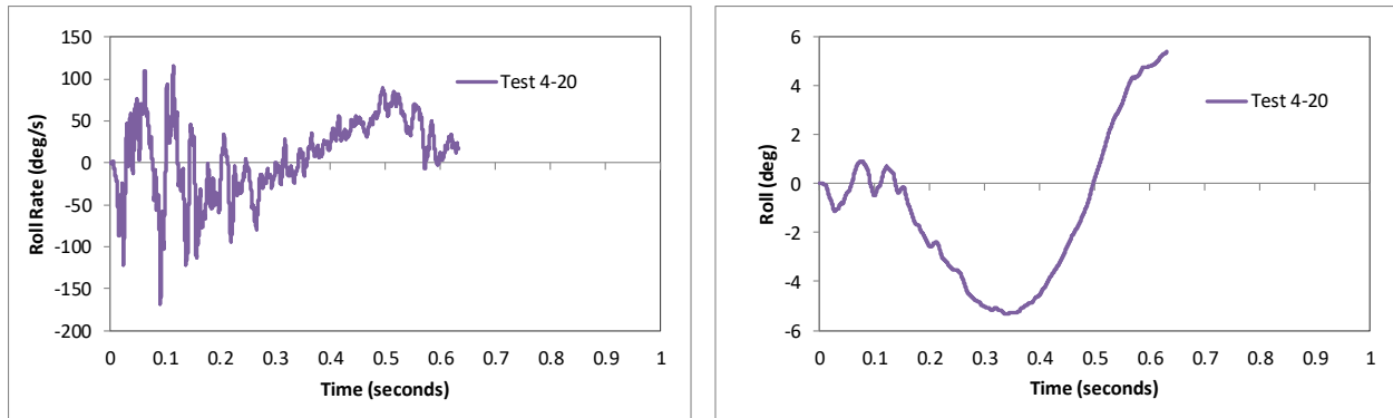
Figure 301. Roll rate and roll angle time-history from FEA of Test 4-20 on the MaineDOT transition.
