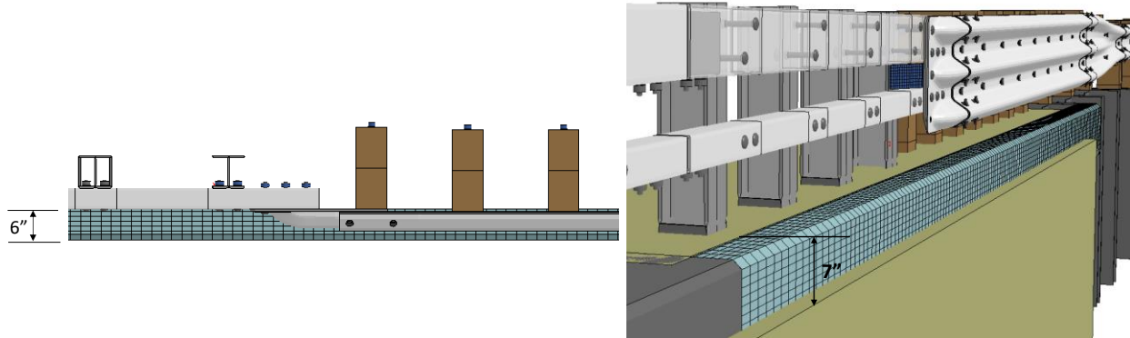
Figure 93. FEA model for curb.
