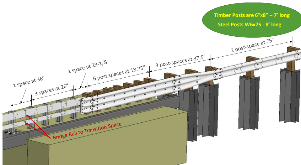
Figure 82. General model assembly for the NETC 2-bar transition (post labeling).
