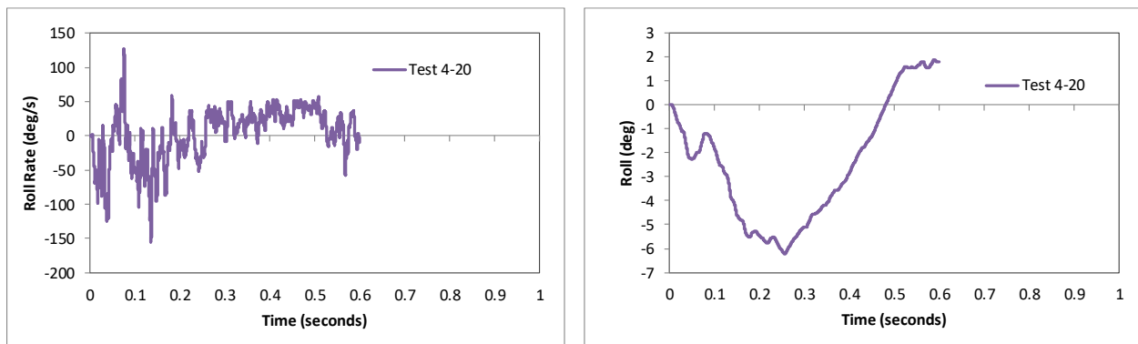
Figure 178. Roll rate and roll angle time-history from FEA of Test 4-20 on the 3-bar transition.
