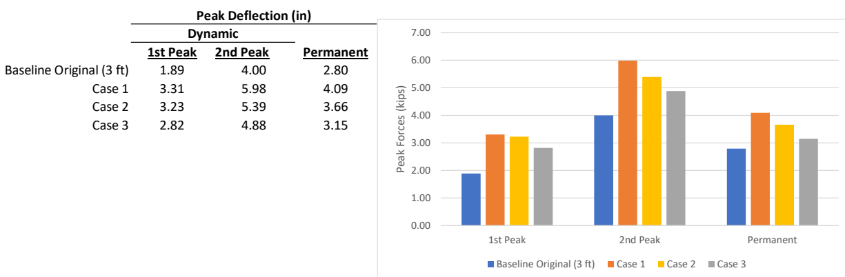
Figure 491. Peak lateral deflections of the barrier for Cases 1-3 compared with baseline case.
