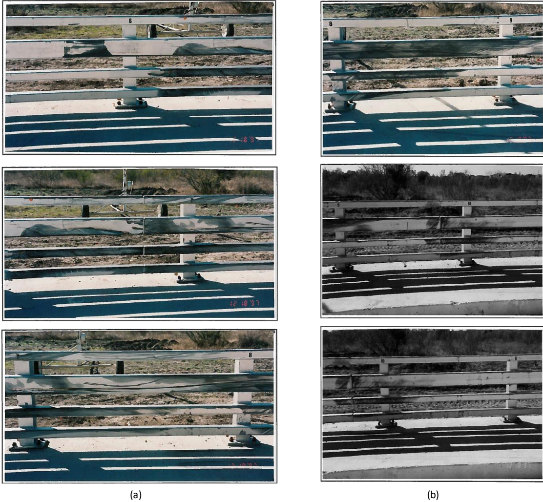
Figure 67. Damage to bridge rail in full-scale test NETC-3 from (a) posts 6 through 8 and (b) 8 through 11.
