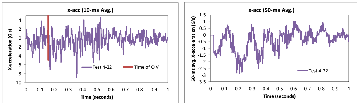
Figure 215. 10- and 50-millisecond average X-acceleration from FEA of Test 4-22 on the 3-bar transition (cabin accelerometer).
