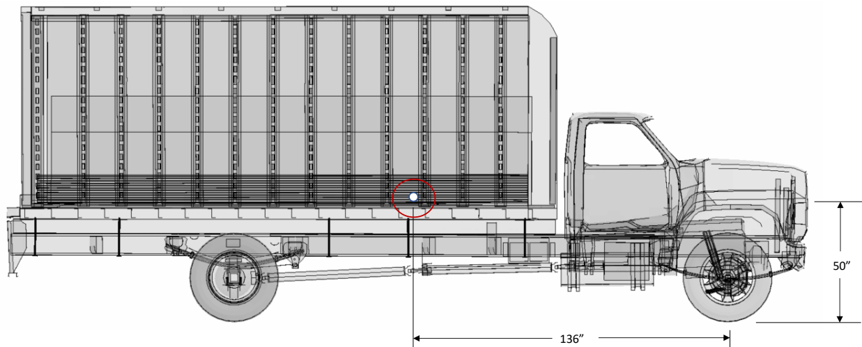
Figure 71. Location of accelerometer in FE model.
