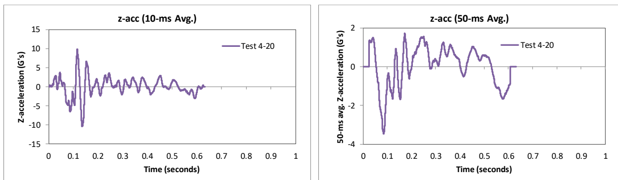
Figure 299. 10- and 50-millisecond average Z-acceleration from FEA of Test 4-20 on the MaineDOT transition.
