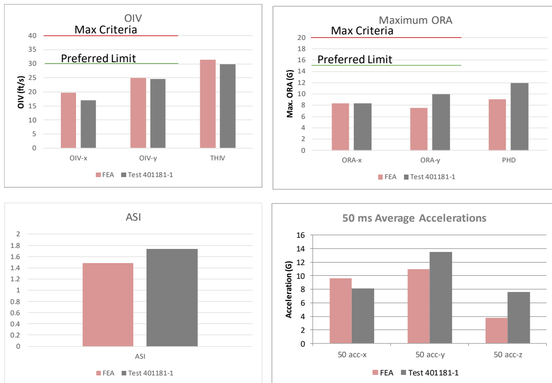
Figure 101. Graphical comparison of FEA vs. Test for key occupant risk metrics.
