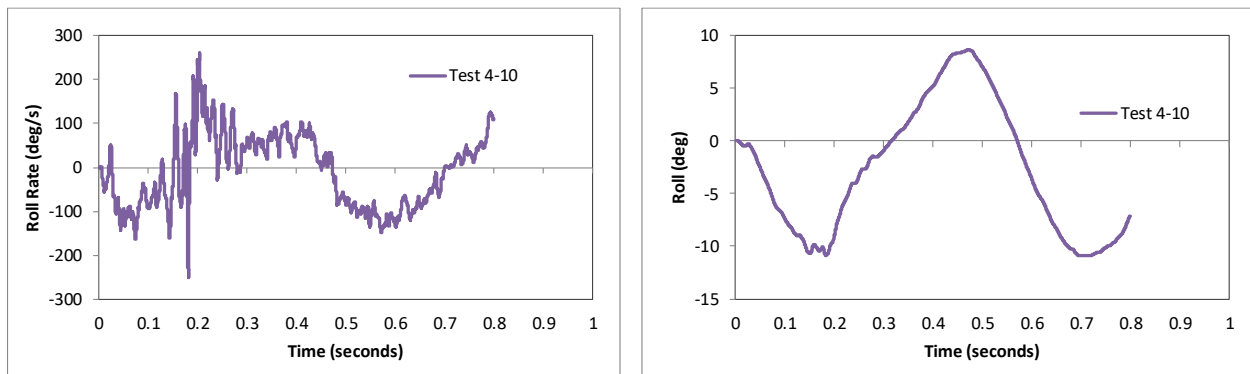
Figure 237. Roll rate and roll angle time-history from FEA of Test 4-10 on the NETC 4-bar bridge rail.
