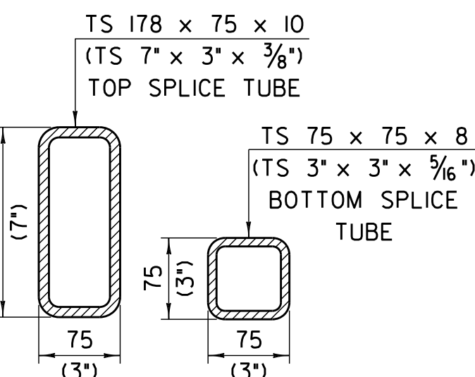
RAIL TUBE SPLICE SECTION
