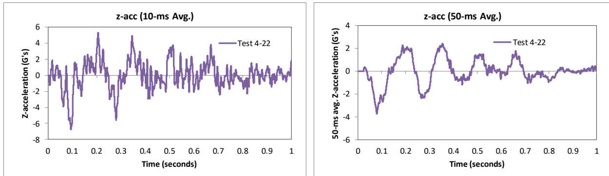
Figure 217. 10- and 50-millisecond average Z-acceleration from FEA of Test 4-22 on the 3-bar transition (cabin accelerometer).
