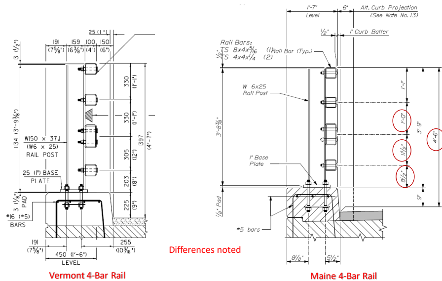
Figure 2. NETC 4-bar curb-mounted bridge rail design.
