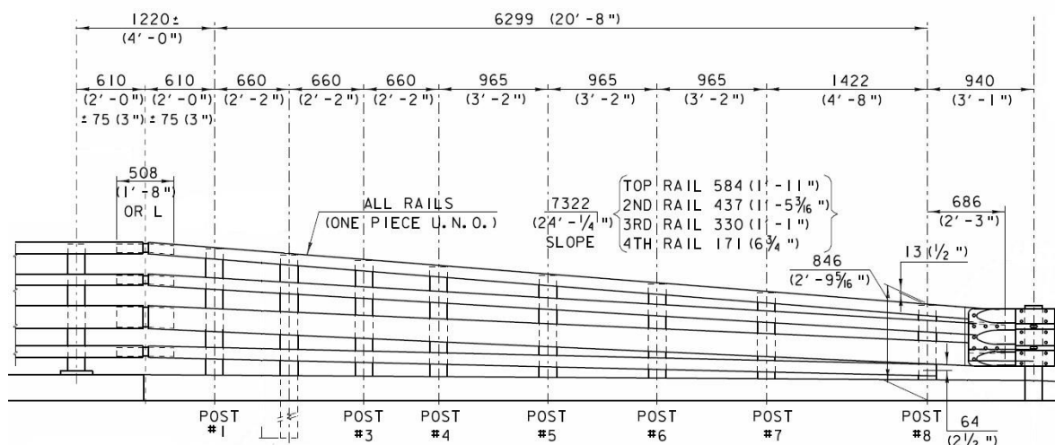
Figure 41. VTrans 4-bar AGT sloped rail section.
