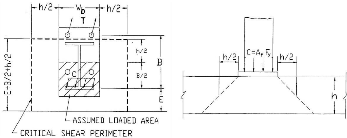
Figure 17. Punching shear failure mode (Figure A13.4.3.2-1 in 2012 LRFD)
