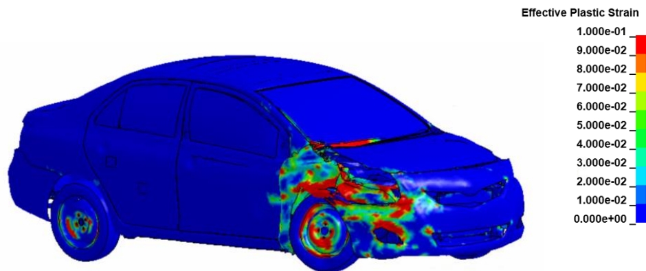
Figure 414. Damages to vehicle in Test 3-20 analysis of the 2-bar transition.
