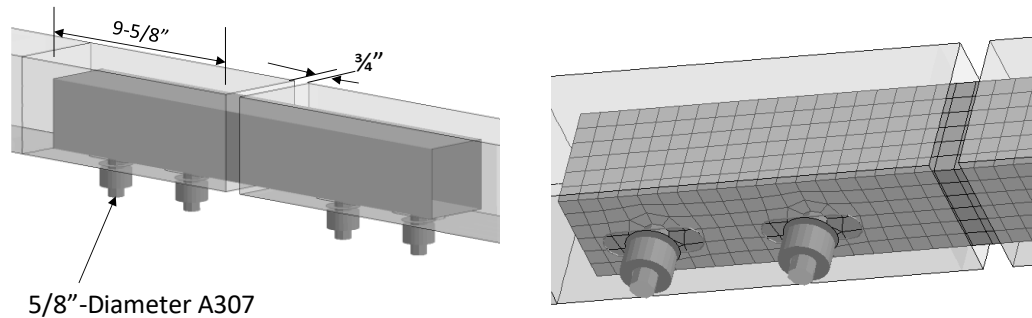
Figure 53. Model of rail splice for validation model with rail-tube shown transparent.
