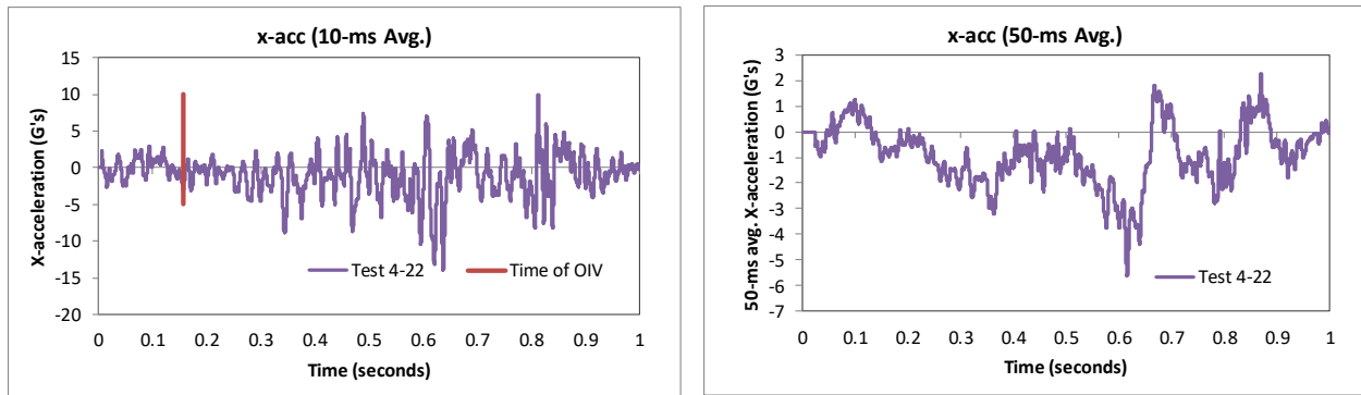
Figure 349. 10- and 50-millisecond average X-acceleration from FEA of Test 4-22 on the MaineDOT transition (cabin accelerometer).
