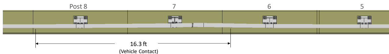
Figure 389. Overhead view of NETC 3-bar bridge rail after Test 3-11.
