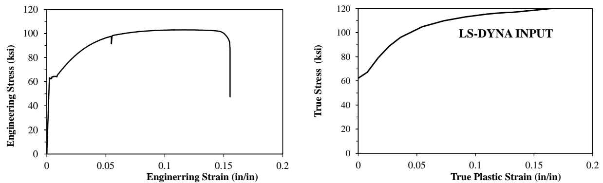
Figure 58. Stress vs. strain curve for ASTM A615 Grade 60 steel.
