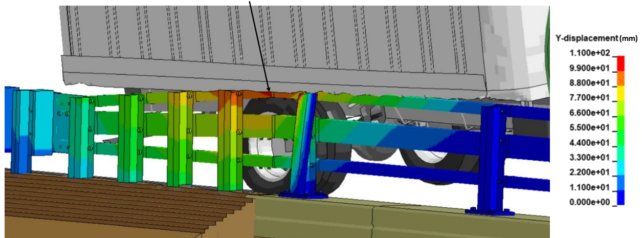
Figure 222. Contour plot of lateral displacement for the 3-bar transition for Test 4-22 at the time of maximum dynamic deflection.
