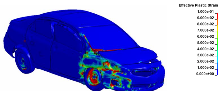
Figure 469. Damages to vehicle in Test 4-20 analysis of the 3-bar transition.
