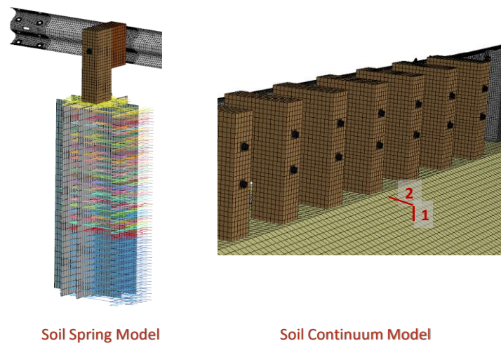
Figure 94. Soil models used in the transition model.
