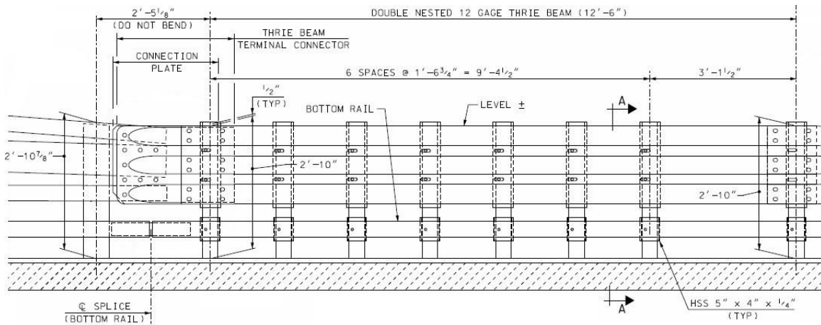
Figure 39. NHDOT T4 AGT double nested thrie-beam section.
