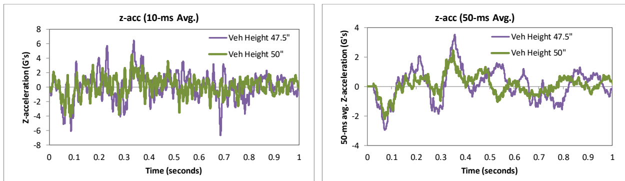
Figure 152. 10- and 50-millisecond average Z-acceleration from FEA of Test 4-12 on the NETC 3-bar bridge rail (cabin accelerometer).
