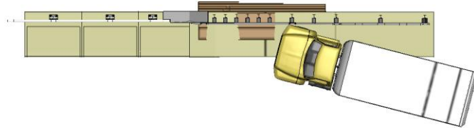
Figure V-1. Sequential views from analysis of MASH Test 4-22 for AGT 4-Bar bridge rail from an overhead viewpoint.
