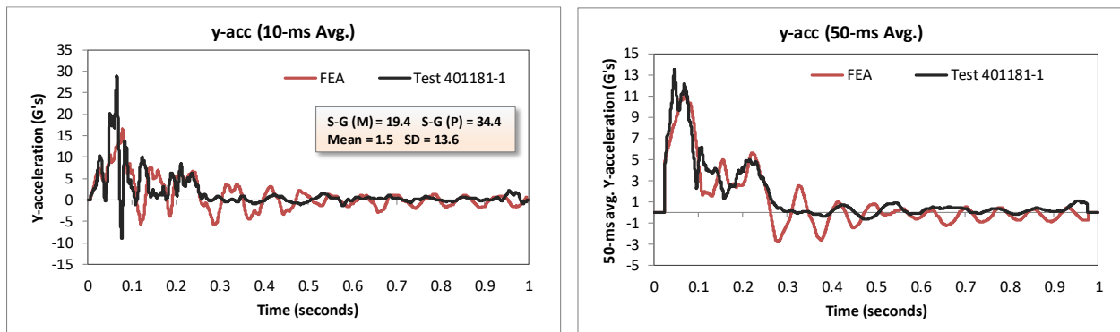
Figure 103. Lateral acceleration-time history plot from accelerometer at c.g. for full-scale Test 401181-1 and FEA (10-ms and 50-ms moving averages).
