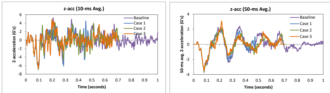
Figure 486. 10- and 50-millisecond average Z-acceleration from FEA of Test 4-22 for Case 1-3 on the 3-bar transition with 5.5-ft post spacing compared with baseline (cabin accelerometer).
