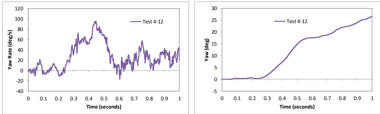
Figure 270. Yaw rate and yaw angle time-history from FEA of Test 4-12 on the NETC 4-bar bridge rail (cabin accelerometer).
