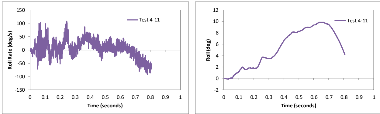
Figure 135. Roll rate and roll angle time-history from FEA of Test 4-11 on the NETC 3-bar bridge rail.
