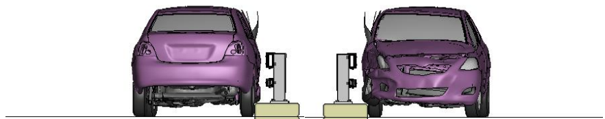
Figure W-2. Sequential views from analysis of MASH Test 3-10 for NETC 2-Bar bridge rail from upstream and downstream viewpoints.
