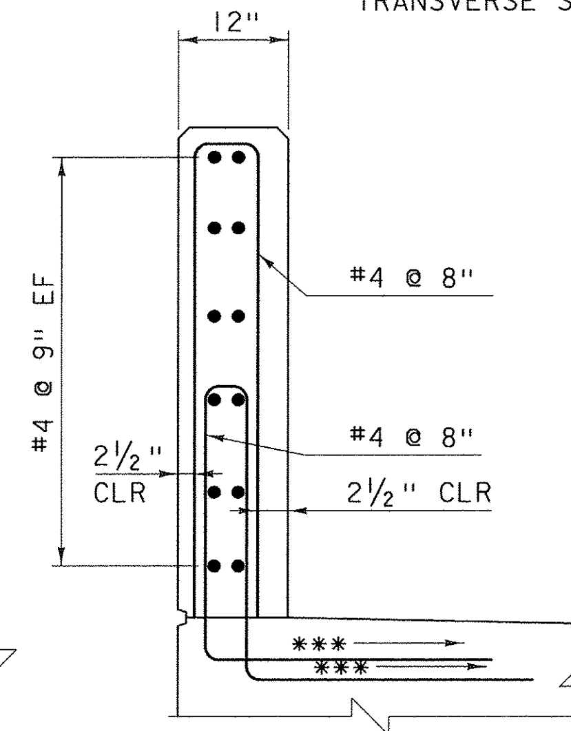
SECTION C-C
