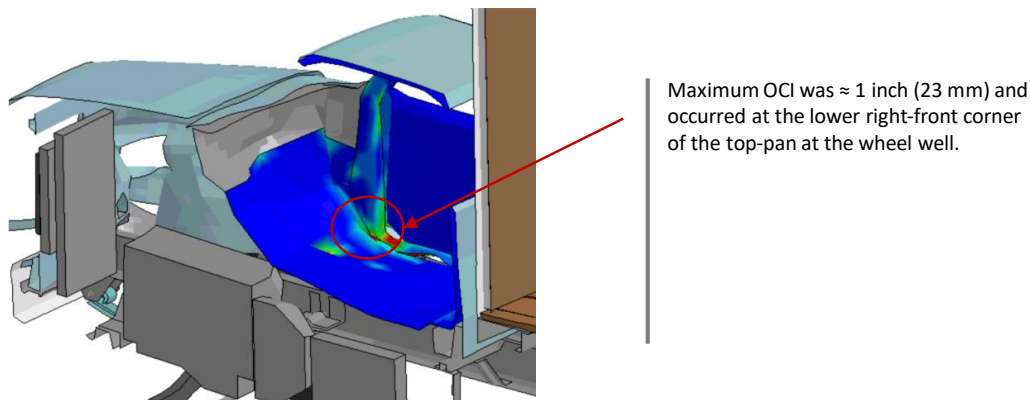
Figure 273. Occupant compartment deformation resulting from Test 4-12 on the NETC 4-bar bridge rail system.
