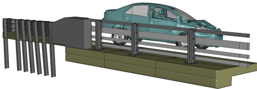
Figure T-3. [Continued] Sequential views from analysis of MASH Test 4-20 for AGT 4-Bar bridge rail from an oblique viewpoint.
