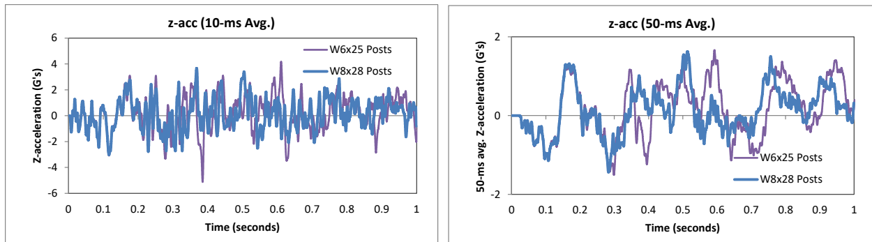
Figure 499. 10- and 50-millisecond average Z-acceleration from FEA of Test 4-12 on the baseline and modified NETC 4-bar bridge rail (cabin accelerometer).
