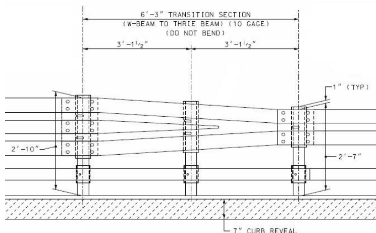
Figure 38. NHDOT T4 AGT symmetrical w-beam to thrie-beam transition section (VTrans similar except bottom bar and height).
