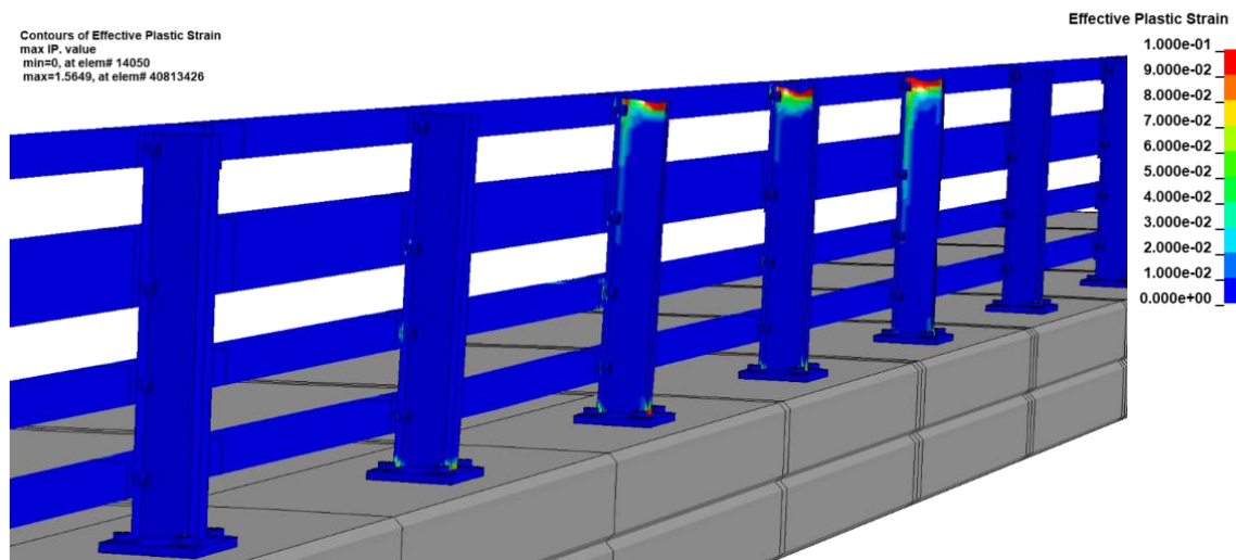
Figure 69. Contour plot of effective plastic strain showing deformations of the bridge rail model (back side).
