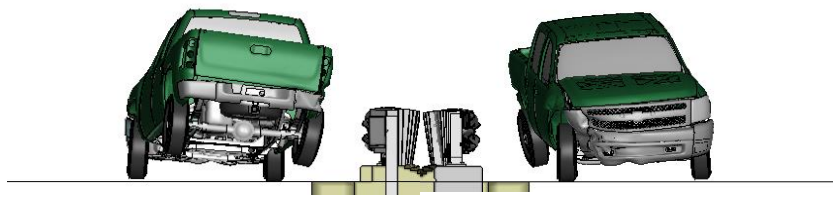
Figure Z-2. [Continued] Sequential views from analysis of MASH Test 3-21 for AGT 2-Bar bridge rail from upstream and downstream viewpoints.
