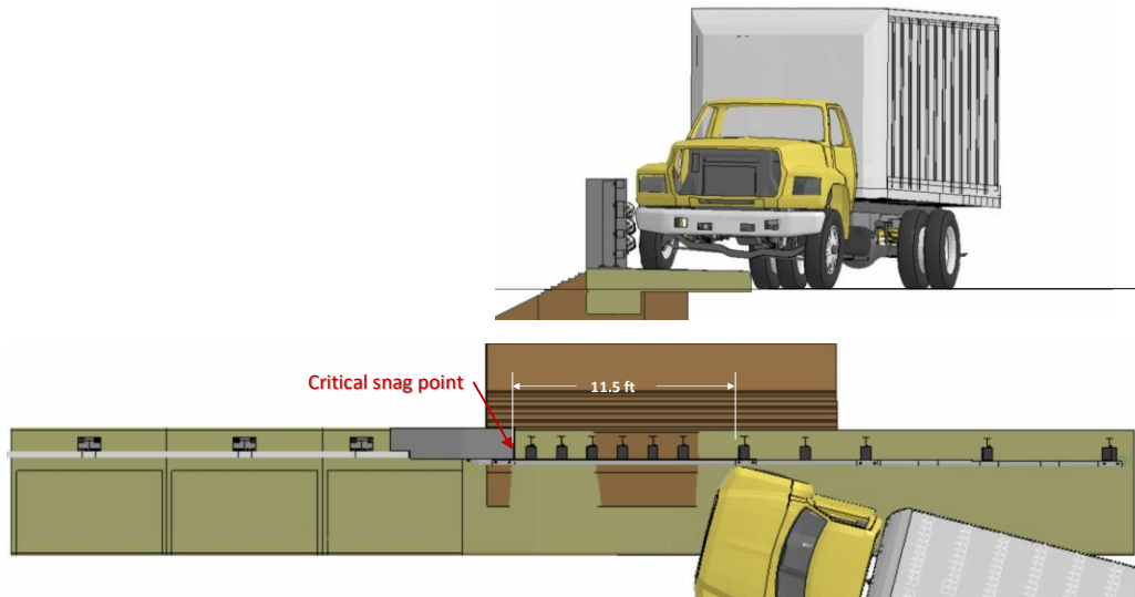
Figure 345. Impact point on the barrier for Test 4-22 on the sidewalk-mounted MaineDOT transition.
