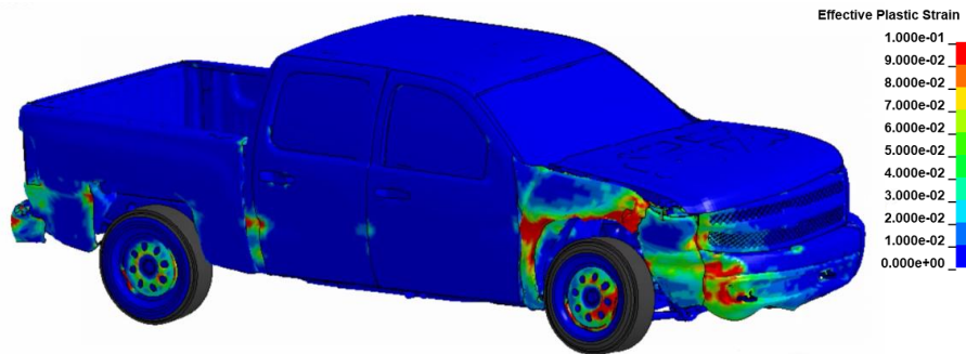
Figure 205. Damages to vehicle in Test 4-21 analysis of the 3-bar transition.
