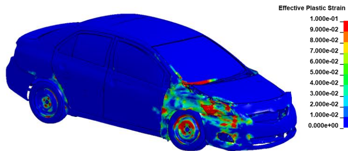
Figure 185. Damages to vehicle in Test 4-20 analysis of the 3-bar transition.
