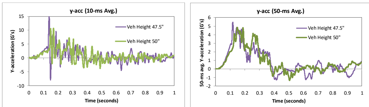
Figure 148. 10- and 50-millisecond average Y-acceleration from FEA of Test 4-12 on the NETC 3-bar bridge rail (c.g. accelerometer).
