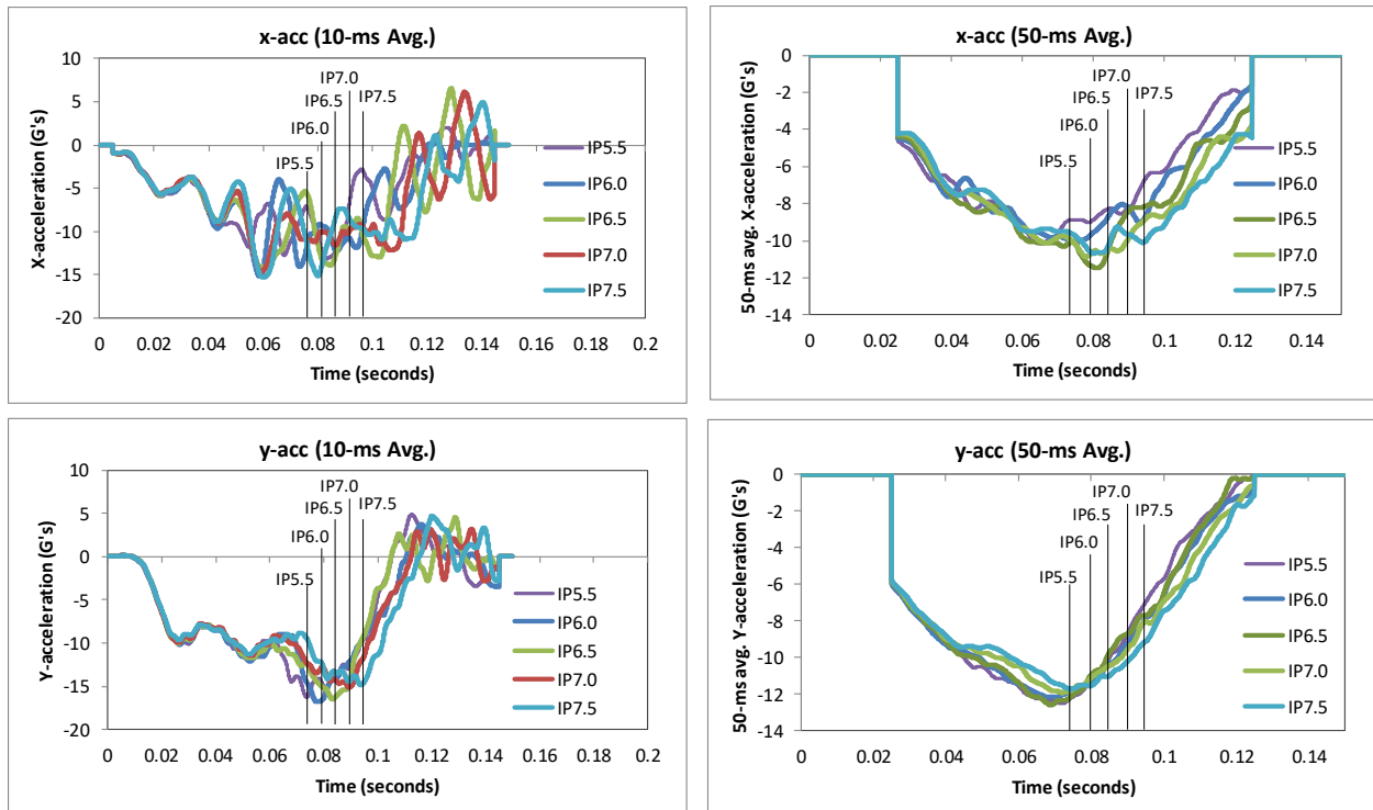
Figure 319. Plots of longitudinal and lateral accelerations indicating the time of vehicle contact with the buttress.
