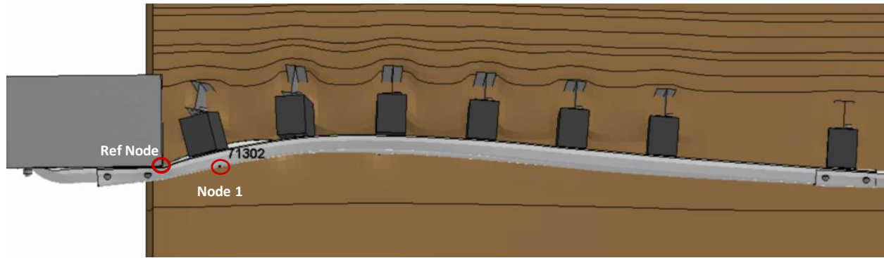
Figure 317. Measurement points for determining CIP for pocketing for Test 4-21.
