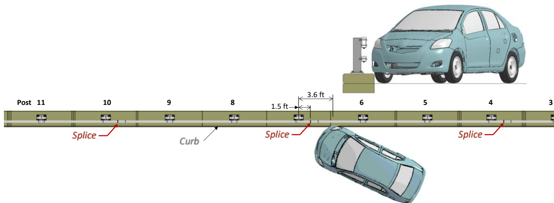
Figure 365. Impact point for Test 3-10 on the NETC 2-bar bridge rail.
