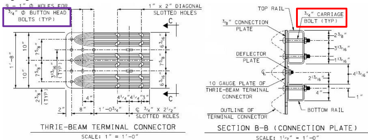
Figure 26. Terminal and connection plate detail drawings for NHDOT T2 AGT (T3 similar)
