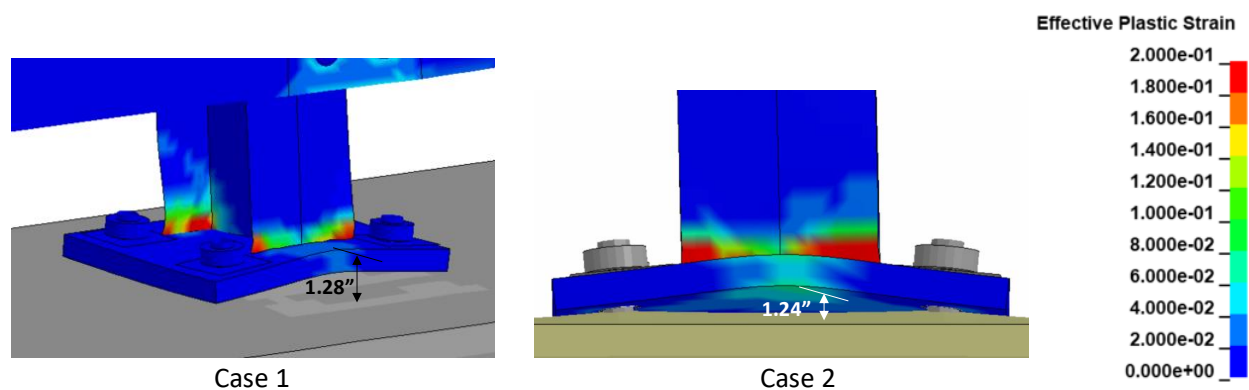
Figure 159. Contours of effective plastic strains on the critical post for Test 4-12 on the NETC 3-bar bridge rail.
