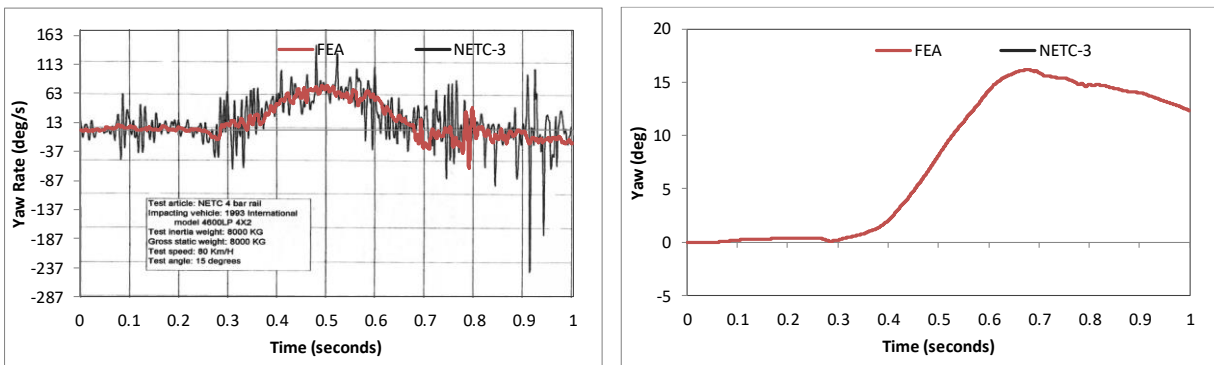
Figure 76. Yaw-time history plot from accelerometer at c.g. for FEA (angular rate and displacement).
