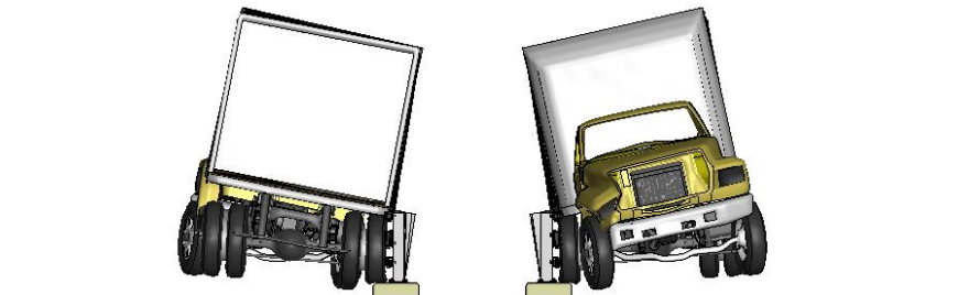
Figure K-2. [Continued] Sequential views from analysis of MASH Test 4-12 for NETC 3-Bar bridge rail from upstream and downstream viewpoints – Case 1.
