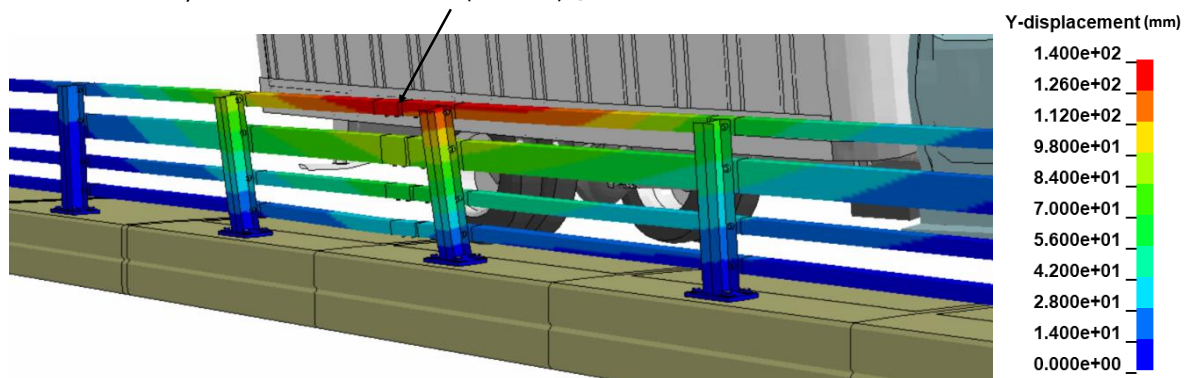
Figure 275. Contour plot of lateral displacement for the bridge rail from Test 4-12 at the time of maximum dynamic deflection for the NETC 4-bar bridge rail.
