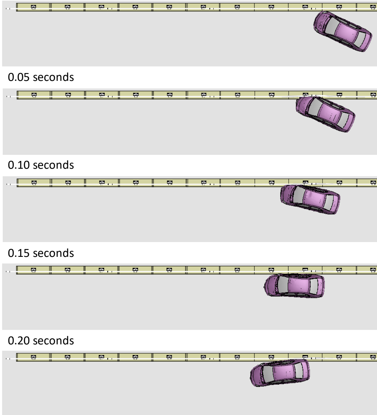
Figure W-1. Sequential views from analysis of MASH Test 3-10 for NETC 2-Bar bridge rail from an overhead viewpoint.
