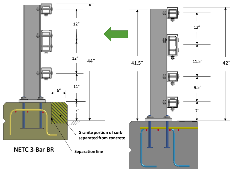
Figure 113. FEA model of curb-mounted NETC 3-bar compared with Baseline sidewalk-mounted 4-bar model.
