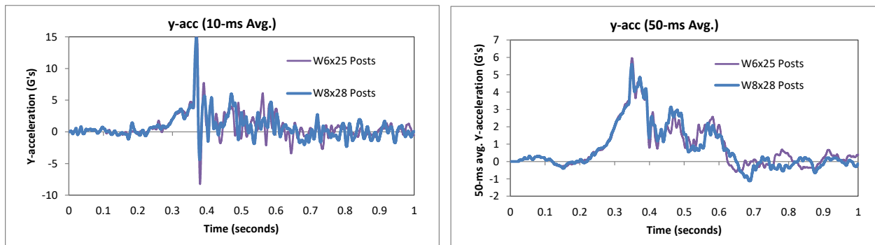
Figure 501. 10- and 50-millisecond average Y-acceleration from FEA of Test 4-12 on the baseline and modified NETC 4-bar bridge rail (c.g. accelerometer).
