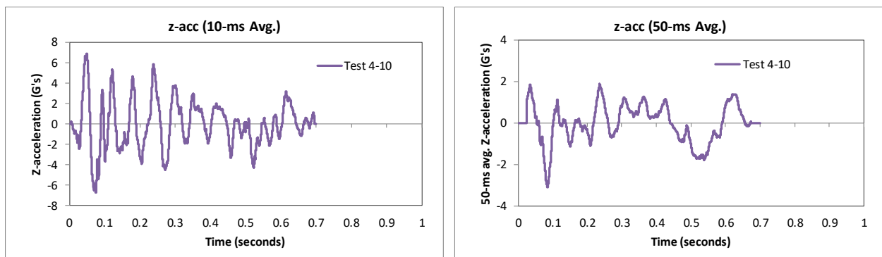
Figure 117. 10- and 50-millisecond average Z-acceleration from FEA of Test 4-10 on the NETC 3-bar bridge rail.
