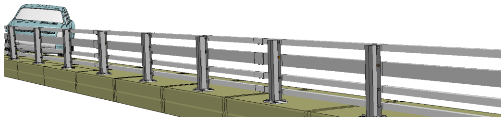
Figure R-3. Sequential views from analysis of MASH Test 4-11 for NETC 4-Bar bridge rail from an oblique viewpoint.
