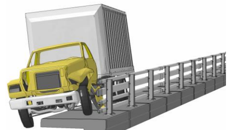
Figure 2. [CONTINUED] Sequential views of Test NETC-3 and FE analysis from downstream viewpoint.
