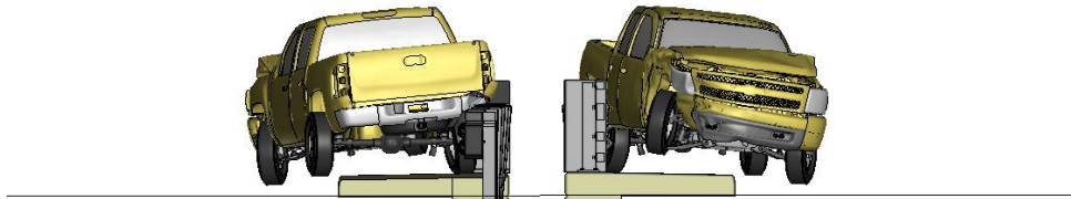
Figure U-2. [Continued] Sequential views from analysis of MASH Test 4-21 for AGT 4-Bar bridge rail from upstream and downstream viewpoints.
