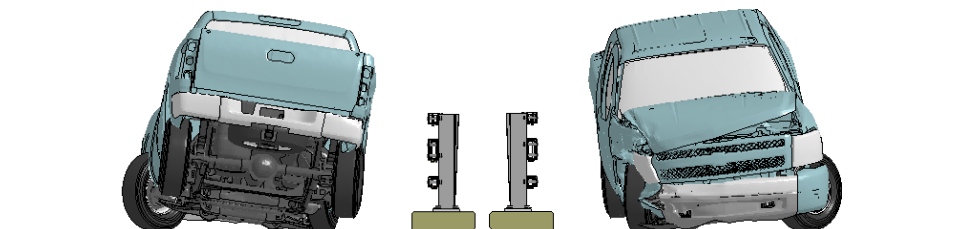
Figure K-2. [Continued] Sequential views from analysis of MASH Test 4-11 for NETC 3-Bar bridge rail from upstream and downstream viewpoints.
