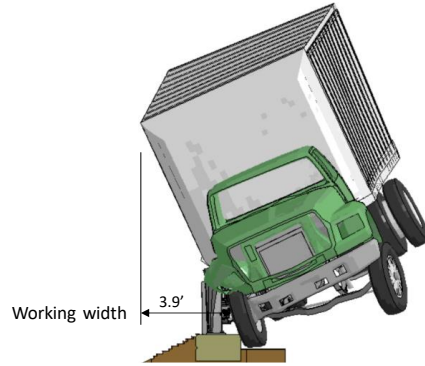
Figure 225. Working width for Test 4-22 on 3-bar transition.
