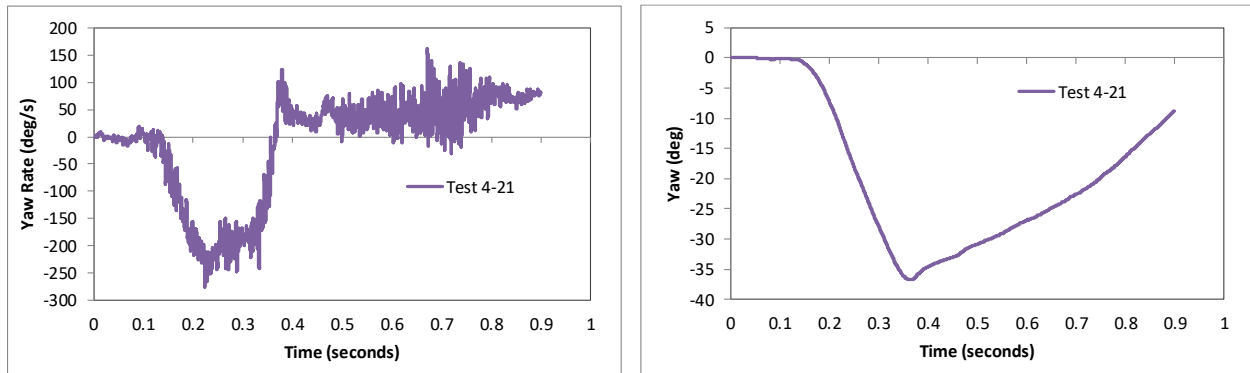
Figure 328. Yaw rate and roll angle time-history from FEA of Test 4-21 on the MaineDOT transition.
