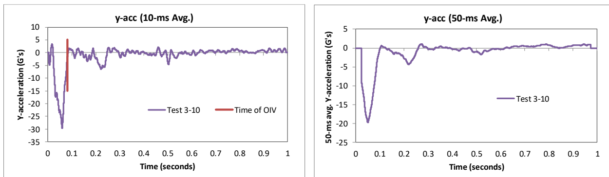
Figure 367. 10- and 50-millisecond average Y-acceleration from FEA of Test 3-10 on the NETC 2-bar bridge rail.
