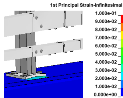
Figure 142. Contours of 1 st principal strains for concrete at the critical post for Test 4-11 on the NETC 3-bar bridge rail.
