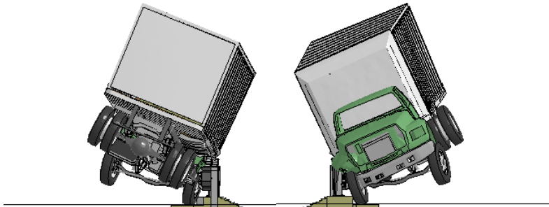
Figure P-2. [Continued] Sequential views from analysis of MASH Test 4-22 for AGT 3-Bar transition from upstream and downstream viewpoints.
