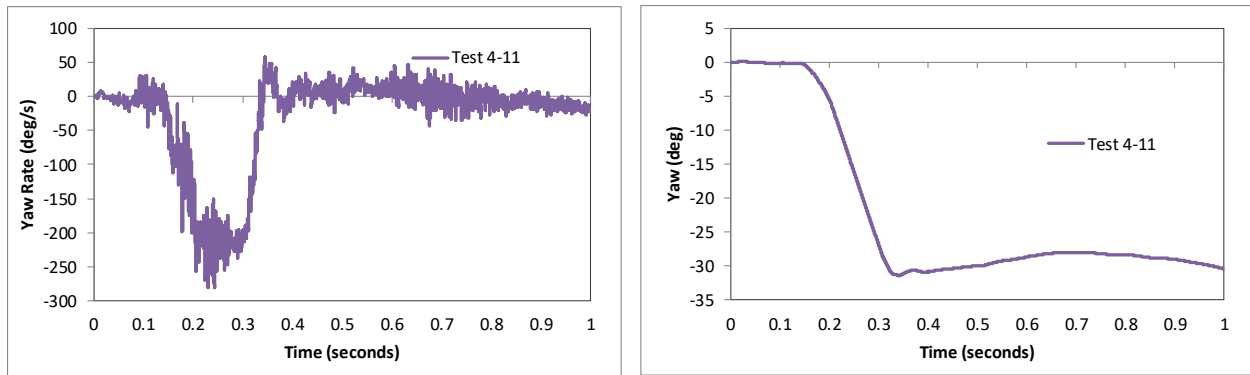
Figure 252. Yaw rate and yaw angle time-history from FEA of Test 4-11 on the NETC 4-bar bridge rail.
