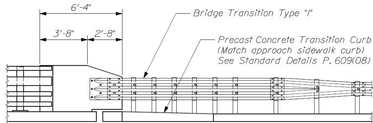
(c) Maine Concrete to Thrie Beam (TL3)
