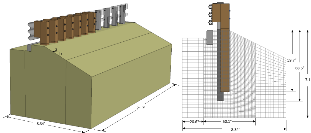
Figure 95. Continuum soil model mesh and dimensions.
