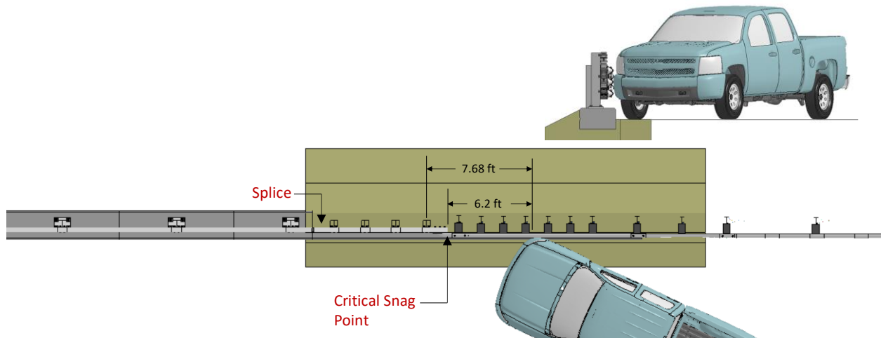
Figure 193. Impact point for Test 4-21 on the 3-bar transition.
