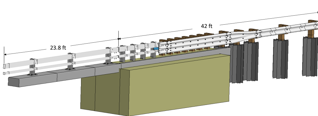
Figure 80. Finite element analysis model of the NETC 2-bar transition and bridge rail.
