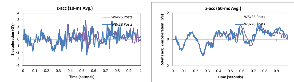
Figure 502. 10- and 50-millisecond average Z-acceleration from FEA of Test 4-12 on the baseline and modified NETC 4-bar bridge rail (c.g. accelerometer).
