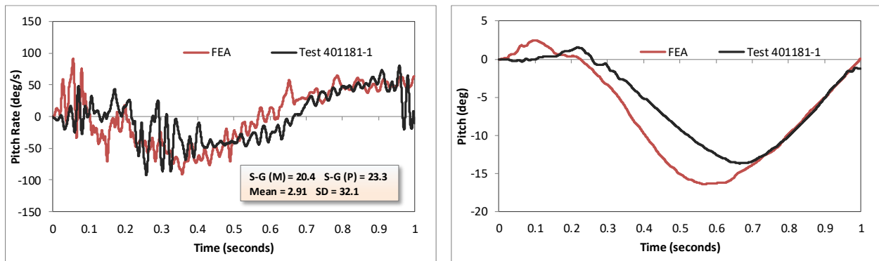
Figure 107. Pitch-time history plot from accelerometer inside cabin for full-scale test 401181-1 and FEA (angular rate and displacement).
