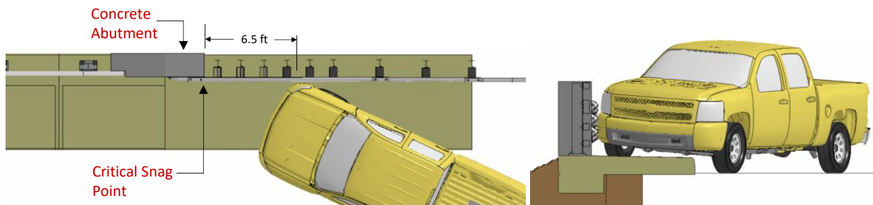
Figure 324. Actual impact point for Test 4-21 on the MaineDOT transition for 4-bar bridge rail.
