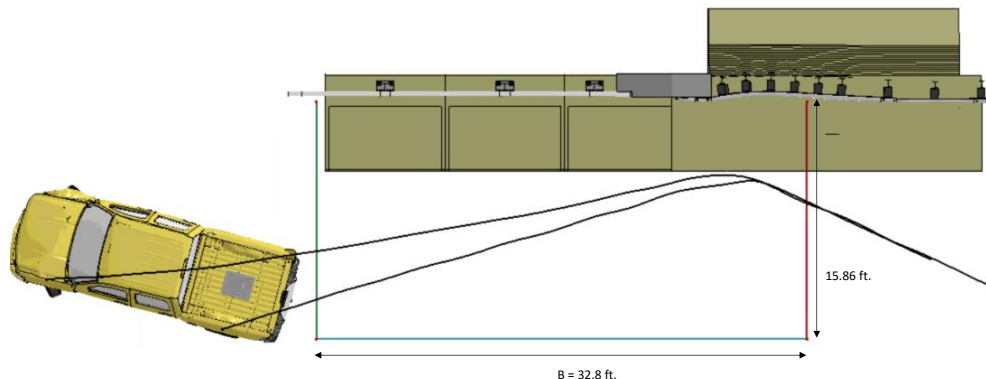
Figure 338. Exit box for Test 4-21 analysis of the MaineDOT transition.
