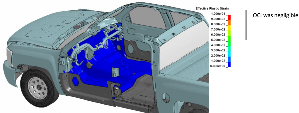
Figure 200. Occupant compartment deformation resulting from Test 4-21 on the 3-bar transition.
