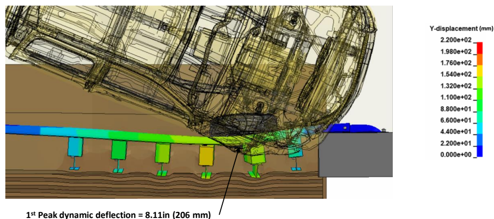
Figure 333. Contour plot of lateral displacement for Test 4-21 on the MaineDOT transition at the 1 st peak deflection.
