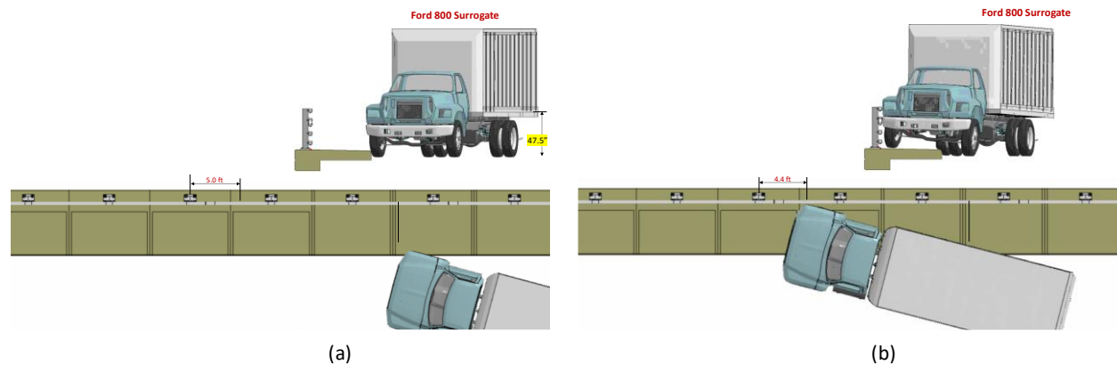
Figure 263. (a) Target and (b) actual impact point for Test 4-12 on the NETC 4-bar bridge rail.
