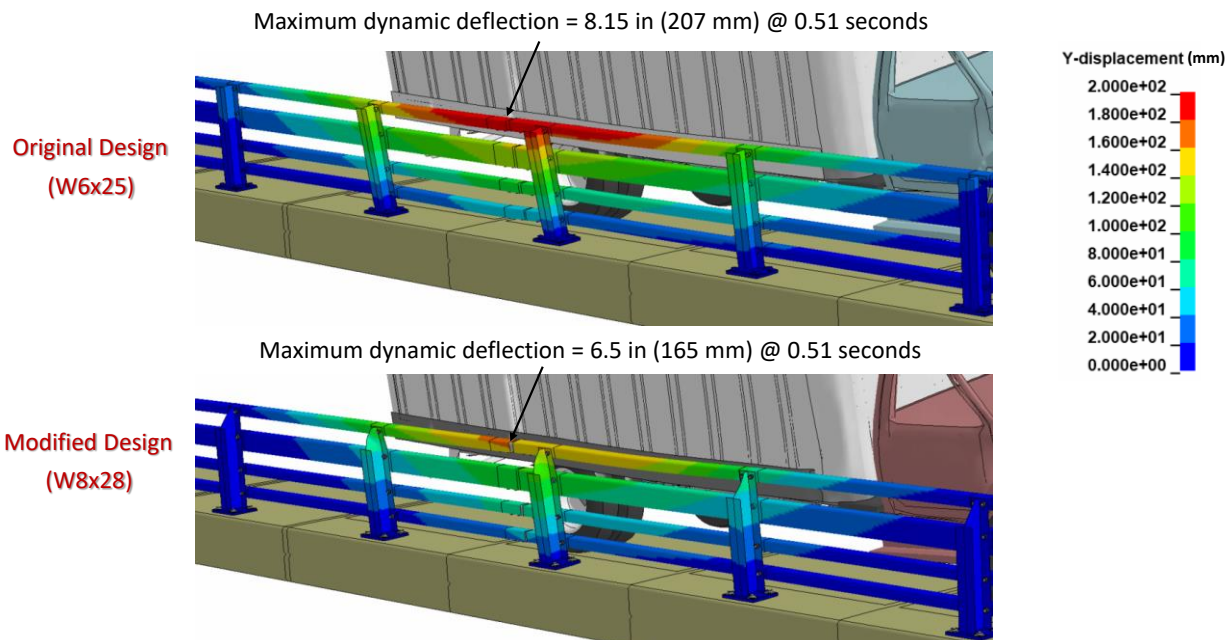
Figure 507. Contour plot of lateral displacement for the bridge rail from Test 4-12 at the time of maximum deflection for the original and modified design cases.
