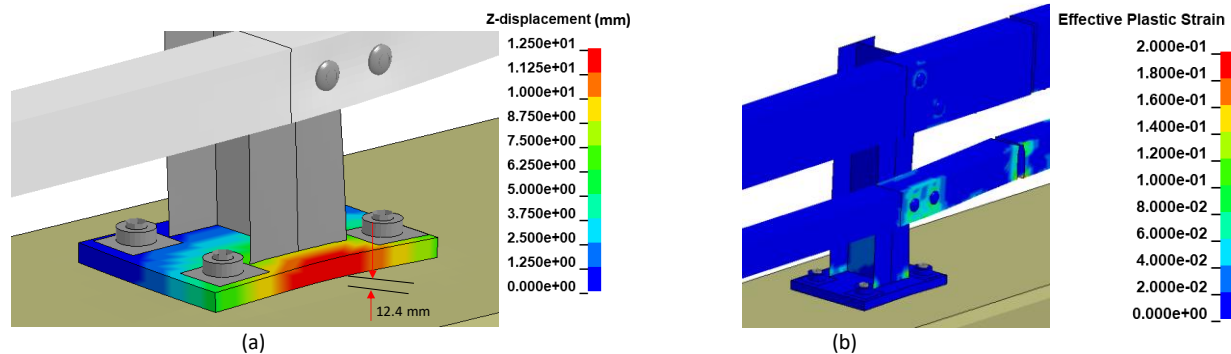
Figure 376. Contours of (a) vertical displacement on baseplate and (b) effective plastic strains on barrier for Test 3-10 on the NETC 2-bar bridge rail.
