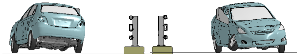
Figure J-2. [Continued] Sequential views from analysis of MASH Test 4-10 for NETC 3-Bar bridge rail from upstream and downstream viewpoints.
