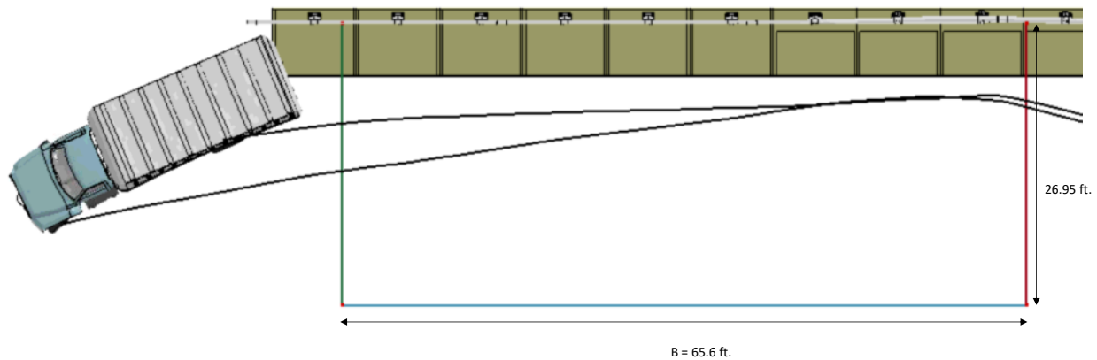
Figure 281. Exit box for Test 4-12 for Case 1 on the NETC 4-bar bridge rail.
