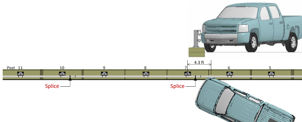
Figure 381. Impact point for Test 3-11 on the NETC 2-bar bridge rail.
