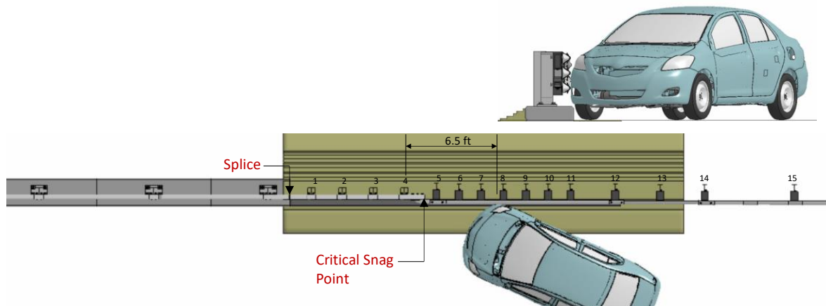
Figure 402. Impact point for Test 3-20 on the 2-bar transition.
