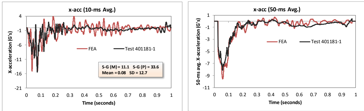
Figure 102. Longitudinal acceleration-time history plot from accelerometer at c.g. for full-scale Test 401181-1 and FEA (10-ms and 50-ms moving averages).
