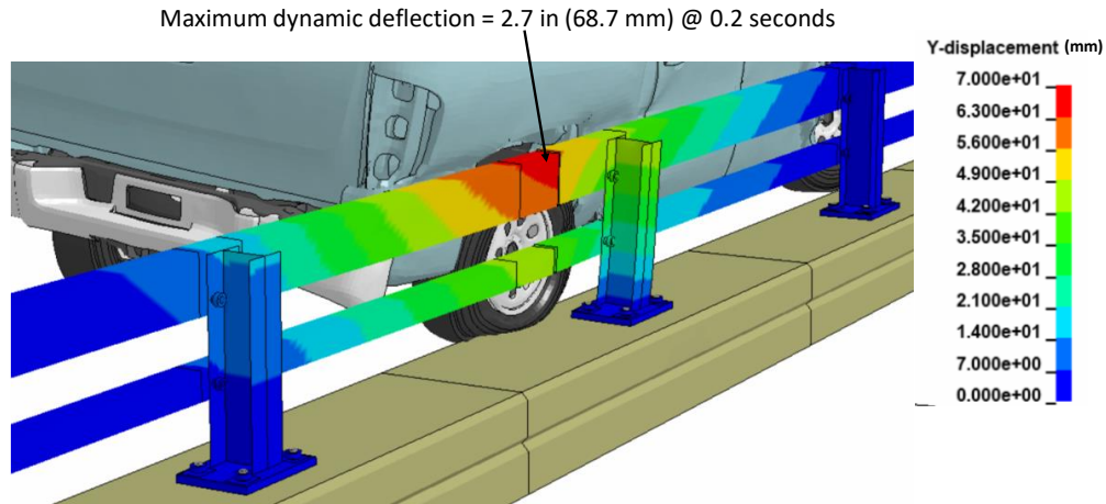
Figure 390. Contour plot of lateral displacement for the bridge rail for Test 3-11 on NETC 2-bar bridge rail at the time of maximum dynamic deflection.
