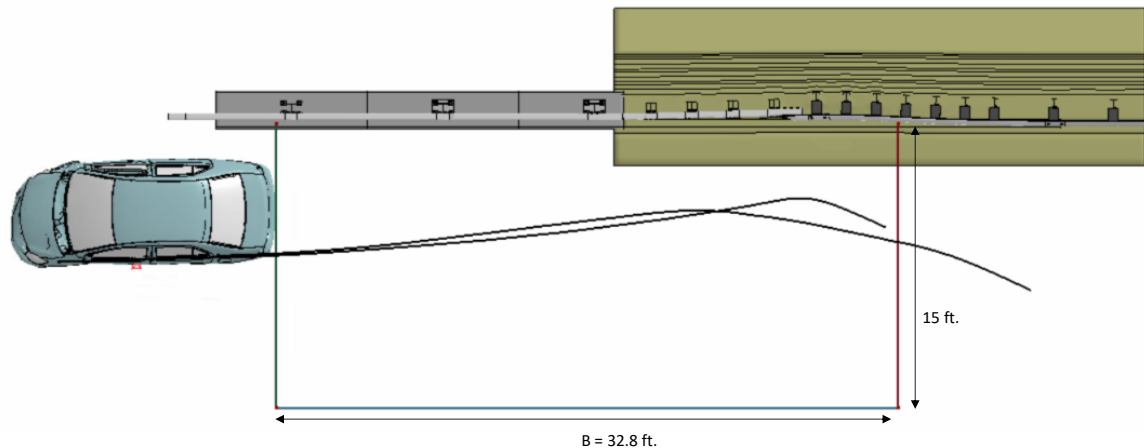
Figure 415. Exit box for Test 3-20 analysis of the 2-bar transition.
