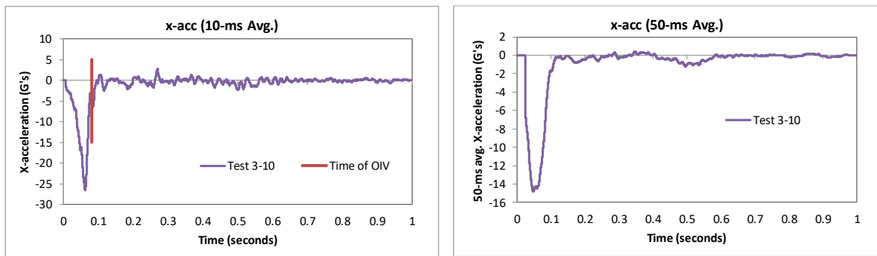
Figure 366. 10- and 50-millisecond average X-acceleration from FEA of Test 3-10 on the NETC 2-bar bridge rail.
