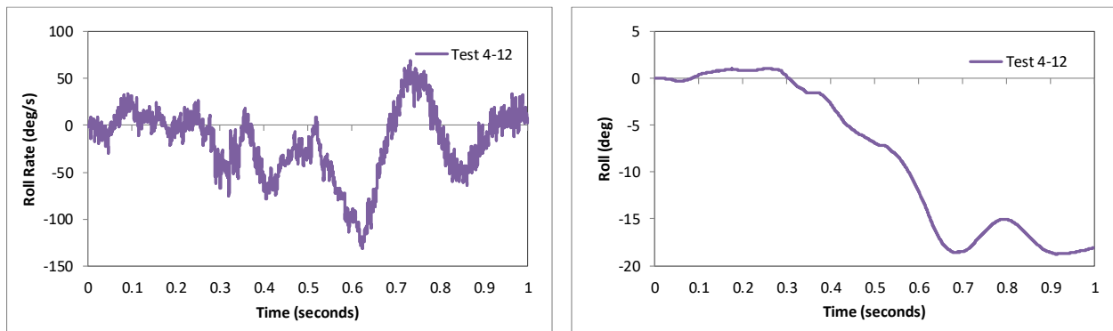
Figure 271. Roll rate and roll angle time-history from FEA of Test 4-12 on the NETC 4-bar bridge rail (cabin accelerometer).
