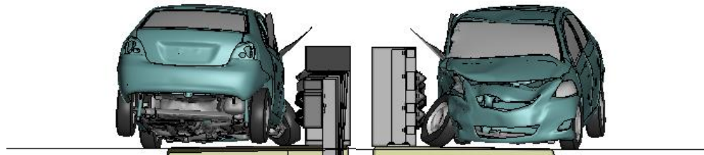
Figure T-2. Sequential views from analysis of MASH Test 4-20 for AGT 4-Bar bridge rail from upstream and downstream viewpoints.
