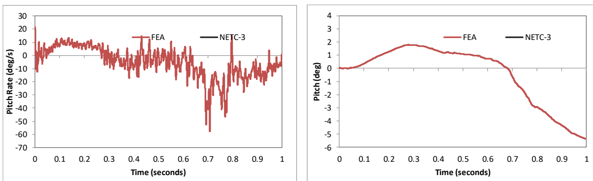
Figure 78. Pitch-time history plot from accelerometer at c.g. for FEA (angular rate and displacement).
