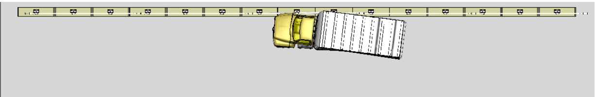
Figure L-1. Sequential views from analysis of MASH Test 4-12 for NETC 3-Bar bridge rail from an overhead viewpoint – Case 1.
