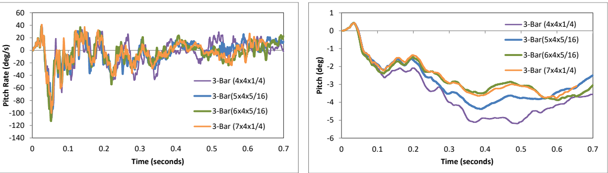
Figure 447. Pitch rate and pitch angle time-history from FEA of Test 4-10 on the Modified NETC 3-bar bridge rail design cases.
