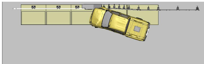
Figure U-1. Sequential views from analysis of MASH Test 4-21 for AGT 4-Bar bridge rail from an overhead viewpoint.
