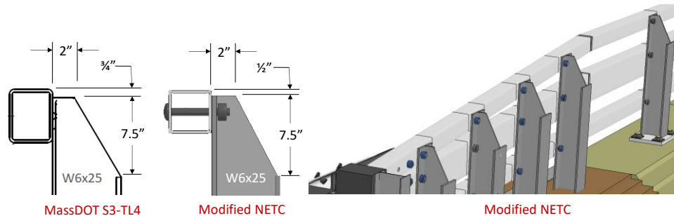
Figure 452. Tapered post based on MassDOT S3-TL4 bridge rail design.
