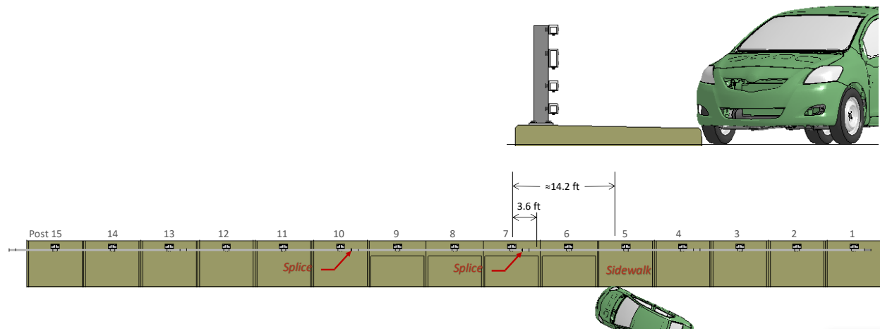
Figure 231. Initial starting point and target impact point for Test 4-10 on the NETC 4-bar bridge rail.
