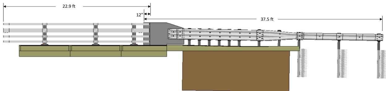
Figure 287. Complete FEA model of the MaineDOT transition and bridge rail.
