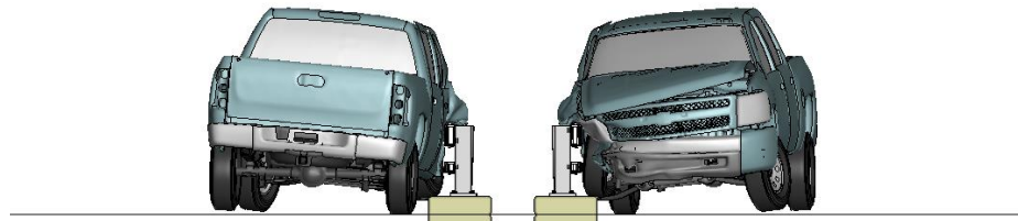
Figure X-2. Sequential views from analysis of MASH Test 3-11 for NETC 2-Bar bridge rail from upstream and downstream viewpoints.
