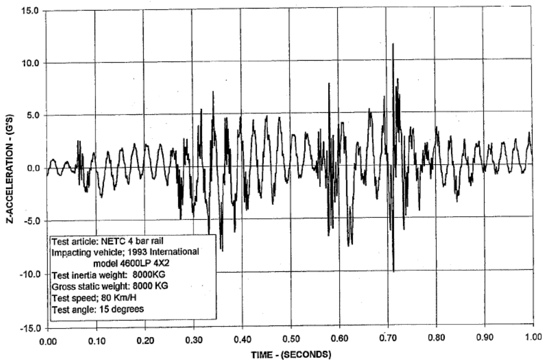
Figure 61. Vertical (z-direction) acceleration measured at vehicle c.g. in Test NETC-3. [Kimball99]
