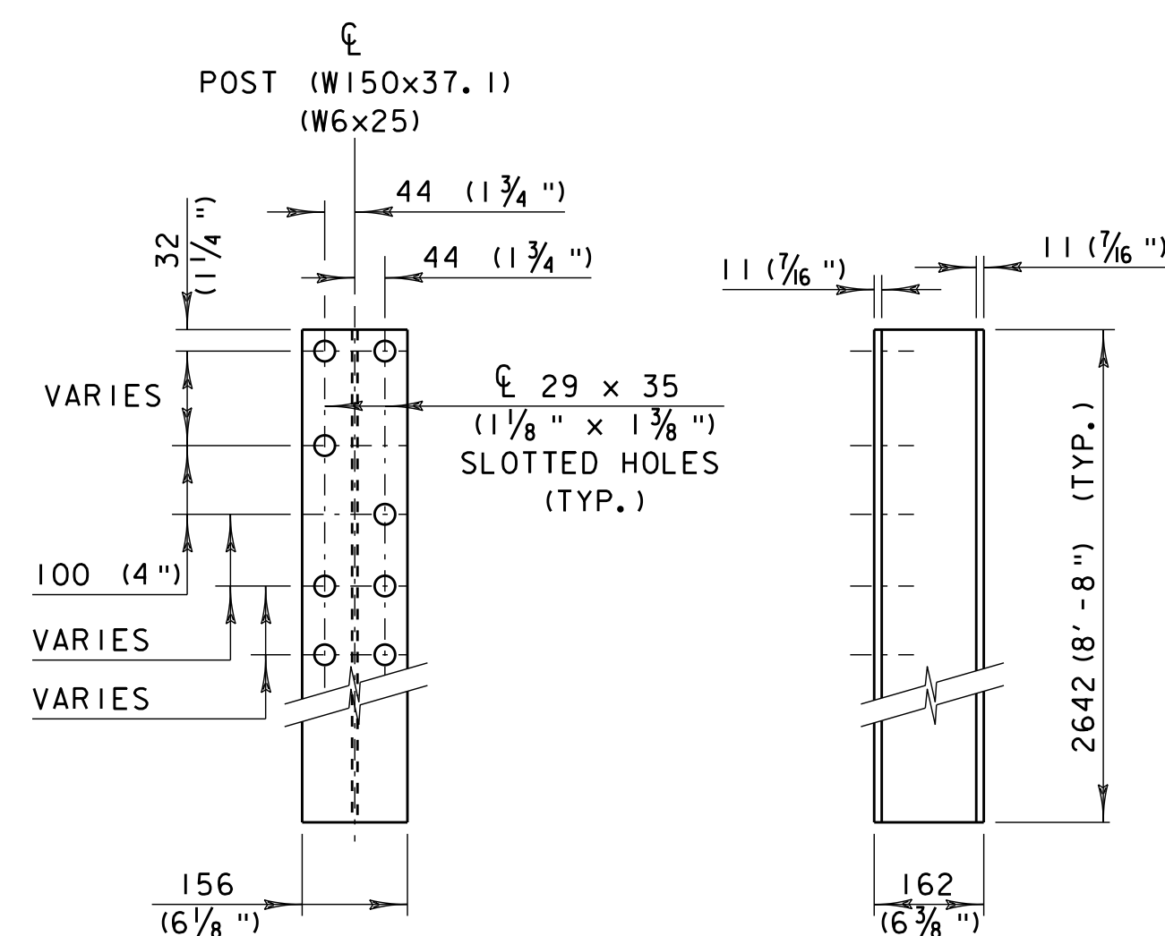
RAIL POST
