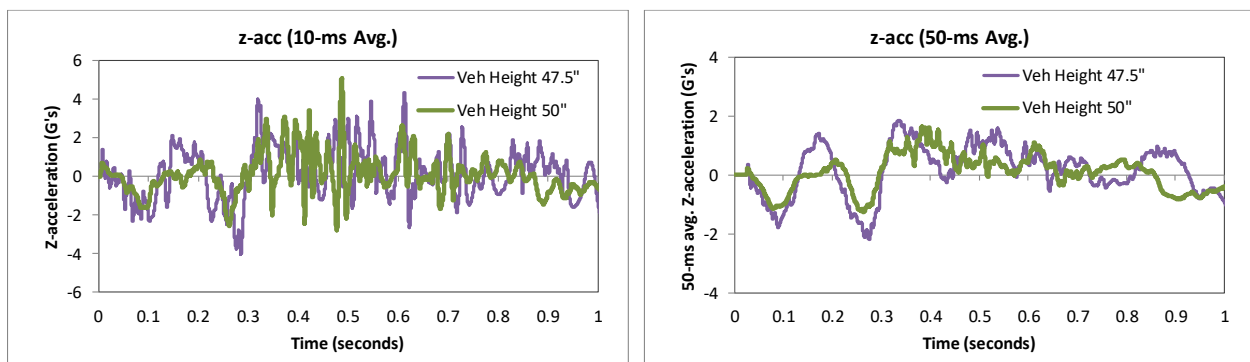
Figure 149. 10- and 50-millisecond average Z-acceleration from FEA of Test 4-12 on the NETC 3-bar bridge rail (c.g. accelerometer).
