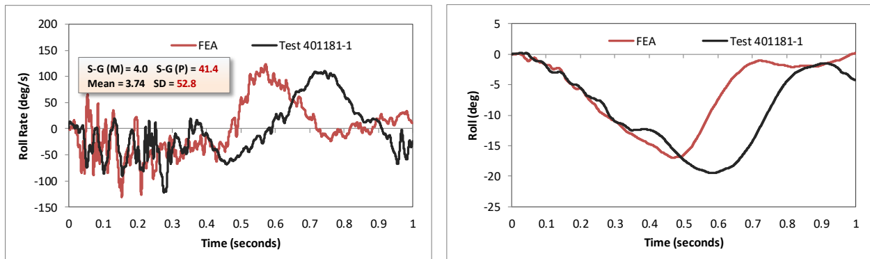
Figure 106. Roll-time history plot from accelerometer inside cabin for full-scale test 401181-1 and FEA (angular rate and displacement).
