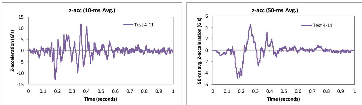
Figure 251. 10- and 50-millisecond average Z-acceleration from FEA of Test 4-11 on the NETC 4-bar bridge rail.
