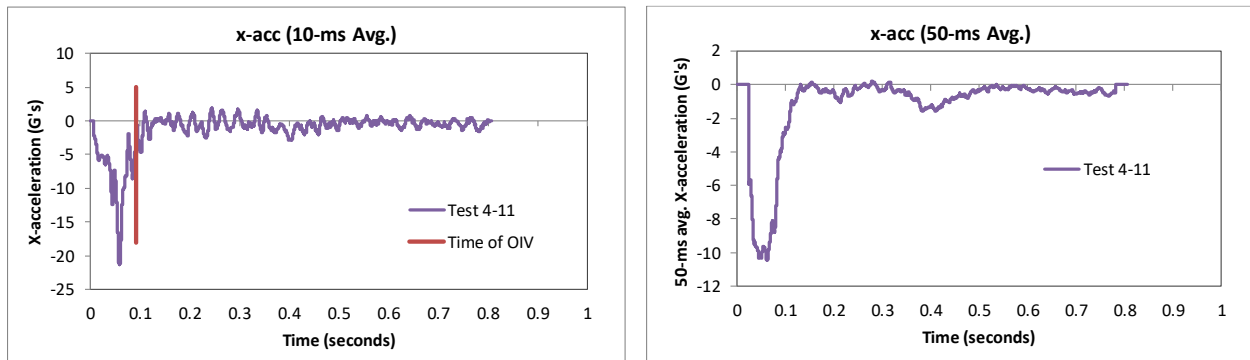
Figure 131. 10- and 50-millisecond average X-acceleration from FEA of Test 4-11 on the NETC 3-bar bridge rail.
