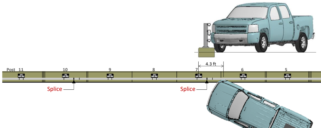
Figure 130. Impact point for Test 4-11 on the NETC 3-bar bridge rail.
