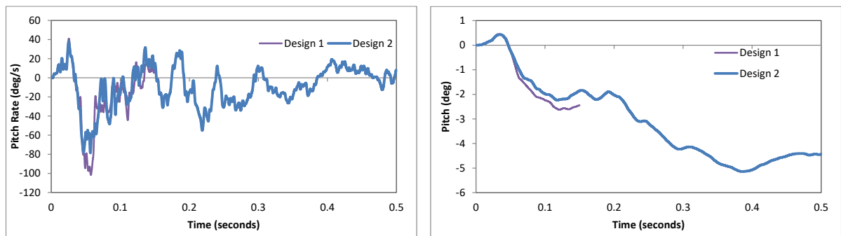
Figure 466. Pitch rate and pitch angle time-history from FEA of Test 4-20 on the 3-bar transition with 5.5-ft post spacing.
