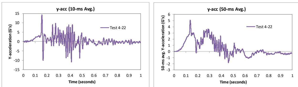
Figure 213. 10- and 50-millisecond average Y-acceleration from FEA of Test 4-22 on the 3-bar transition (c.g. accelerometer).
