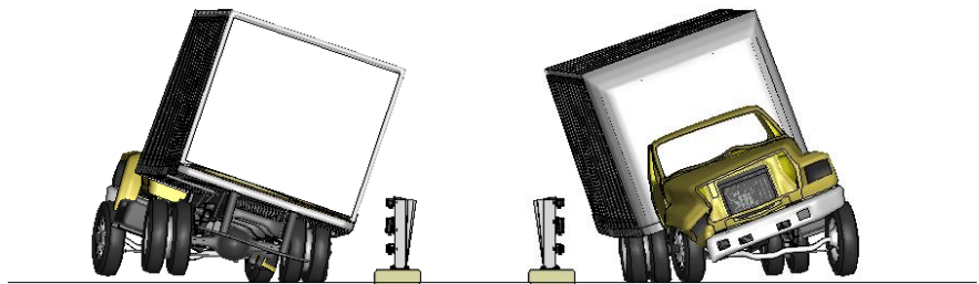
Figure K-2. [Continued] Sequential views from analysis of MASH Test 4-12 for NETC 3-Bar bridge rail from upstream and downstream viewpoints – Case 1.
