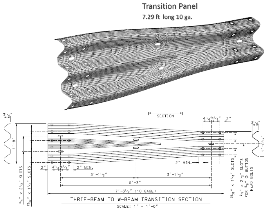
Figure 84. FEA mesh for the thrie-beam transition panel.
