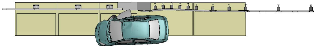
Figure T-1. Sequential views from analysis of MASH Test 4-20 for AGT 4-Bar bridge rail from an overhead viewpoint.
