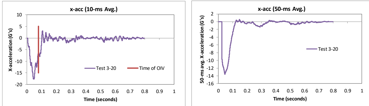
Figure 403. 10- and 50-millisecond average X-acceleration from FEA of Test 3-20 on the 2-bar transition.
