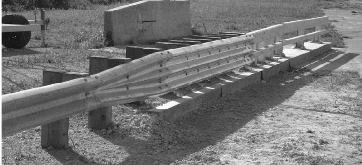
Figure 6. NHDOT 2-Bar rail to thrie-beam AGT. [Alberson06]
