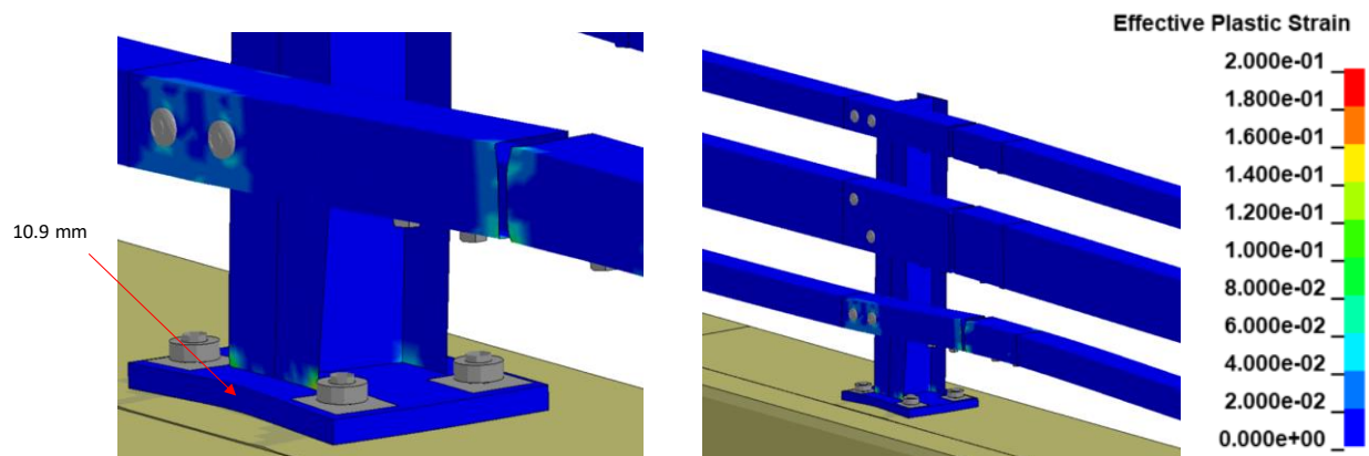
Figure 125. Contours of effective plastic strains for Test 4-10 on the NETC 3-bar bridge rail.
