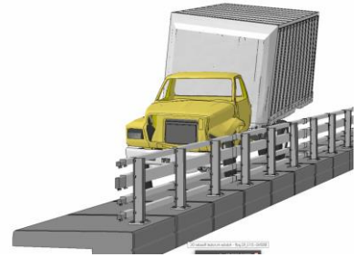
Figure 2. Sequential views of Test NETC-3 and FE analysis from downstream viewpoint.
