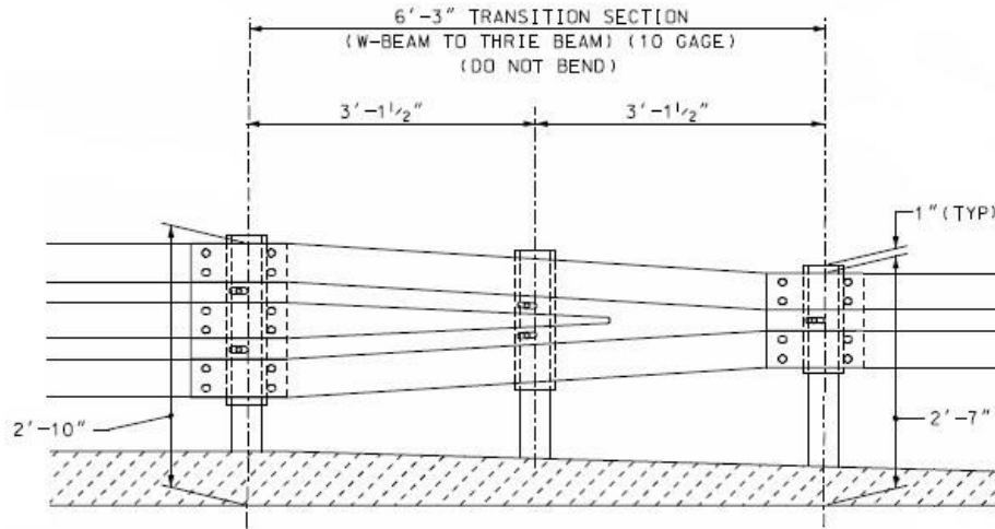
Figure 22. NHDOT T2 AGT symmetrical w-beam to thrie-beam transition section.
