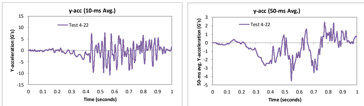
Figure 347. 10- and 50-millisecond average Y-acceleration from FEA of Test 4-22 on the MaineDOT transition (c.g. accelerometer).
