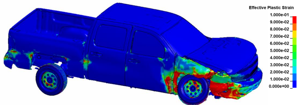
Figure 394. Damages to vehicle in Test 3-11 analysis of the NETC 2-bar bridge rail.
