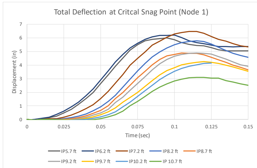
Figure 191. Total deflection of the rail at the critical snag point on the transition for Test 4-21.
