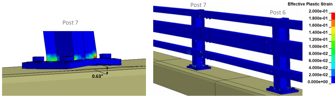
Figure 141. Contours of effective plastic strains for Test 4-11 on the NETC 3-bar bridge rail.
