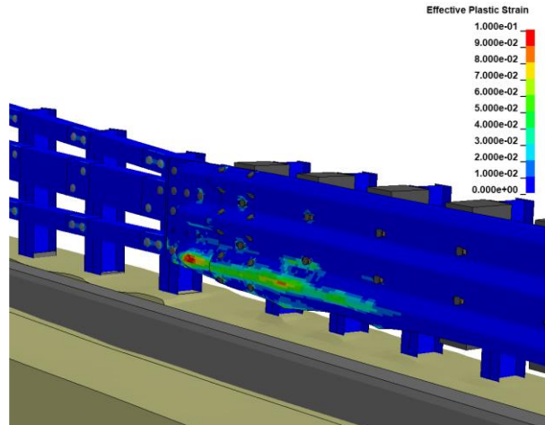
Figure 184. Contours of effective plastic strains on the steel rails and posts for 3-bar transition.
