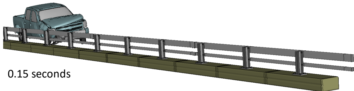
Figure X-3. Sequential views from analysis of MASH Test 3-11 for NETC 2-Bar bridge rail from an oblique viewpoint.
