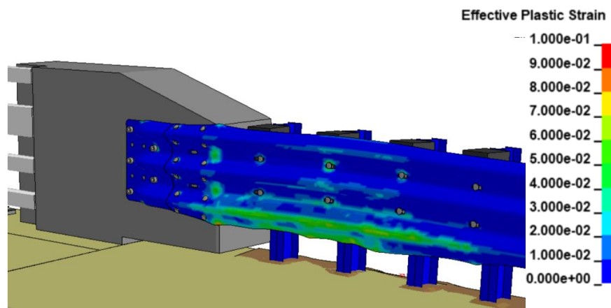
Figure 305. Contours of effective plastic strains on the steel rails and posts for Test 4-20 on the MaineDOT transition.
