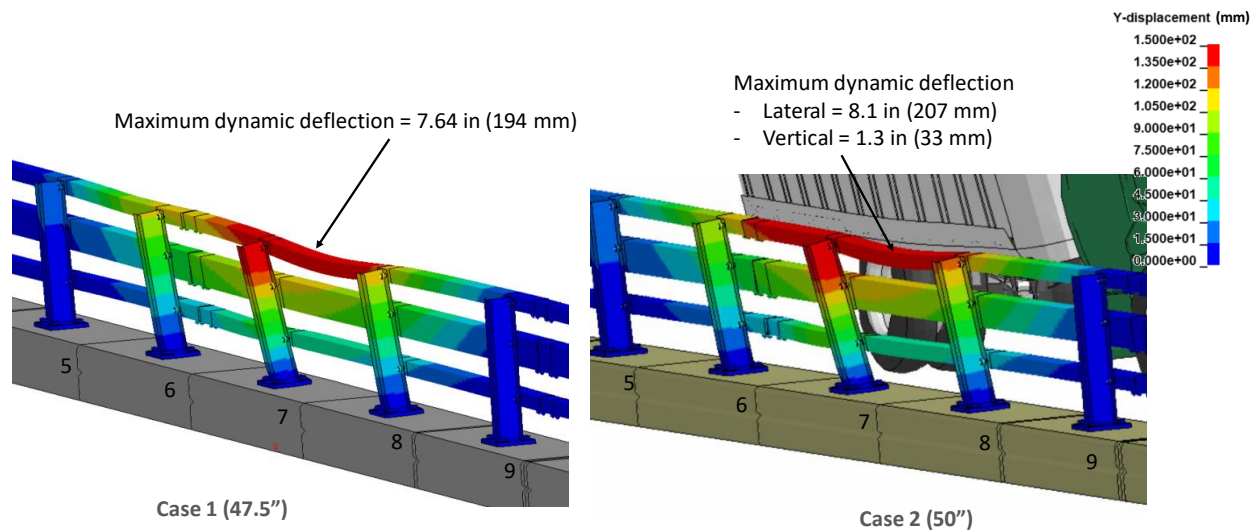
Figure 157. Contour plot of lateral displacement for the bridge rail from Test 4-12 at the time of maximum dynamic deflection for the NETC 3-bar bridge rail.
