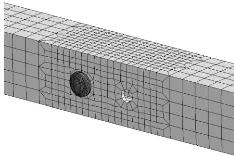
Figure 52. FE mesh of the middle tube-rail and bolt (one bolt removed to facilitate viewing slotted mounting hole).
