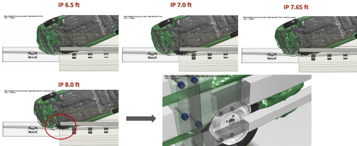
Figure 457. Test 4-20 results at time of potential snag on critical splice.
