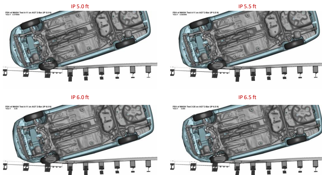
Figure 399. Results of Test 3-20 CIP evaluations for the 2-bar Transition.
