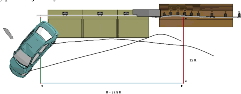
Figure 310. Exit box for Test 4-20 analysis of the 3-bar transition.
