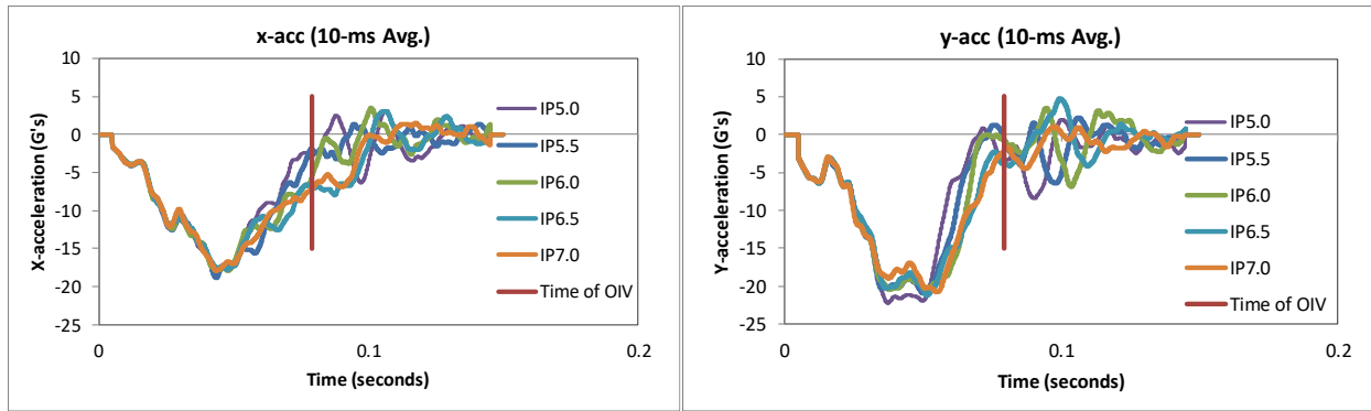
Figure 400. Plots of x-acceleration and y-acceleration measured at the c.g. of the vehicle.
