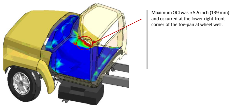
Figure 355. Occupant compartment deformation resulting from Test 4-22 on the MaineDOT transition.
