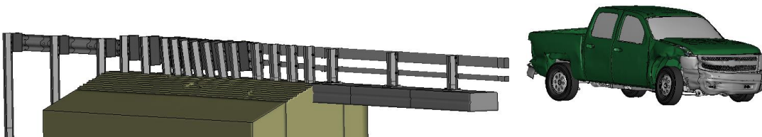
Figure Z-3. [Continued] Sequential views from analysis of MASH Test 3-21 for AGT 2-Bar bridge rail from an oblique viewpoint.
