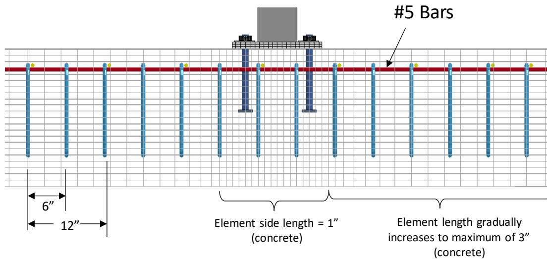
Figure 57. Plan view of sidewalk model (from back of bridge rail).
