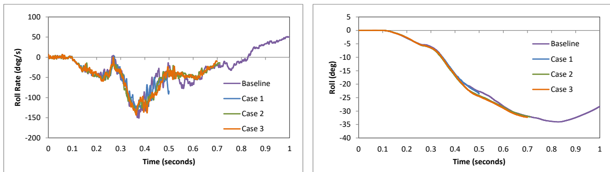
Figure 488. Roll rate and roll angle time-history from FEA of Test 4-22 for Case 1-3 on the 3-bar transition with 5.5-ft post spacing compared with baseline (c.g. accelerometer).
