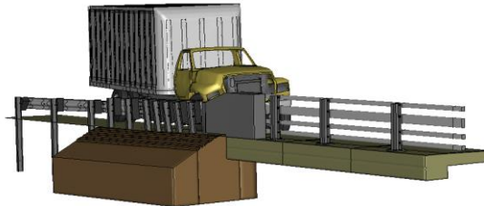
Figure V-3. [Continued] Sequential views from analysis of MASH Test 4-22 for AGT 4-Bar bridge rail from an oblique viewpoint.
