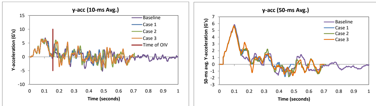
Figure 485. 10- and 50-millisecond average Y-acceleration from FEA of Test 4-22 for Case 1-3 on the 3-bar transition with 5.5-ft post spacing compared with baseline (cabin accelerometer).
