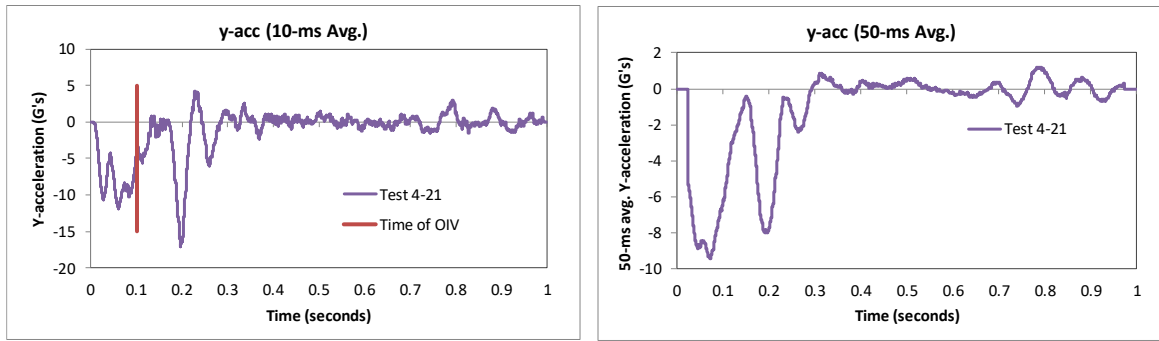
Figure 425. 10- and 50-millisecond average Y-acceleration from FEA of Test 3-21 on the 2-bar transition.
