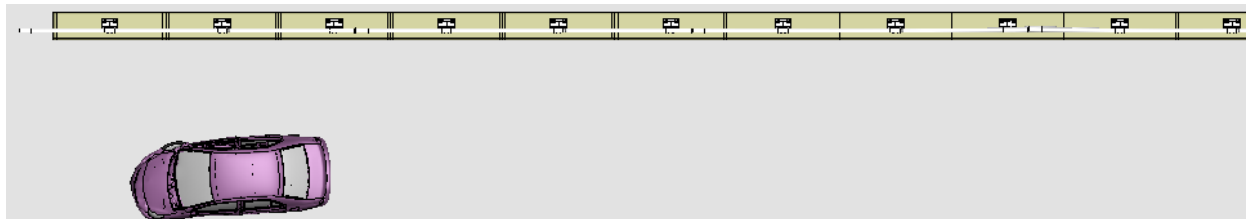
Figure W-1. [Continued] Sequential views from analysis of MASH Test 3-10 for NETC 2-Bar bridge rail from an overhead viewpoint.
