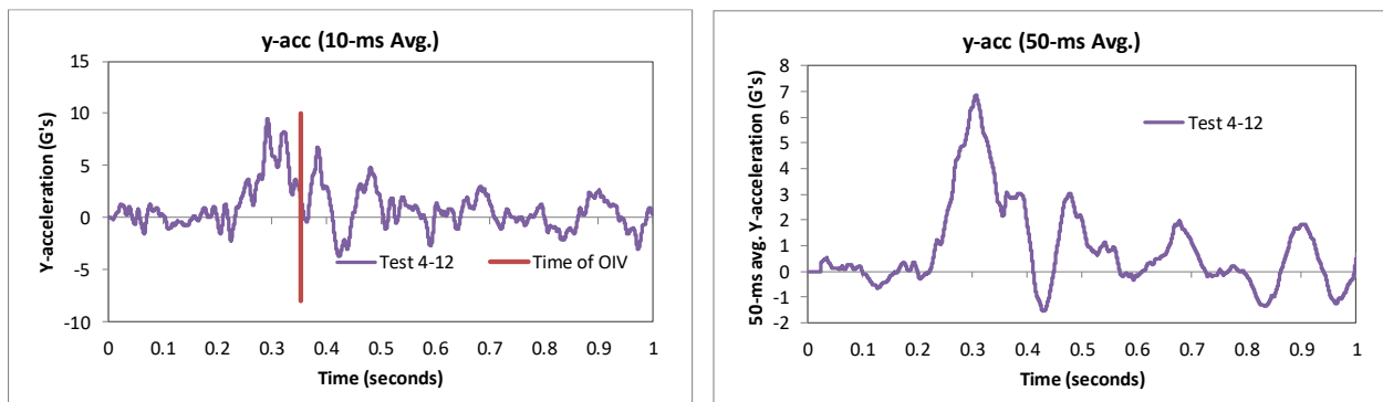
Figure 268. 10- and 50-millisecond average Y-acceleration from FEA of Test 4-12 on the NETC 4-bar bridge rail (cabin accelerometer).
