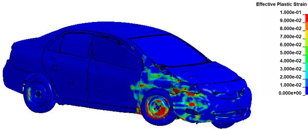
Figure 244. Damages to vehicle in Test 4-10 analysis of the NETC 4-bar bridge rail.
