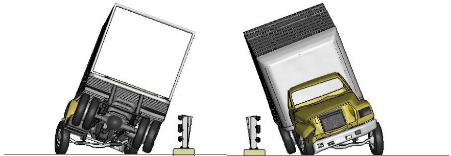
Figure K-2. [Continued] Sequential views from analysis of MASH Test 4-12 for NETC 3-Bar bridge rail from upstream and downstream viewpoints – Case 1.
