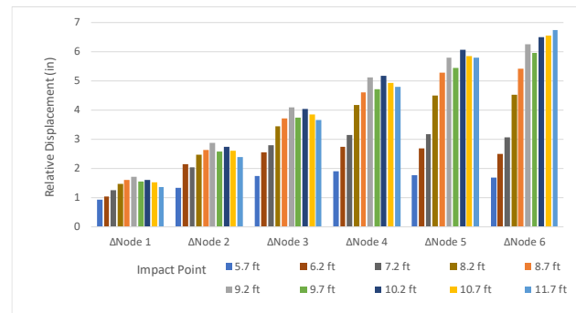
Figure 189. Relative displacements of rail for Test 4-21 simulations in CIP evaluations.
