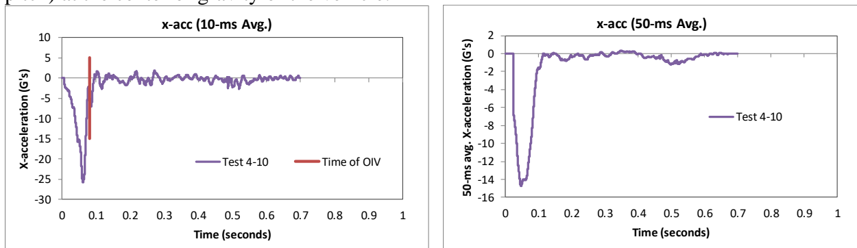
Figure 115. 10- and 50-millisecond average X-acceleration from FEA of Test 4-10 on the NETC 3-bar bridge rail.
