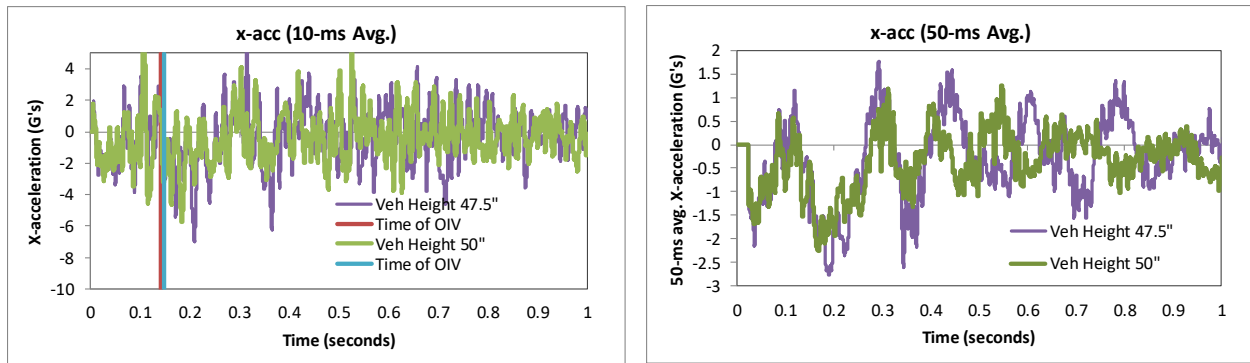
Figure 150. 10- and 50-millisecond average X-acceleration from FEA of Test 4-12 on the NETC 3-bar bridge rail (cabin accelerometer).
