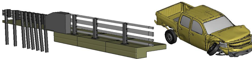
Figure U-3. [Continued] Sequential views from analysis of MASH Test 4-21 for AGT 4-Bar bridge rail from an oblique viewpoint.
