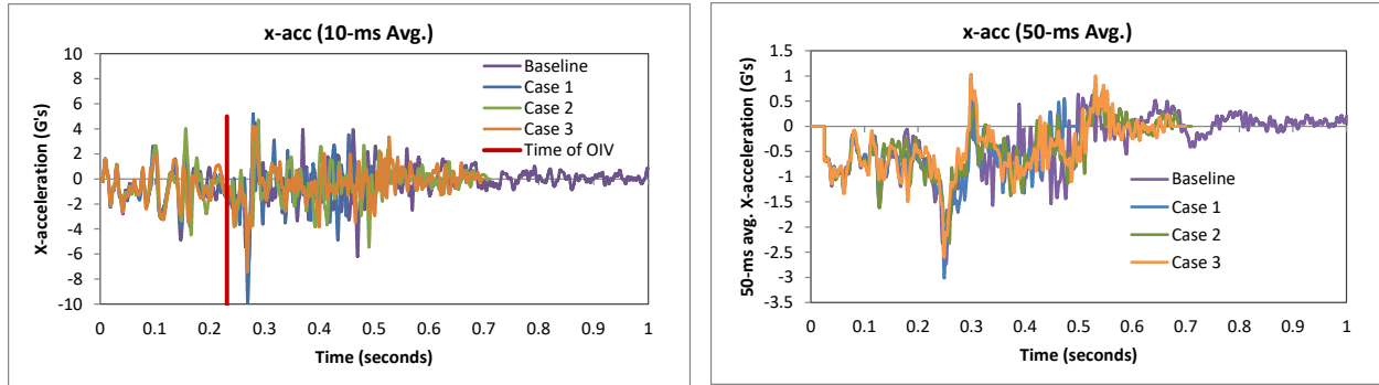
Figure 481. 10- and 50-millisecond average X-acceleration from FEA of Test 4-22 for Case 1-3 on the 3-bar transition with 5.5-ft post spacing compared with baseline (c.g. accelerometer).
