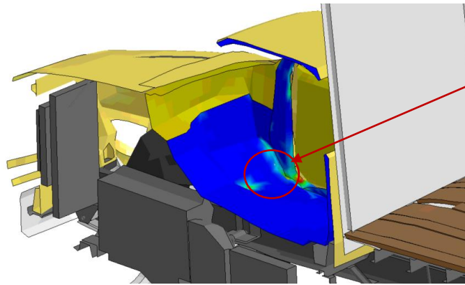
Figure 156. Occupant compartment deformation resulting from Test 4-12 on the NETC 3-bar bridge rail system.
