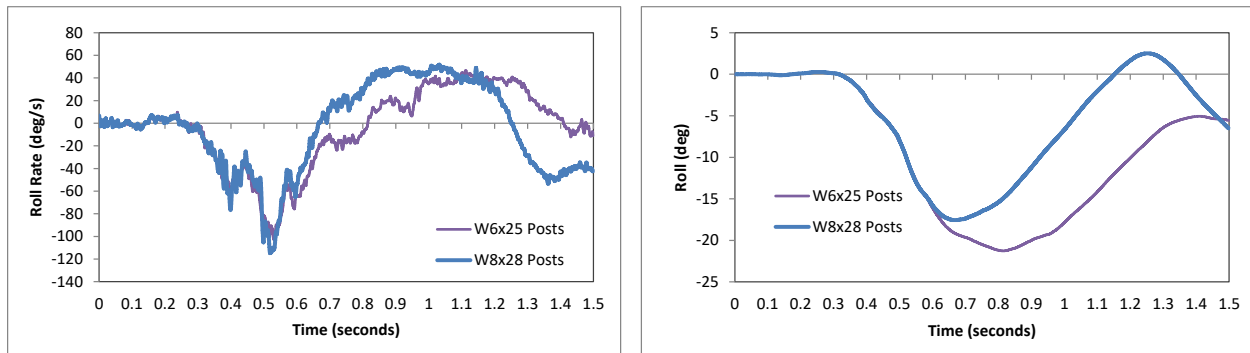
Figure 504. Roll rate and roll angle time-history from FEA of Test 4-12 on the baseline and modified NETC 4-bar bridge rail (c.g. accelerometer).
