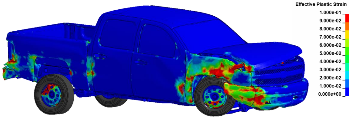
Figure 260. Damages to vehicle in Test 4-11 analysis of the NETC 4-bar bridge rail.
