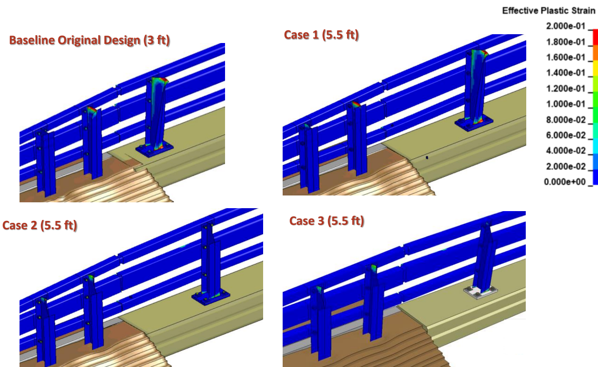
Figure 492. Contour plot of effective plastic strain for Cases 1-3 compared with baseline case.
