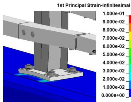
Figure 126. Contours of 1 st principal strains for concrete at the critical post for Test 4-10 on the NETC 3-bar bridge rail.
