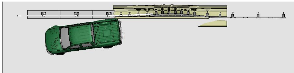
Figure Z-1. [Continued] Sequential views from analysis of MASH Test 3-21 for AGT 2-Bar bridge rail from an overhead viewpoint.
