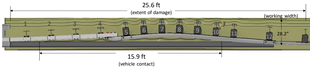
Figure 431. Overhead view of 2-bar transition after Test 3-21 showing extent of damage.
