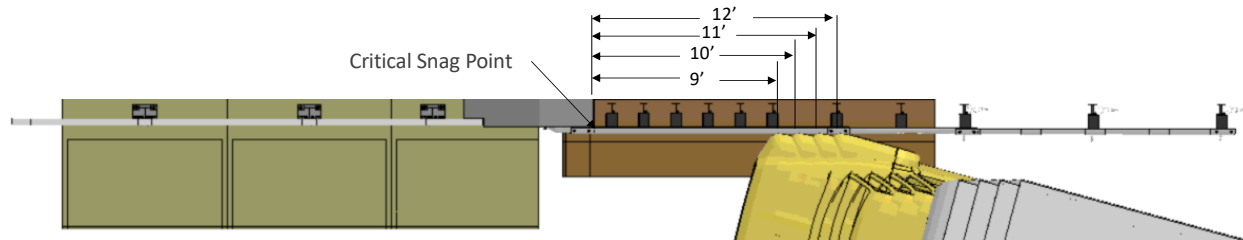
Figure 340. Illustration of potential snag point for Test 4-22 on the MaineDOT transition and impact points evaluated.
