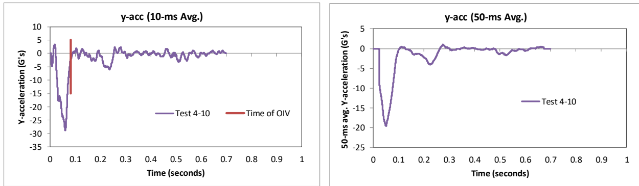
Figure 116. 10- and 50-millisecond average Y-acceleration from FEA of Test 4-10 on the NETC 3-bar bridge rail.
