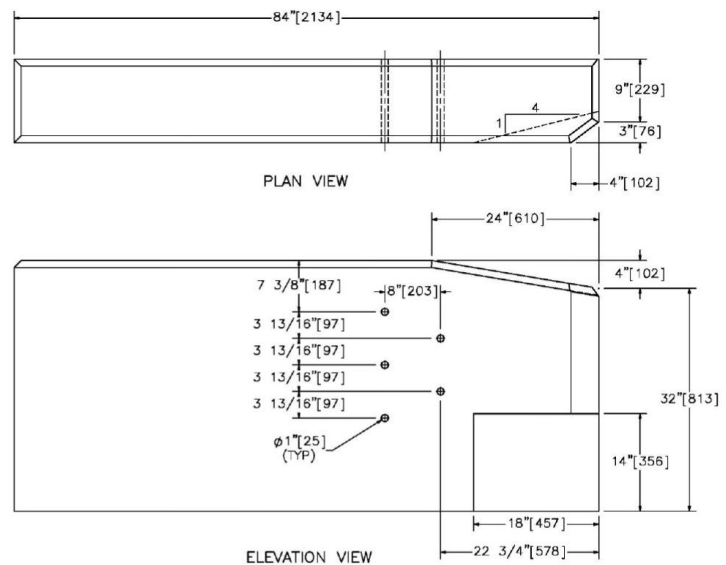
Figure 35. Standardized buttress design. [Rosenbaugh18]
