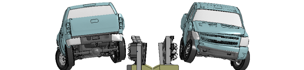
Figure O-2. [Continued] Sequential views from analysis of MASH Test 4-21 for AGT 3-Bar transition from upstream and downstream viewpoints.
