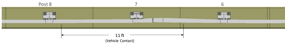
Figure 373. Overhead view of NETC 3-bar bridge rail after Test 3-10 showing extent of damage.
