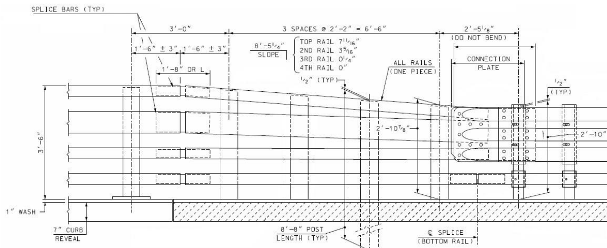
Figure 40. NHDOT T4 AGT sloped rail section.
