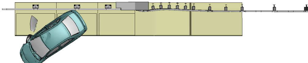
Figure T-1. [Continued] Sequential views from analysis of MASH Test 4-20 for AGT 4-Bar bridge rail from an overhead viewpoint.
