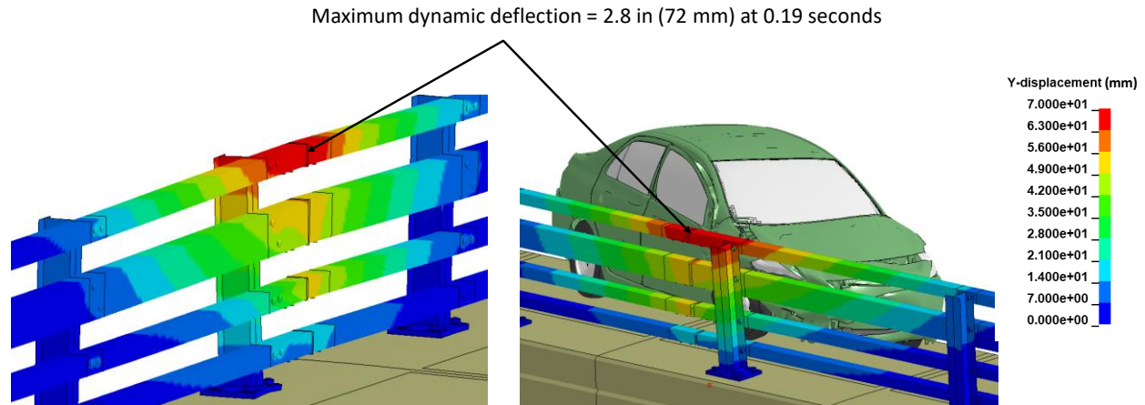
Figure 240. Contour plot of lateral displacement for the bridge rail for Test 4-10 at the time of maximum dynamic deflection.
