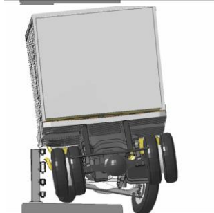
Figure 64. [CONTINUED] Sequential views of Test NETC-3 and FE analysis from upstream viewpoint.
