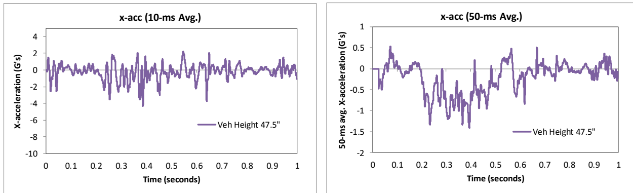
Figure 264. 10- and 50-millisecond average X-acceleration from FEA of Test 4-12 on the NETC 4-bar bridge rail (c.g. accelerometer).
