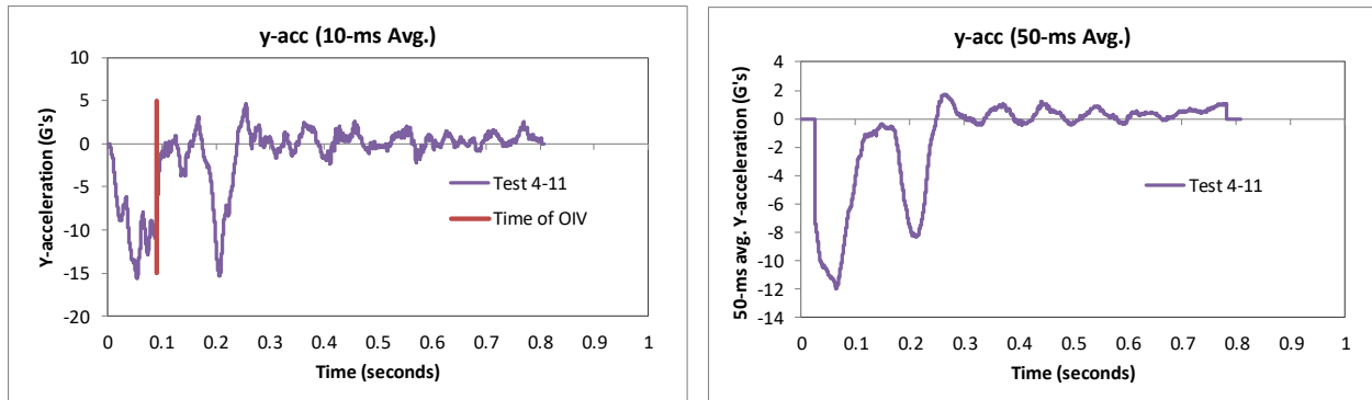
Figure 132. 10- and 50-millisecond average Y-acceleration from FEA of Test 4-11 on the NETC 3-bar bridge rail.
