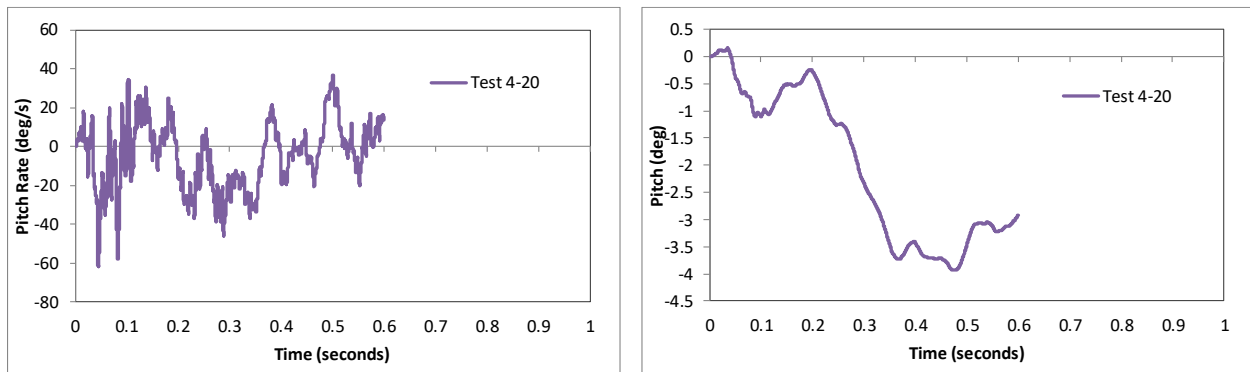
Figure 179. Pitch rate and pitch angle time-history from FEA of Test 4-20 on the 3-bar transition.
