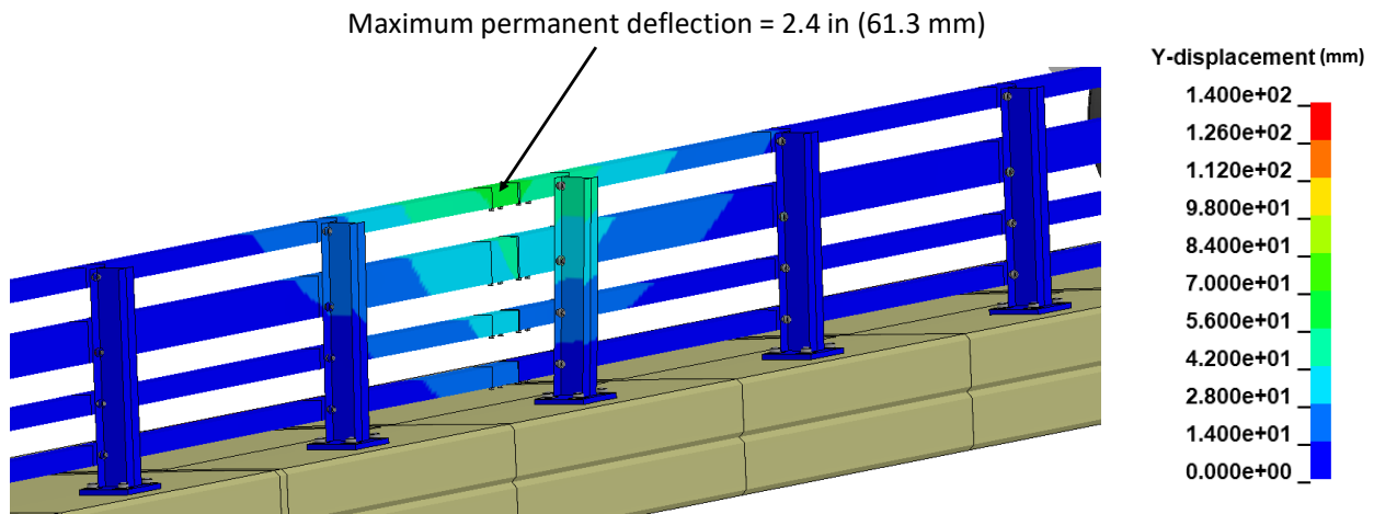
Figure 257. Contour plot of maximum permanent deflection of the bridge rail for test 4-11.
