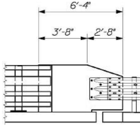
Figure 34. MaineDOT Type IA AGT concrete buttress section.
