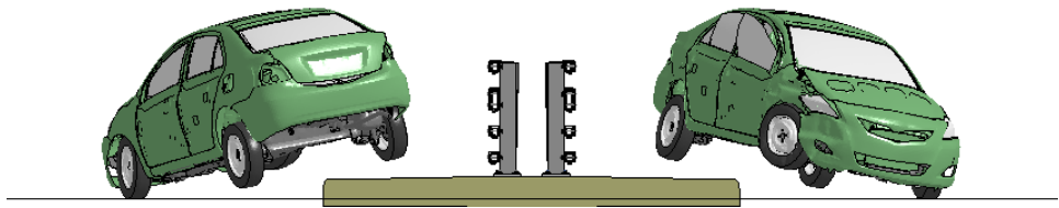
Figure Q-2. [Continued] Sequential views from analysis of MASH Test 4-10 for NETC 4-Bar bridge rail from upstream and downstream viewpoints.
