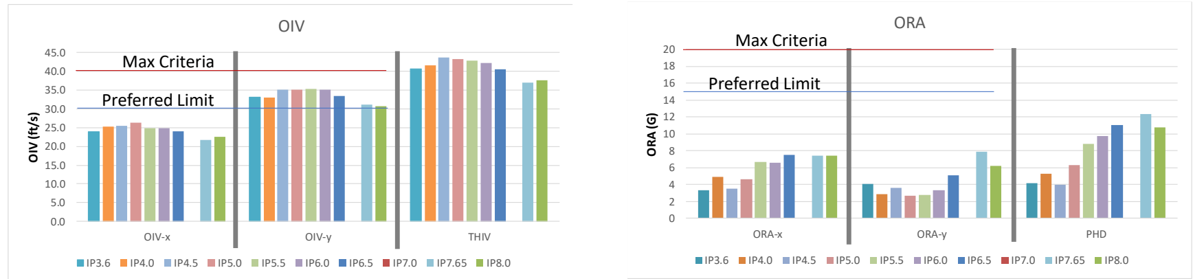
Figure 459. Graphical representation of OIV, THIV, ORA and PHD metrics for Test 4-20.
