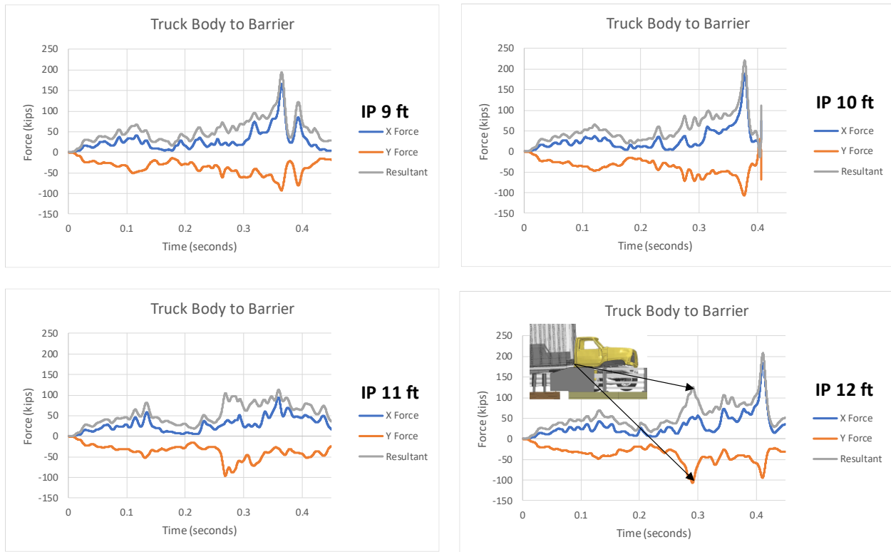
Figure 341. Longitudinal, lateral and resultant forces on barrier for each analysis case.
