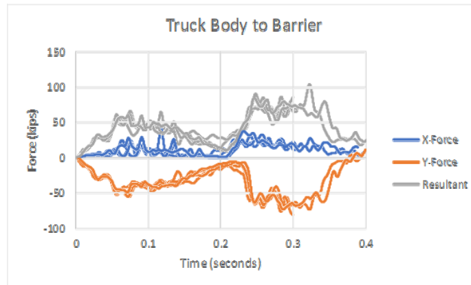
Figure 210. Overlay of force-time history for all cases.
