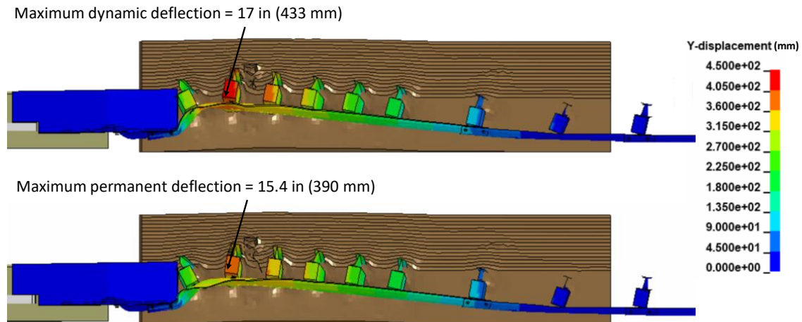
Figure 356. Contour plot of lateral displacement for the MaineDOT transition for Test 4-22 at the time of maximum dynamic deflection.
