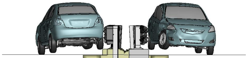
Figure Y-2. [Continued] Sequential views from analysis of MASH Test 3-20 for AGT 2-Bar bridge rail from upstream and downstream viewpoints.
