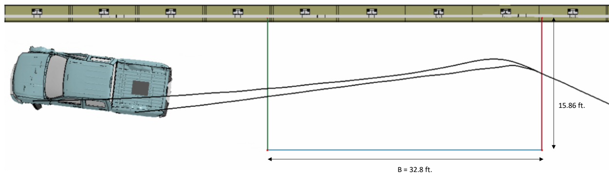
Figure 395. Exit box for Test 3-11 analysis of the NETC 2-bar bridge rail.
