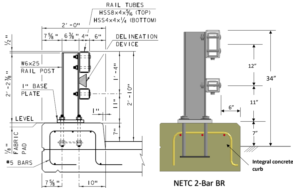
Figure 364. Section view drawing and the FEA model of the NETC 2-Bar bridge rail.
