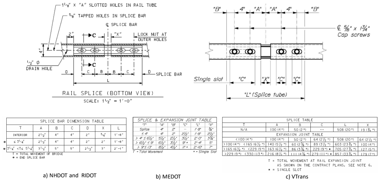
Figure 19. Expansion splice details for a) NHDOT and RIDOT, b) MaineDOT and c) VTrans.
