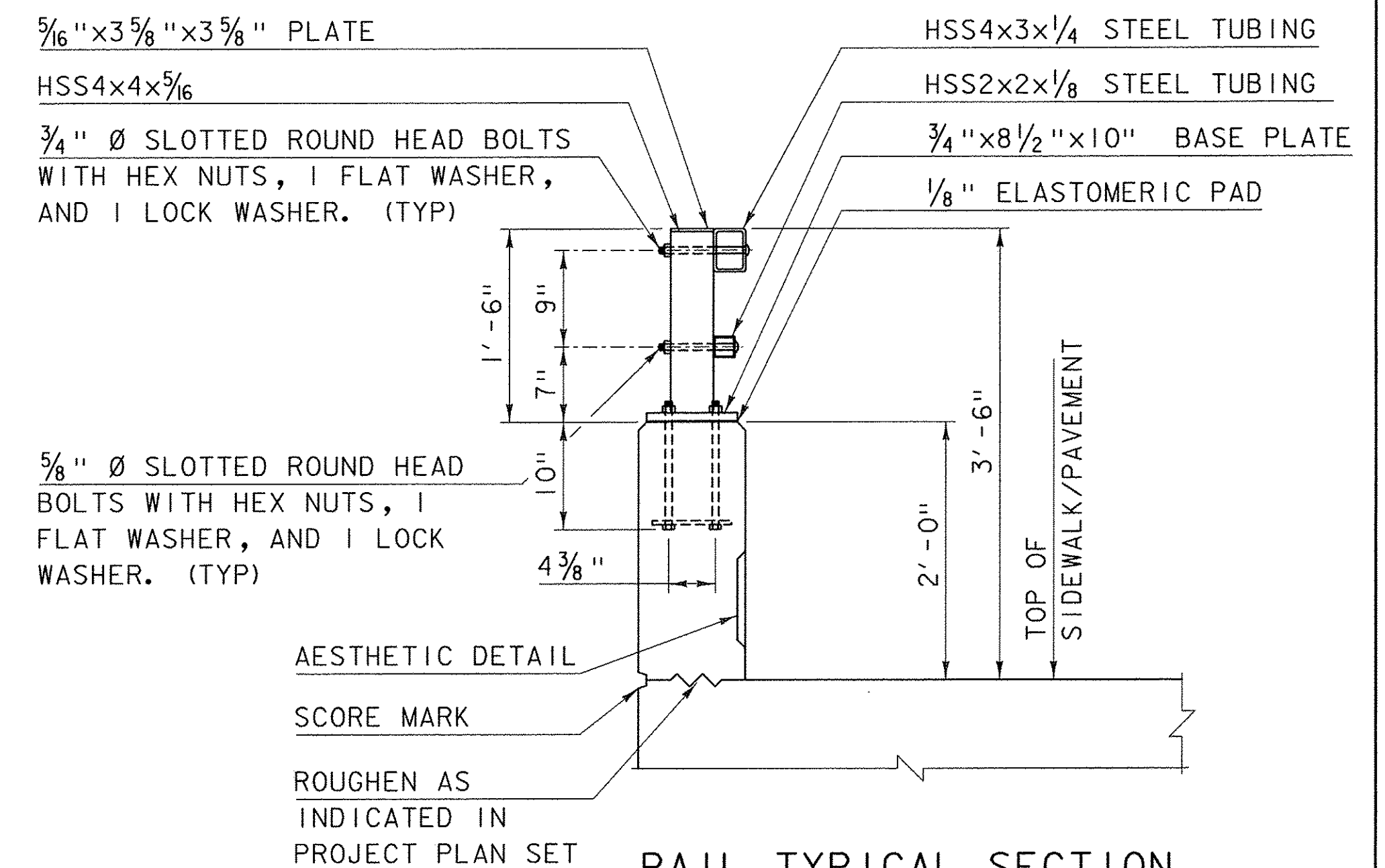
RAIL TYPICAL SECTION
