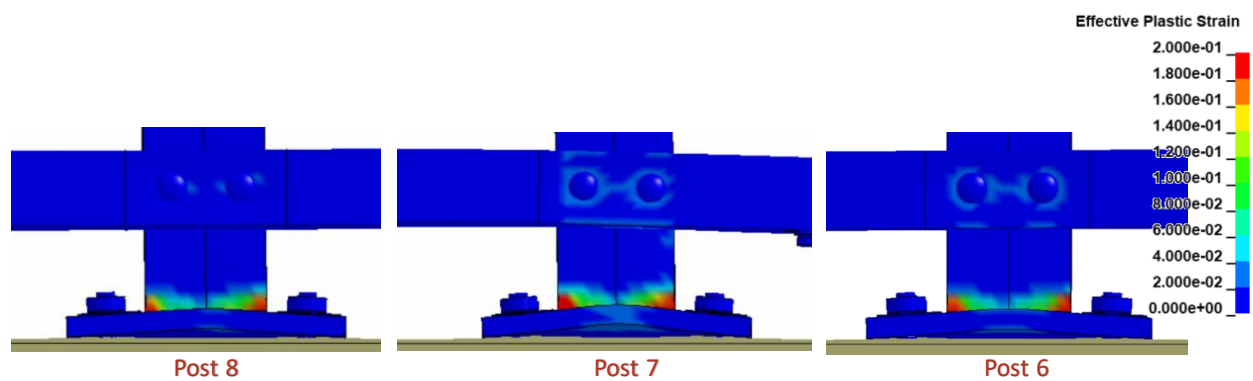
Figure 277. Contours of effective plastic strains on the critical post for Test 4-12 on the NETC 4-bar bridge rail.
