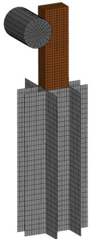
FEA Model
