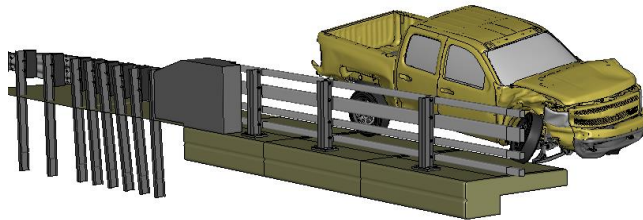
Figure U-3. [Continued] Sequential views from analysis of MASH Test 4-21 for AGT 4-Bar bridge rail from an oblique viewpoint.
