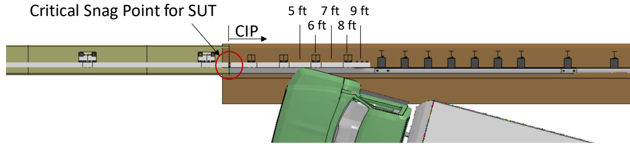
Figure 208. Illustration of potential snag point for Test 4-22 on the 3-bar transition and impact points evaluated.
