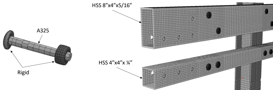
Figure 92. FEA mesh of the transition tube rails.
