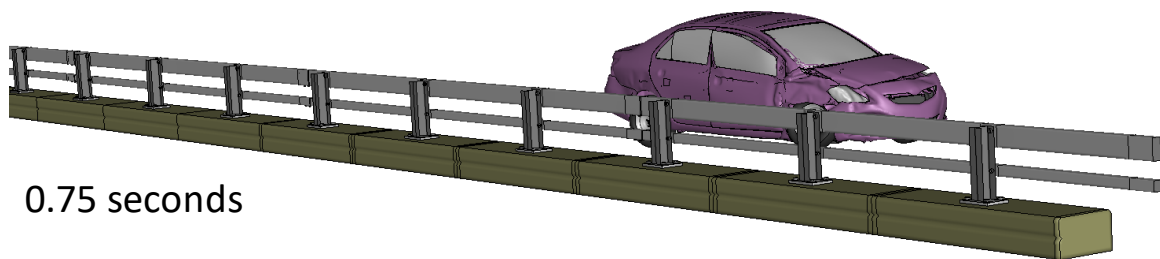
Figure W-3. [Continued] Sequential views from analysis of MASH Test 3-10 for NETC 2-Bar bridge rail from an oblique viewpoint.
