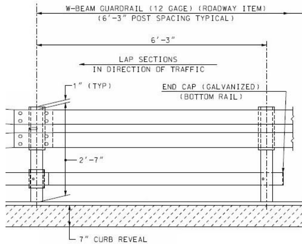
Figure 37. NHDOT T4 AGT upstream w-beam section (VTrans similar except bottom bar and sidewalk).
