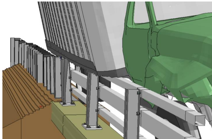
Figure 211. Cargo-box bed rails snag on top of bridge rail posts.
