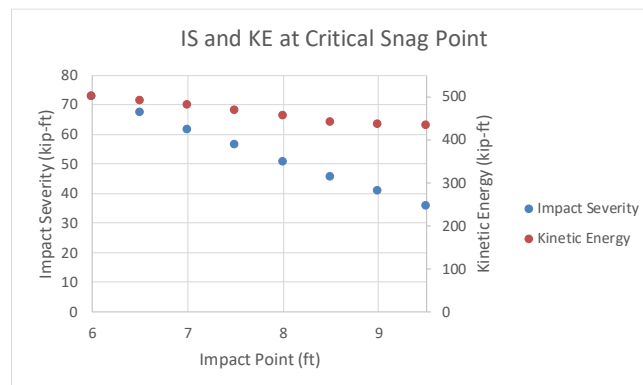
Figure 421. Impact severity and kinetic energy of the vehicle at the time when the vehicle is positioned at the critical snag point.
