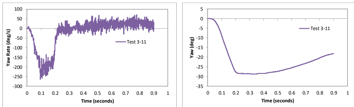
Figure 385. Yaw rate and yaw angle time-history from FEA of Test 3-11 on the NETC 2-bar bridge rail.
