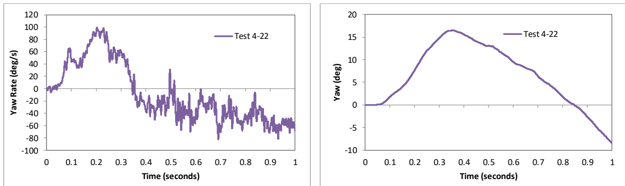
Figure 218. Yaw rate and yaw angle time-history from FEA of Test 4-22 on the 3-bar transition (cabin accelerometer).
