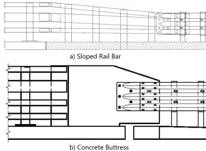
Figure 20. Drawings of the two design concepts for NETC approach guardrail transitions (AGT).
