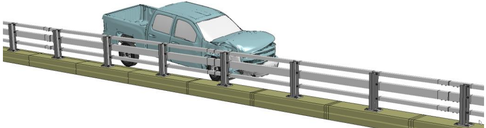
Figure K-3. [Continued] Sequential views from analysis of MASH Test 4-11 for NETC 3-Bar bridge rail from from an oblique viewpoint.
