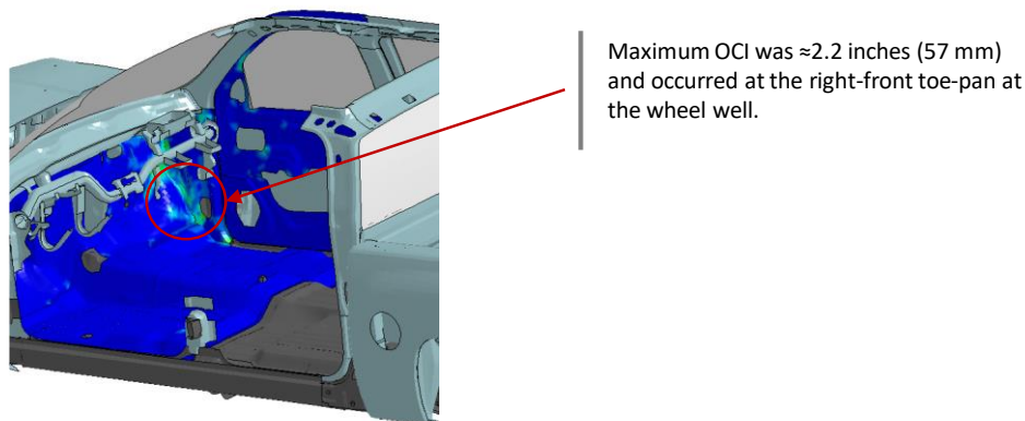
Figure 255. Occupant compartment deformation resulting from Test 4-11 on the NETC 4-bar bridge rail.
