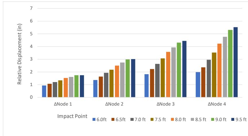
Figure 418. Relative displacements of rail for Test 3-21 simulations in CIP evaluations.
