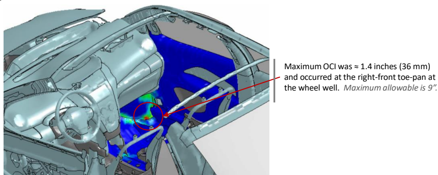
Figure 409. Occupant compartment deformation resulting from Test 3-20 on the 2-bar transition.
