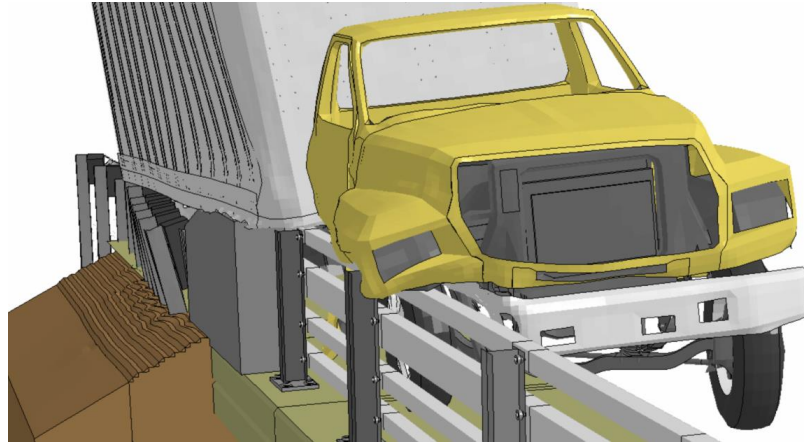
Figure 343. Cargo-box bed rails snag on top of bridge rail posts.
