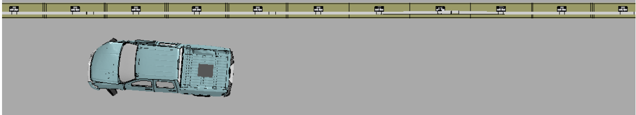
Figure K-1. [Continued] Sequential views from analysis of MASH Test 4-11 for NETC 3-Bar bridge rail from an overhead viewpoint.
