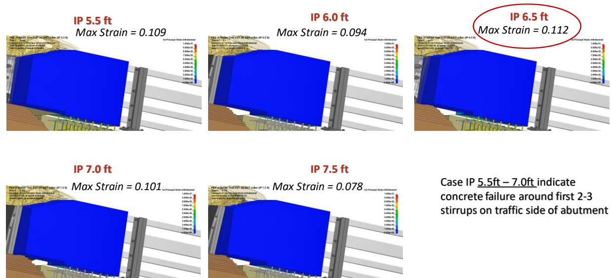
Figure 321. Contour plots of 1 st principle strain for the buttress.
