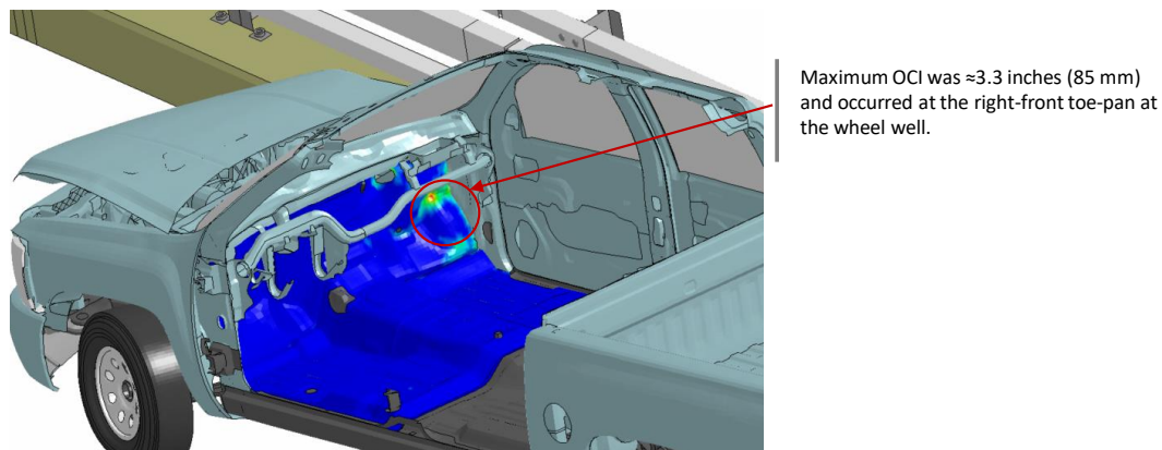
Figure 137. Occupant compartment deformation resulting from Test 4-11 on the NETC 3-bar bridge rail.
