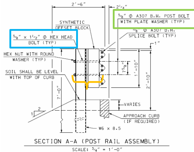
Figure 25. Post rail assembly NHDOT T2 AGT (T3 similar)
