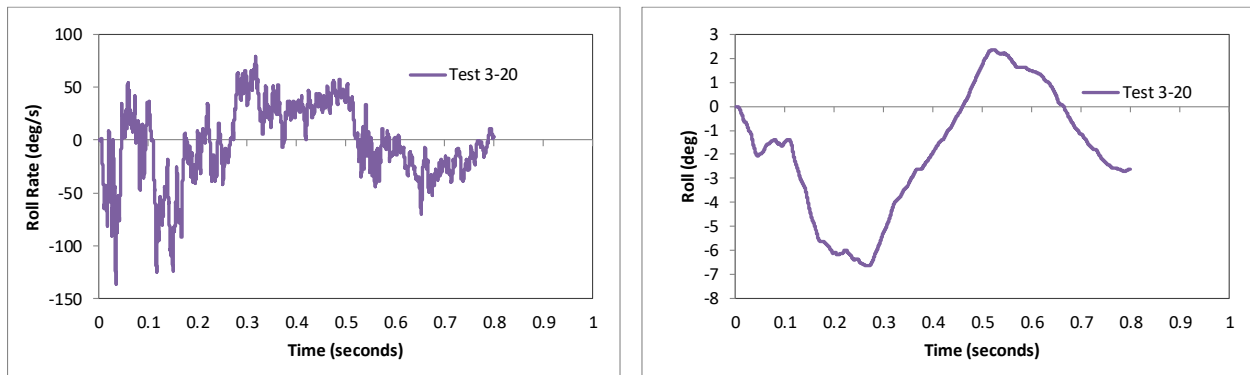
Figure 407. Roll rate and roll angle time-history from FEA of Test 3-20 on the 2-bar transition.
