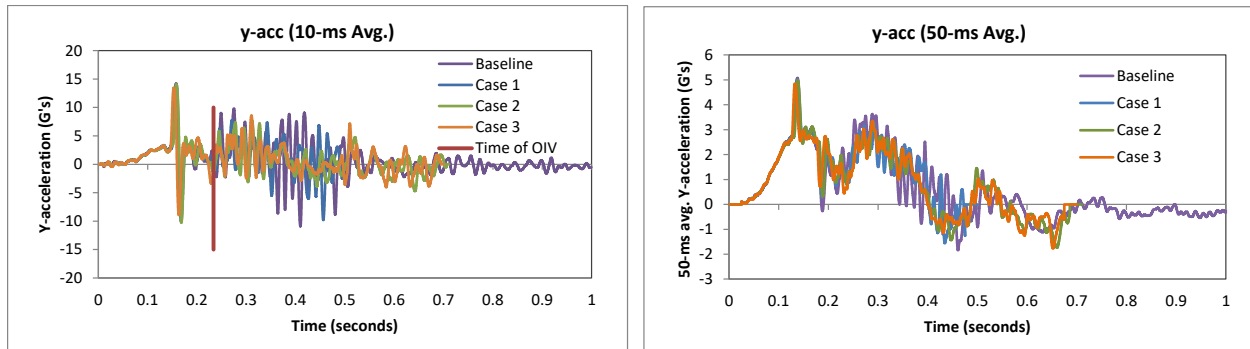
Figure 482. 10- and 50-millisecond average Y-acceleration from FEA of Test 4-22 for Case 1-3 on the 3-bar transition with 5.5-ft post spacing compared with baseline (c.g. accelerometer).
