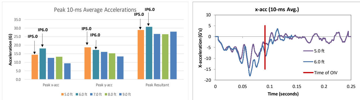
Figure 476. Peak 10-ms moving average acceleration data for Test 4-21 impact cases.
