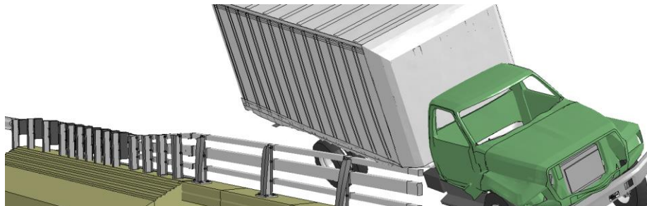
Figure P-3. [Continued] Sequential views from analysis of MASH Test 4-22 for AGT 3-Bar transition from an oblique viewpoint.
