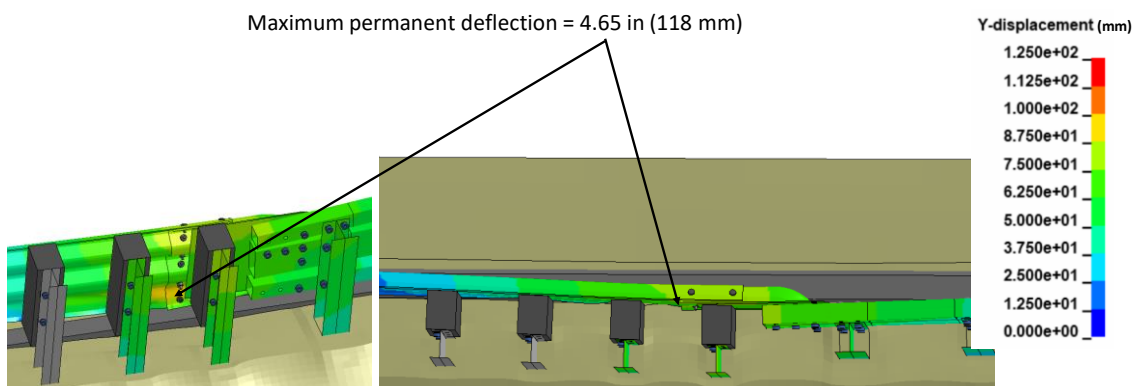
Figure 183. Contour plot of maximum permanent deflection for the transition.
