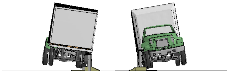
Figure P-2. [Continued] Sequential views from analysis of MASH Test 4-22 for AGT 3-Bar transition from upstream and downstream viewpoints.
