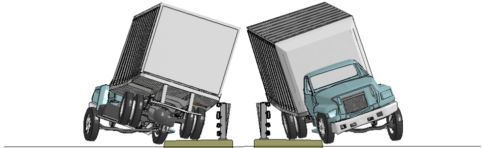
Figure S-2. [Continued] Sequential views from analysis of MASH Test 4-12 for NETC 4-Bar bridge rail from upstream and downstream viewpoints.
