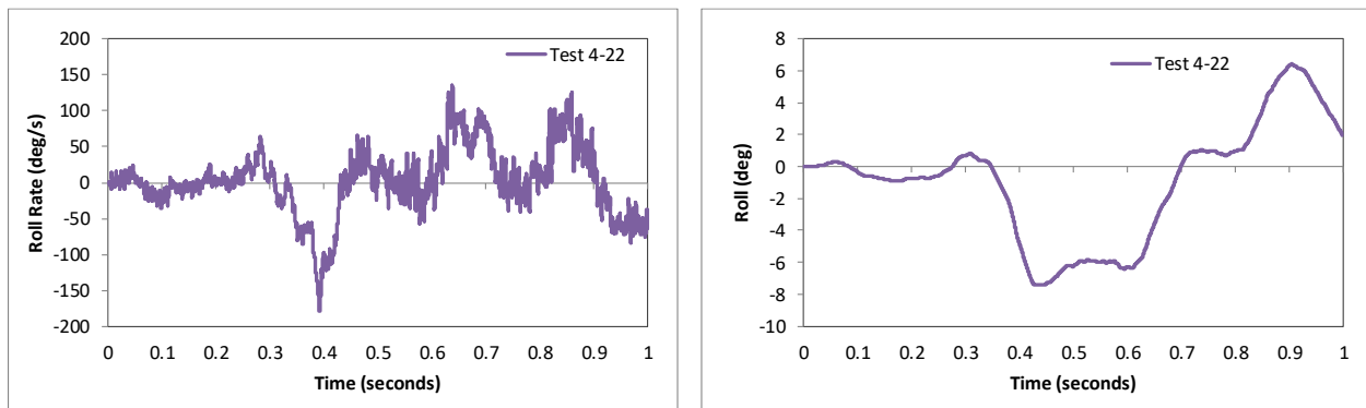
Figure 353. Roll rate and roll angle time-history from FEA of Test 4-22 on the MaineDOT transition (cabin accelerometer).
