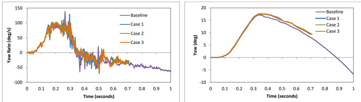
Figure 487. Yaw rate and yaw angle time-history from FEA of Test 4-22 for Case 1-3 on the 3-bar transition with 5.5-ft post spacing compared with baseline (c.g. accelerometer).
