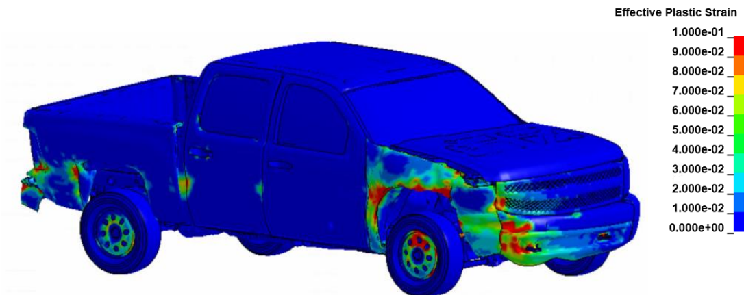
Figure 434. Damages to vehicle in Test 3-21 analysis of the 2-bar transition.
