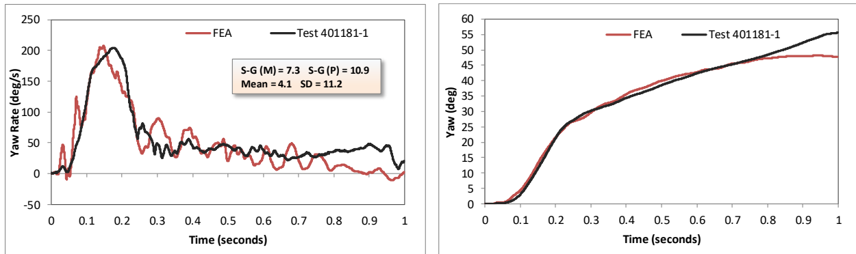
Figure 105. Yaw-time history plot from accelerometer inside cabin for full-scale test 401181-1 and FEA (angular rate and displacement).
