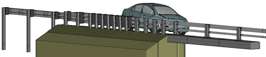
Figure Y-3. Sequential views from analysis of MASH Test 3-20 for AGT 2-Bar bridge rail from an oblique viewpoint.
