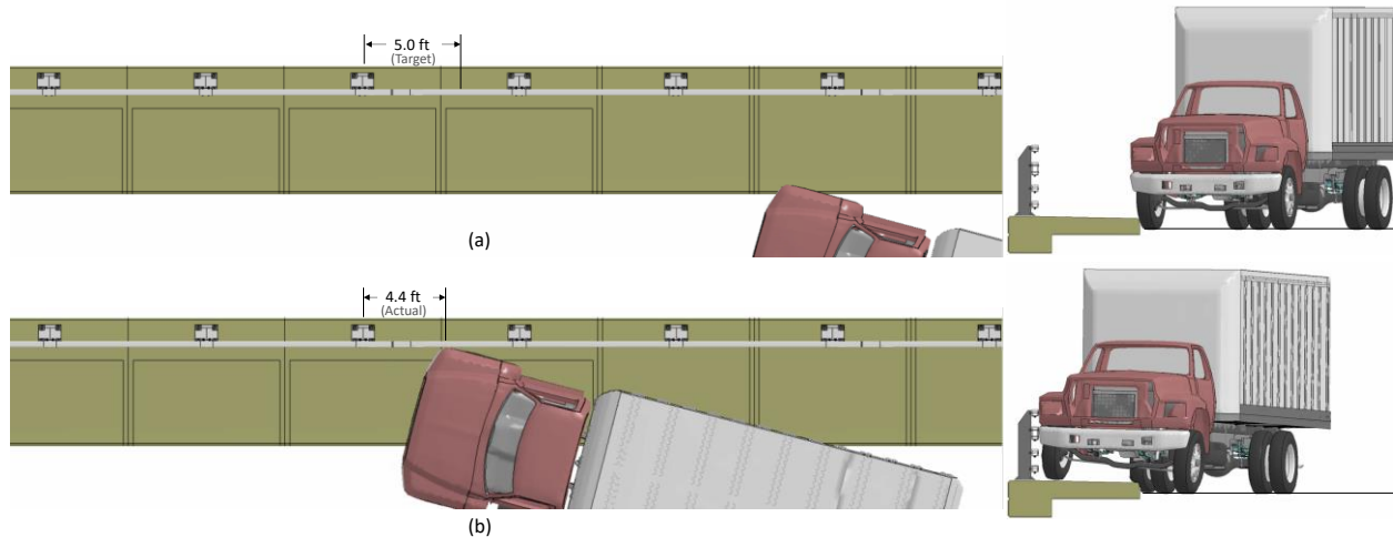
Figure 495. (a) Target and (b) actual impact point for Test 4-12 on the modified NETC 4-Bar bridge rail.
