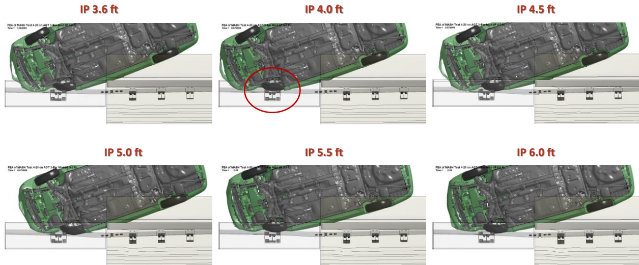
Figure 456. Test 4-20 results at time of potential impact with critical post.
