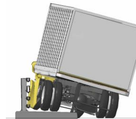
Figure 64. [CONTINUED] Sequential views of Test NETC-3 and FE analysis from upstream viewpoint.
