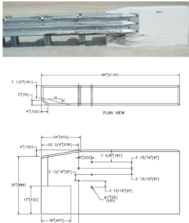
Figure 312. Concrete AGT tested by MwRSF (Test 34AGT-2). [Rosenbaugh19]
