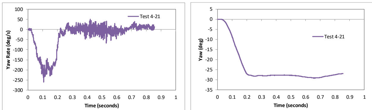
Figure 197. Yaw rate and yaw angle time-history from FEA of Test 4-21 on the 3-bar transition.
