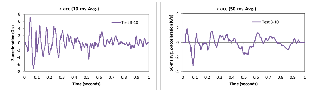
Figure 368. 10- and 50-millisecond average Z-acceleration from FEA of Test 3-10 on the NETC 2-bar bridge rail.
