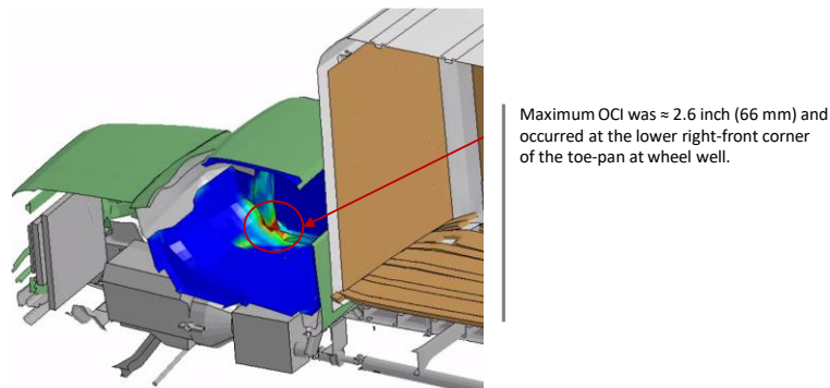
Figure 221. Occupant compartment deformation resulting from Test 4-12 on the NETC 3-bar bridge rail system.
