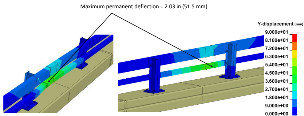
Figure 375. Contour plot of maximum permanent deflection of the NETC 2-bar bridge rail for test 3-10.
