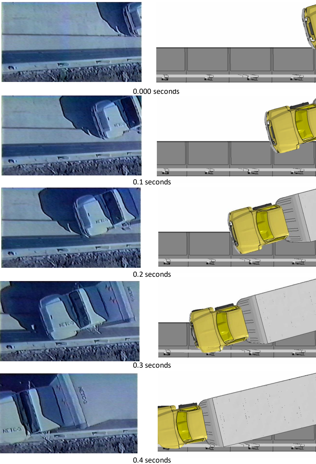
Figure 66. Sequential views of Test NETC-3 and FE analysis from overhead viewpoint.
