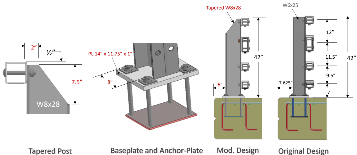
Figure 494. Design modifications for the 4-bar bridge rail.
