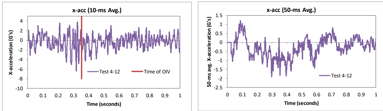
Figure 267. 10- and 50-millisecond average X-acceleration from FEA of Test 4-12 on the NETC 4-bar bridge rail (cabin accelerometer).
