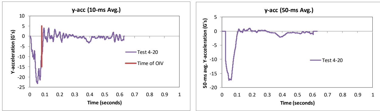
Figure 298. 10- and 50-millisecond average Y-acceleration from FEA of Test 4-20 on the MaineDOT transition.
