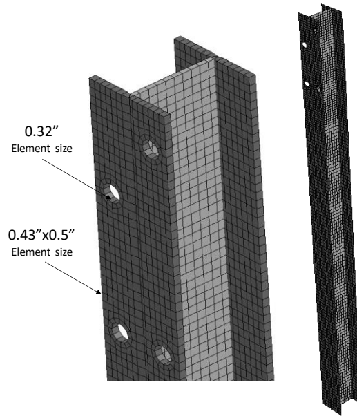
Figure 91. FEA mesh of the W6x25 posts of the transition.
