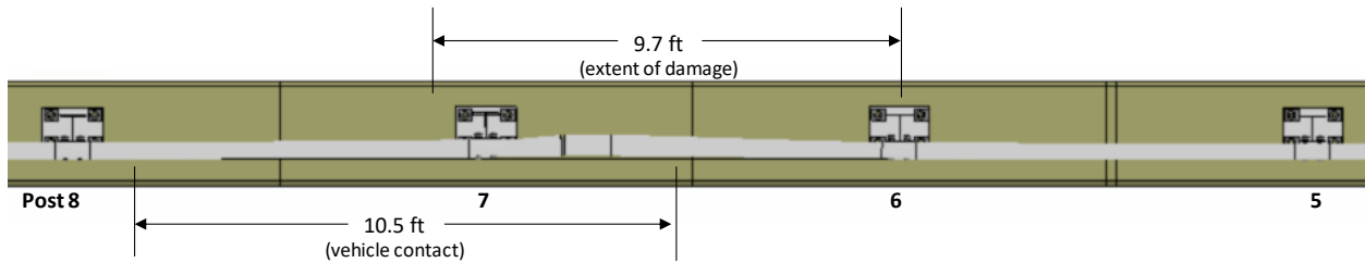
Figure 122. Overhead view of NETC 3-bar bridge rail after Test 4-10 showing extent of damage.
