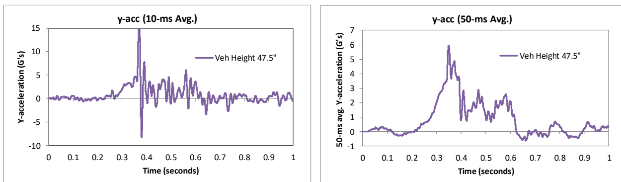
Figure 265. 10- and 50-millisecond average Y-acceleration from FEA of Test 4-12 on the NETC 4-bar bridge rail (c.g. accelerometer).
