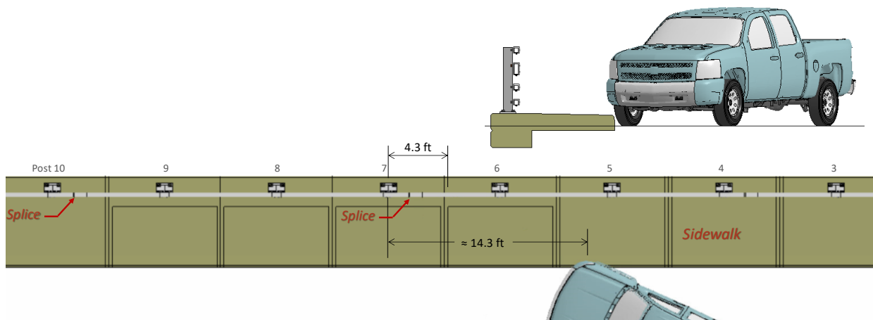
Figure 247. Initial starting point and target impact point for Test 4-11 on the NETC 4-bar bridge rail.
