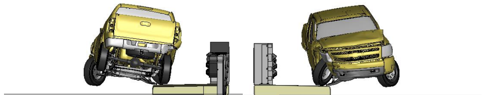
Figure U-2. [Continued] Sequential views from analysis of MASH Test 4-21 for AGT 4-Bar bridge rail from upstream and downstream viewpoints.
