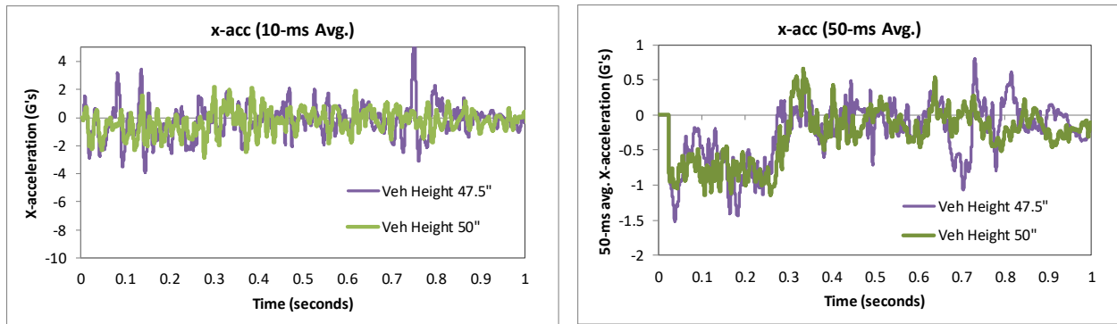
Figure 147. 10- and 50-millisecond average X-acceleration from FEA of Test 4-12 on the NETC 3-bar bridge rail (c.g. accelerometer).
