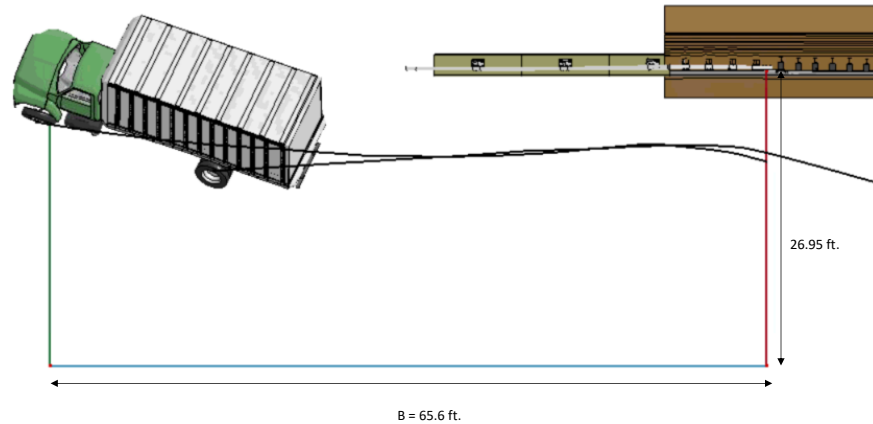
Figure 228. Exit box for Test 4-22 for the 3-bar transition.
