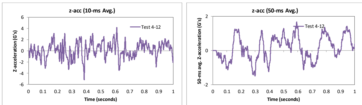
Figure 269. 10- and 50-millisecond average Z-acceleration from FEA of Test 4-12 on the NETC 4-bar bridge rail (cabin accelerometer).
