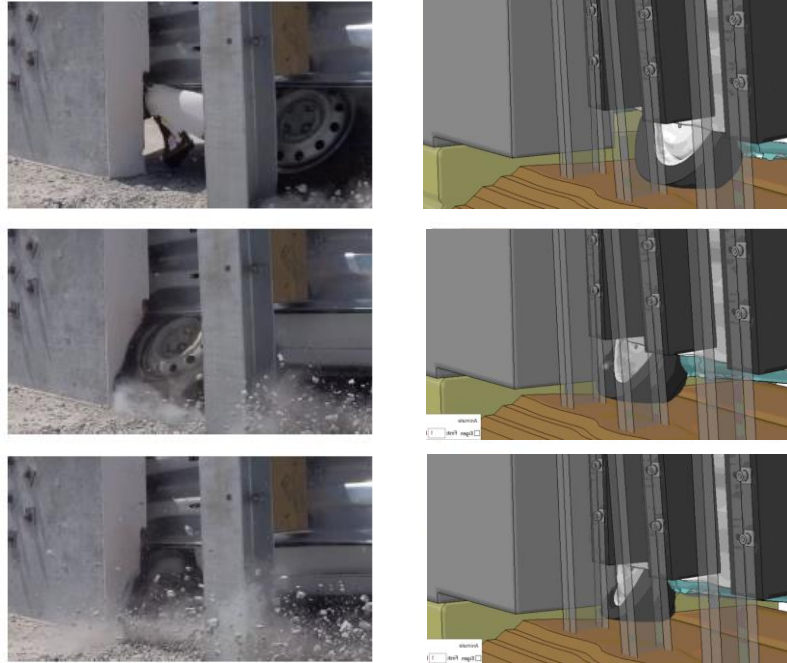
Figure 313. Tire snag on the buttress for Test 34AGT-2 and the FEA analysis.
