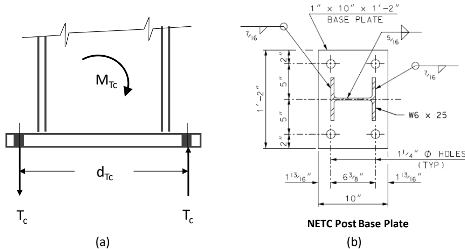
Figure 14. (a) Assumed load/reaction points for the anchor bolt pry-out resistance calculations and (b) dimensions of the NETC baseplate.
