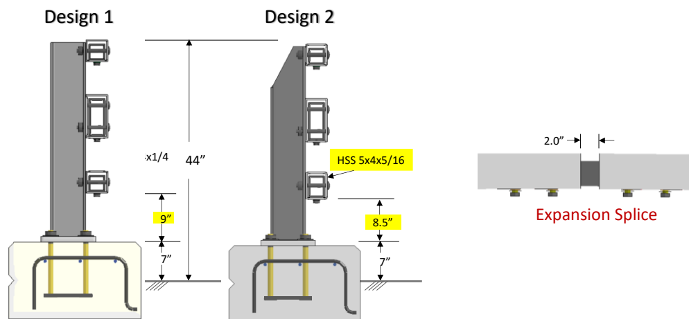
Figure 454. Bridge rail and splice designs used for the Test 4-20 evaluations.
