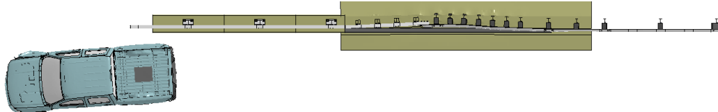
Figure O-1. [Continued] Sequential views from analysis of MASH Test 4-21 for AGT 3-Bar transition from an overhead viewpoint.
