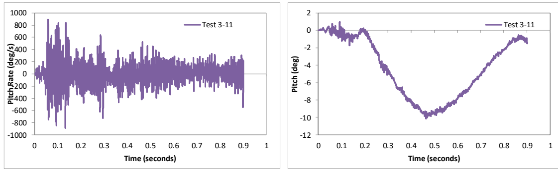
Figure 387. Pitch rate and pitch angle time-history from FEA of Test 3-11 on the NETC 2-bar bridge rail.
