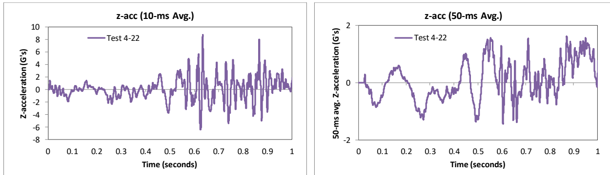
Figure 348. 10- and 50-millisecond average Z-acceleration from FEA of Test 4-22 on the MaineDOT transition (c.g. accelerometer).
