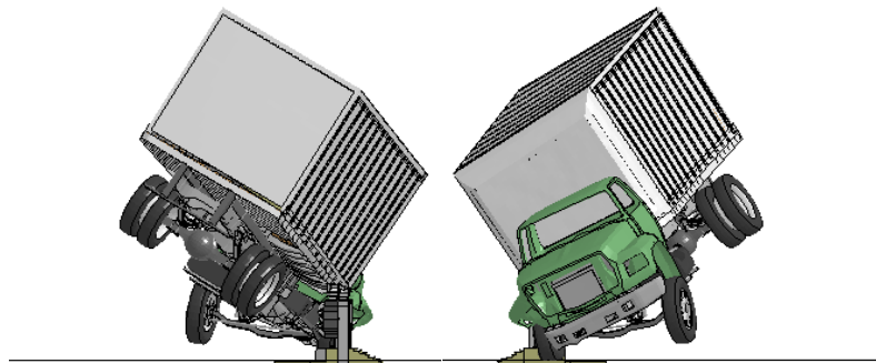
Figure P-2. [Continued] Sequential views from analysis of MASH Test 4-22 for AGT 3-Bar transition from upstream and downstream viewpoints.
