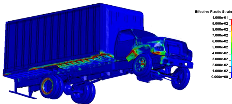
Figure 227. Damages to vehicle in Test 4-22 analysis of the 3-bar transition.
