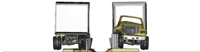
Figure V-2. [Continued] Sequential views from analysis of MASH Test 4-22 for AGT 4-Bar bridge rail from upstream and downstream viewpoints.
