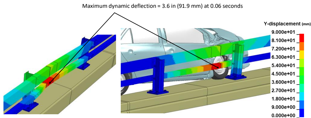
Figure 374. Contour plot of lateral displacement for the bridge rail for Test 3-10 at the time of maximum dynamic deflection.
