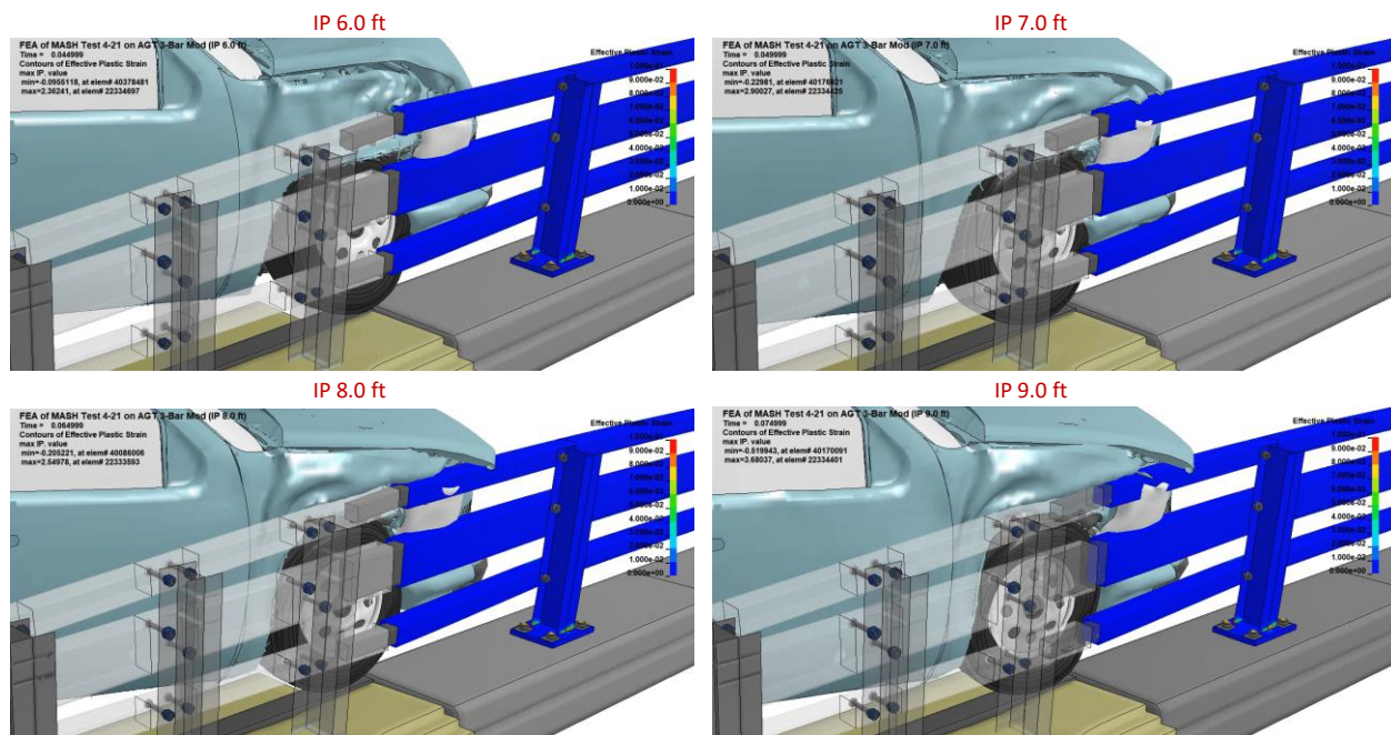
Figure 472. Test 4-21 results at time of impact with expansion splice (oblique view).
