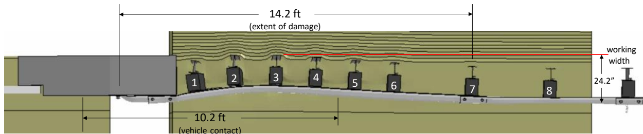
Figure 332. Overhead view of MaineDOT transition after Test 4-21 showing extent of damage.
