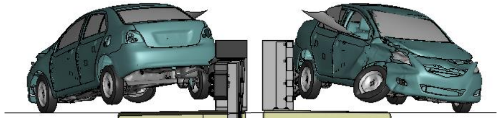
Figure T-2. [Continued] Sequential views from analysis of MASH Test 4-20 for AGT 4-Bar bridge rail from upstream and downstream viewpoints.
