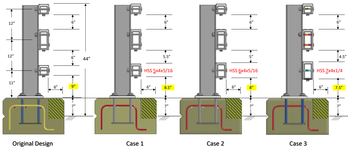
Figure 437. Analysis cases evaluated for the Modified NETC 3-bar with stiffer lower rail.
