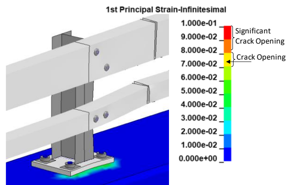
Figure 377. Contours of 1 st principal strains for concrete at the critical post for Test 3-10 on the NETC 2-bar bridge rail.
