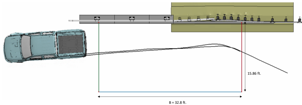
Figure 206. Exit box for Test 4-21 analysis of the 3-bar transition.
