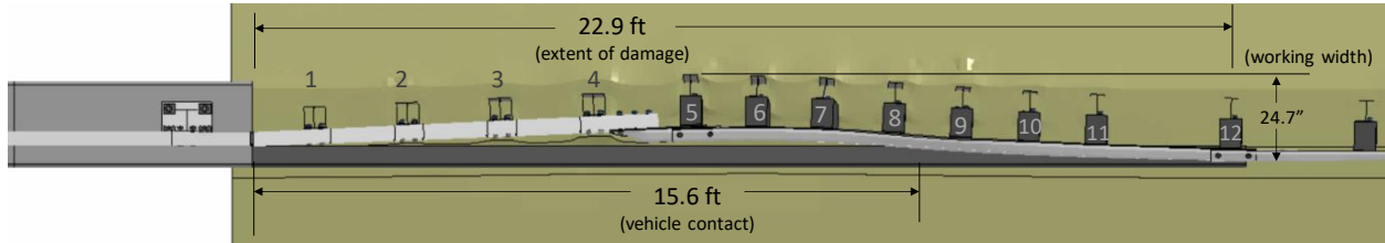
Figure 201. Overhead view of 3-bar transition after Test 4-21 showing extent of damage.
