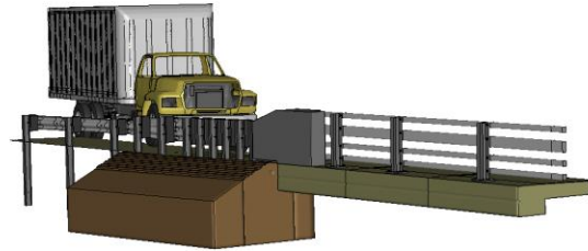
Figure V-3. Sequential views from analysis of MASH Test 4-22 for AGT 4-Bar bridge rail from an oblique viewpoint.
