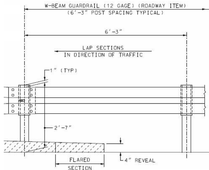
Figure 27. NHDOT T3 AGT upstream w-beam section.
