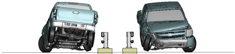
Figure X-2. [Continued] Sequential views from analysis of MASH Test 3-11 for NETC 2-Bar bridge rail from upstream and downstream viewpoints.
