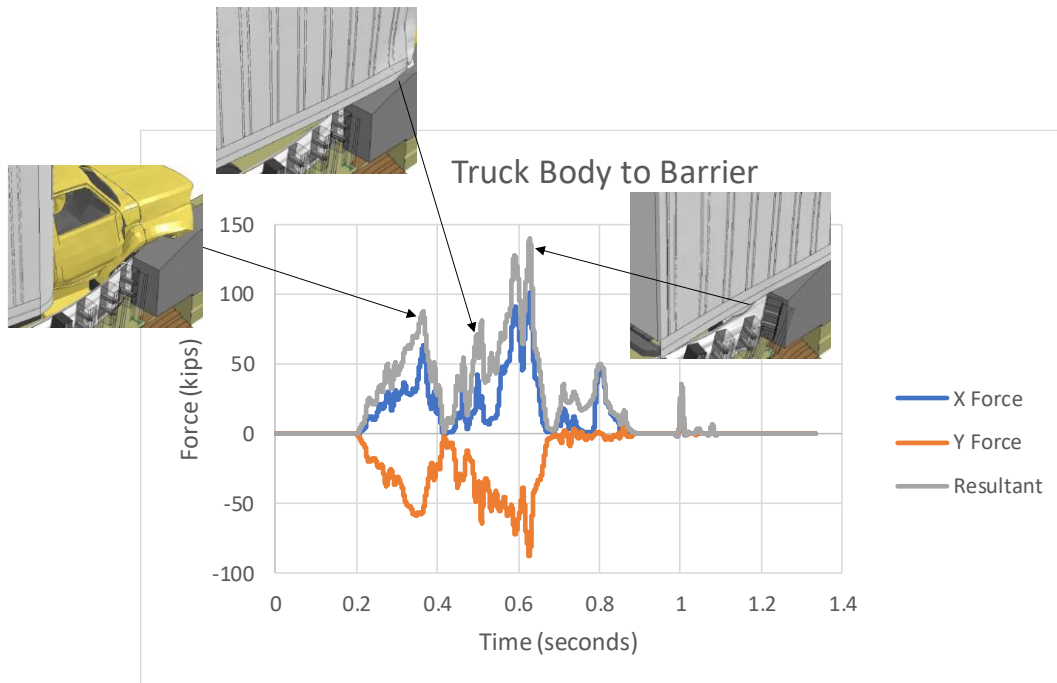
Figure 360. Longitudinal, lateral and resultant force-time history between vehicle and barrier for Test 4-22 on the MaineDOT transition.
