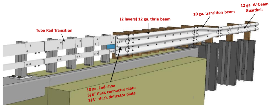
Figure 81. General model assembly for the NETC 2-bar transition (rail labeling).
