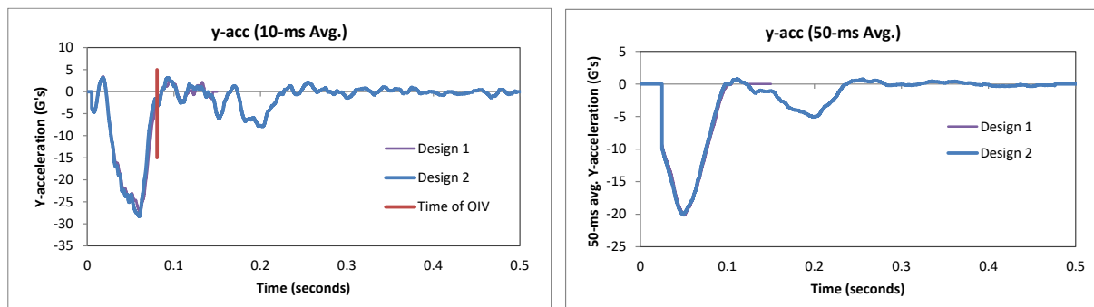
Figure 462. 10- and 50-millisecond average Y-acceleration from FEA of Test 4-20 on the 3-bar transition with 5.5-ft post spacing.
