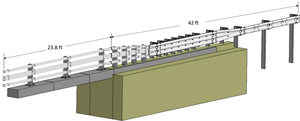
Figure 169. FEA model of the 3-bar transition (oblique viewpoint).
