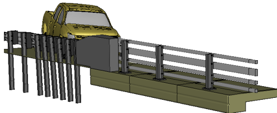
Figure U-3. Sequential views from analysis of MASH Test 4-21 for AGT 4-Bar bridge rail from an oblique viewpoint.
