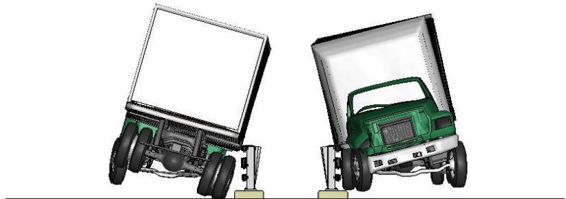
Figure M-2. [Continued] Sequential views from analysis of MASH Test 4-12 for NETC 3-Bar bridge rail from upstream and downstream viewpoints – Case 2.
