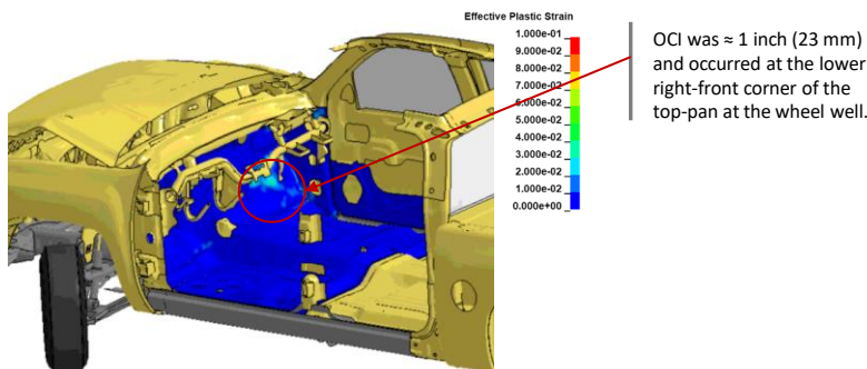
Figure 331. Occupant compartment deformation resulting from Test 4-21 on the MaineDOT transition.
