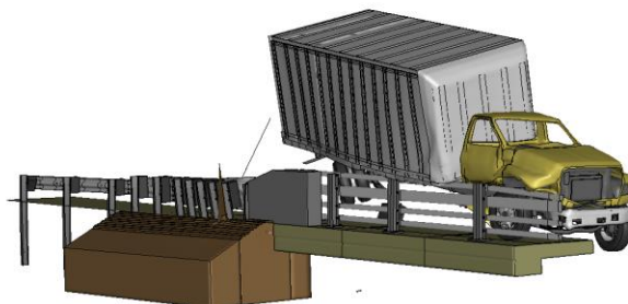
Figure V-3. [Continued] Sequential views from analysis of MASH Test 4-22 for AGT 4-Bar bridge rail from an oblique viewpoint.
