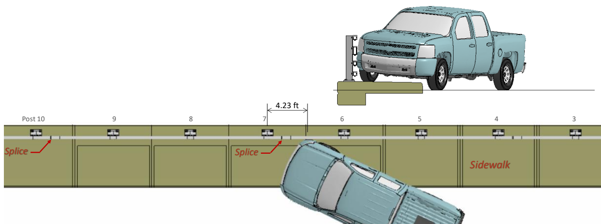
Figure 248. Actual impact point on barrier for test 4-11 on the NETC 4-bar bridge rail.
