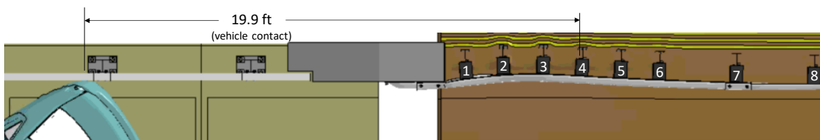
Figure 304. Overhead view of MaineDOT transition after Test 4-20 showing extent of damage.
