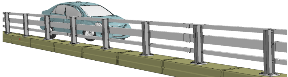
Figure J-3. [Continued] Sequential views from analysis of MASH Test 4-10 for NETC 3-Bar bridge rail from from an oblique viewpoint.
