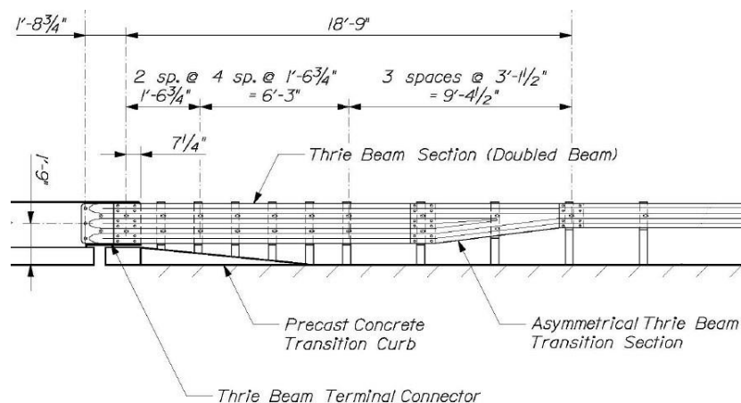
Figure 33. MaineDOT Type IA AGT double nested thrie-beam section.
