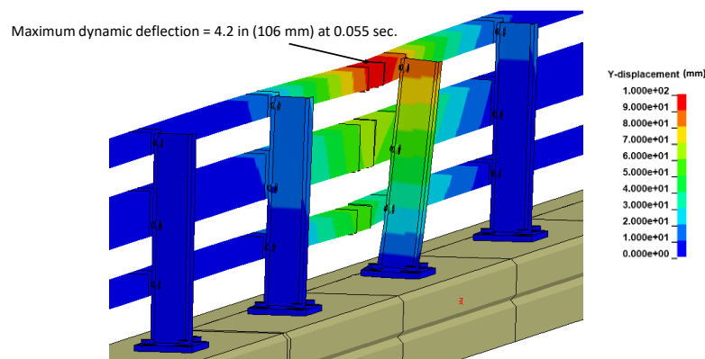
Figure 139. Contour plot of lateral displacement for the bridge rail for Test 4-11 at the time of maximum dynamic deflection.
