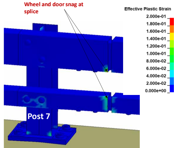
Figure 392. Contours of effective plastic strains for Test 3-11 on the NETC 2-bar bridge rail.
