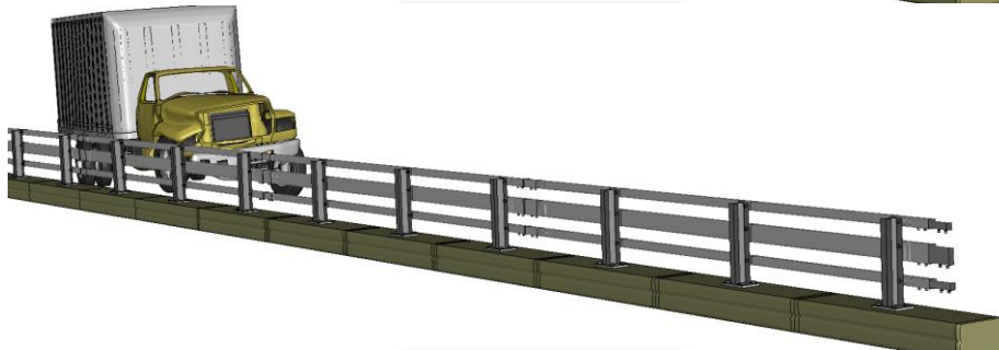
Figure K-3. Sequential views from analysis of MASH Test 4-12 for NETC 3-Bar bridge rail from an oblique viewpoint – Case 1.
