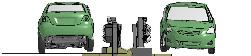
Figure N-2. [Continued] Sequential views from analysis of MASH Test 4-20 for AGT 3-Bar transition from upstream and downstream viewpoints.
