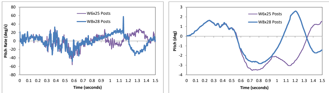
Figure 505. Pitch rate and pitch angle time-history from FEA of Test 4-12 on the baseline and modified NETC 4-bar bridge rail (c.g. accelerometer).
