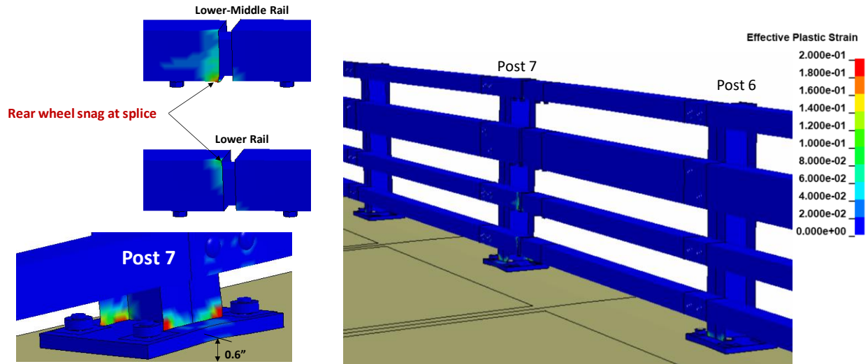
Figure 258. Contours of effective plastic strains for Test 4-11 on the NETC 4-bar bridge rail.
