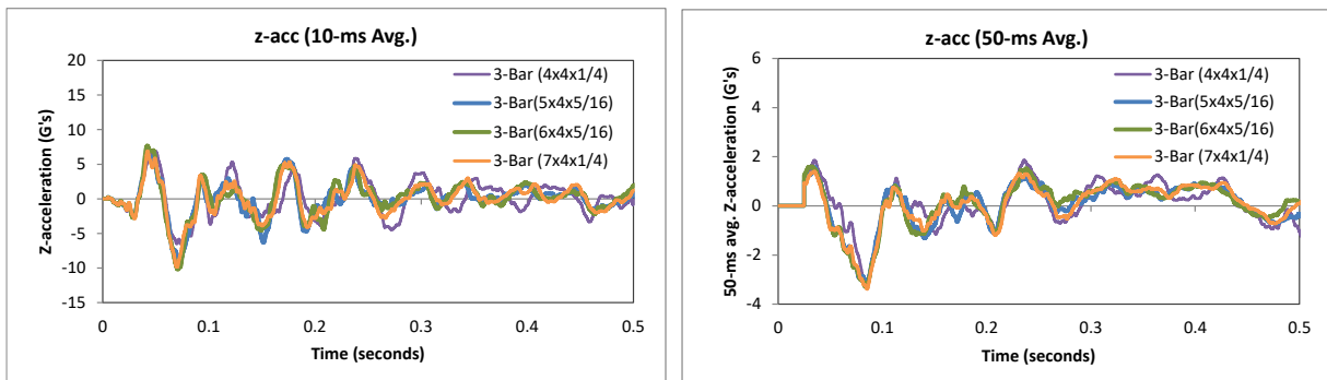
Figure 444. 10- and 50-millisecond average z-acceleration from FEA of Test 4-10 on the Modified NETC 3-bar bridge rail design cases.
