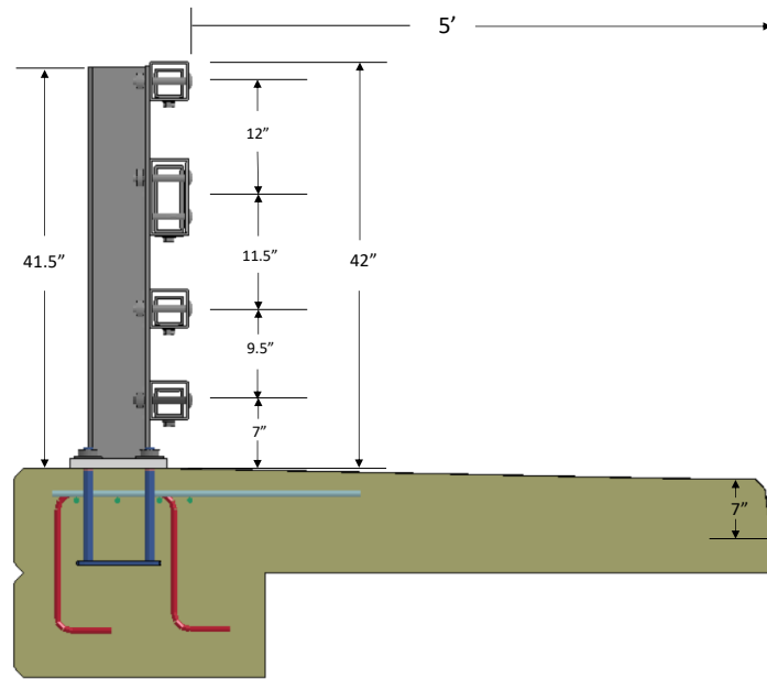
Figure 230. FEA model of sidewalk-mounted NETC 4-Bar bridge rail.
