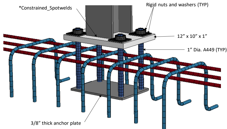
Figure 55. Transparent view of concrete showing model of baseplate and anchor bolts.
