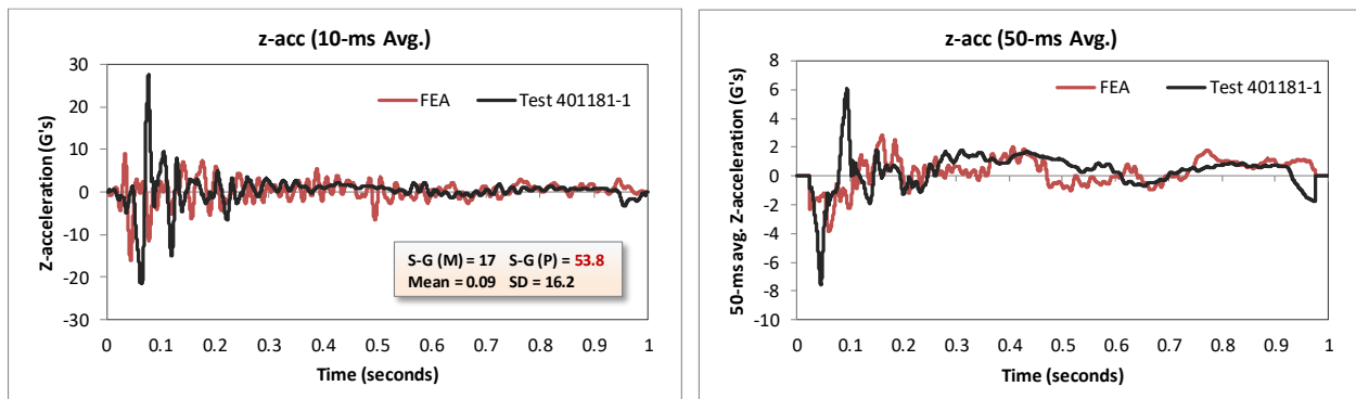
Figure 104. Vertical acceleration-time history plot from accelerometer at c.g. for full-scale Test 401181-1 and FEA (10-ms and 50-ms moving averages).
