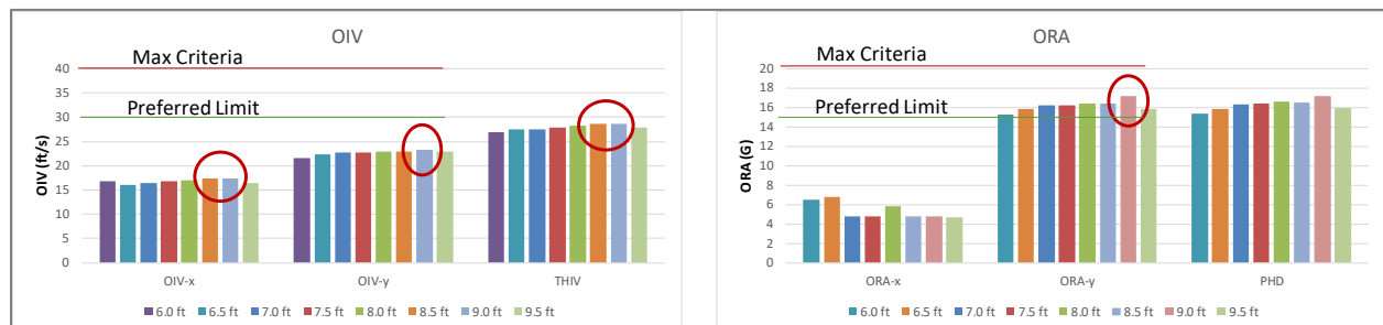
Figure 422. maximum OIV and ORA values for the Test 4-21 cases.
