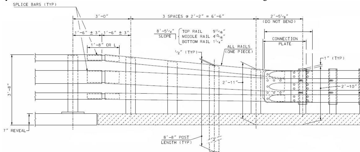
Figure 30. NHDOT T3 AGT sloped rail section.
