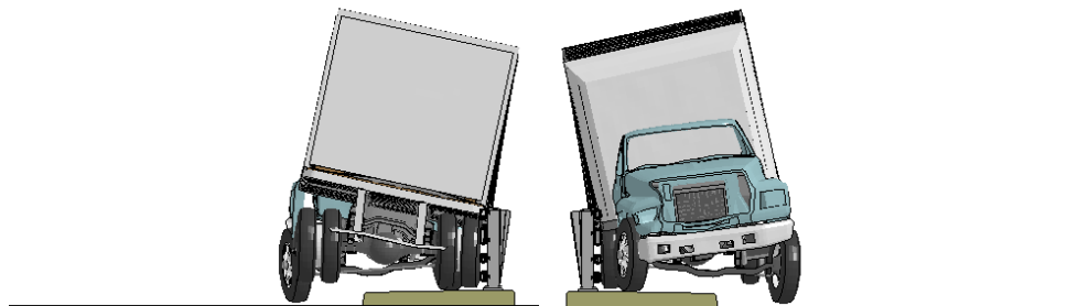
Figure S-2. [Continued] Sequential views from analysis of MASH Test 4-12 for NETC 4-Bar bridge rail from upstream and downstream viewpoints.
