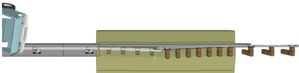
Figure 1. [Continued] Sequential views from FEA and Test 401181-1 from an overhead viewpoint.
