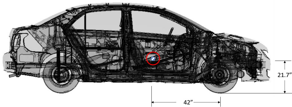
Figure 109. Location of c.g. in FEA model of 1100C vehicle.
