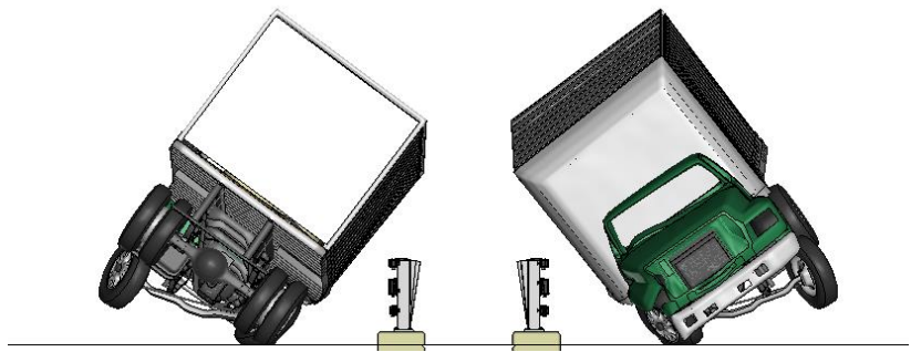
Figure M-2. [Continued] Sequential views from analysis of MASH Test 4-12 for NETC 3-Bar bridge rail from upstream and downstream viewpoints – Case 2.
