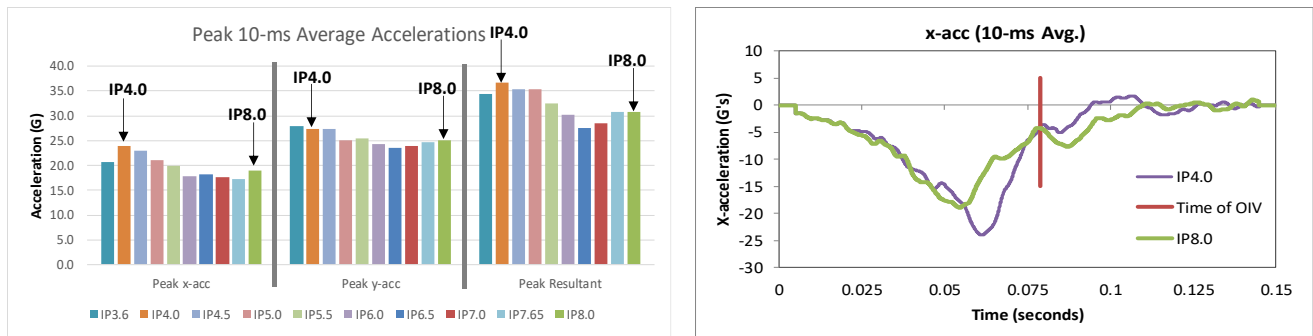
Figure 458. Peak 10-ms moving average acceleration data for Test 4-20 impact cases.
