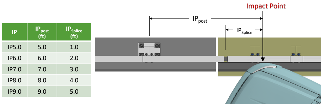
Figure 471. Impact point locations for Test 4-21 on the 3-bar transition with increased post spacing.
