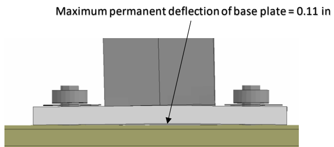
Figure 70. Deformation of baseplate for test (left) and FEA model (right).
