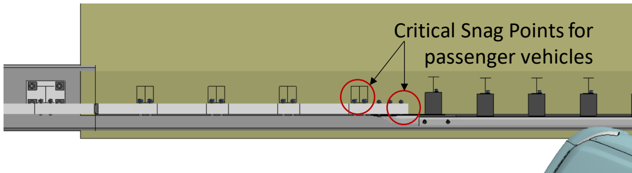
Figure 170. Illustration of potential snag points on the 3-bar transition for passenger vehicles.
