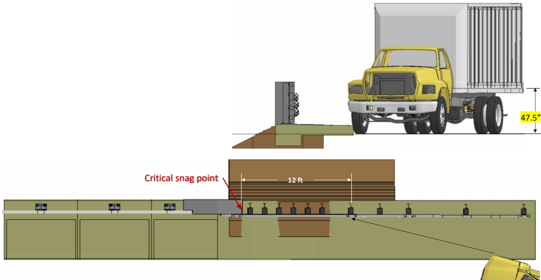
Figure 344. Initial impact point on the curb-face for Test 4-22 on the sidewalk-mounted MaineDOT transition.
