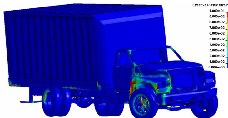
Figure 280. Damages to vehicle in Test 4-12 analysis of NETC 4-bar bridge rail.
