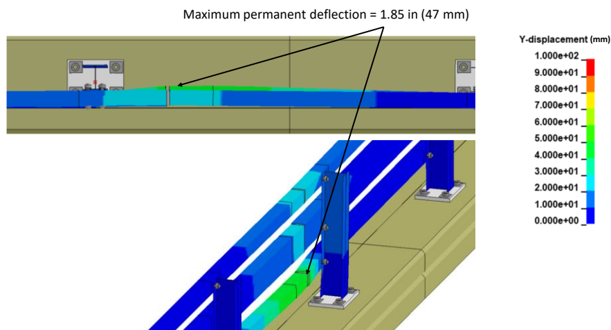
Figure 124. Contour plot of maximum permanent deflection of the bridge rail for test 4-10.
