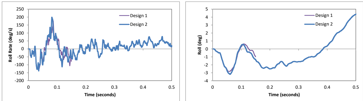
Figure 465. Roll rate and roll angle time-history from FEA of Test 4-20 on the 3-bar transition with 5.5-ft post spacing.
