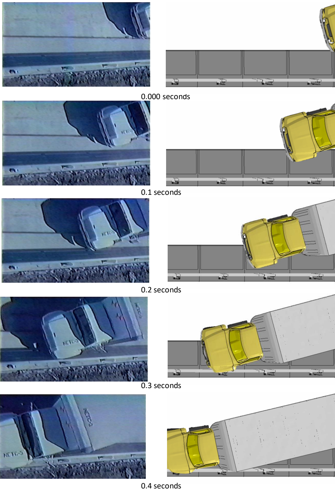
Figure 3. Sequential views of Test NETC-3 and FE analysis from overhead viewpoint.
