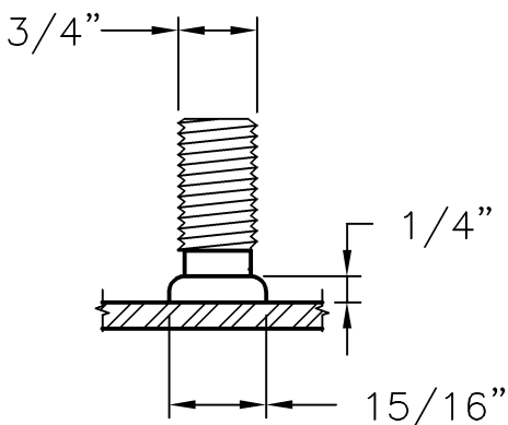
STUD WELD DETAIL NOT TO SCALE
