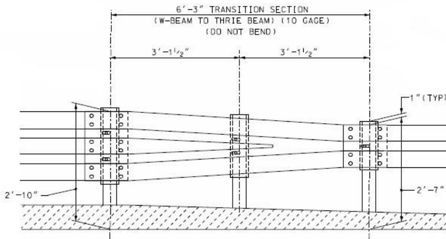
Figure 28. NHDOT T3 AGT symmetrical w-beam to thrie-beam transition section.
