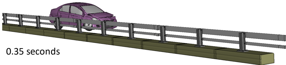
Figure W-3. [Continued] Sequential views from analysis of MASH Test 3-10 for NETC 2-Bar bridge rail from an oblique viewpoint.
