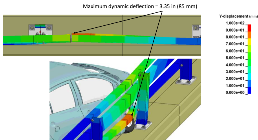
Figure 123. Contour plot of lateral displacement for the bridge rail for Test 4-10 at the time of maximum dynamic deflection.
