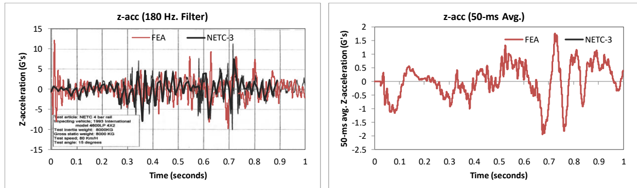
Figure 75. Vertical acceleration-time history plot from accelerometer at c.g. for full-scale Test NETC-3 and FEA (180 Hz. filter and 50-ms moving averages).
