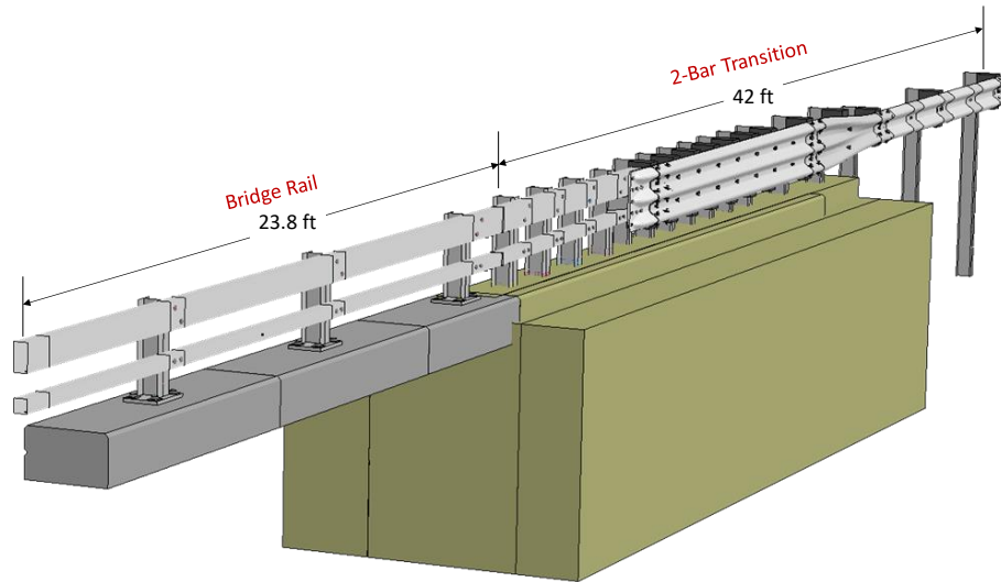
Figure 397. FEA model of the 2-bar transition (oblique viewpoint).
