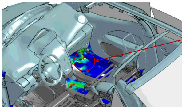
Figure 121. Occupant compartment deformation resulting from Test 4-10 on the NETC 3-bar bridge rail.
