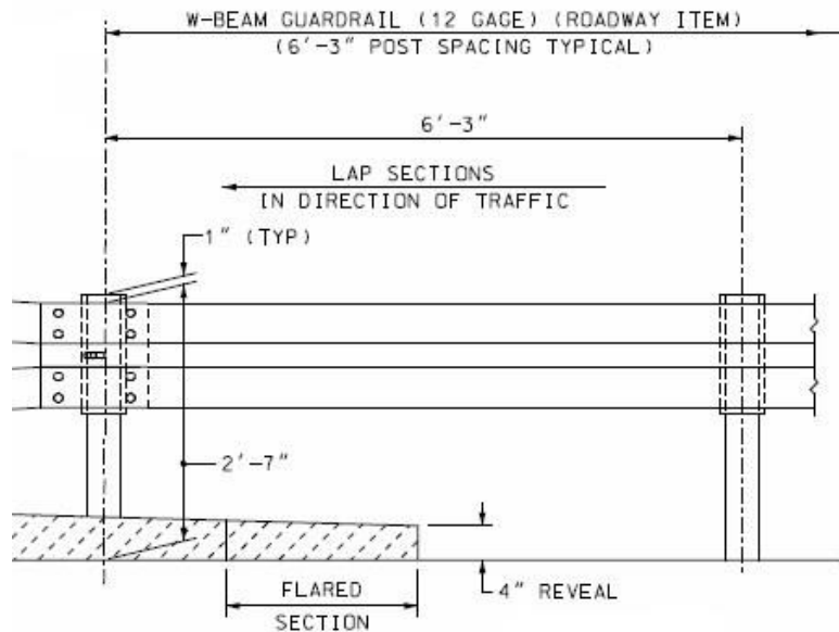
Figure 21. NHDOT T2 AGT upstream w-beam section.
