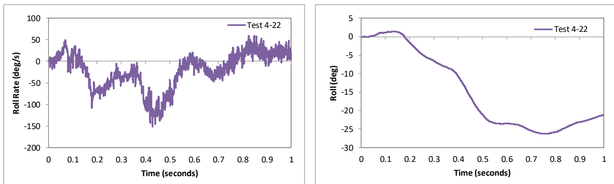
Figure 219. Roll rate and roll angle time-history from FEA of Test 4-22 on the 3-bar transition (cabin accelerometer).
