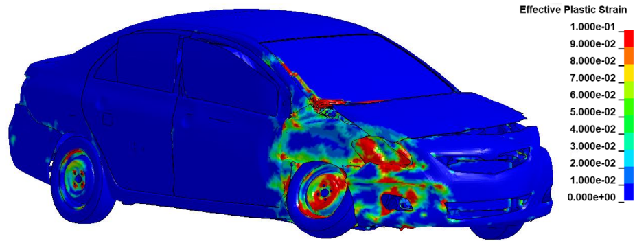
Figure 378. Damages to vehicle in Test 3-10 analysis of the NETC 2-bar bridge rail.
