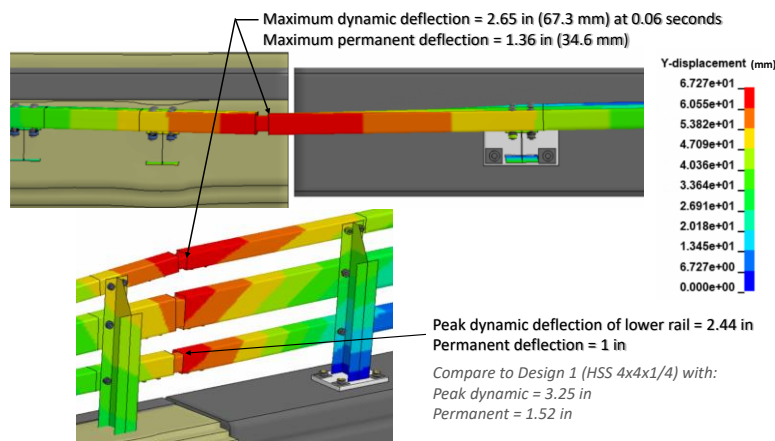
Figure 467. Contour plot of lateral displacement for the system at the time of maximum dynamic deflection.
