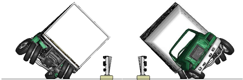
Figure M-2. [Continued] Sequential views from analysis of MASH Test 4-12 for NETC 3-Bar bridge rail from upstream and downstream viewpoints – Case 2.
