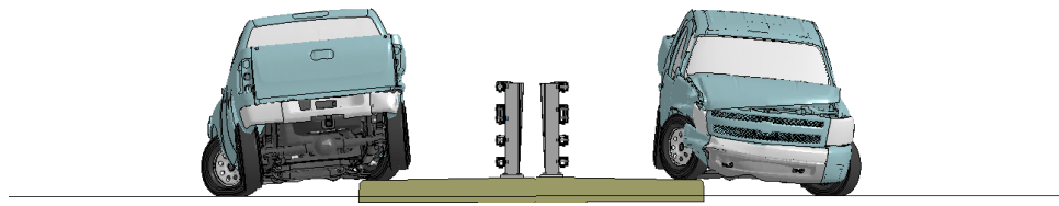
Figure R-2. [Continued] Sequential views from analysis of MASH Test 4-11 for NETC 4-Bar bridge rail from upstream and downstream viewpoints.
