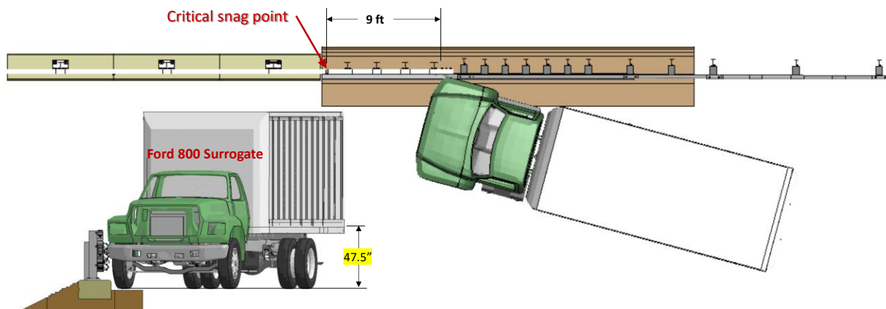
Figure 478. Critical impact point and 10000S vehicle selected for the Test 4-22 simulations.
