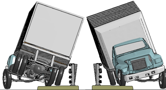
Figure S-2. [Continued] Sequential views from analysis of MASH Test 4-12 for NETC 4-Bar bridge rail from upstream and downstream viewpoints.
