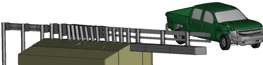
Figure Z-3. [Continued] Sequential views from analysis of MASH Test 3-21 for AGT 2-Bar bridge rail from an oblique viewpoint.
