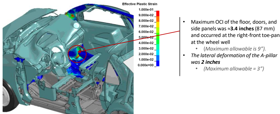
Figure 303. Occupant compartment deformation resulting from Test 4-20 on the MaineDOT transition.
