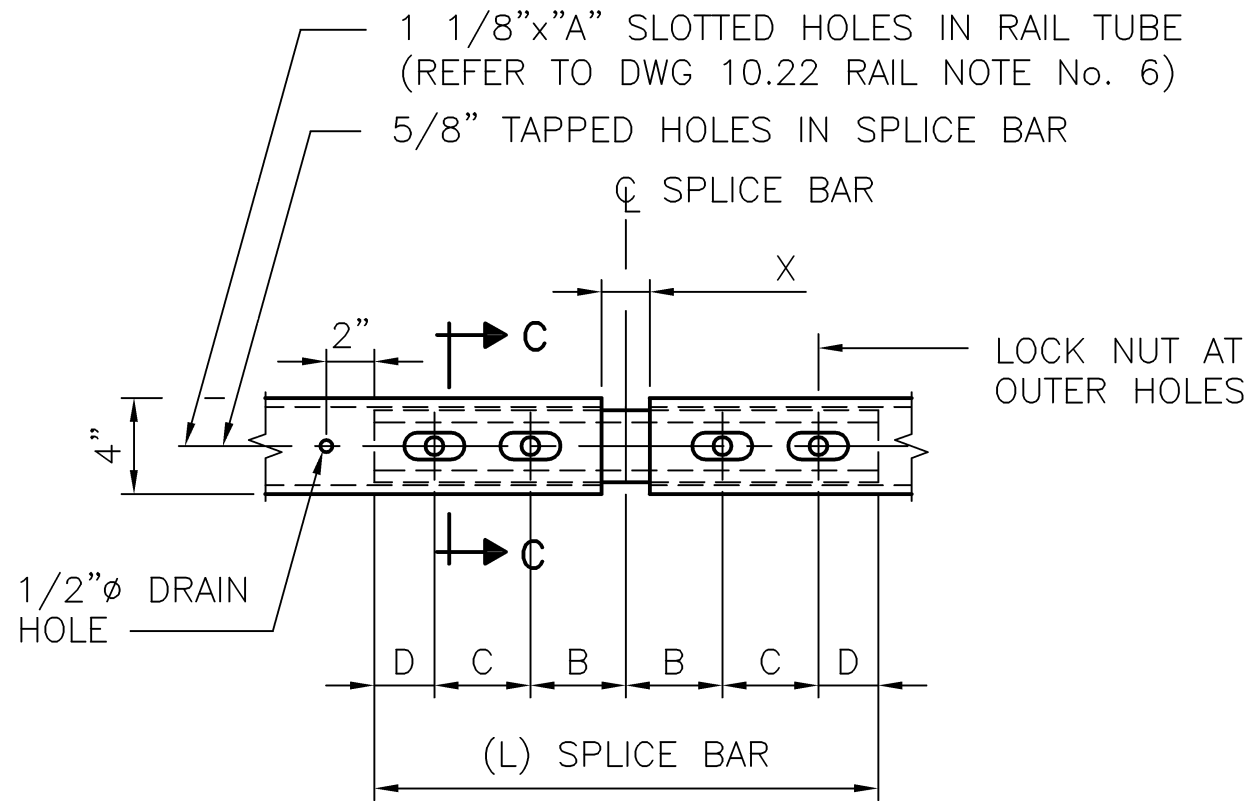
SEE SPLICE BAR DIMENSION TABLE THIS SHEET (BOTTOM VIEW) RAIL SPLICE SCALE: 1 1/2"=1'-0"
