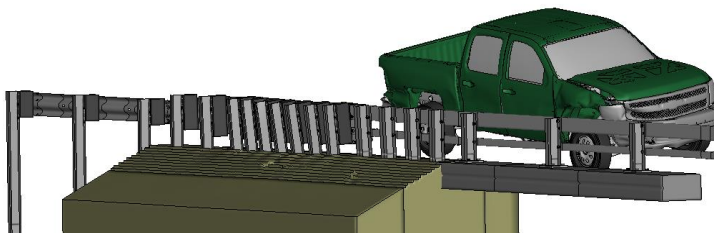
Figure Z-3. [Continued] Sequential views from analysis of MASH Test 3-21 for AGT 2-Bar bridge rail from an oblique viewpoint.
