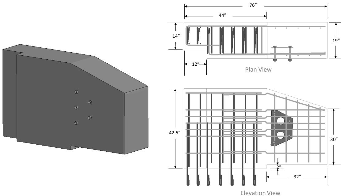
Figure 289. FEA model of transition buttress with dimensions and steel reinforcement details.
