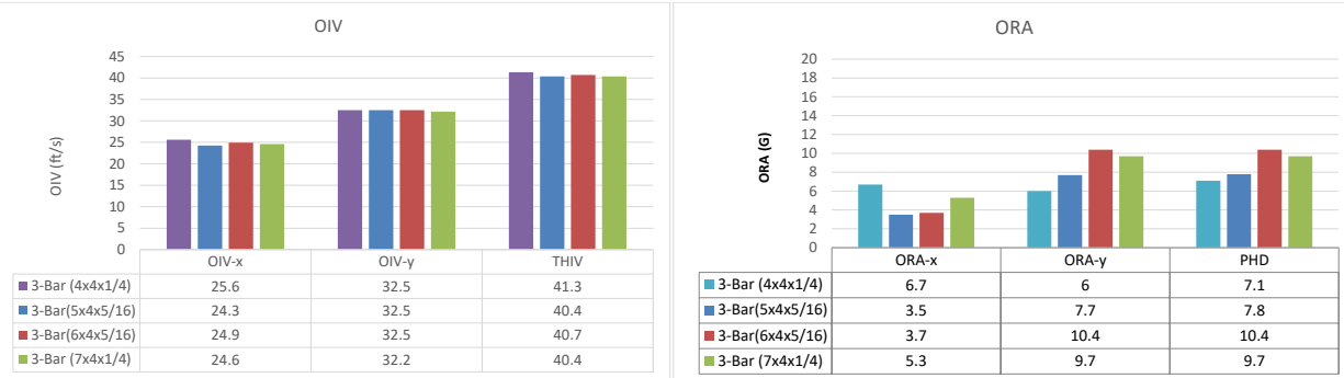
Figure 448. OI32.5V and ORA values for Test 4-10 on the Modified NETC 3-bar design case.
