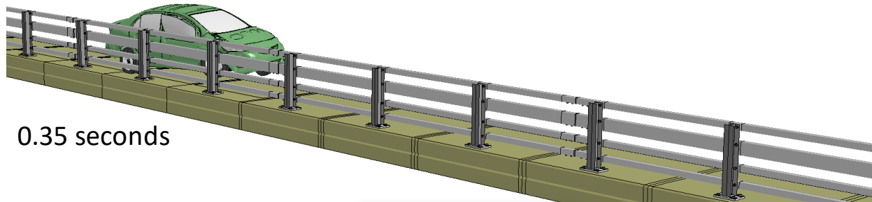
Figure Q-3. [Continued] Sequential views from analysis of MASH Test 4-10 for NETC 4-Bar bridge rail from from an oblique viewpoint.
