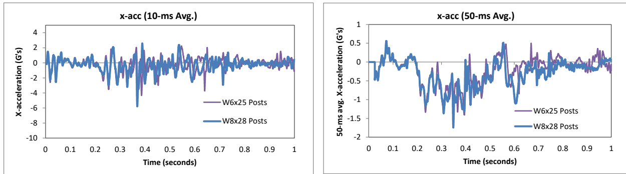
Figure 500. 10- and 50-millisecond average X-acceleration from FEA of Test 4-12 on the baseline and modified NETC 4-bar bridge rail (c.g. accelerometer).
