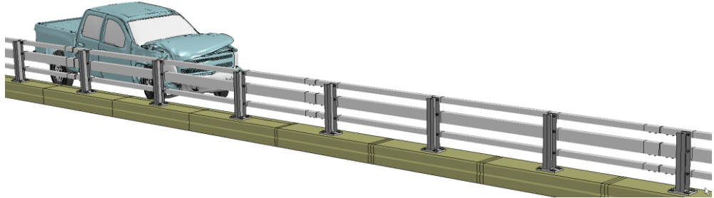
Figure K-3. Sequential views from analysis of MASH Test 4-11 for NETC 3-Bar bridge rail from an oblique viewpoint.
