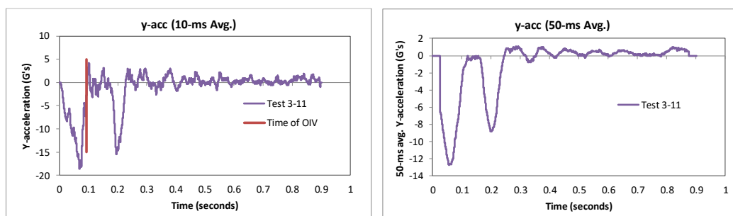
Figure 383. 10- and 50-millisecond average Y-acceleration from FEA of Test 3-11 on the NETC 2-bar bridge rail.
