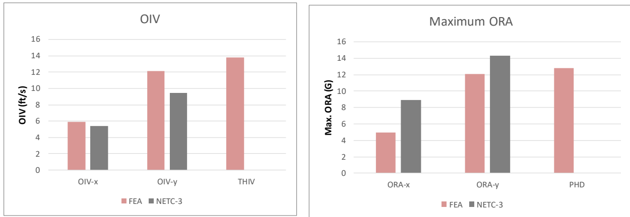
Figure 72. Graphical comparison of FEA vs. Test for key occupant risk metrics
