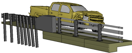
Figure U-3. [Continued] Sequential views from analysis of MASH Test 4-21 for AGT 4-Bar bridge rail from an oblique viewpoint.
