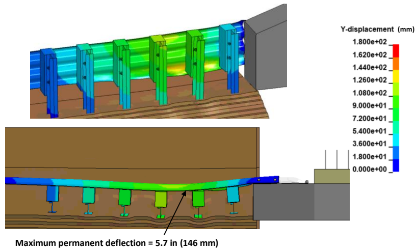
Figure 307. Contour plot of maximum permanent deflection for the MaineDOT transition.
