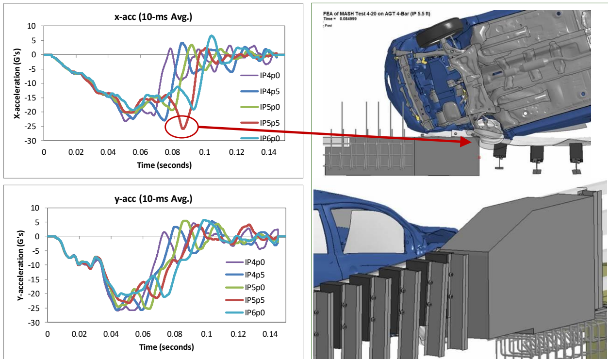
Figure 294. Acceleration data collected at the c.g. of the vehicle for each case.
