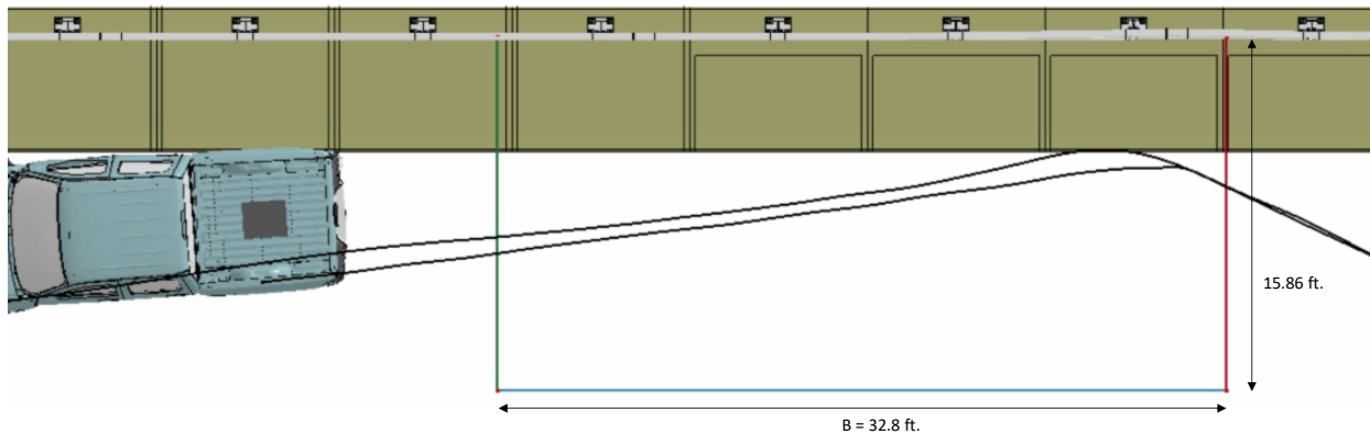
Figure 261. Exit box for Test 4-11 analysis of the NETC 4-bar bridge rail.
