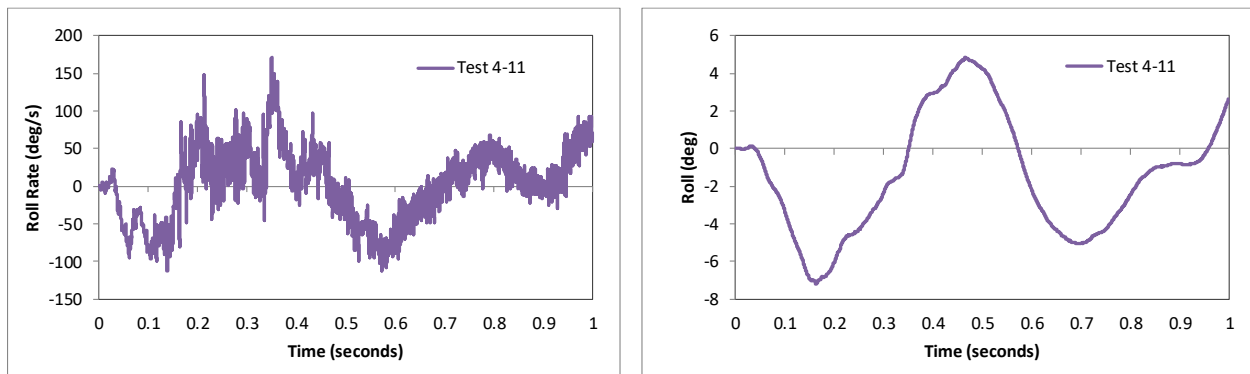
Figure 253. Roll rate and roll angle time-history from FEA of Test 4-11 on the NETC 4-bar bridge rail.
