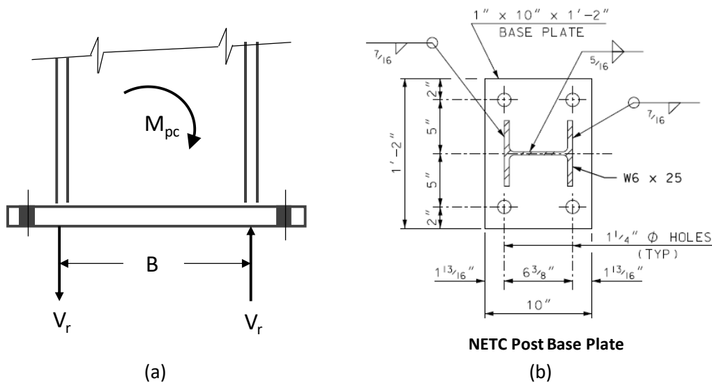
Figure 18. (a) Assumed load/reaction points for the punching shear resistance calculations and (b) dimensions of the NETC baseplate.
