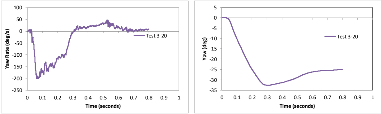
Figure 406. Yaw rate and yaw angle time-history from FEA of Test 3-20 on the 2-bar transition.
