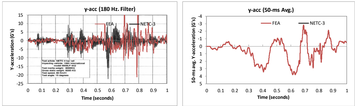
Figure 74. Lateral acceleration-time history plot from accelerometer at c.g. for full-scale Test NETC-3 and FEA (180 Hz. filter and 50-ms moving averages).
