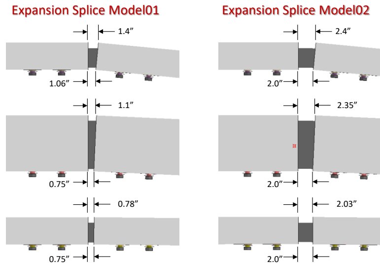
Figure 451. Expansion splice cases evaluated.
