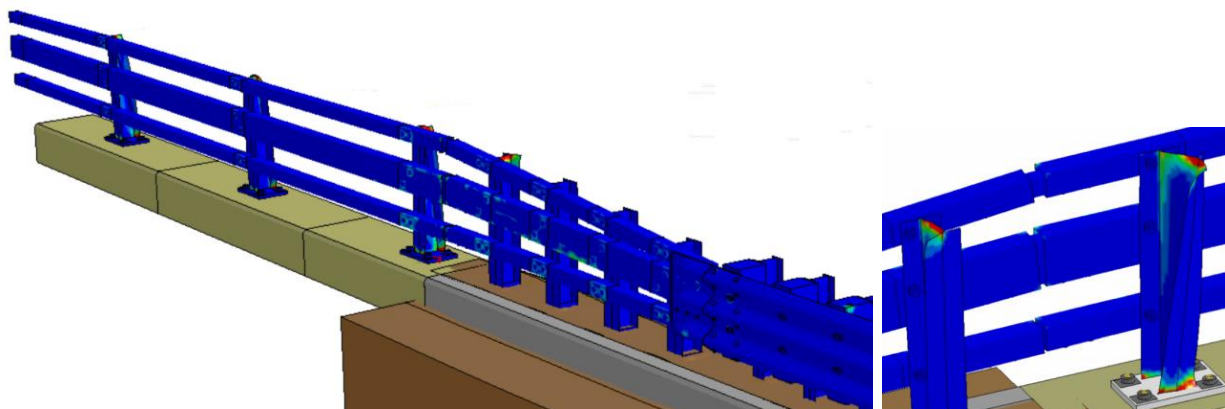
Figure 224. Contours of effective plastic strains on the transition and bridge rail for Test 4-22 on the 3-bar transition.
