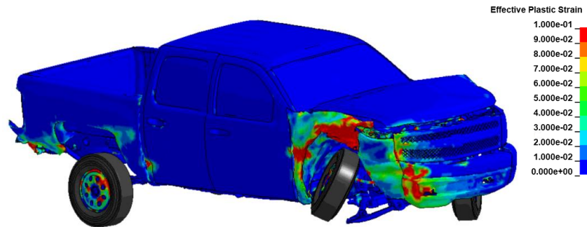
Figure 337. Damages to vehicle in Test 4-21 analysis of the MaineDOT transition.
