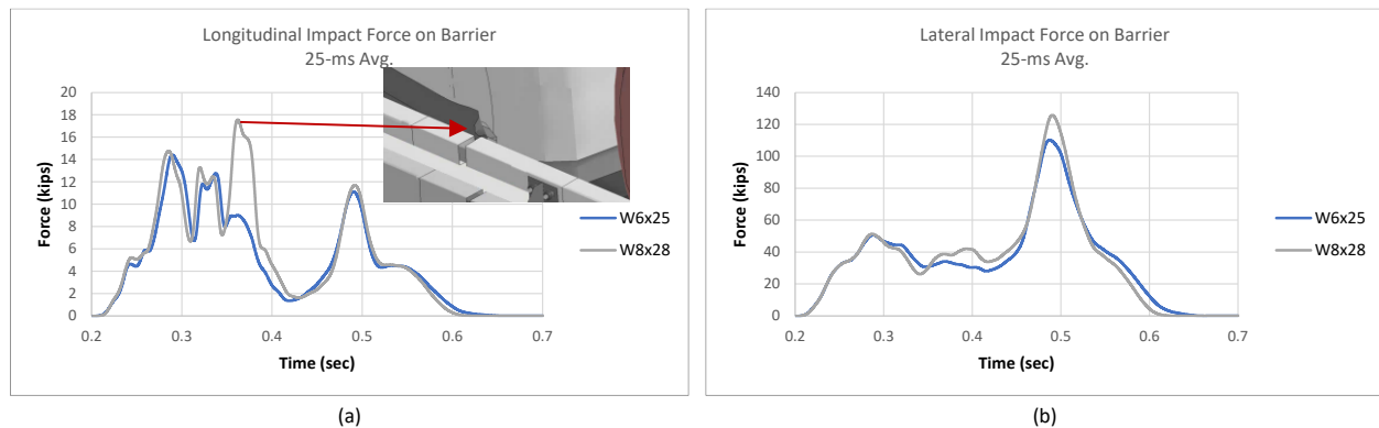
Figure 506. (a) longitudinal and (b) lateral impact force-time history for the baseline and modified design cases.
