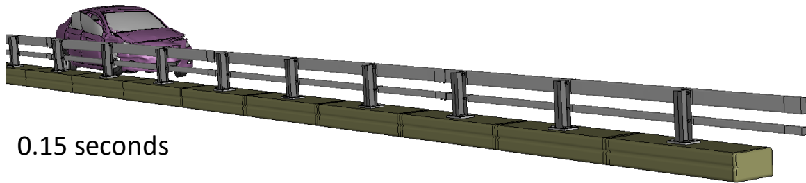
Figure W-3. Sequential views from analysis of MASH Test 3-10 for NETC 2-Bar bridge rail from an oblique viewpoint.
