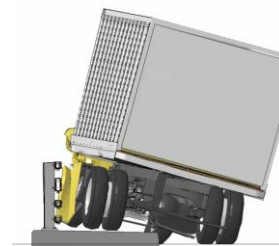
Figure 1. [Continued] Sequential views from FEA and Test NETC-3 from an upstream viewpoint.
