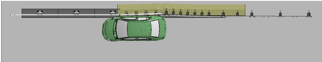
Figure N-1. Sequential views from analysis of MASH Test 4-20 for AGT 3-Bar transition from an overhead viewpoint.
