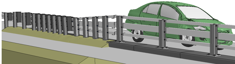
Figure N-3. [Continued] Sequential views from analysis of MASH Test 4-20 for AGT 3-Bar transition from an oblique viewpoint.
