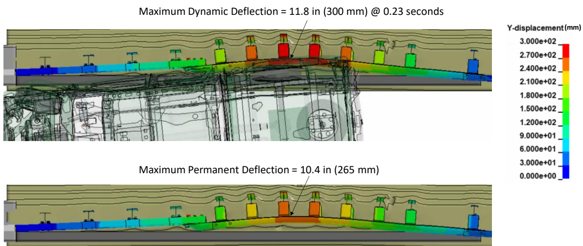
Figure 432. Contour plot of lateral displacement for Test 3-21 on the 3-bar transition at the time of maximum dynamic deflection and maximum permanent deflection.
