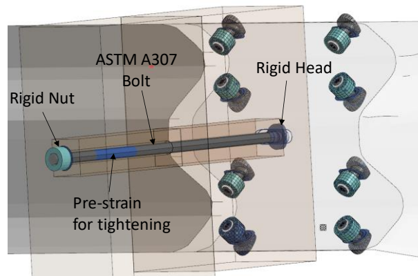
Figure 89. FEA model of the post bolt (typ) with the blockout, post, and rail displayed in transparency mode to facilitate viewing.
