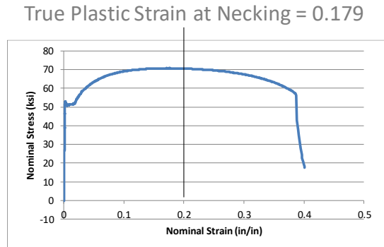
Figure 160. Plot of material stress-strain curve for Post with necking strain identified.
