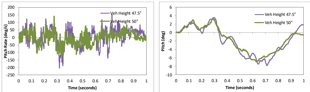
Figure 155. Pitch rate and pitch angle time-history from FEA of Test 4-12 on the NETC 3-bar bridge rail (cabin accelerometer).
