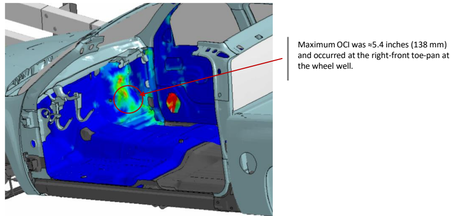
Figure 388. Occupant compartment deformation resulting from Test 3-11 on the NETC 2-bar bridge rail.
