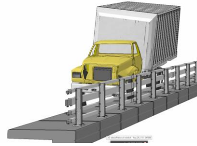
Figure 65. Sequential views of Test NETC-3 and FE analysis from downstream viewpoint.
