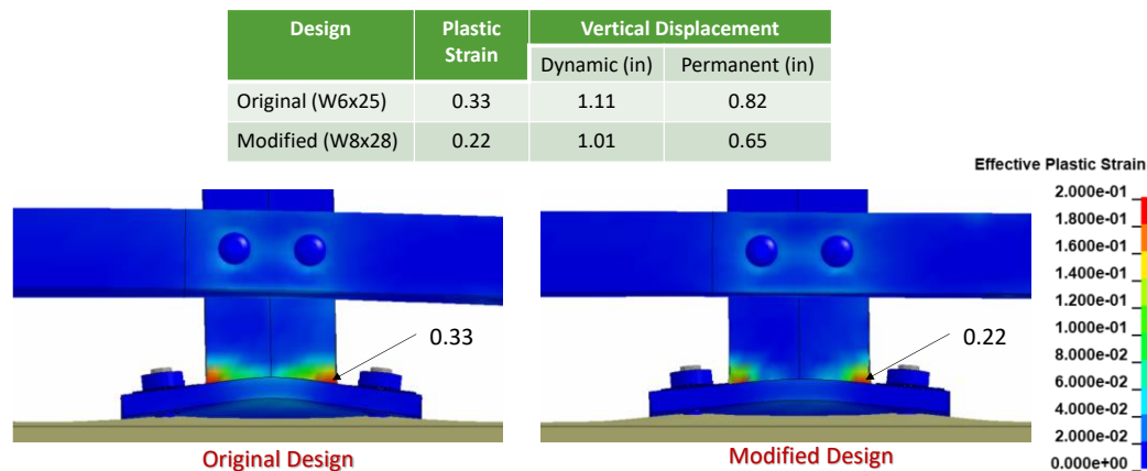
Figure 508. Contours of effective plastic strain on the bridge rail posts and baseplates for the original and modified design cases.
