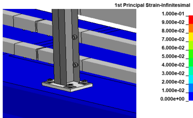
Figure 243. Contours of 1 st principal strains for concrete at the critical post for Test 4-10 on the NETC 4-bar bridge rail.
