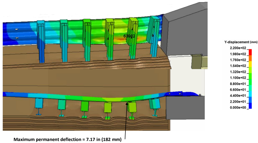
Figure 335. Contour plot of maximum permanent deflection for Test 4-21 on the MaineDOT transition.
