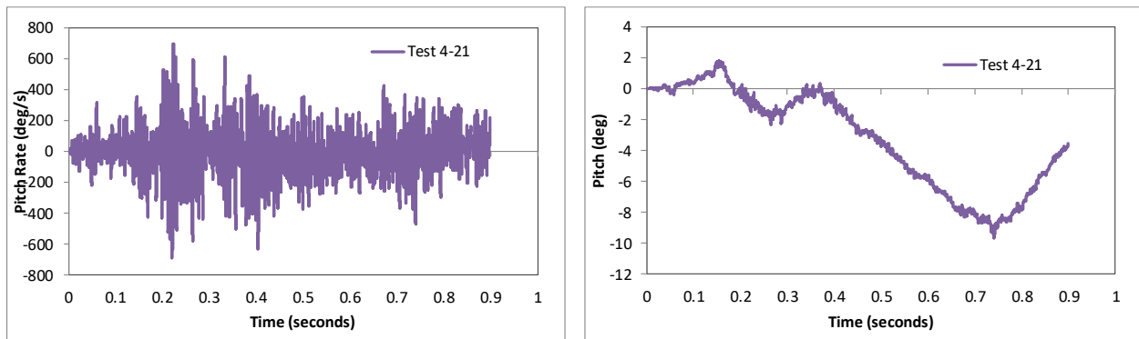
Figure 330. Pitch rate and yaw angle time-history from FEA of Test 4-21 on the MaineDOT transition.
