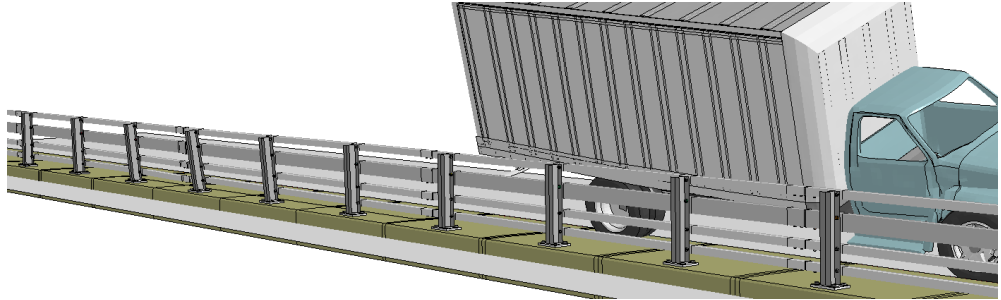
Figure S-3. [Continued] Sequential views from analysis of MASH Test 4-12 for NETC 4-Bar bridge rail from an oblique viewpoint.
