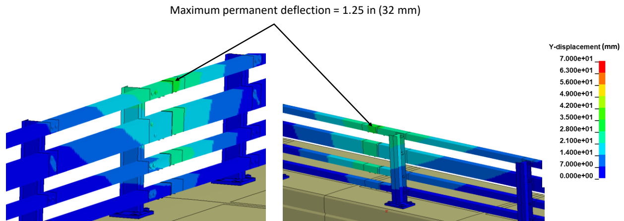
Figure 241. Contour plot of maximum permanent deflection of the bridge rail for Test 4-10.
