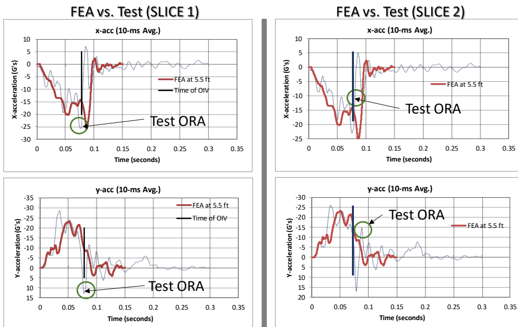
Figure 315. Overlay of acceleration-time histories for FEA and tests.
