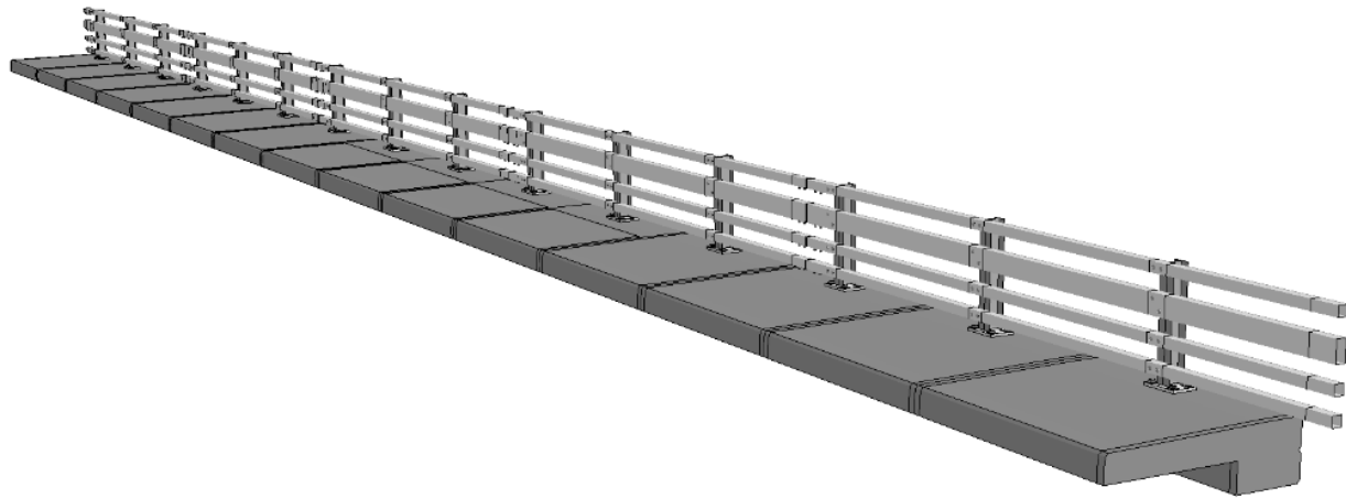
Figure 49. Finite element analysis model of the NETC 4-bar bridge rail (isometric view).
