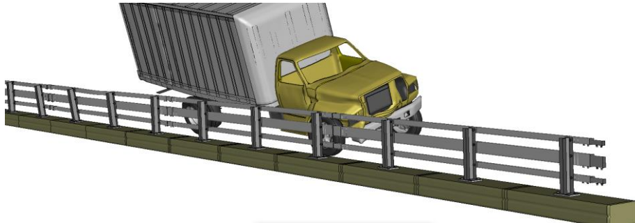
Figure K-3. [Continued] Sequential views from analysis of MASH Test 4-12 for NETC 3-Bar bridge rail from an oblique viewpoint – Case 1.
