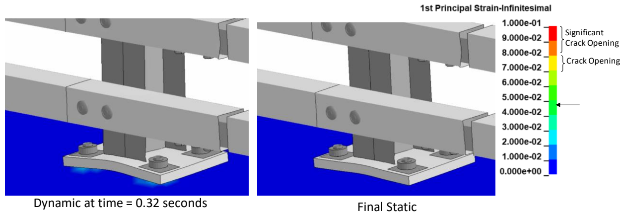
Figure 259. Contours of 1 st principal strains for concrete at the critical post for Test 4-11 on the NETC 4-bar bridge rail.
