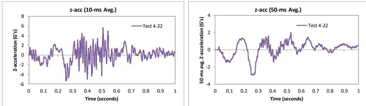
Figure 214. 10- and 50-millisecond average Z-acceleration from FEA of Test 4-22 on the 3-bar transition (c.g. accelerometer).
