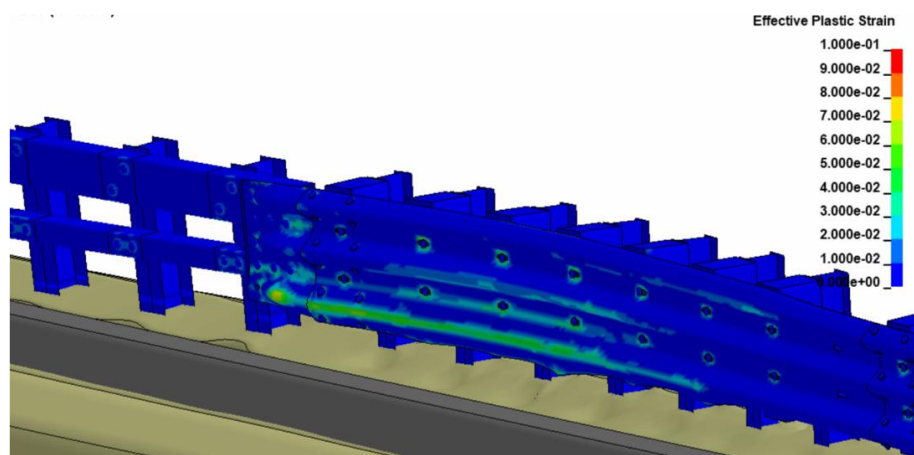
Figure 433. Contours of effective plastic strains on the steel rails and posts for Test 3-21 on 2-bar transition.
