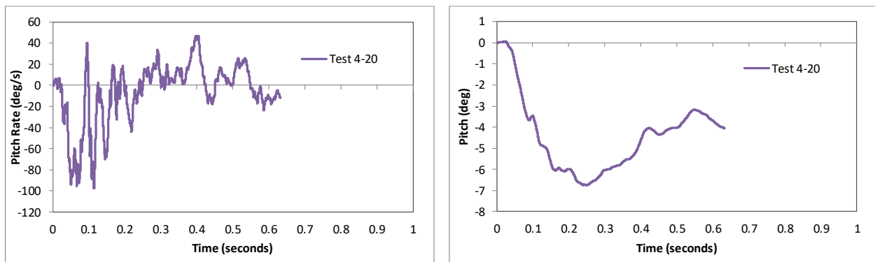
Figure 302. Pitch rate and pitch angle time-history from FEA of Test 4-20 on the MaineDOT transition.
