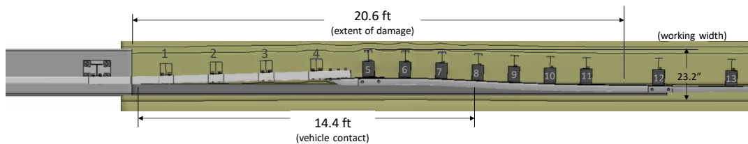
Figure 410. Overhead view of 2-bar transition after Test 3-20 showing extent of damage.
