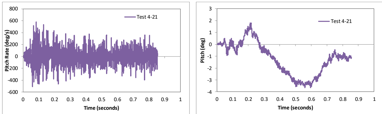
Figure 199. Pitch rate and pitch angle time-history from FEA of Test 4-21 on the 3-bar transition.
