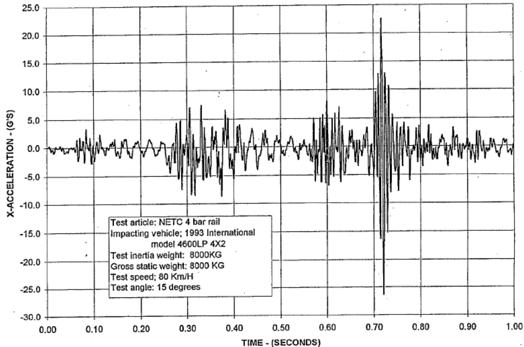
Figure 59. Longitudinal (x-direction) acceleration measured at vehicle c.g. in Test NETC-3. [Kimball99]
