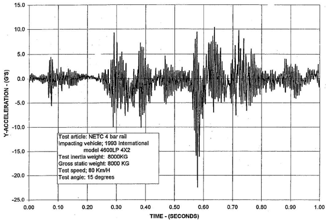
Figure 60. Lateral (y-direction) acceleration measured at vehicle c.g. in Test NETC-3. [Kimball99]
