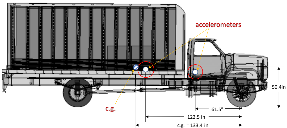
Figure 111. Location of accelerometers and c.g. in FEA model of 10000S vehicle.
