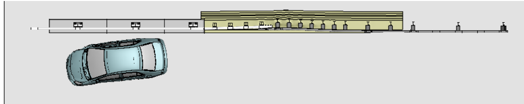
Figure Y-1. [Continued] Sequential views from analysis of MASH Test 3-20 for AGT 2-Bar bridge rail from an overhead viewpoint.
