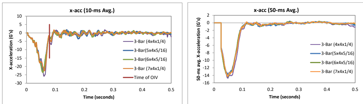
Figure 442. 10- and 50-millisecond average x-acceleration from FEA of Test 4-10 on the Modified NETC 3-bar bridge rail.
