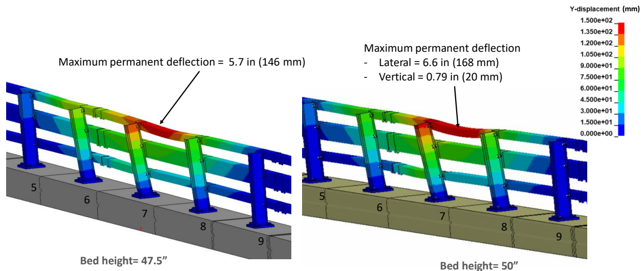
Figure 158. Contour plot of permanent deflection for the bridge rail from Test 4-12 for the NETC 3-bar bridge rail.
