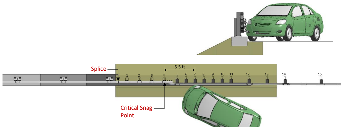
Figure 173. Impact point for Test 4-20 on the 3-bar transition.
