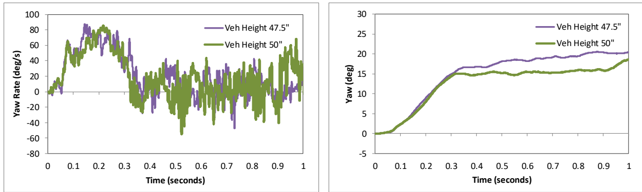
Figure 153. Yaw rate and yaw angle time-history from FEA of Test 4-12 on the NETC 3-bar bridge rail (cabin accelerometer).
