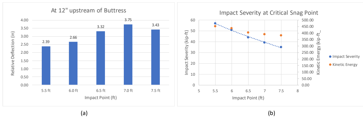
Figure 318. (a) Relative displacements of rail and (b) impact severity and kinetic energy at time of impact with buttress for Test 4-21 CIP evaluations.
