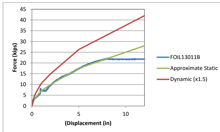
Figure 292. Measured and approximated force-deflection response for the end-anchor.
