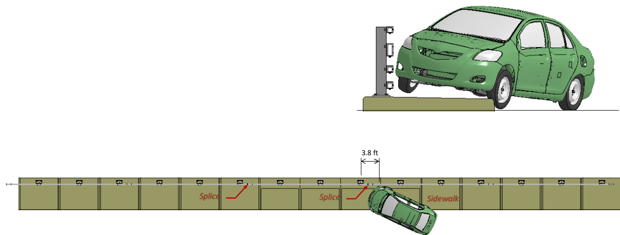
Figure 232. Actual impact point on barrier for test 4-10 on the NETC 4-bar bridge rail.
