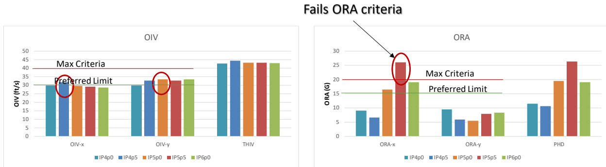
Figure 295. Plots of OIV and maximum ORA for each case.
