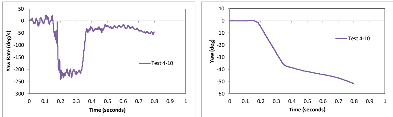
Figure 236. Yaw rate and yaw angle time-history from FEA of Test 4-10 on the NETC 4-bar bridge rail.
