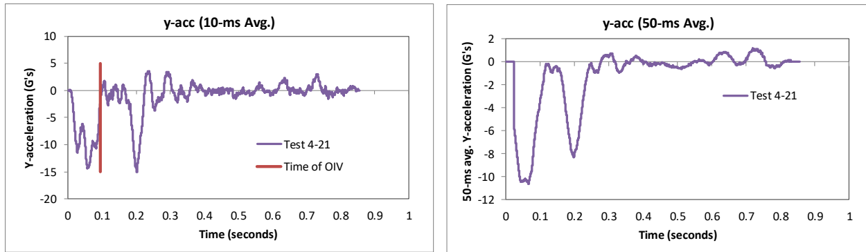
Figure 195. 10- and 50-millisecond average Y-acceleration from FEA of Test 4-21 on the 3-bar transition.
