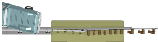
Figure 1. [Continued] Sequential views from FEA and Test 401181-1 from an overhead viewpoint.
