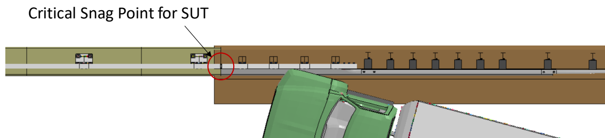
Figure 171. Illustration of potential snag point on the 3-bar transition for the single unit truck.
