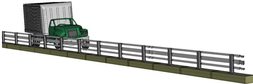
Figure M-3. Sequential views from analysis of MASH Test 4-12 for NETC 3-Bar bridge rail from an oblique viewpoint – Case 2.
