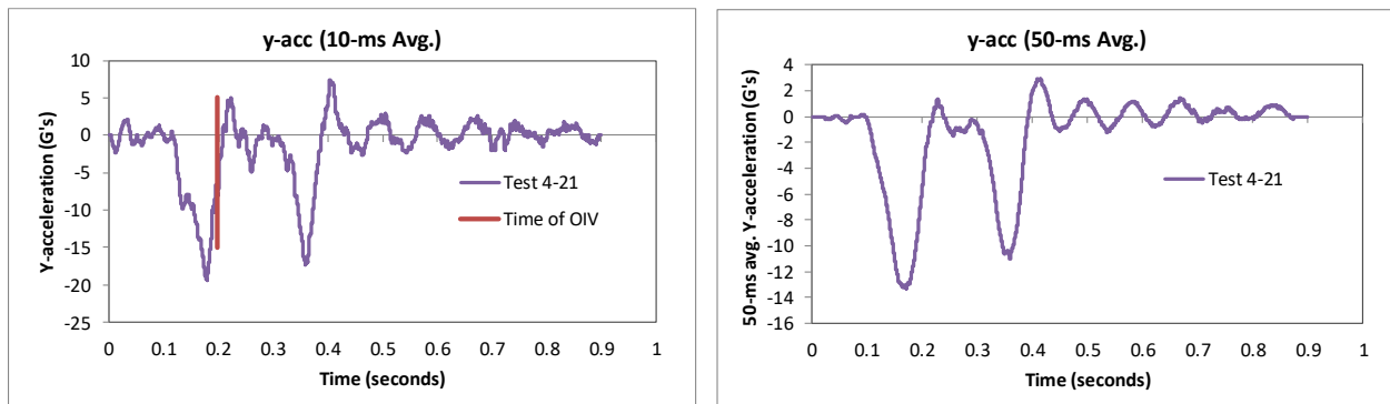
Figure 326. 10- and 50-millisecond average Y-acceleration from FEA of Test 4-21 on the MaineDOT transition.
