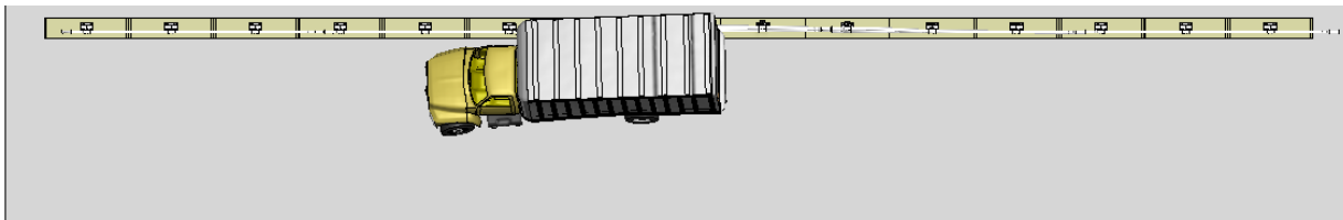
Figure L-1. [Continued] Sequential views from analysis of MASH Test 4-12 for NETC 3-Bar bridge rail from an overhead viewpoint – Case 1.
