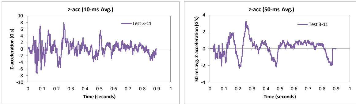
Figure 384. 10- and 50-millisecond average Z-acceleration from FEA of Test 3-11 on the NETC 2-bar bridge rail.
