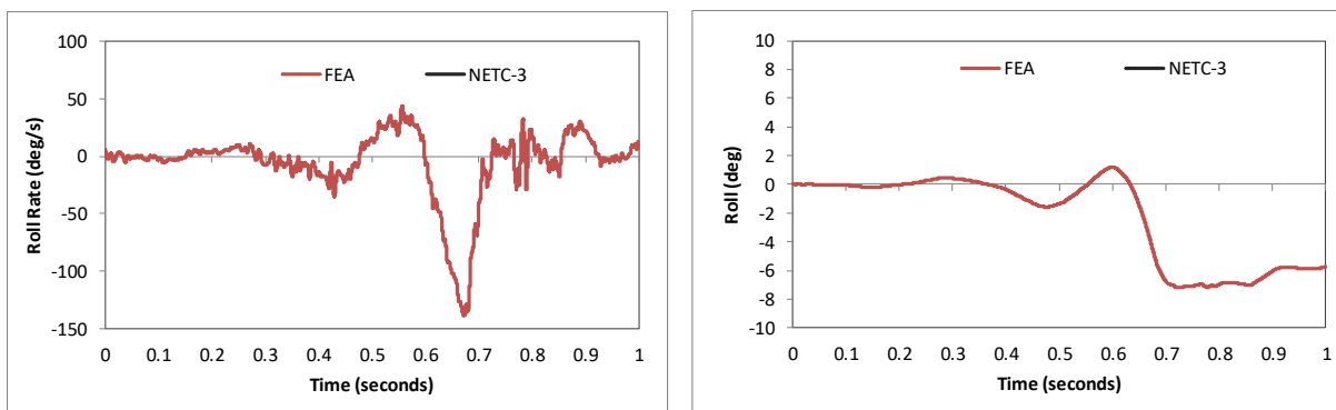
Figure 77. Roll-time history plot from accelerometer at c.g. for FEA (angular rate and displacement).
