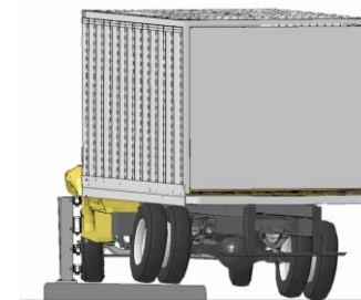
Figure 1. Sequential views from FEA and Test NETC-3 from a upstream view point.
