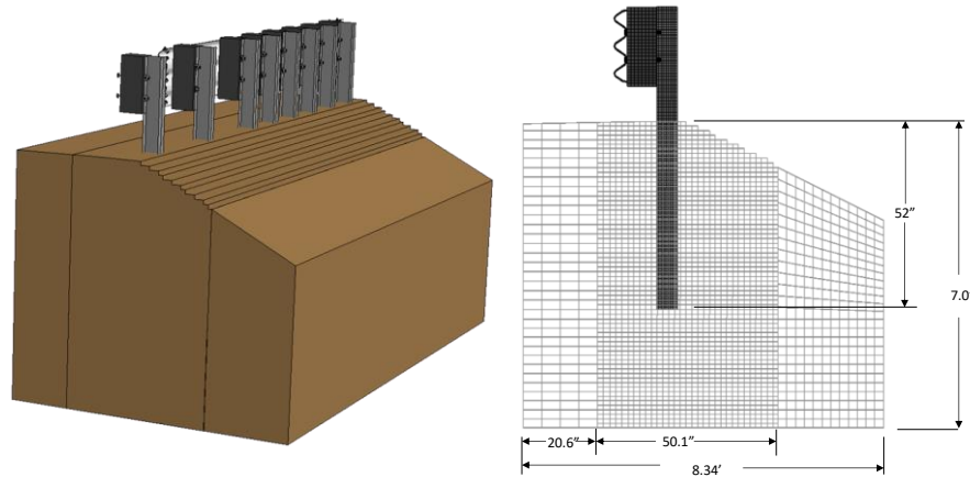
Figure 288. Soil continuum model from an oblique and section view.
