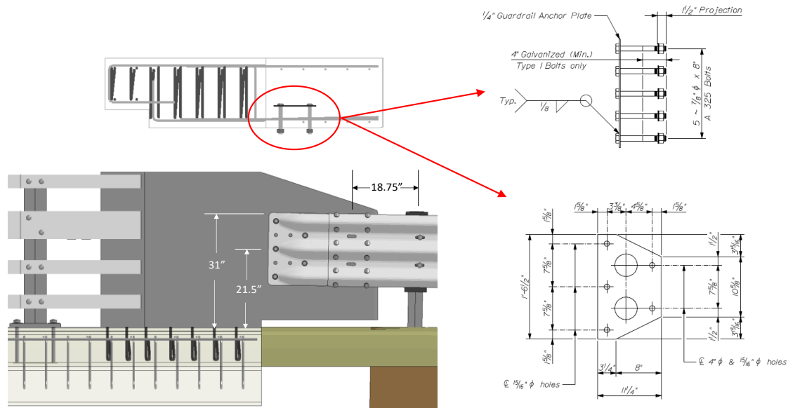
Figure 290. FEA model of buttress illustrating attachment details to thrie-beam and bridge deck.
