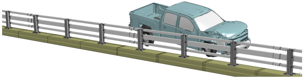
Figure K-3. [Continued] Sequential views from analysis of MASH Test 4-11 for NETC 3-Bar bridge rail from an oblique viewpoint.
