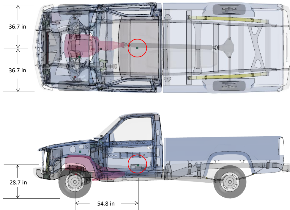
Figure 100. Location of accelerometer in the FE model.
