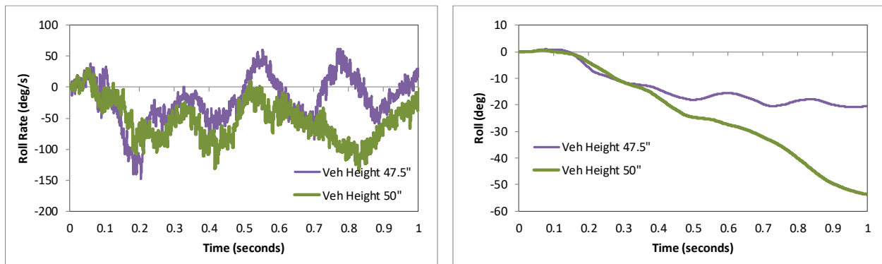
Figure 154. Roll rate and roll angle time-history from FEA of Test 4-12 on the NETC 3-bar bridge rail (cabin accelerometer).
