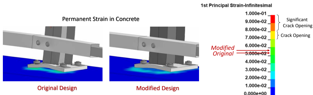
Figure 510. Contours of 1 st principal strains for concrete at the critical post for the original and modified design cases (permanent strains).
