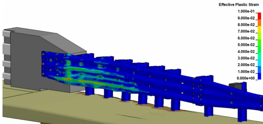
Figure 336. Contours of effective plastic strains on the steel rails and posts for Test 4-21 on MaineDOT transition.
