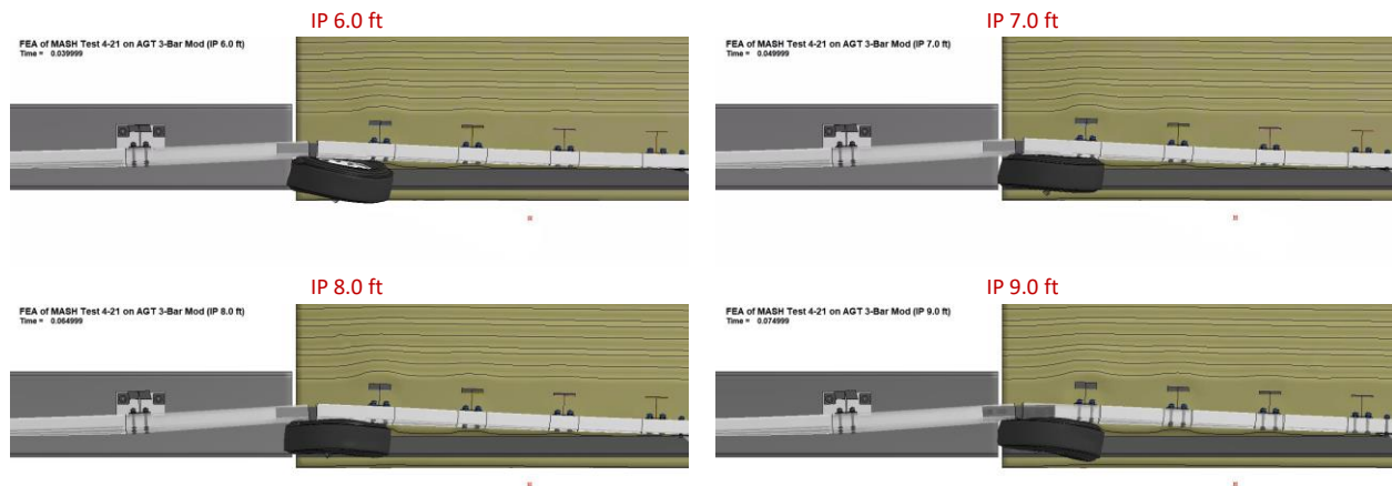
Figure 473. Test 4-21 results at time of impact with expansion splice (underneath view).
