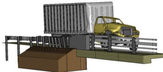
Figure V-3. [Continued] Sequential views from analysis of MASH Test 4-22 for AGT 4-Bar bridge rail from an oblique viewpoint.
