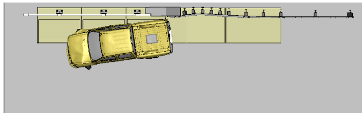
Figure U-1. [Continued] Sequential views from analysis of MASH Test 4-21 for AGT 4-Bar bridge rail from an overhead viewpoint.
