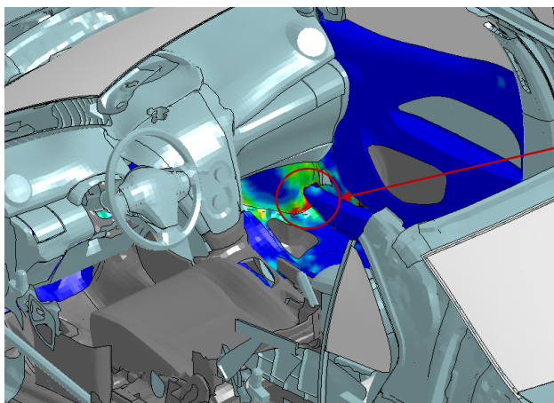
Figure 372. Occupant compartment deformation resulting from Test 3-10 on the NETC 2-bar bridge rail.
