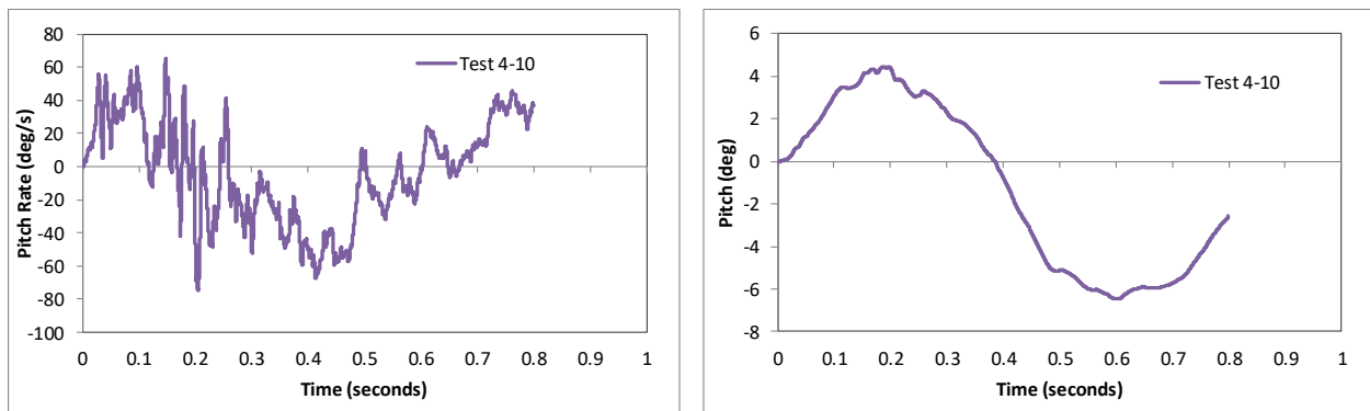
Figure 238. Pitch rate and pitch angle time-history from FEA of Test 4-10 on the NETC 4-bar bridge rail.
