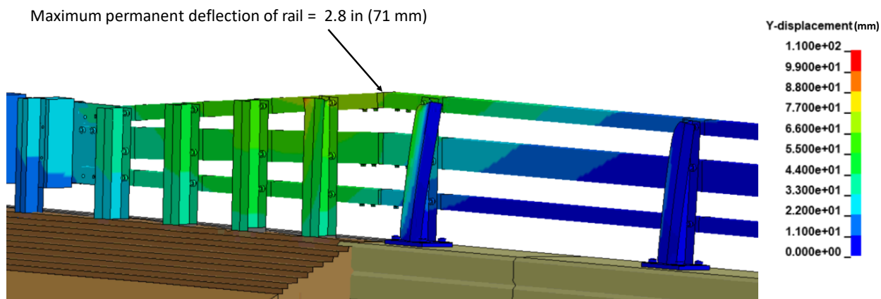
Figure 223. Contour plot of permanent deflection for the 3-bar transition for Test 4-22.
