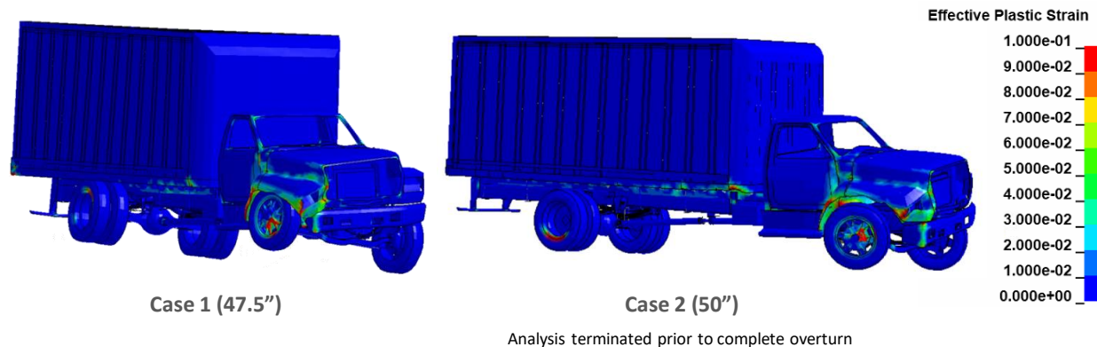
Figure 163. Damages to vehicle in Test 4-12 analysis of NETC 3-bar bridge rail for Cases 1 and 2.
