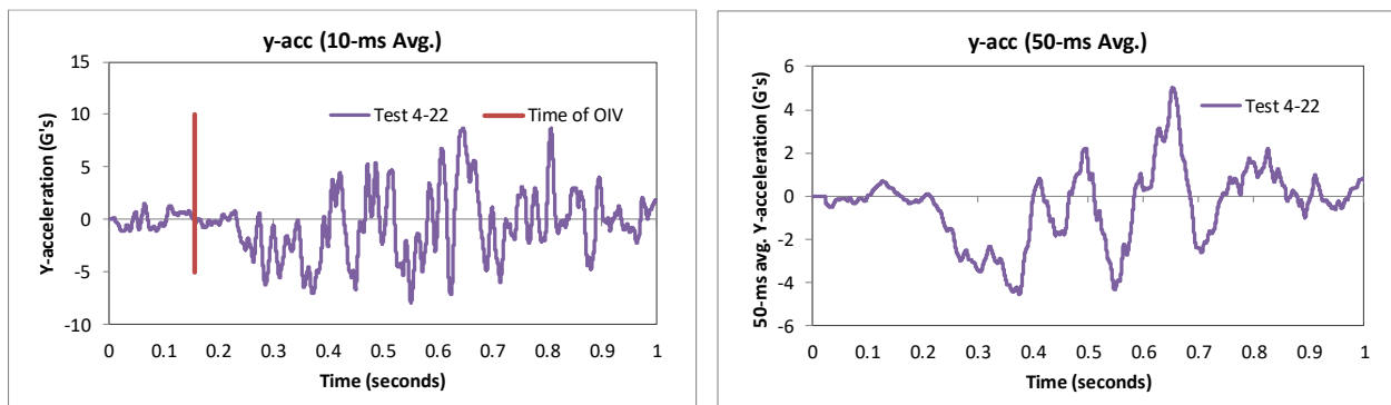
Figure 350. 10- and 50-millisecond average Y-acceleration from FEA of Test 4-22 on the MaineDOT transition (cabin accelerometer).
