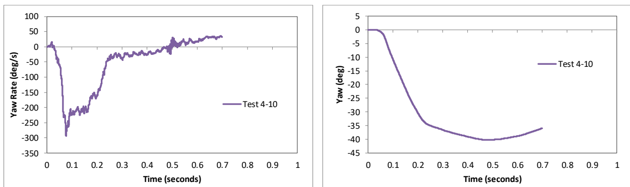
Figure 118. Yaw rate and yaw angle time-history from FEA of Test 4-10 on the NETC 3-bar bridge rail.
