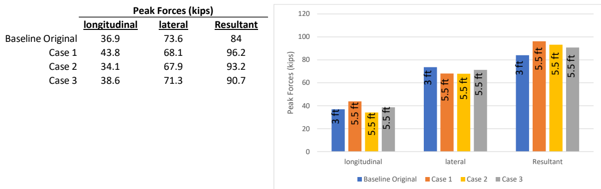
Figure 480. Peak impact forces on the barrier for Case 1 – 3 compared with baseline case.
