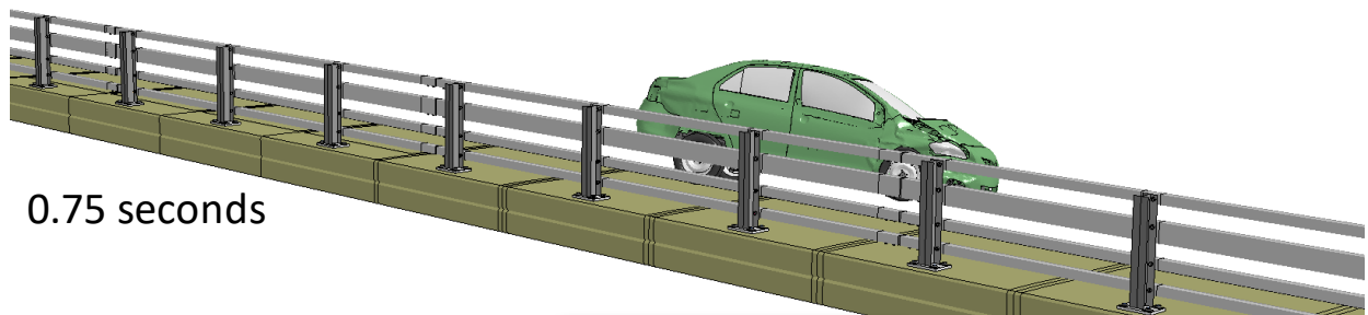
Figure Q-3. [Continued] Sequential views from analysis of MASH Test 4-10 for NETC 4-Bar bridge rail from an oblique viewpoint.
