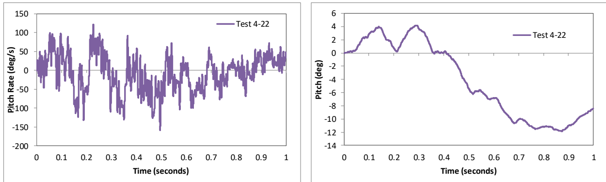
Figure 220. Pitch rate and pitch angle time-history from FEA of Test 4-22 on the 3-bar transition (cabin accelerometer).
