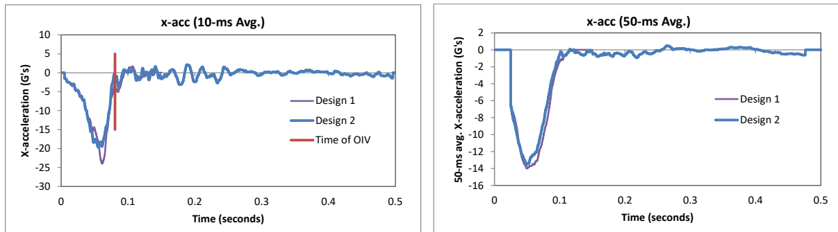
Figure 461. 10- and 50-millisecond average X-acceleration from FEA of Test 4-20 on the 3-bar transition with 5.5-ft post spacing.
