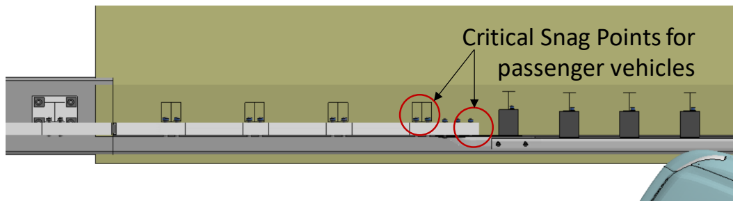
Figure 398. Illustration of potential snag points on the 2-bar transition for passenger vehicles.
