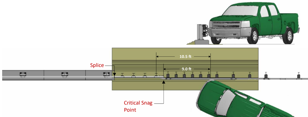
Figure 423. Impact point for Test 3-21 on the 2-bar transition.
