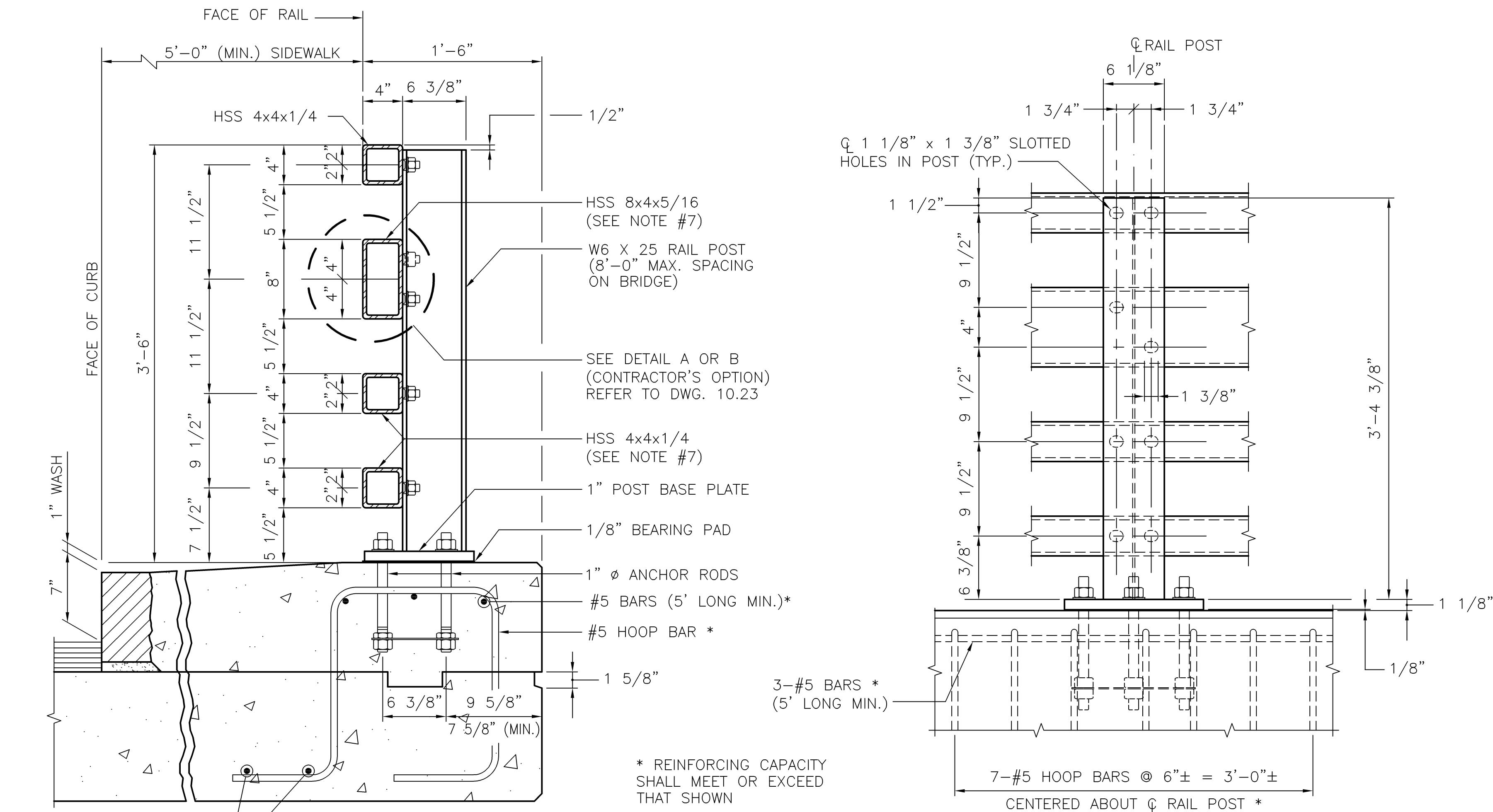
SECTION VIEW
