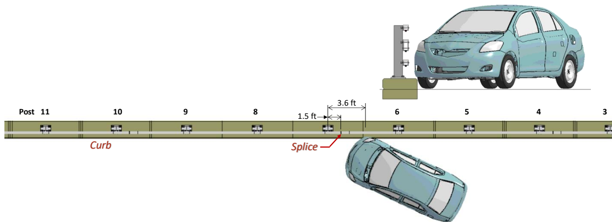
Figure 114. Impact point for Test 4-10 on the NETC 3-bar bridge rail.
