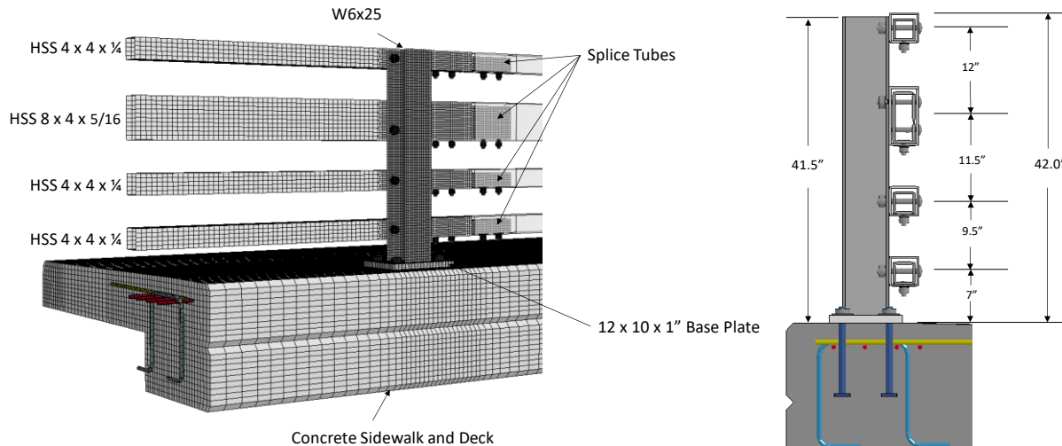
Figure 50. Representative section of the FEA model of the bridge rail.
