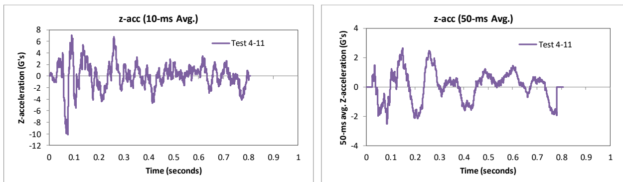
Figure 133. 10- and 50-millisecond average Z-acceleration from FEA of Test 4-11 on the NETC 3-bar bridge rail.
