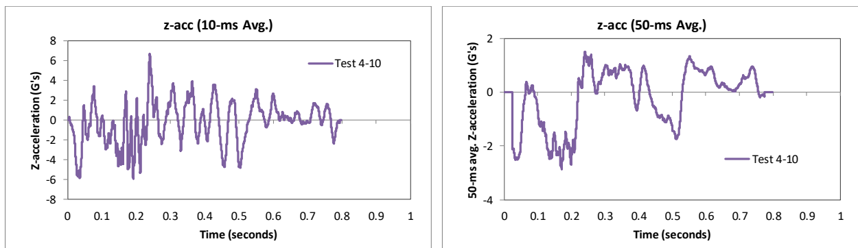
Figure 235. 10- and 50-millisecond average Z-acceleration from FEA of Test 4-10 on the NETC 4-bar bridge rail.
