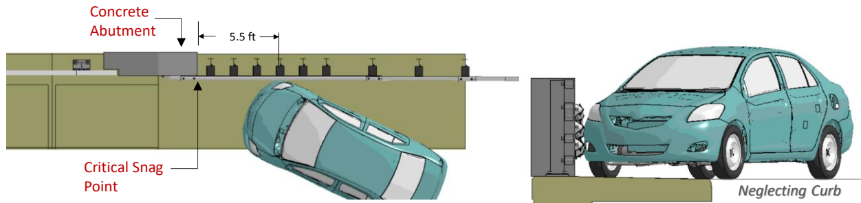
Figure 296. Impact point for Test 4-20 on the MaineDOT transition for 4-bar bridge rail.
