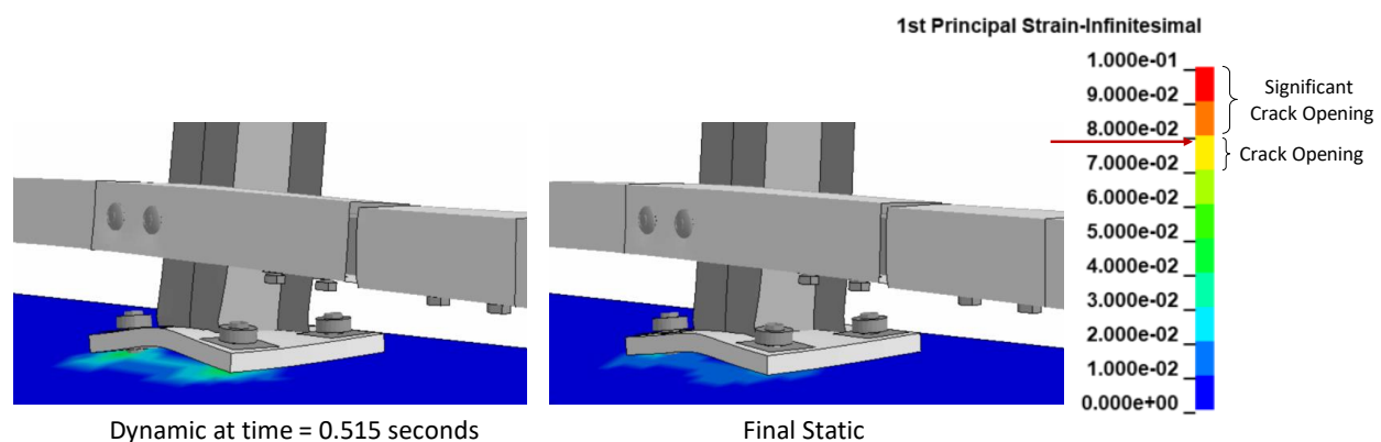
Figure 278. Contours of 1 st principal strains for concrete at the critical post for Test 4-12 on the NETC 4-bar bridge rail.
