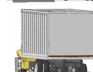
Figure 64. Sequential views of Test NETC-3 and FE analysis from upstream viewpoint.
