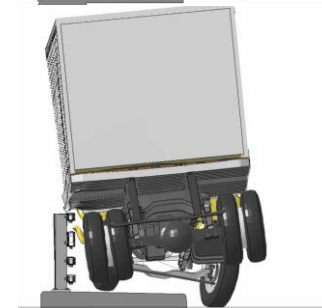
Figure 1. [Continued] Sequential views from FEA and Test NETC-3 from an upstream viewpoint.
