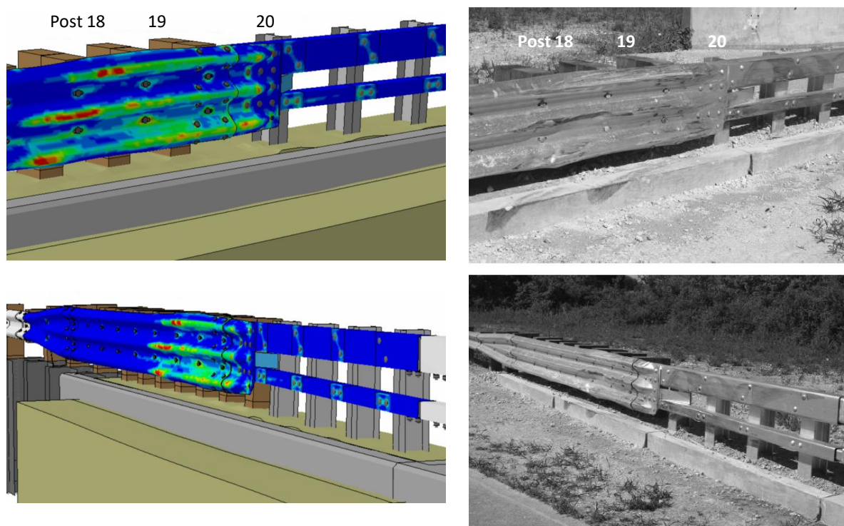
Figure 99. Comparing overall deformation of system for FEA and Test 401181-1.
