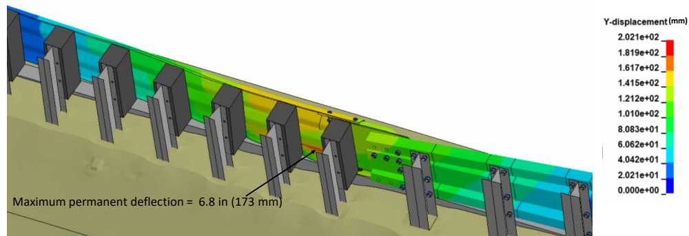
Figure 203. Contour plot of maximum permanent deflection for Test 4-21 on the 3-bar transition.
