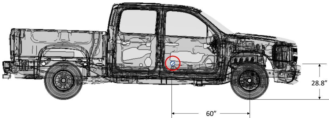
Figure 110. Location of c.g. in FEA model of 2270P vehicle.
