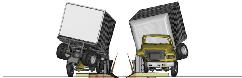
Figure V-2. [Continued] Sequential views from analysis of MASH Test 4-22 for AGT 4-Bar bridge rail from upstream and downstream viewpoints.
