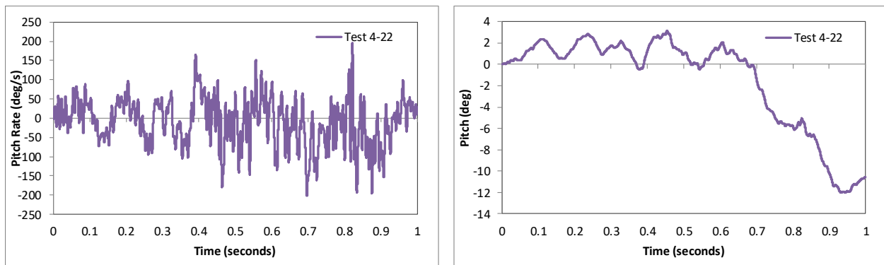
Figure 354. Pitch rate and pitch angle time-history from FEA of Test 4-22 on the MaineDOT transition (cabin accelerometer).
