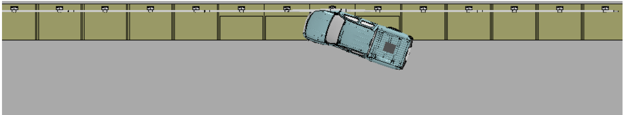
Figure R-1. Sequential views from analysis of MASH Test 4-11 for NETC 4-Bar bridge rail from an overhead viewpoint.
