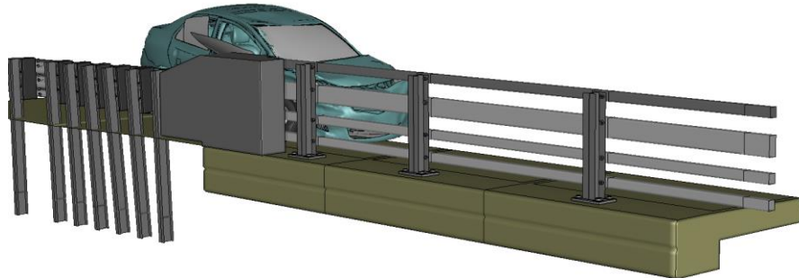
Figure T-3. Sequential views from analysis of MASH Test 4-20 for AGT 4-Bar bridge rail from an oblique viewpoint.
