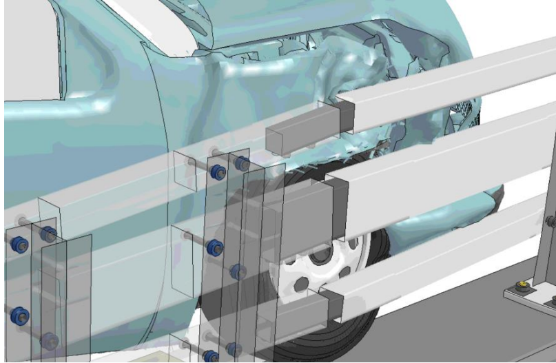
Figure 475. Closeup view of splice for Test 4-21 impact case IP 6.0 ft.
