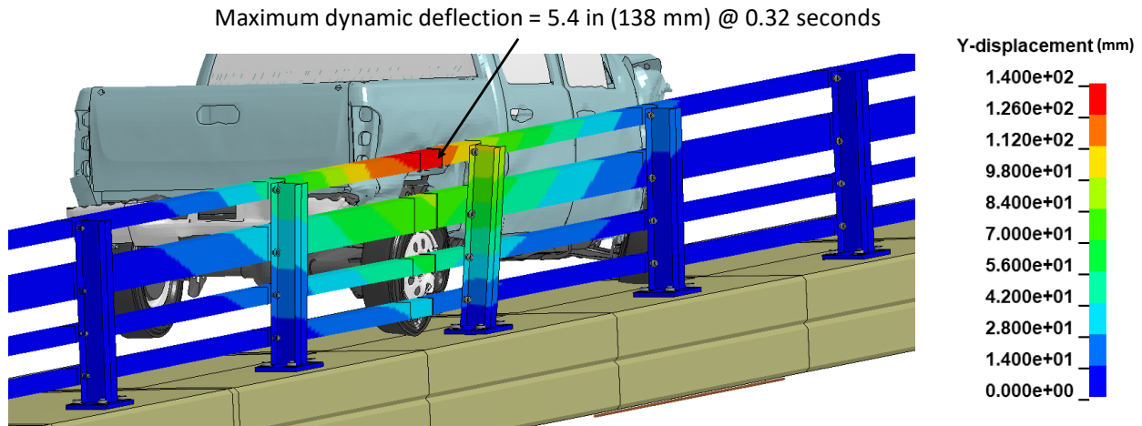
Figure 256. Contour plot of lateral displacement for the bridge rail for Test 4-11 at the time of maximum dynamic deflection.
