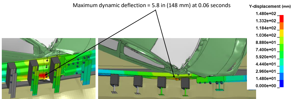
Figure 182. Contour plot of lateral displacement for the transition at the time of maximum dynamic deflection.
