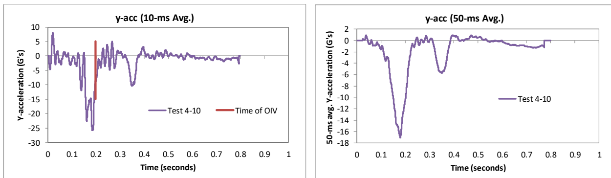
Figure 234. 10- and 50-millisecond average Y-acceleration from FEA of Test 4-10 on the NETC 4-bar bridge rail.
