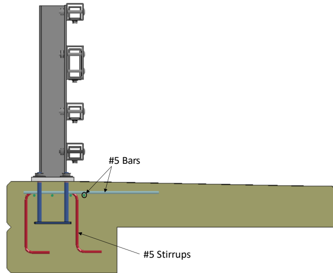
Figure 56. Profile view of sidewalk model.
