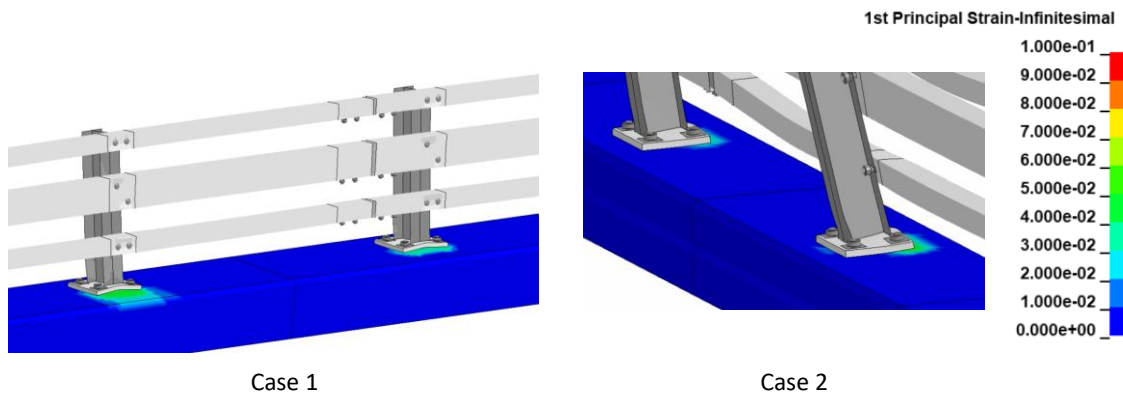
Figure 161. Contours of 1 st principal strains for concrete at the critical post for Test 4-12 on the NETC 3-bar bridge rail.
