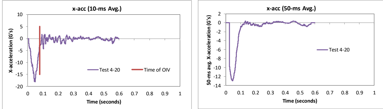
Figure 174. 10- and 50-millisecond average X-acceleration from FEA of Test 4-20 on the 3-bar transition.
