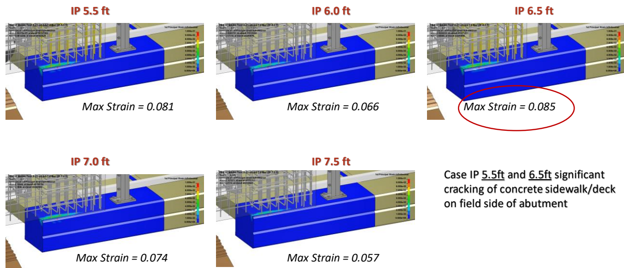
Figure 322. Contour plots of 1 st principle strain for the deck.
