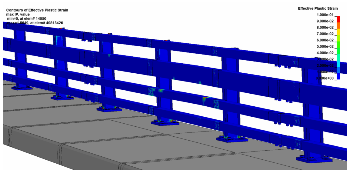
Figure 68. Contour plot of effective plastic strain showing deformations of the bridge rail model (traffic side).
