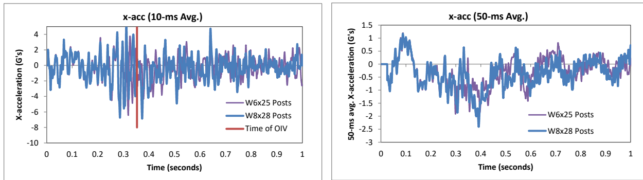
Figure 497. 10- and 50-millisecond average X-acceleration from FEA of Test 4-12 on the baseline and modified NETC 4-bar bridge rail (cabin accelerometer).
