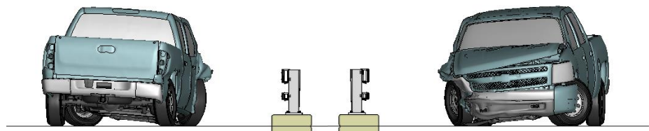
Figure X-2. [Continued] Sequential views from analysis of MASH Test 3-11 for NETC 2-Bar bridge rail from upstream and downstream viewpoints.
