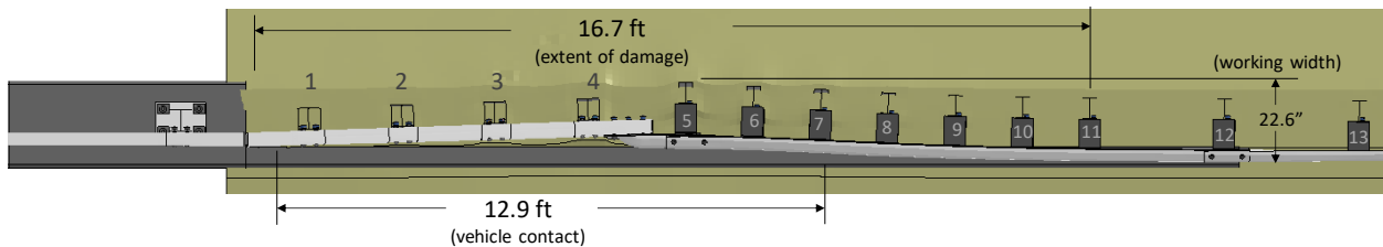
Figure 181. Overhead view of 3-bar transition after Test 4-20 showing extent of damage.
