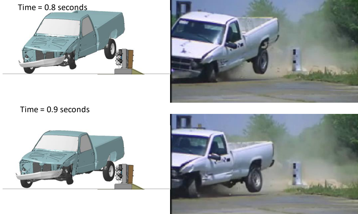
Figure 98. [Continued] Sequential views of FE analysis and Test 401181-1 from a downstream viewpoint.
