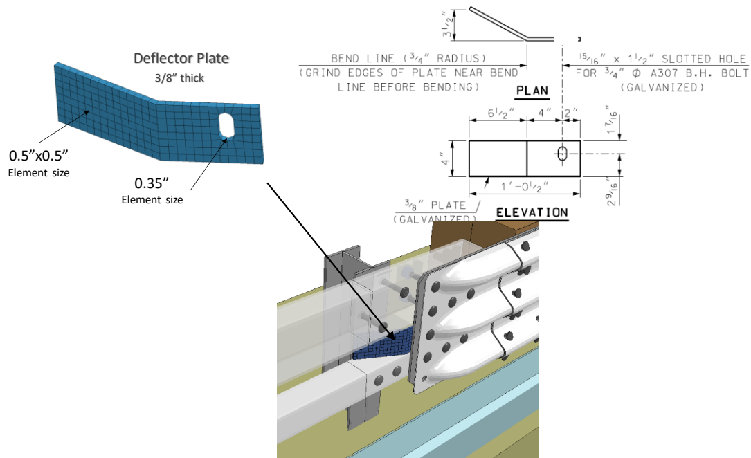
Figure 87. FEA mesh for the deflector plate.
