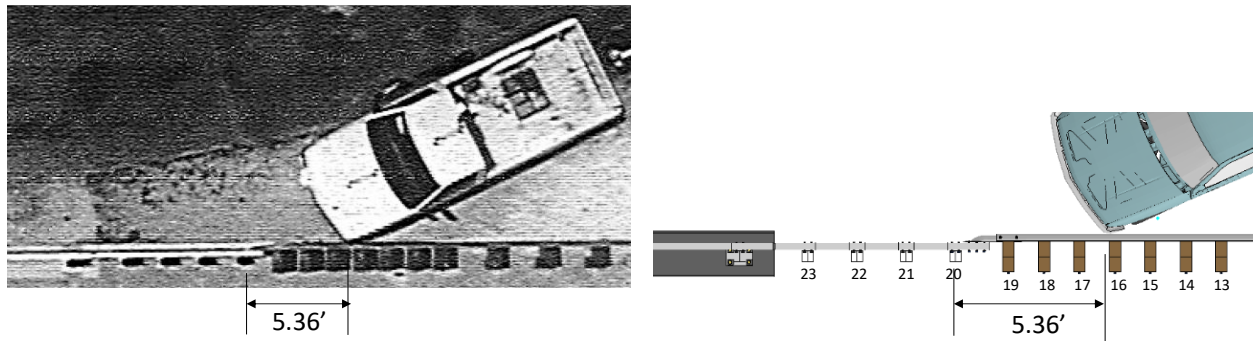
Figure 96. Impact point for test and simulation for Report 350 Test 3-21 on the 2-bar transition.
