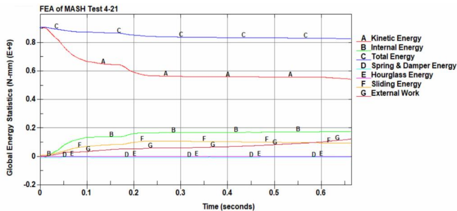
Figure 108. Plot of global energy-time histories from the analysis.
