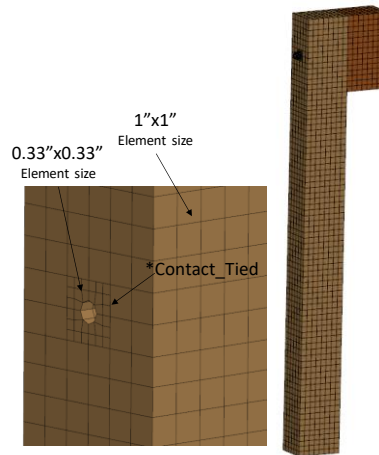
Figure 90. FEA model of wood AGT posts.
