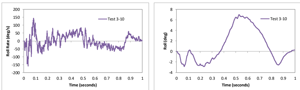
Figure 370. Roll rate and roll angle time-history from FEA of Test 3-10 on the NETC 2-bar bridge rail.
