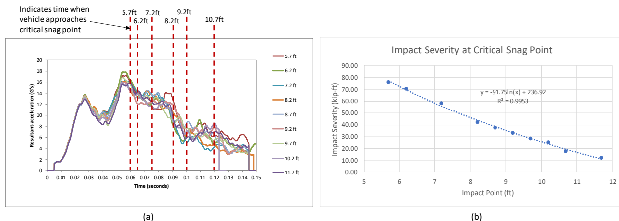
Figure 192. Plots of (a) vehicle accelerations and (b) impact severity at time when vehicle is positioned at critical snag point.
