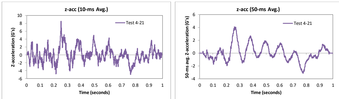
Figure 426. 10- and 50-millisecond average Z-acceleration from FEA of Test 3-21 on the 2-bar transition.
