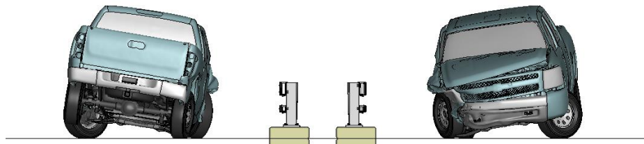
Figure X-2. [Continued] Sequential views from analysis of MASH Test 3-11 for NETC 2-Bar bridge rail from upstream and downstream viewpoints.
