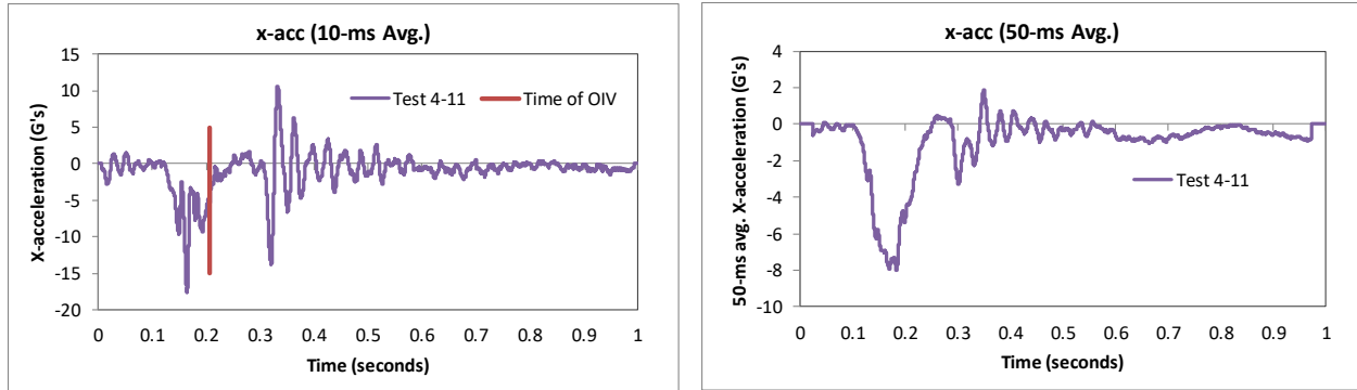
Figure 249. 10- and 50-millisecond average X-acceleration from FEA of Test 4-11 on the NETC 4-bar bridge rail.
