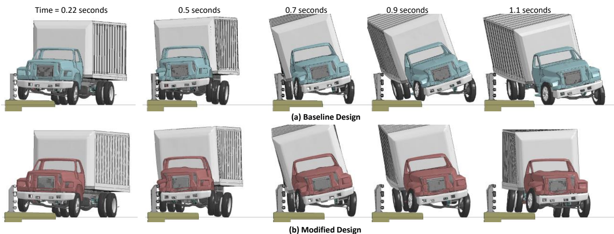
Figure 496. Sequential views for analyses of (a) baseline design and (b) modified design.
