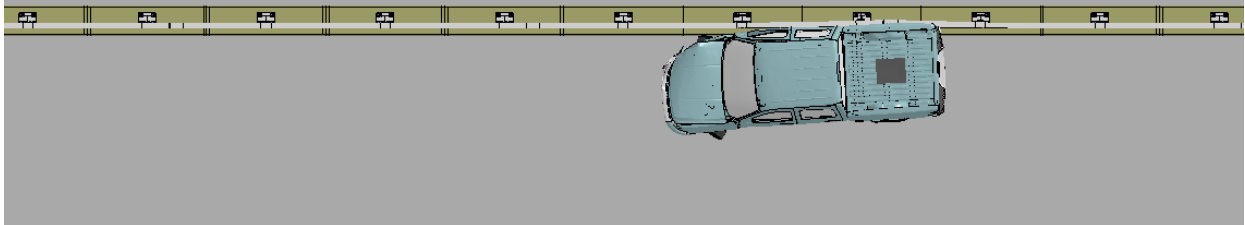
Figure K-1. Sequential views from analysis of MASH Test 4-11 for NETC 3-Bar bridge rail from an overhead viewpoint.
