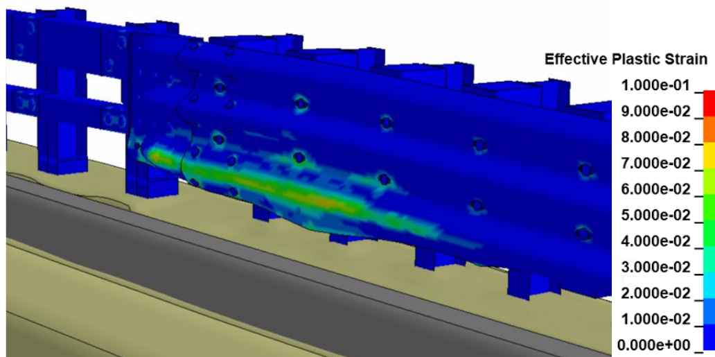
Figure 413. Contours of effective plastic strains on the steel rails and posts for 2-bar transition.
