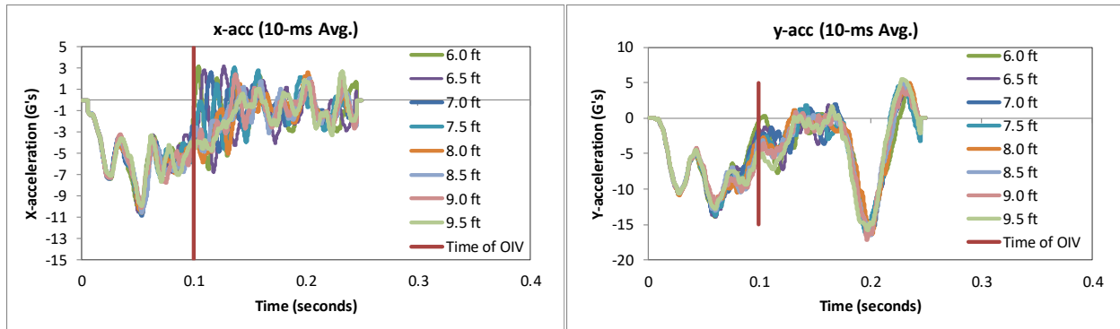
Figure 420. Plots of vehicle longitudinal and lateral accelerations measured at the c.g. of the vehicle.
