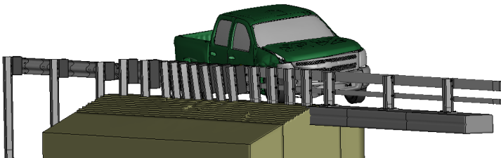
Figure Z-3. Sequential views from analysis of MASH Test 3-21 for AGT 2-Bar bridge rail from an oblique viewpoint.
