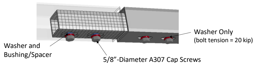
Figure 54. Updated model of rail splice used in MASH evaluations with rail-tube shown transparent.
