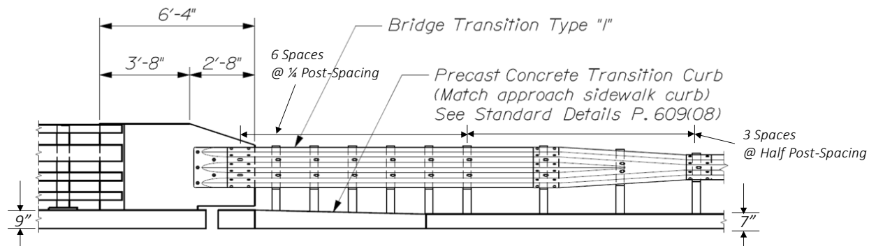
Figure 283. Elevation view of the concrete transition barrier for the NETC 4-bar bridge rail.
