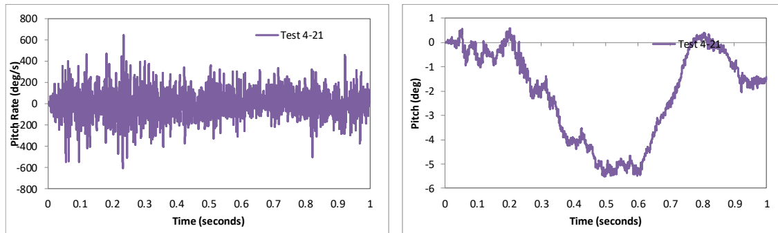
Figure 429. Pitch rate and pitch angle time-history from FEA of Test 3-21 on the 2-bar transition.
