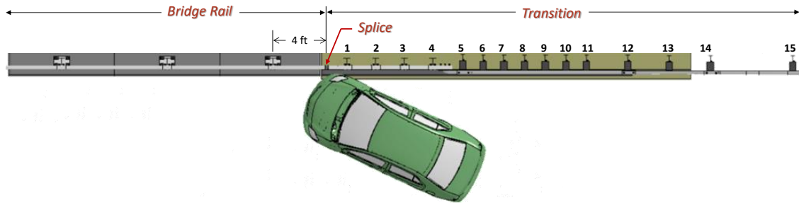
Figure 460. Impact point for Test 4-20 on Design Case 2.
