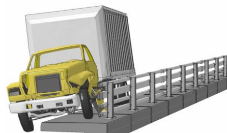
Figure 65. [CONTINUED] Sequential views of Test NETC-3 and FE analysis from downstream viewpoint.
