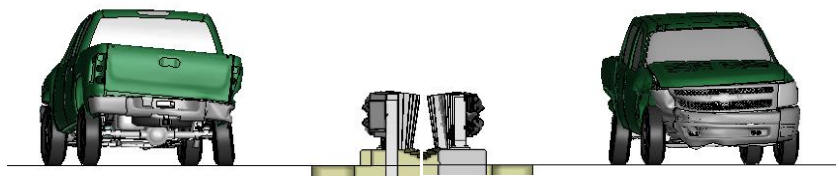
Figure Z-2. [Continued] Sequential views from analysis of MASH Test 3-21 for AGT 2-Bar bridge rail from upstream and downstream viewpoints.
