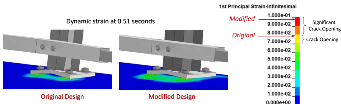
Figure 509. Contours of 1 st principal strains for concrete at the critical post for the original and modified design cases at time of peak dynamic strain.
