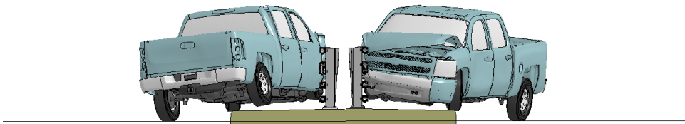
Figure R-2. Sequential views from analysis of MASH Test 4-11 for NETC 4-Bar bridge rail from upstream and downstream viewpoints.
