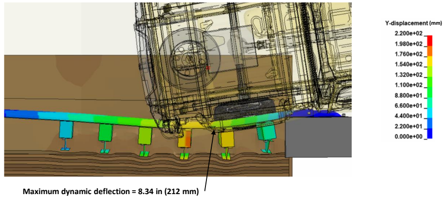
Figure 334. Contour plot of lateral displacement for Test 4-21 on the MaineDOT transition at maximum dynamic deflection.
