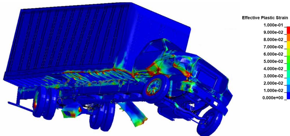
Figure 361. Damages to vehicle in Test 4-22 analysis of the MaineDOT transition.
