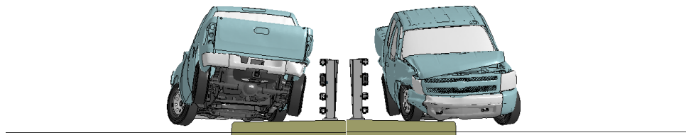
Figure R-2. [Continued] Sequential views from analysis of MASH Test 4-11 for NETC 4-Bar bridge rail from upstream and downstream viewpoints.
