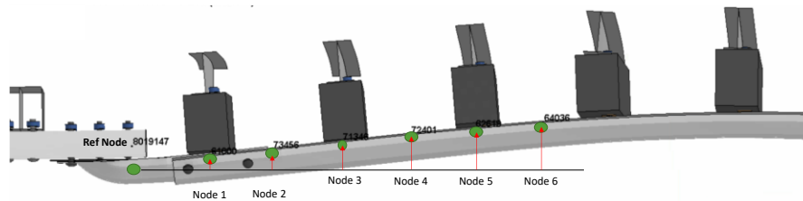
Figure 188. Measurement points for determining CIP for pocketing for Test 4-21.
