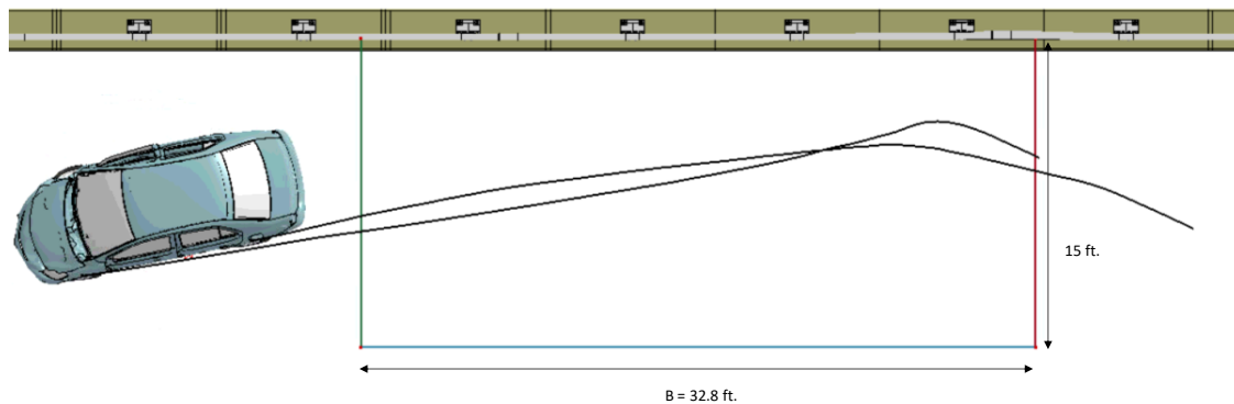
Figure 379. Exit box for Test 3-10 analysis of the NETC 2-bar bridge rail.
