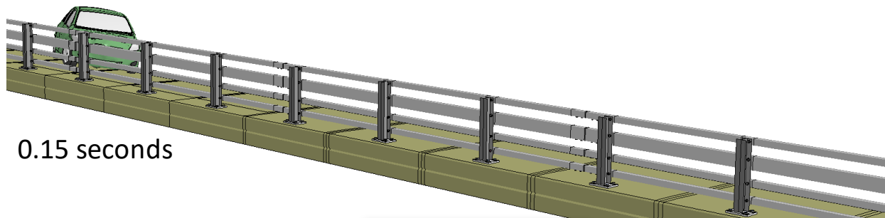
Figure Q-3. Sequential views from analysis of MASH Test 4-10 for NETC 4-Bar bridge rail from an oblique viewpoint.
