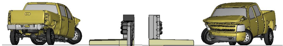
Figure U-2. [Continued] Sequential views from analysis of MASH Test 4-21 for AGT 4-Bar bridge rail from upstream and downstream viewpoints.
