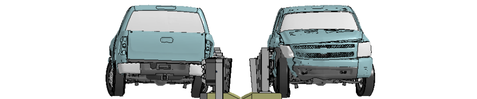
Figure O-2. Sequential views from analysis of MASH Test 4-21 for AGT 3-Bar transition from upstream and downstream viewpoints.
