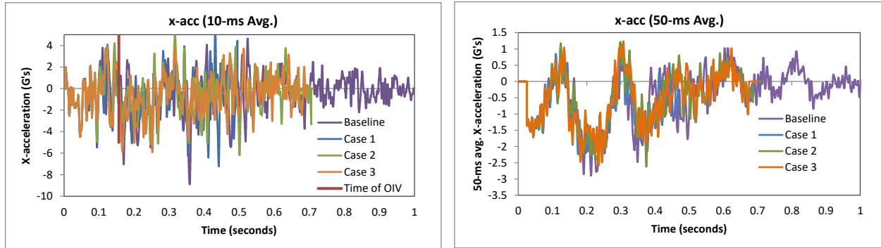
Figure 484. 10- and 50-millisecond average X-acceleration from FEA of Test 4-22 for Case 1-3 on the 3-bar transition with 5.5-ft post spacing compared with baseline (cabin accelerometer).
