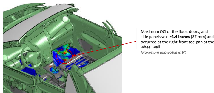
Figure 239. Occupant compartment deformation resulting from Test 4-10 on the NETC 4-bar bridge rail.
