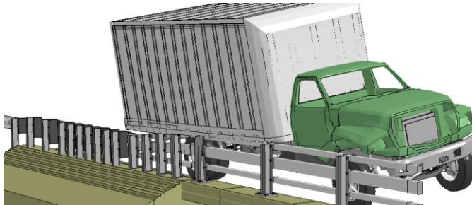
Figure P-3. [Continued] Sequential views from analysis of MASH Test 4-22 for AGT 3-Bar transition from an oblique viewpoint.
