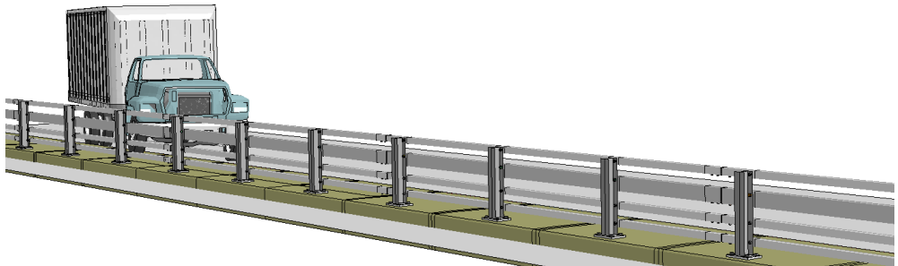
Figure S-3. Sequential views from analysis of MASH Test 4-12 for NETC 4-Bar bridge rail from an oblique viewpoint.
