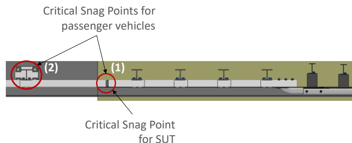
Figure 453. Critical impact point locations.
