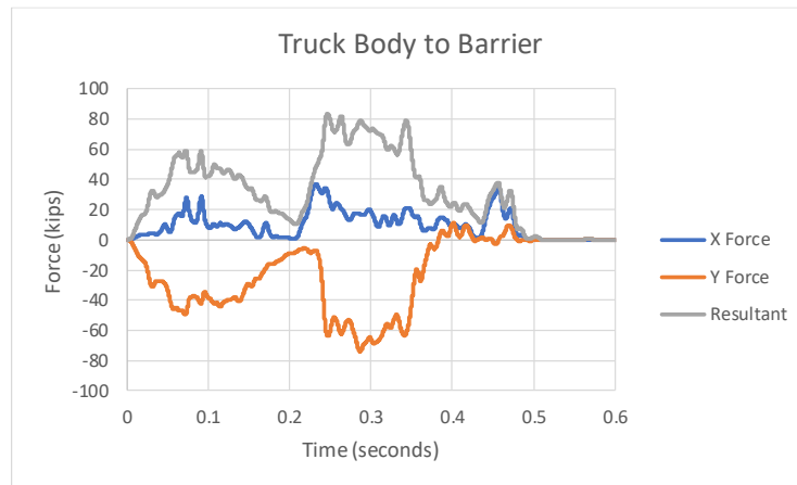
Figure 226. Longitudinal, lateral and resultant force-time history between vehicle and barrier for Test 4-22 on the 3-bar transition.
