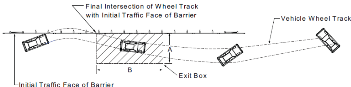
Figure 112. MASH exit box. [AASHTO16]
