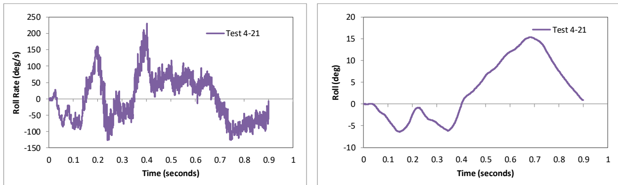
Figure 329. Roll rate and pitch angle time-history from FEA of Test 4-21 on the MaineDOT transition.
