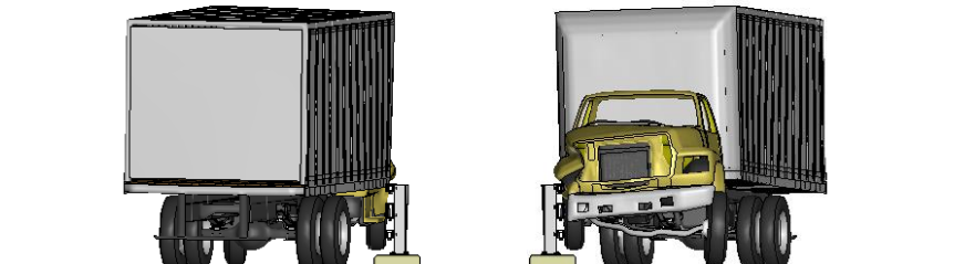
Figure K-2. Sequential views from analysis of MASH Test 4-12 for NETC 3-Bar bridge rail from upstream and downstream viewpoints – Case 1.
