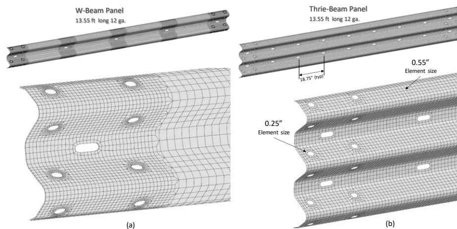
Figure 83: FEA mesh for (a) w-beam panel and (b) thrie-beam panel.
