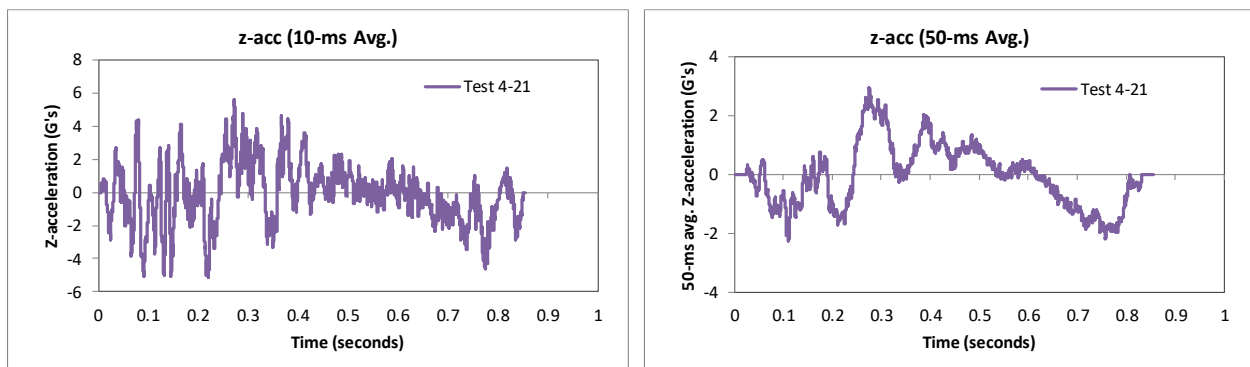
Figure 196. 10- and 50-millisecond average Z-acceleration from FEA of Test 4-21 on the 3-bar transition.
