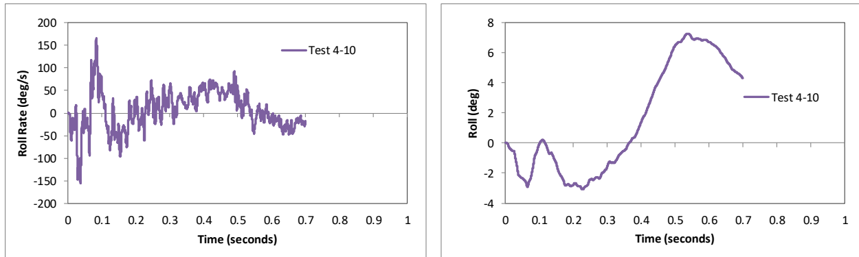
Figure 119. Roll rate and roll angle time-history from FEA of Test 4-10 on the NETC 3-bar bridge rail.
