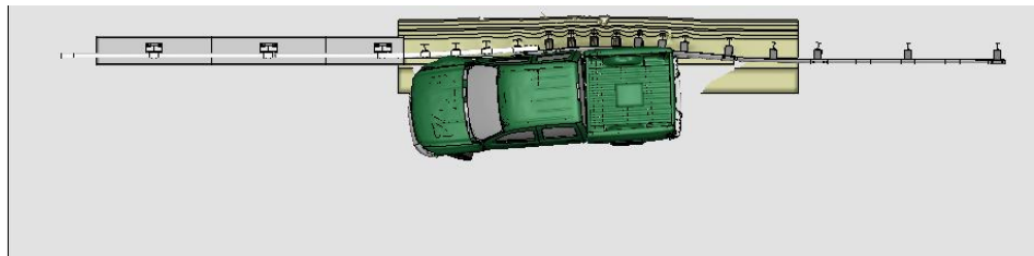
Figure Z-1. Sequential views from analysis of MASH Test 3-21 for AGT 2-Bar bridge rail from an overhead viewpoint.
