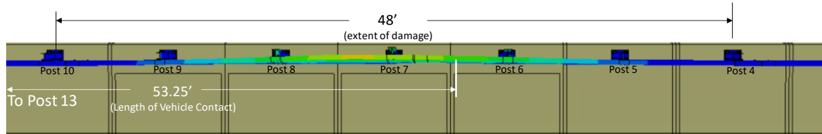
Figure 274. Extent of damage to the bridge rail for Test 4-12 on the NETC 4-bar bridge rail system.
