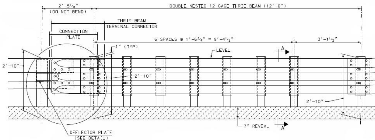
Figure 23. NHDOT T2 AGT double nested thrie-beam section.
