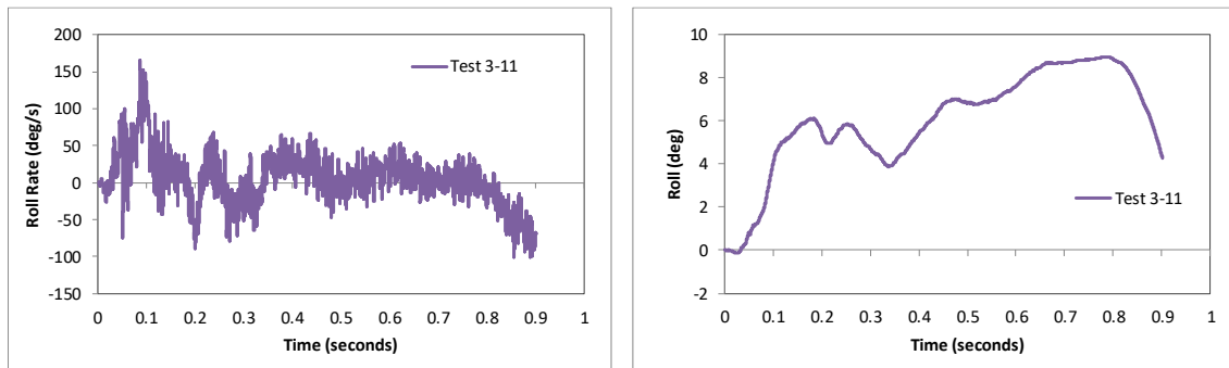
Figure 386. Roll rate and roll angle time-history from FEA of Test 3-11 on the NETC 2-bar bridge rail.
