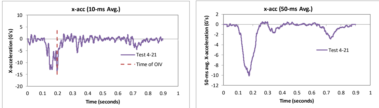
Figure 325. 10- and 50-millisecond average X-acceleration from FEA of Test 4-21 on the MaineDOT transition.
