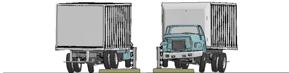
Figure S-2. [Continued] Sequential views from analysis of MASH Test 4-12 for NETC 4-Bar bridge rail from upstream and downstream viewpoints.
