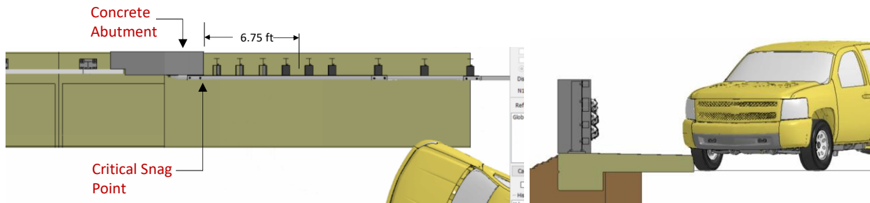
Figure 323. Starting point and target impact point for Test 4-21 on the MaineDOT transition for 4-bar bridge rail.
