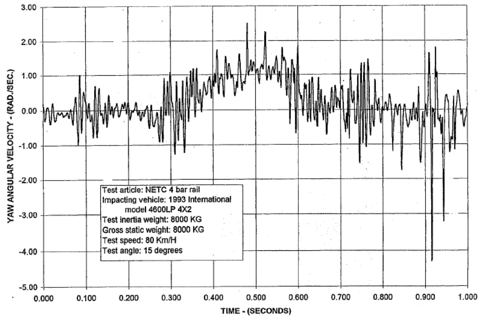
Figure 62. Yaw-rate measured at vehicle c.g. in Test NETC-3.[ Kimball99]
