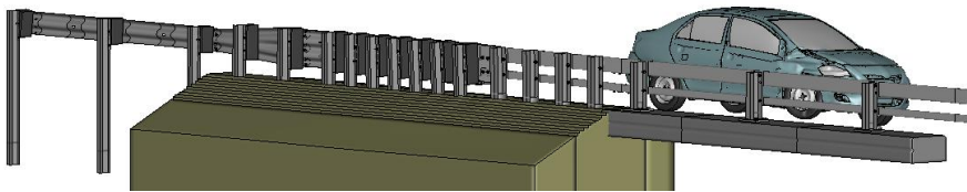
Figure Y-3. [Continued] Sequential views from analysis of MASH Test 3-20 for AGT 2-Bar bridge rail from an oblique viewpoint.
