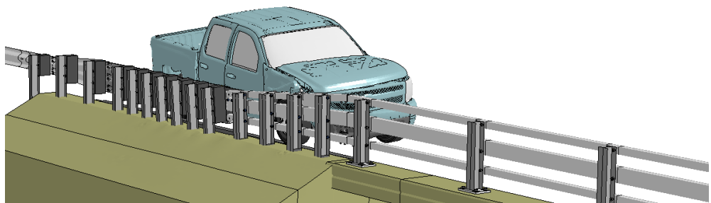
Figure O-3. Sequential views from analysis of MASH Test 4-21 for AGT 3-Bar transition from an oblique viewpoint.
