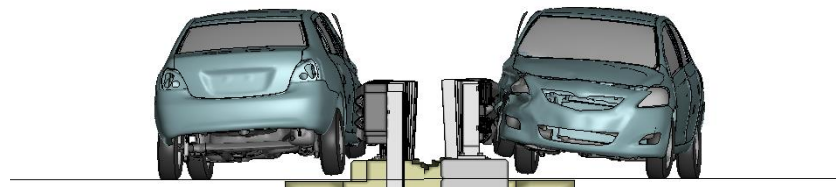
Figure Y-2. Sequential views from analysis of MASH Test 3-20 for AGT 2-Bar bridge rail from upstream and downstream viewpoints.
