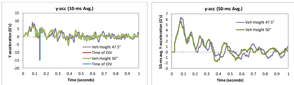
Figure 151. 10- and 50-millisecond average Y-acceleration from FEA of Test 4-12 on the NETC 3-bar bridge rail (cabin accelerometer).
