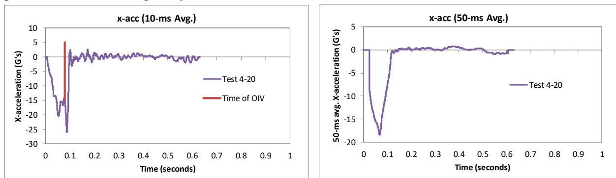
Figure 297. 10- and 50-millisecond average X-acceleration from FEA of Test 4-20 on the MaineDOT transition.
