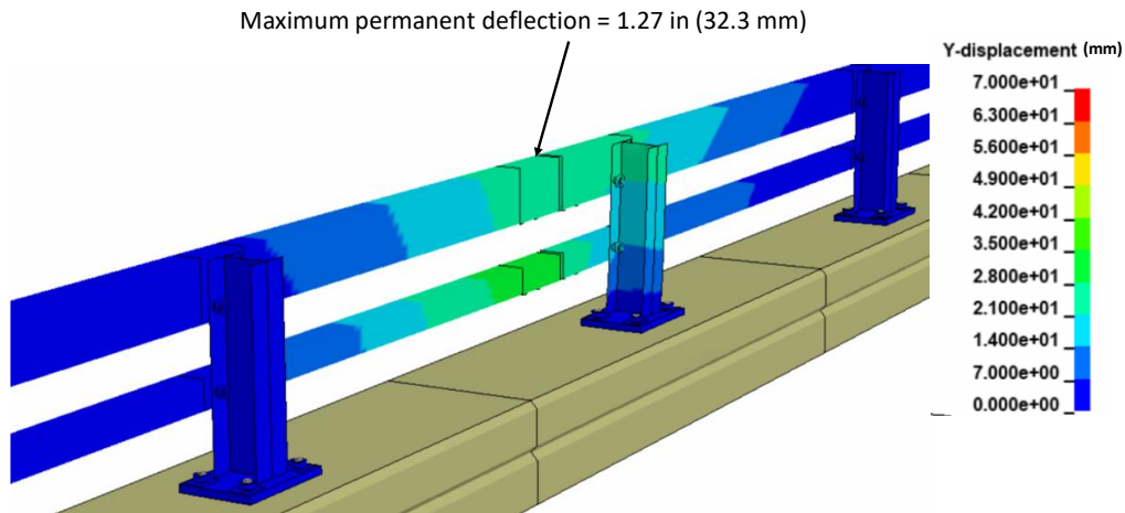
Figure 391. Contour plot of maximum permanent deflection of the NETC 2-bar bridge rail for test 3-11.
