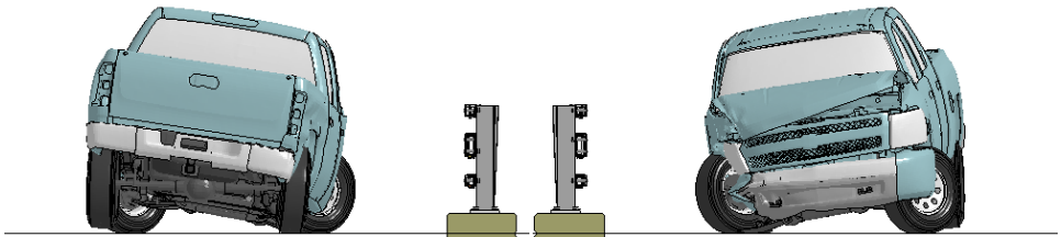
Figure K-2. [Continued] Sequential views from analysis of MASH Test 4-11 for NETC 3-Bar bridge rail from upstream and downstream viewpoints.
