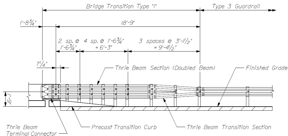
Figure 284. MaineDOT Bridge Transition Type 1.
