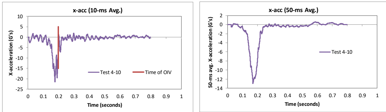
Figure 233. 10- and 50-millisecond average X-acceleration from FEA of Test 4-10 on the NETC 4-bar bridge rail.
