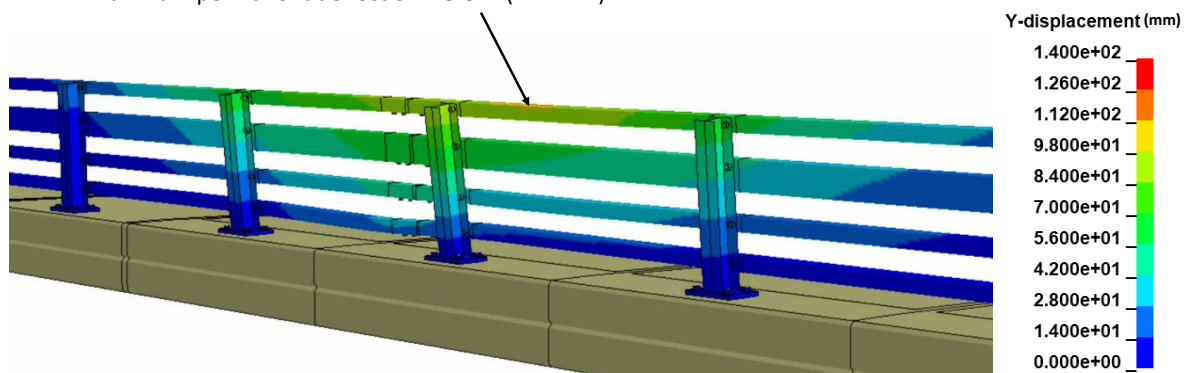
Figure 276. Contour plot of permanent deflection for the bridge rail from Test 4-12 for the NETC 4-bar bridge rail.
