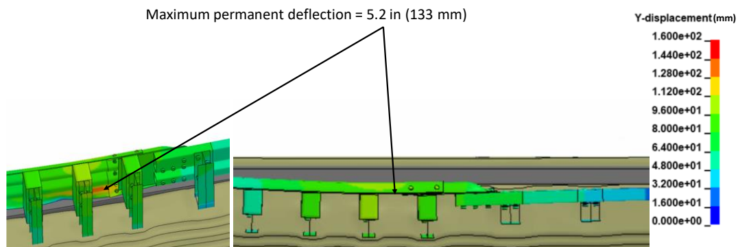
Figure 412. Contour plot of maximum permanent deflection for the transition.
