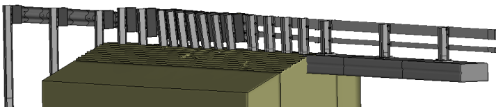
Figure Z-3. [Continued] Sequential views from analysis of MASH Test 3-21 for AGT 2-Bar bridge rail from an oblique viewpoint.
