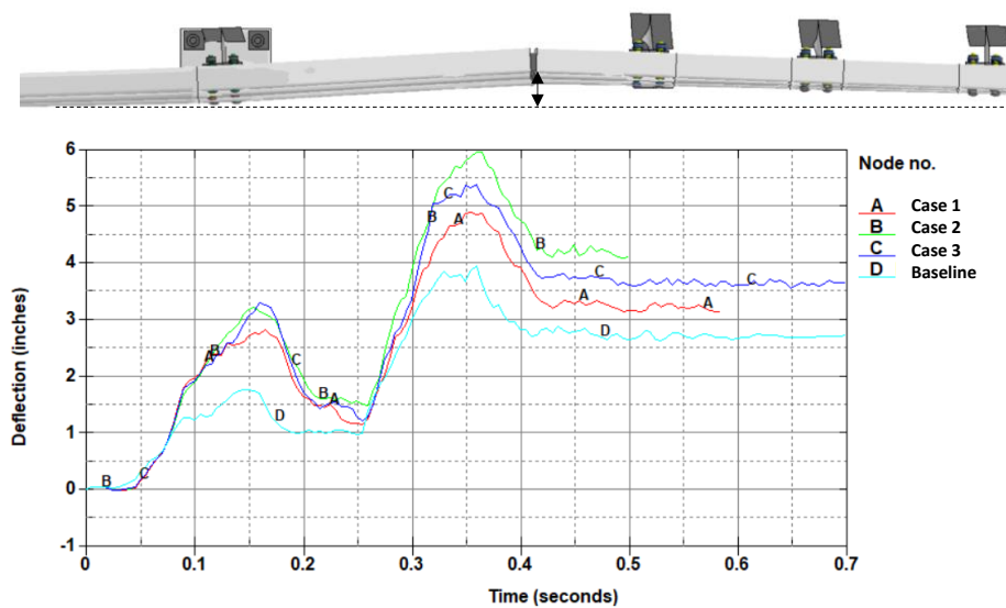
Figure 490. Deflection-time history at expansion splice for Cases 1-3 compared with baseline case.
