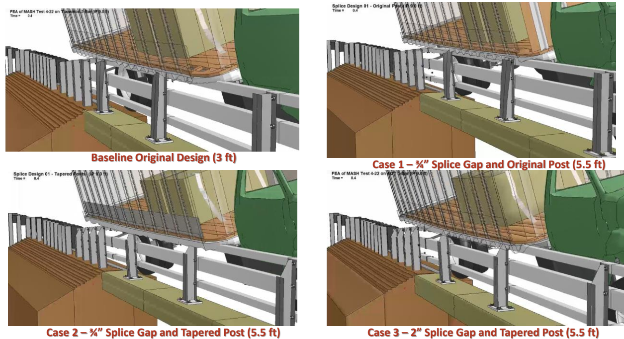
Figure 479. Images of the analysis results for Cases 1 – 3 compared to the baseline case at 0.4 seconds of the impact (cargo box transparent).
