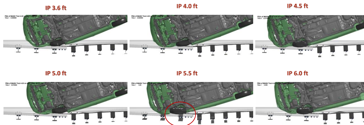
Figure 172. Results of Test 4-20 CIP evaluations for the 3-bar Transition.
