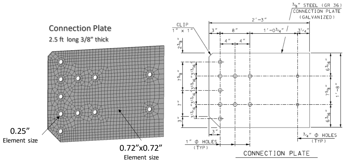
Figure 86. FEA mesh for the connection plate.
