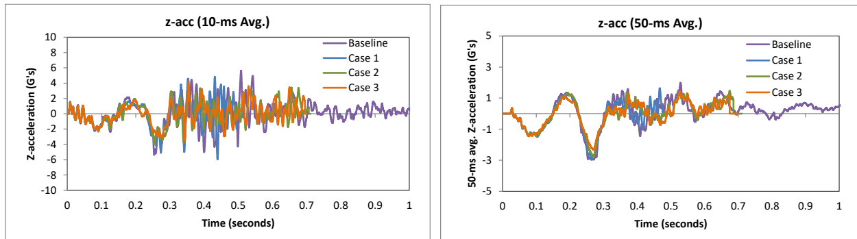
Figure 483. 10- and 50-millisecond average Z-acceleration from FEA of Test 4-22 for Case 1-3 on the 3-bar transition with 5.5-ft post spacing compared with baseline (c.g. accelerometer).
