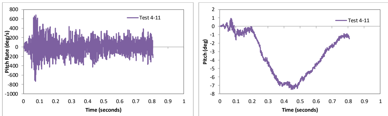
Figure 136. Pitch rate and pitch angle time-history from FEA of Test 4-11 on the NETC 3-bar bridge rail.
