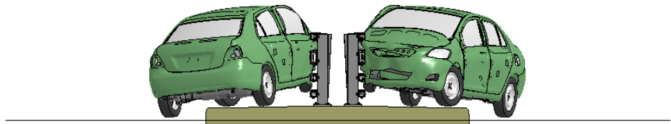
Figure Q-2. Sequential views from analysis of MASH Test 4-10 for NETC 4-Bar bridge rail from upstream and downstream viewpoints.
