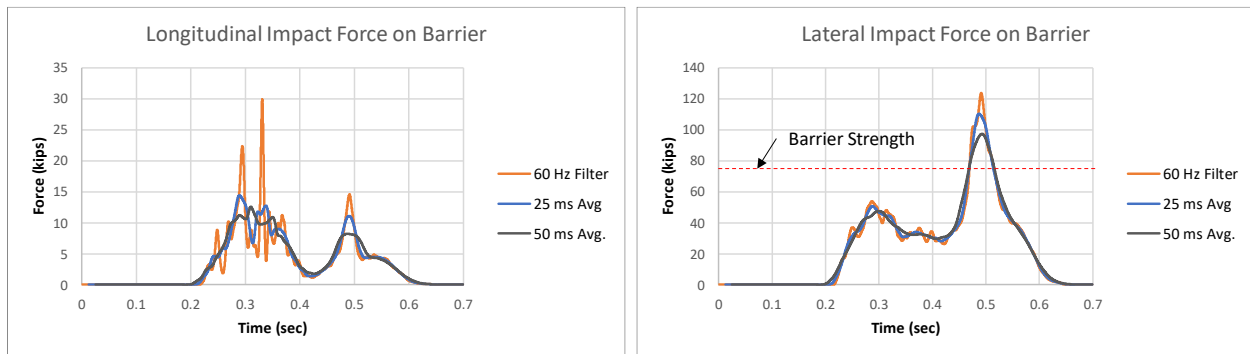
Figure 279. Longitudinal and lateral force-time history between vehicle and barrier for Test 4-12 on NETC 4-bar bridge rail.
