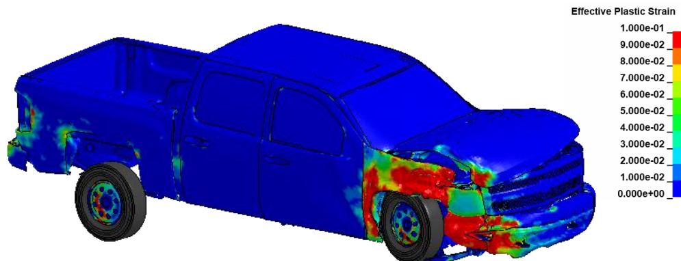
Figure 143. Damages to vehicle in Test 4-11 analysis of the NETC 3-bar bridge rail.
