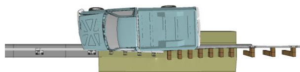
Figure 97. Sequential views of FE analysis and Test 401181-1 from an overhead viewpoint.
