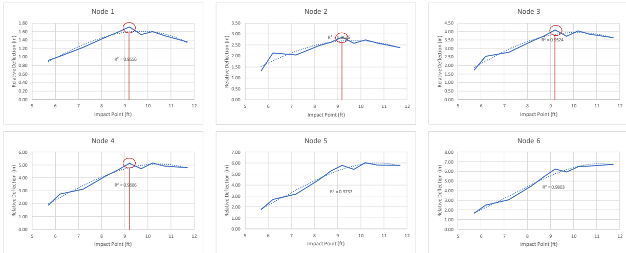
Figure 190. Plots of relative displacements for Test 4-21 simulations in CIP evaluations.
